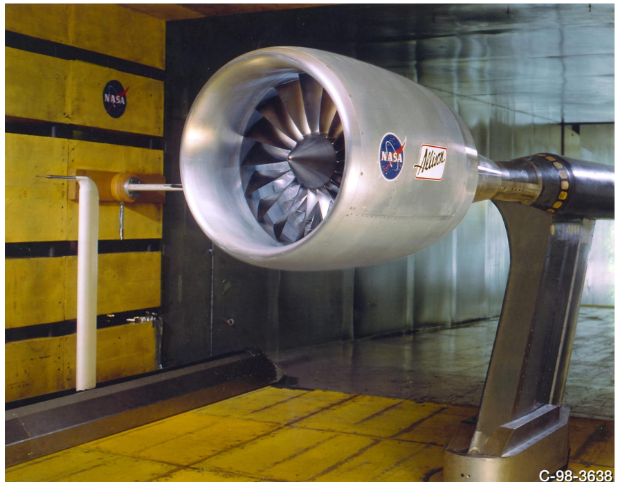
NASA/Allison Engine Company Low Noise Fan test in Lewis' 9- by 15-Foot Low-Speed Wind Tunnel.
