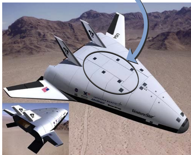
VentureStar reusable launch vehicle, showing where the titanium aluminide metallic thermal protection system will be used.
