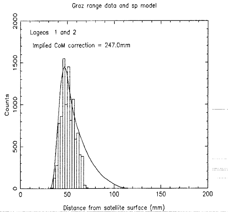
Figure 3.5-2. Comparison of Graz data distribution with single-photon empirical model.
