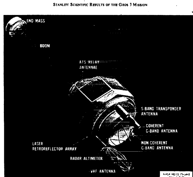
Fig. 1. Artist concept of Geos 3 spacecraft.
