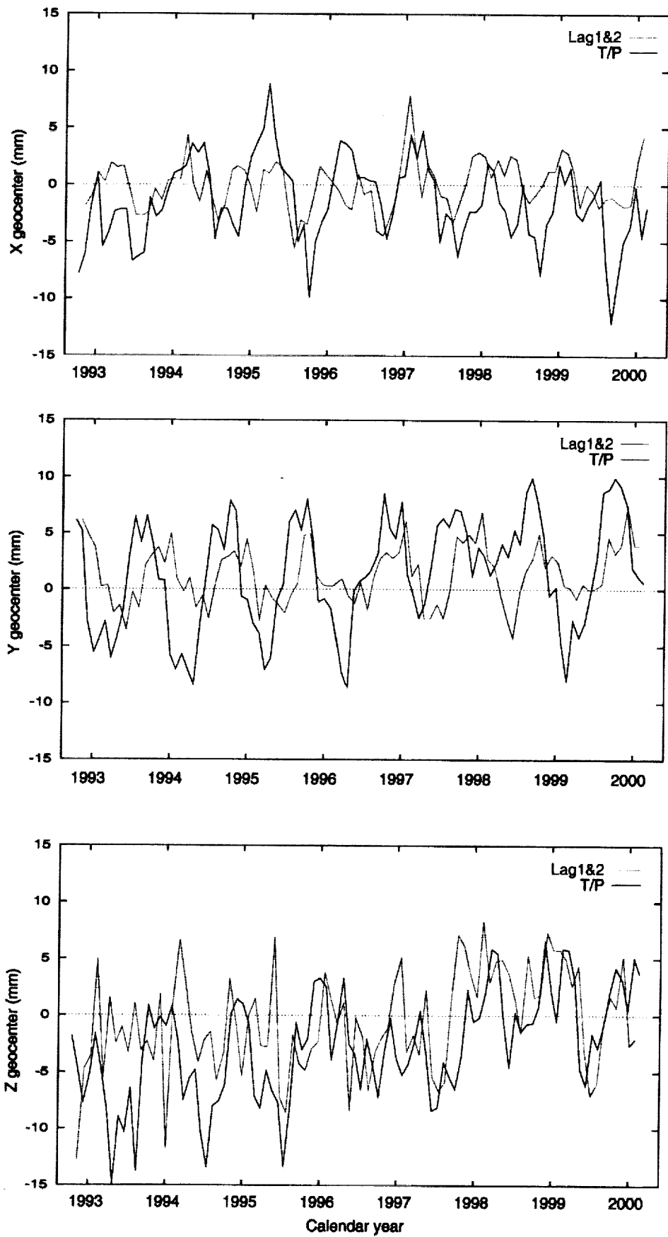
Figure 7.1.1.1-1 Geocenter motion determined by LAGEOS-1/2 and TOPEX/POSEIDON
