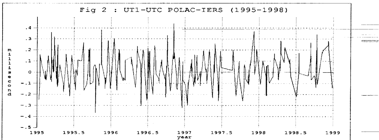
Figure 7.2.2.1-2 The precision of the determination is about 0.20 ms for UT0-UTC and 3.0 mas for VOL.
