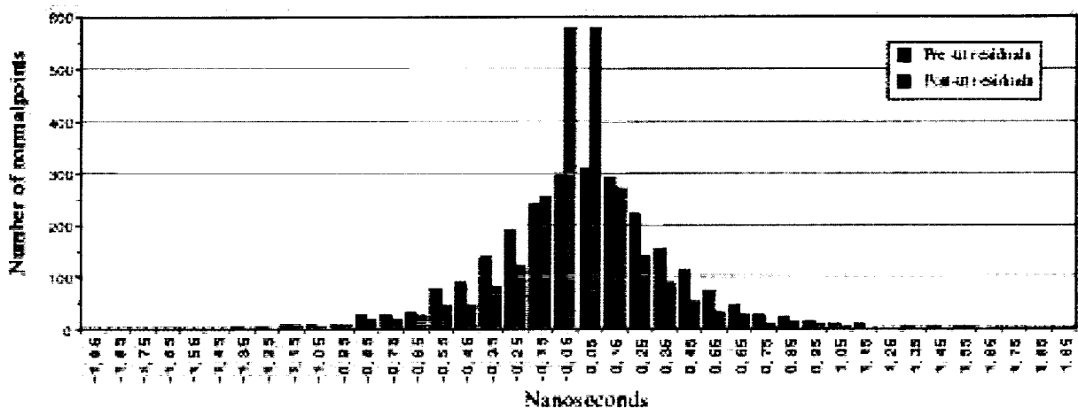
Figure 7.2.2.4-2 The distribution of the pre- and post UT0-UTC determination of MLRS residuals
