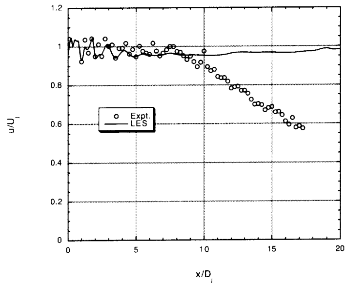
Figure 7.18: Time averaged centerline velocity profile for the axisymmetric LES solution
