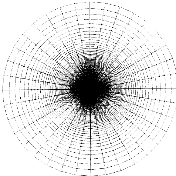
(b) crossstream, y-z plane at outflow boundary
