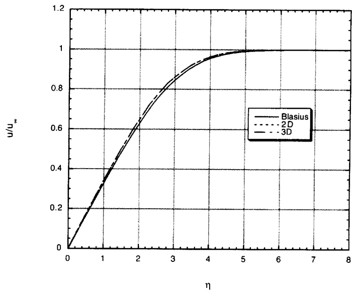
(b) velocity profiles at Re_x = 4000
