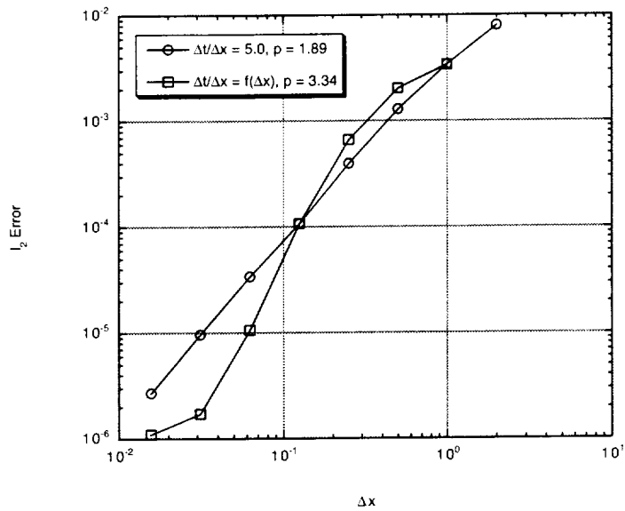
Figure 4.8: Improved spatial error of Gottlieb-Turkel scheme for the smooth nonlinear problem
