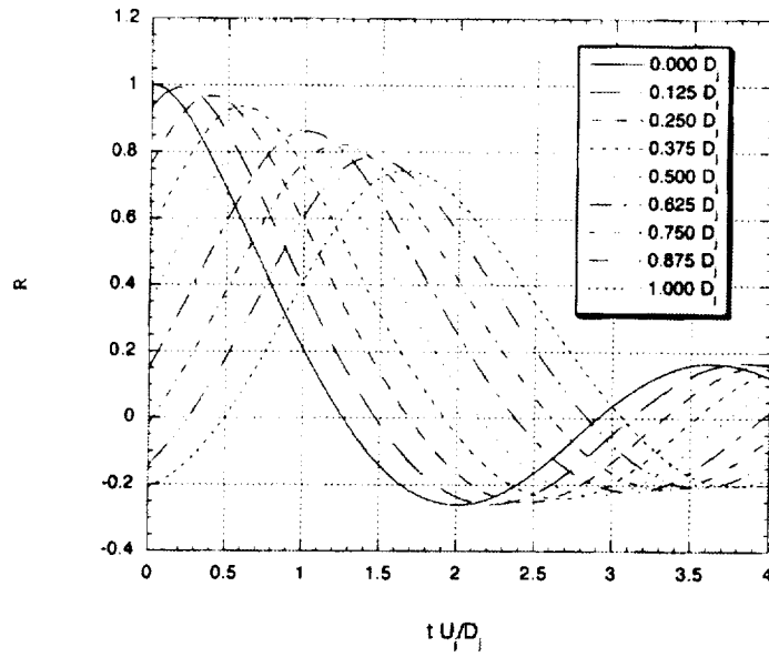
(b) 45 degrees
