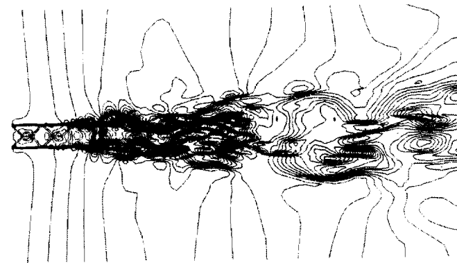
(c) \frac{tD_j}{U_j} = 32.297
