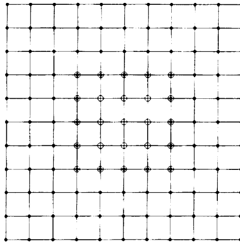
(c) grid point specification (filled = active, open = hole, both = boundary)
