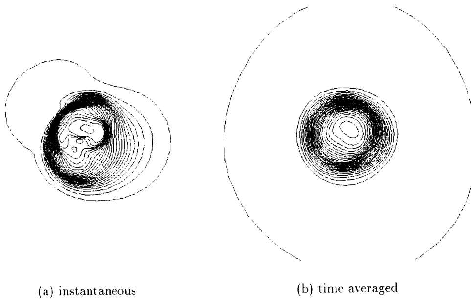
Figure 7.25: Total velocity contours at x/D_j = 6 for 3D LES solution
