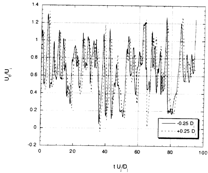
(a) 0 degrees
