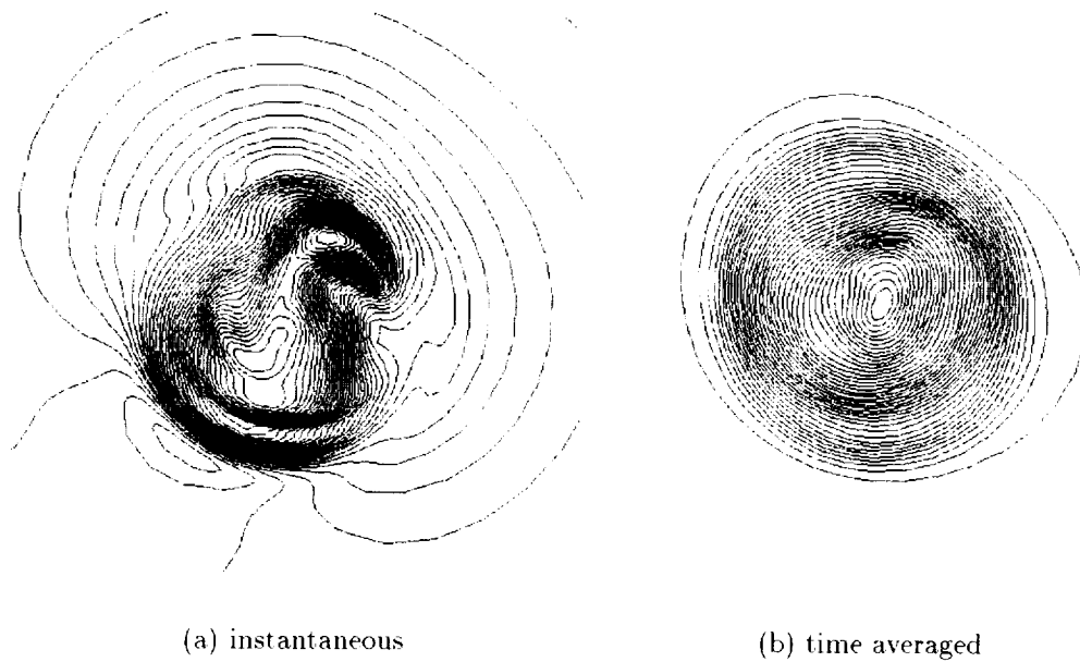
Figure 7.26: Total velocity contours at x/D_j = 9 for 3D LES solution
