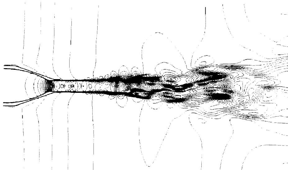
(a) instantaneous
