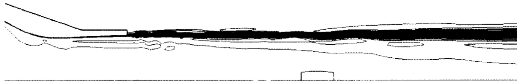
(a) Coarse grid
