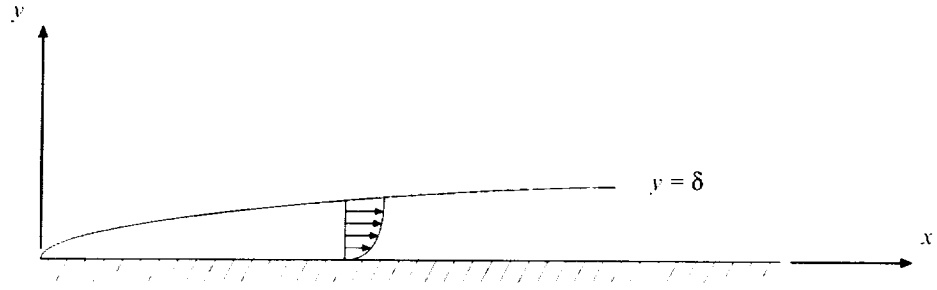
Figure 6.6: 2D laminar flat plate
