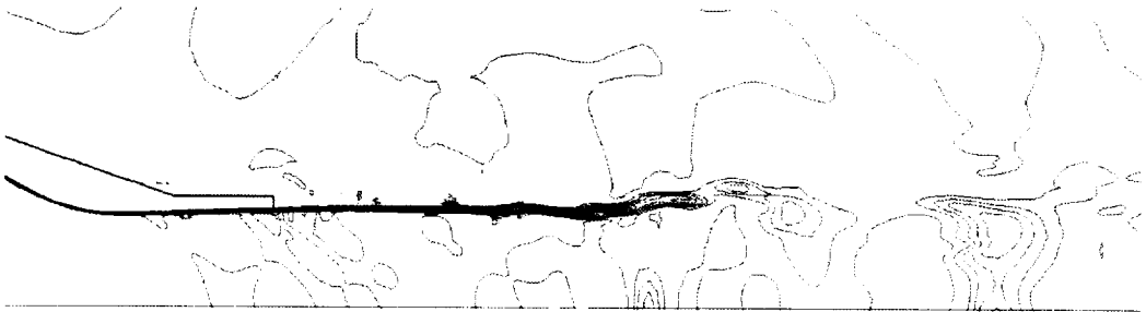
(b) sub-grid turbulent kinetic energy
