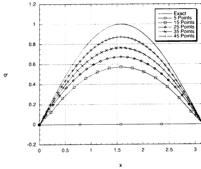
(a) fourth-order filter
