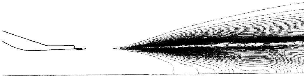
(b) detail of nozzle exit
