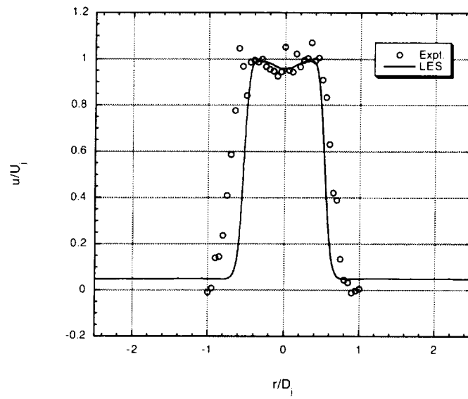
(a) x/D_j = 2
