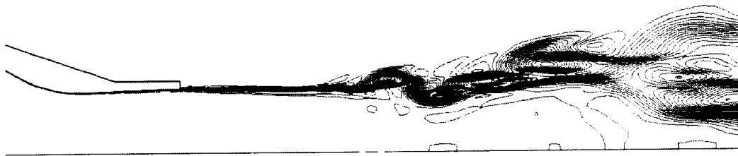
(a) Gottlieb-Turkel
