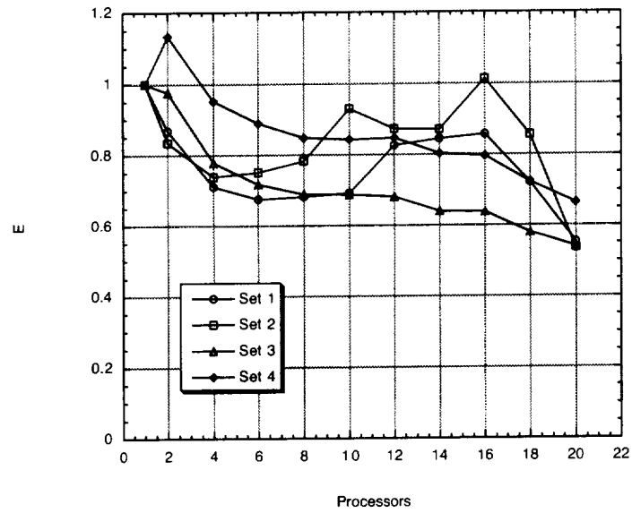
Figure 6.5: Parallel processing efficiency
