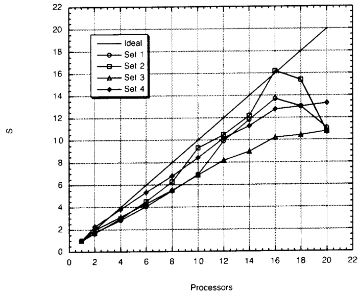
Figure 6.4: Parallel processing speedup
