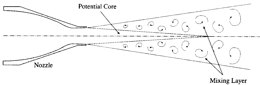
Figure 1.1: Jet schematic
