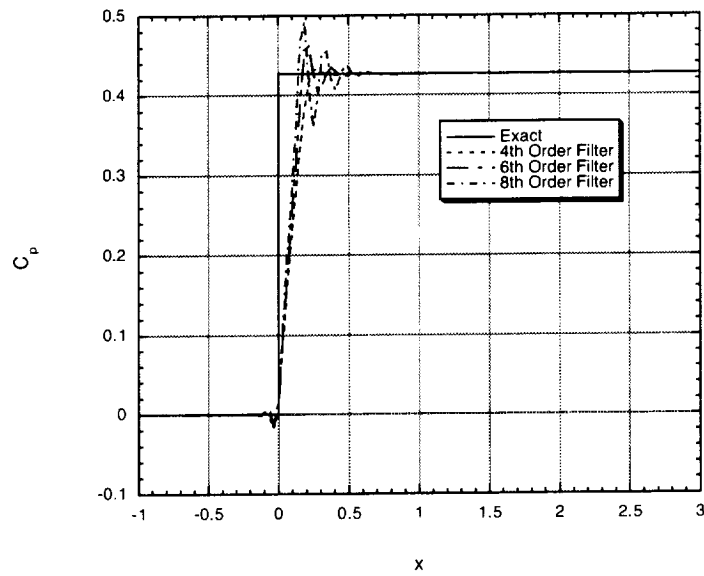
(b) Comparison of filters with Runge-Kutta scheme
