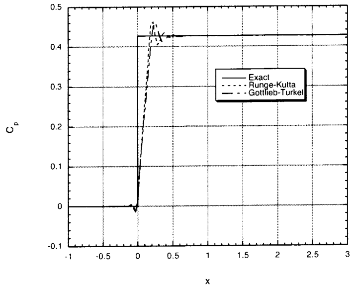
(a) Comparison of numerical schemes with 6th order filter
