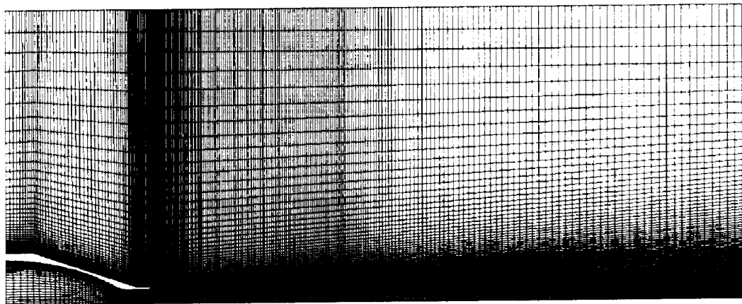
Figure 7.2: Axisymmetric computational grid
