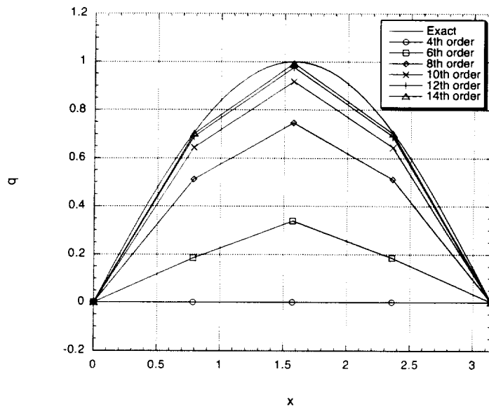
Figure 3.5: Effect of filter order on a five point wave
