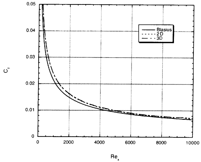
(a) skin friction coefficient
