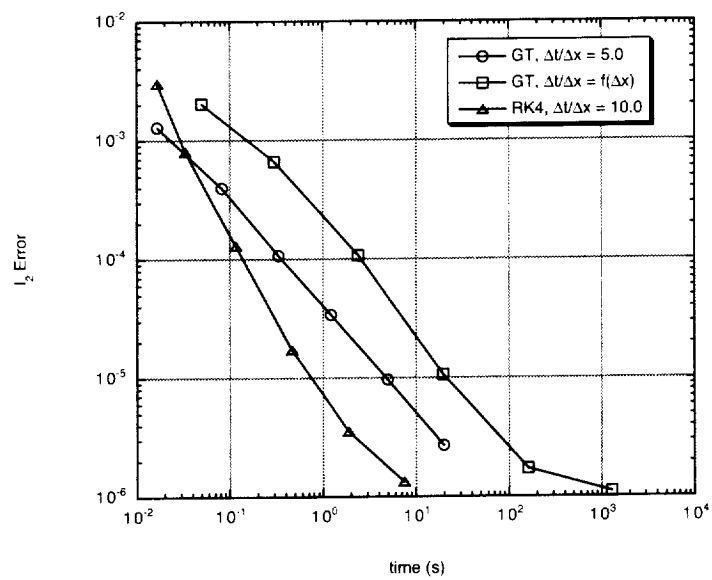
Figure 4.10: Efficiency of the numerical schemes for the linear convection problem
