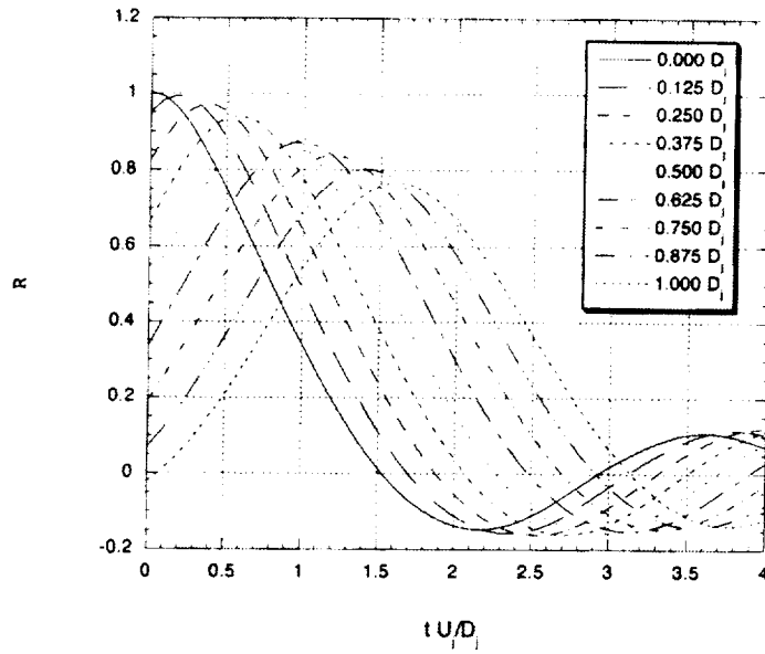
(a) 0 degrees
