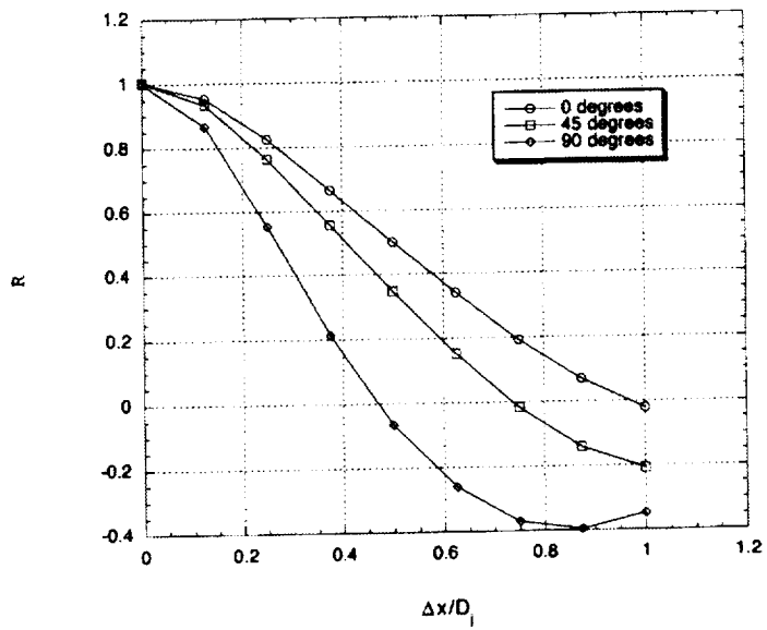
Figure 7.42: Two point space correlation coefficient
