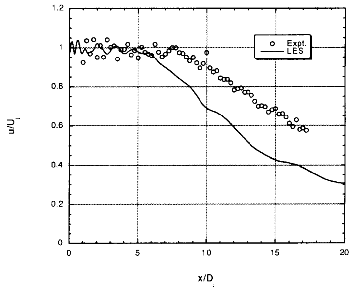
Figure 7.29: Time averaged centerline velocity profile for the 3D LES solution
