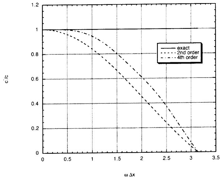
Figure 3.1: Error in wave speed
