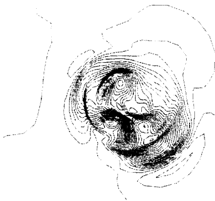
(b) \frac{tD_j}{U_j} = 16.149
