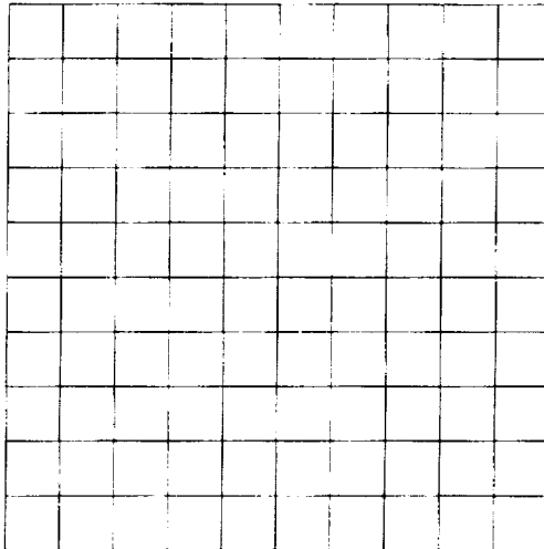
(a) computational grid
