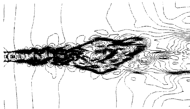
(b) \frac{tD_j}{U_j} = 16.149
