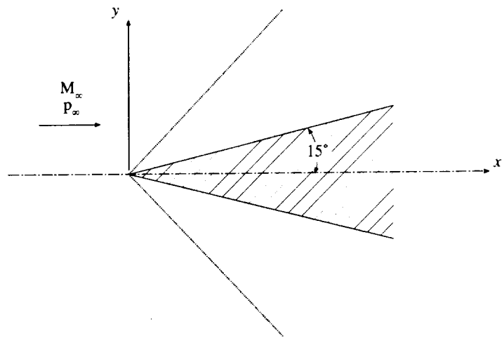
Figure 6.12: Mach 2 flow over a 15 degree wedge
