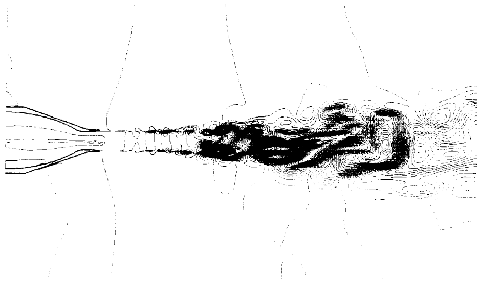
(a) instantaneous
