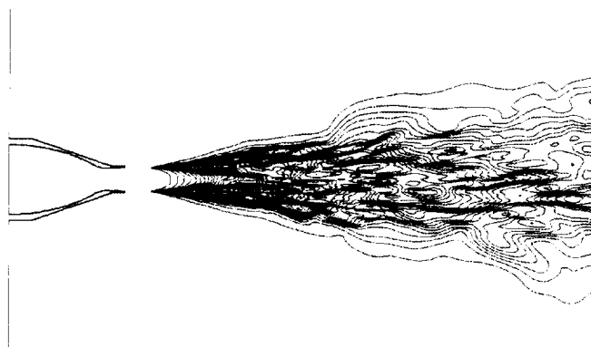
(c) azimuthal turbulent intensity
