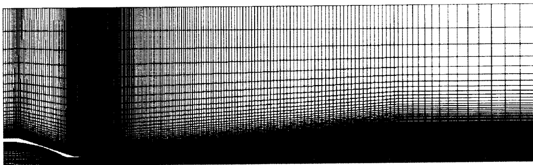
Figure 7.7: Axisymmetric computational grid with exit zone
