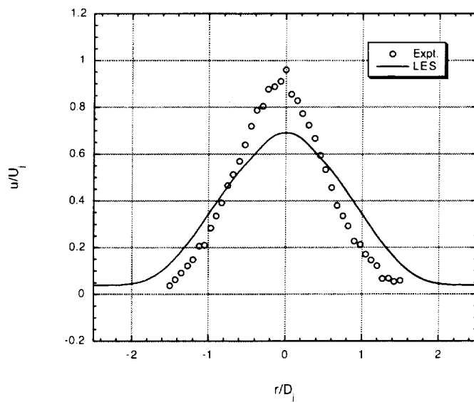
(e) x/D_j = 10
