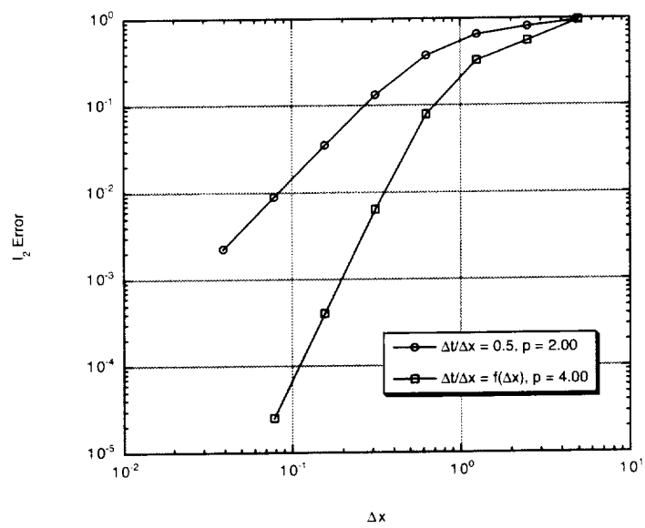
Figure 4.3: Improved spatial error of Gottlieb-Turkel scheme for the linear problem
