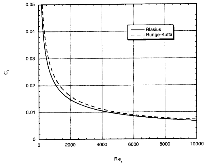
(b) Runge-Kutta scheme
