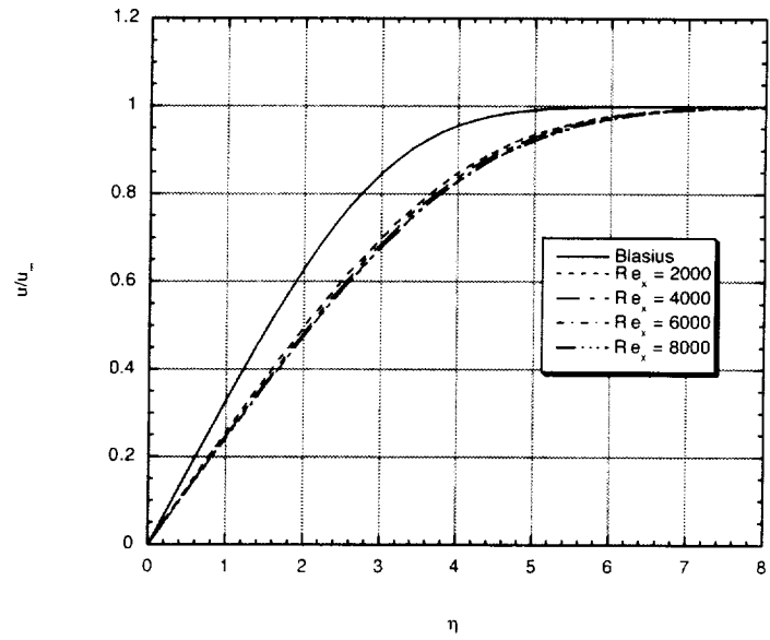
(a) Gottlieb-Turkel scheme
