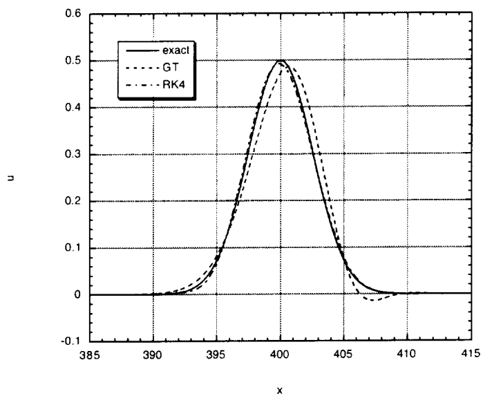
Figure 4.1: Solution to linear convection problem
