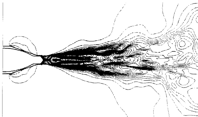
(b) radial turbulent intensity
