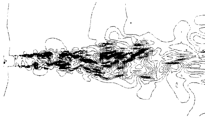
(b) \frac{tD_j}{U_j} = 16.149
