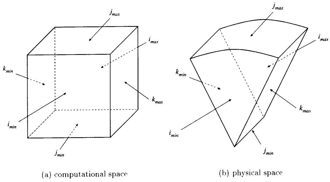
Figure 6.2: Pole boundary condition
