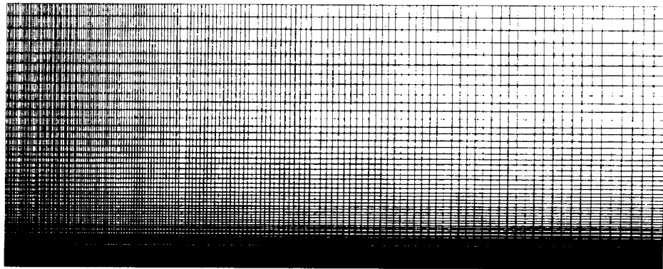
Figure 6.7: 2D grid for laminar flat plate calculations
