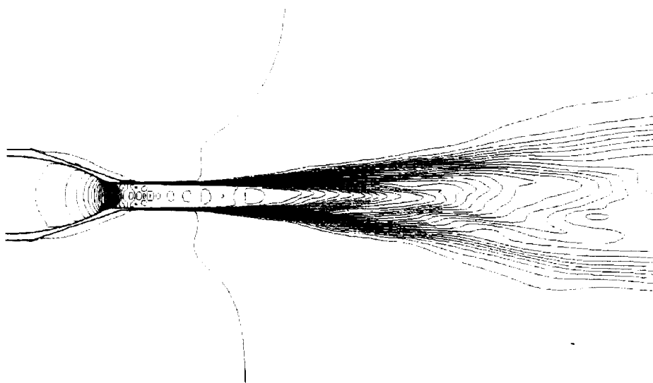
(b) time averaged
