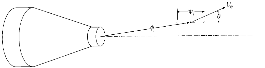
Figure 7.1: Two point correlation schematic
