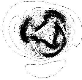
(a) \frac{tD_j}{U_j} = 0.0000
