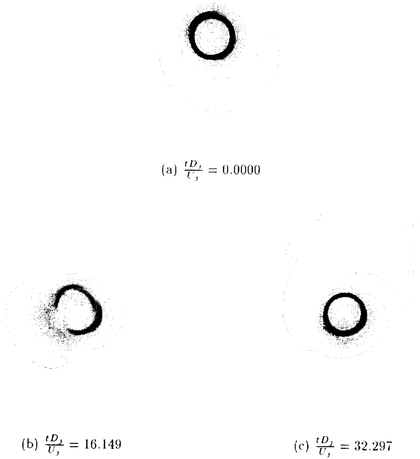
Figure 7.35: Instantaneous total velocity contours at x/D_j = 3 for the 3D LES solution
