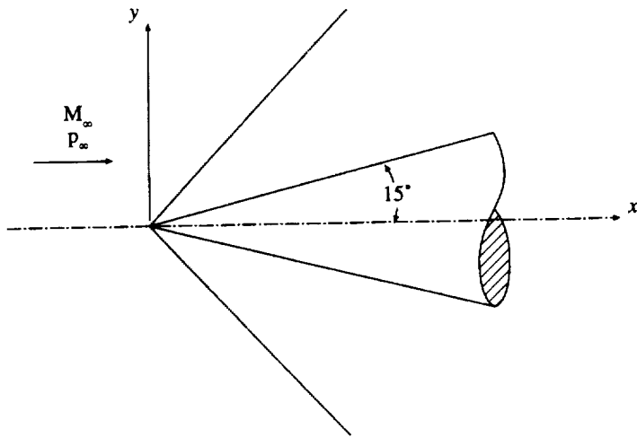
Figure 6.16: Mach 2 flow over a 15 degree cone
