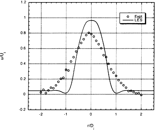
(f) x/D_j = 12
