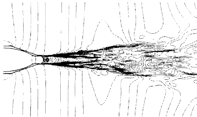
(a) axial turbulent intensity
