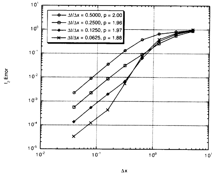
(a) Spatial error
