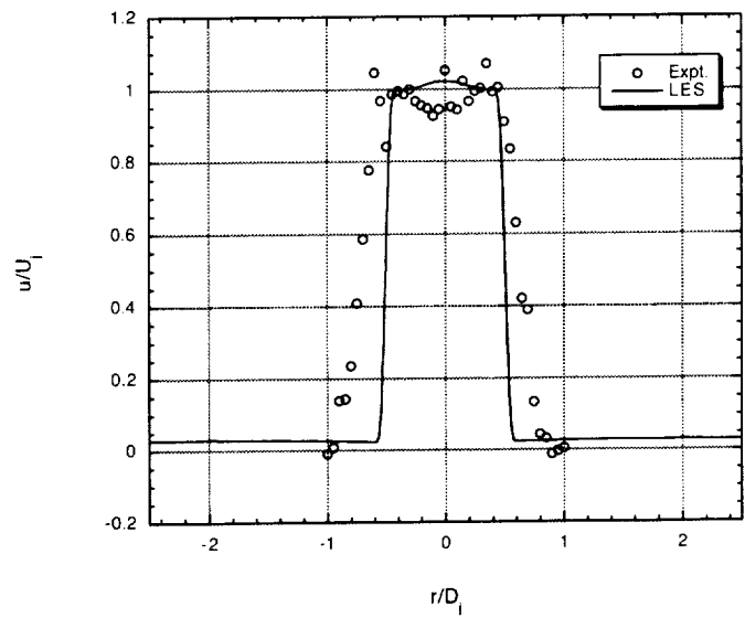
(b) x/D_j = 4
