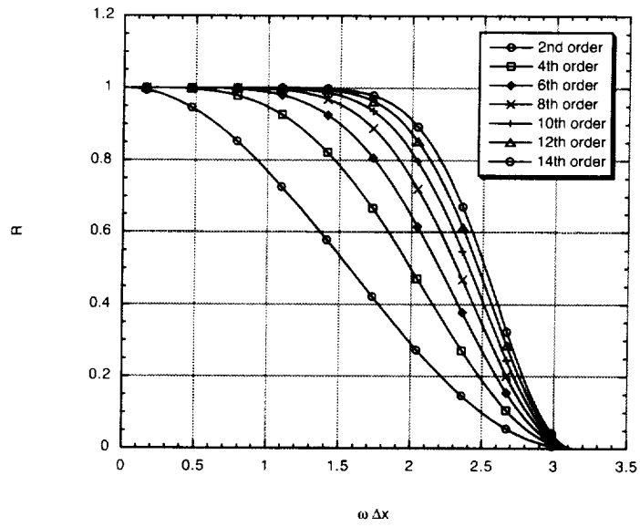
Figure 3.3: Filter response
