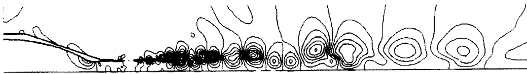
(a) instantaneous
