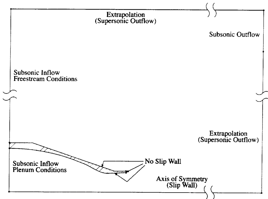
Figure 7.3: Boundary conditions for axisymmetric calculations
