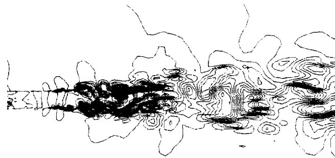
(b) \frac{tD_j}{U_j} = 16.149
