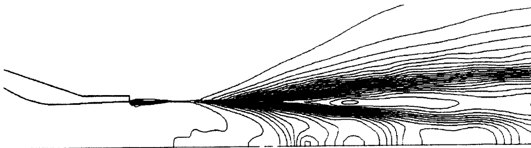
(b) detail of nozzle exit
