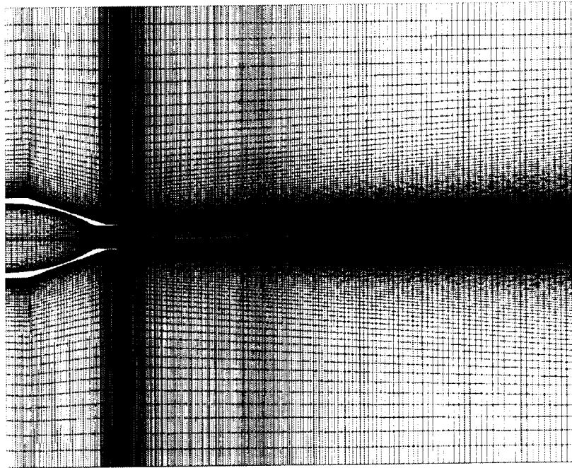
(a) streamwise, x-y plane
