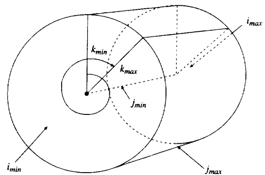
(c) physical space with overlap
