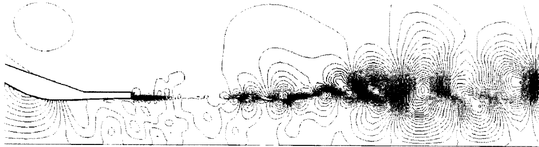
(a) instantaneous radial velocity
