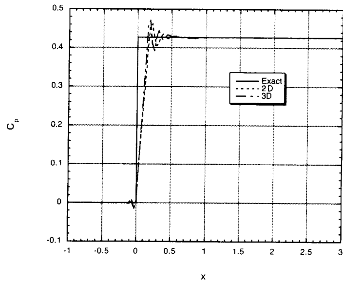
(b) Runge-Kutta scheme
