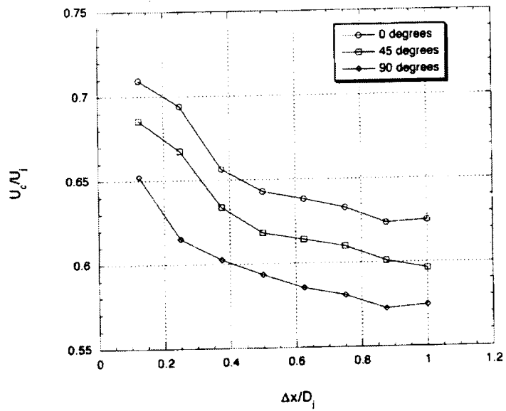
Figure 7.44: Convection velocity
