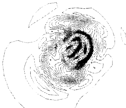
(c) \frac{tD_j}{U_j} = 32.2970
