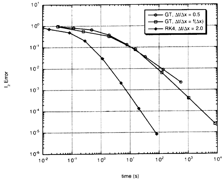
Figure 4.5: Efficiency of the numerical schemes for the linear convection problem
