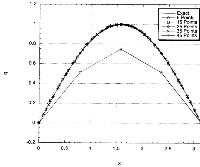
(c) eight-order filter
