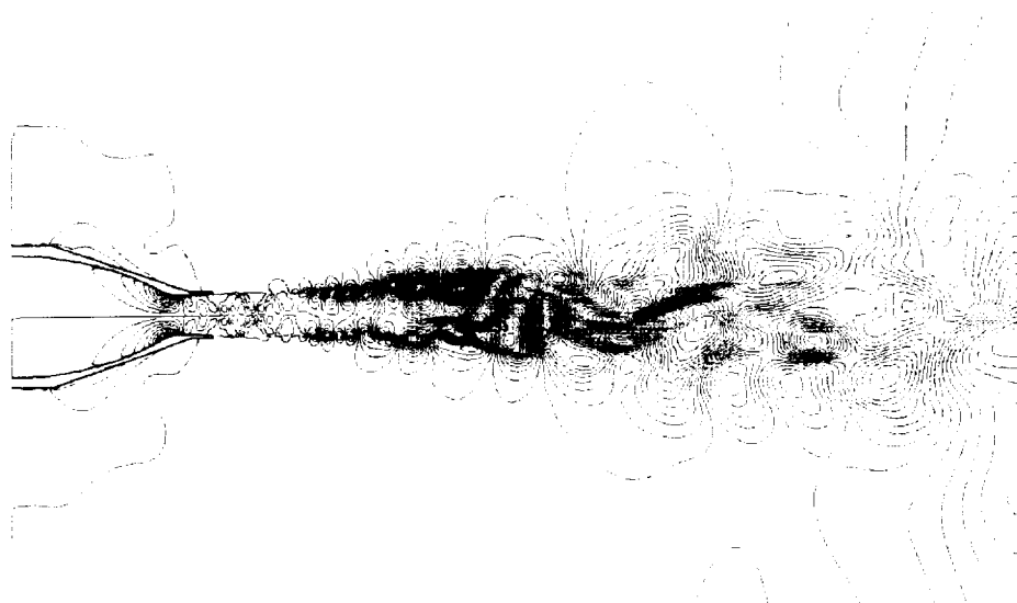
(a) instantaneous
