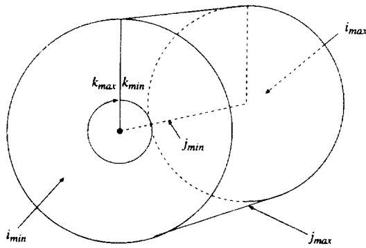
(b) physical space without overlap
