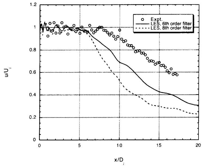
Figure 7.31: Comparison of sixth- and eighth- order filters on 3D LES solution
