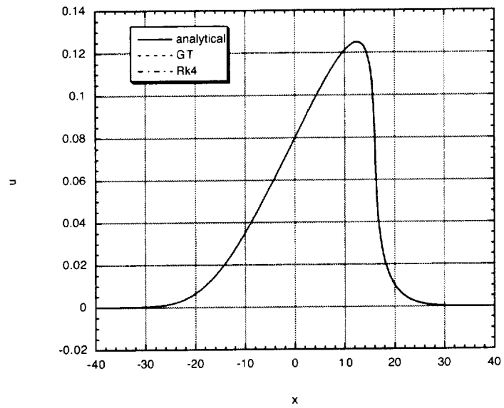
Figure 4.6: Solution to smooth nonlinear convection problem
