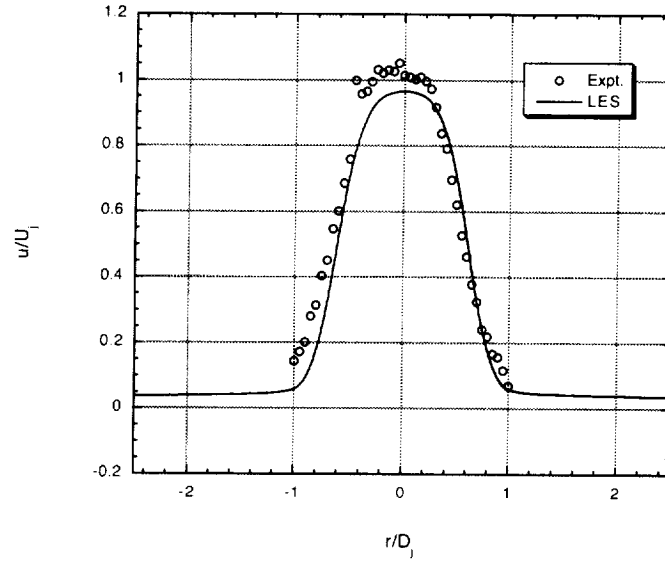
(c) x/D_j = 6
