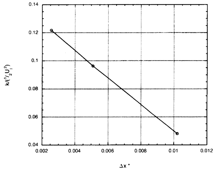
(b) Turbulent kinetic energy
