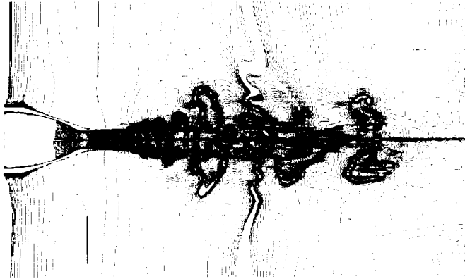
Figure 7.28: Dilatation contours for 3D LES solution
