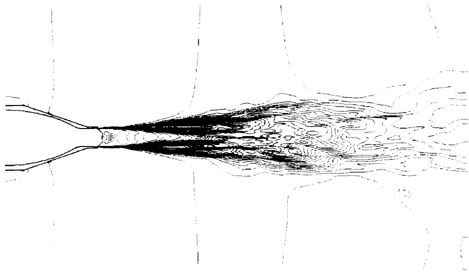
Figure 7.39: Turbulent kinetic energy contours for the 3D LES solution
