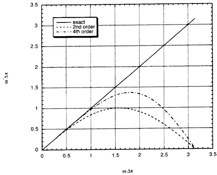
Figure 3.2: Error in wave number
