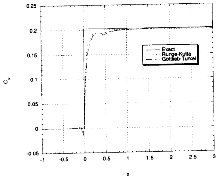
Figure 6.17: Pressure distribution on cone surface
