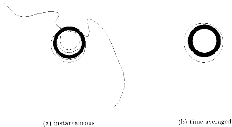
Figure 7.24: Total velocity contours at x/D_j = 3 for 3D LES solution
