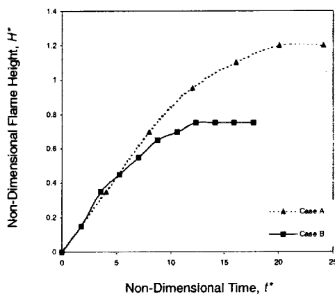
Figure 8. Methane-air results for the effect of ring circulation on ring trajectory H^*(t^*) with similar fuel volumes. Ring circulations are 482 and 212 cm 2 /s for Case A and B, respectively.
