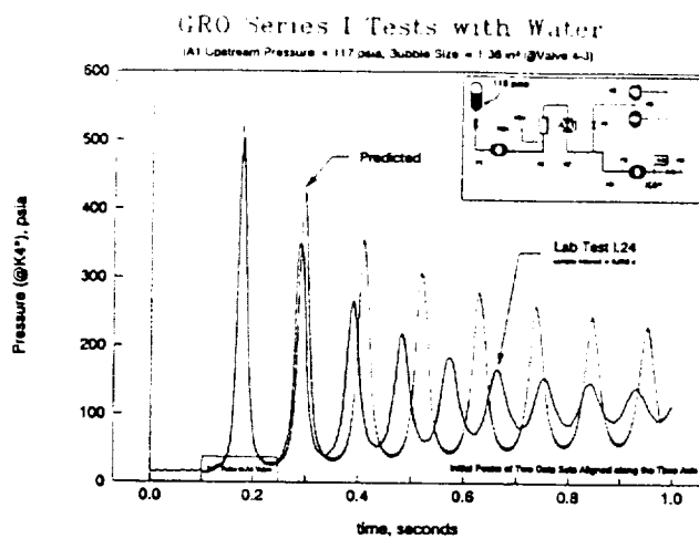
Figure 6. Water/1.36 in 3 Bubble/117 psia Tank
