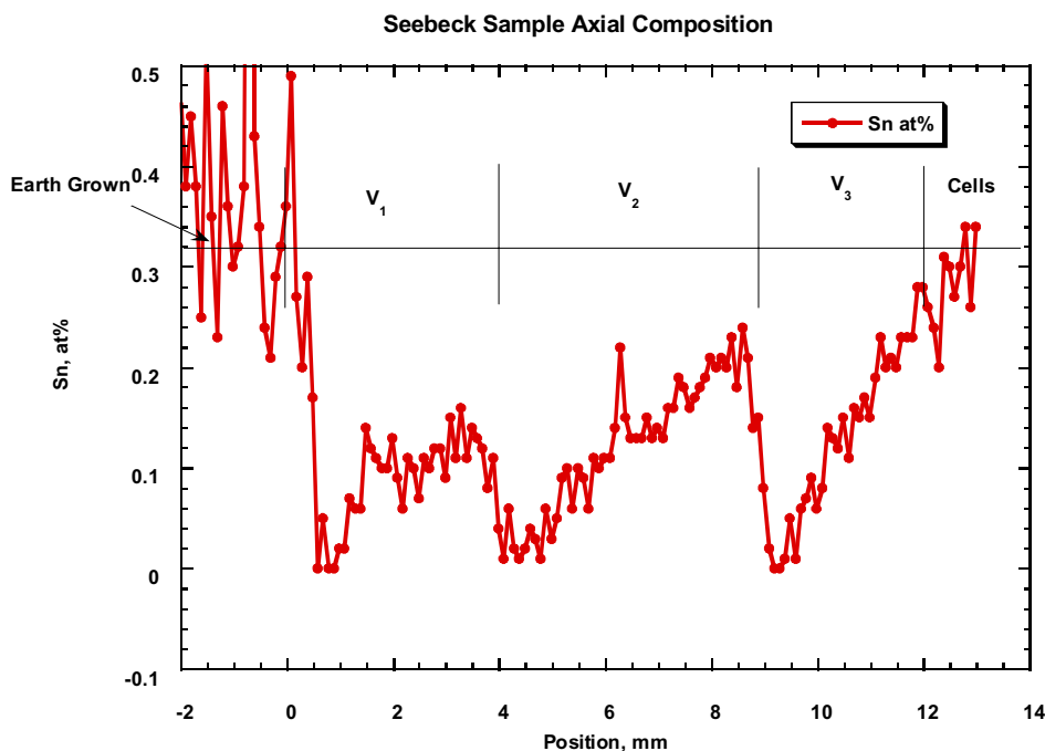
Figure 21. The microprobe compositional line scan for the Seebeck sample during events 11A, 11B, 12, which includes three velocities V1, V2, V3.
