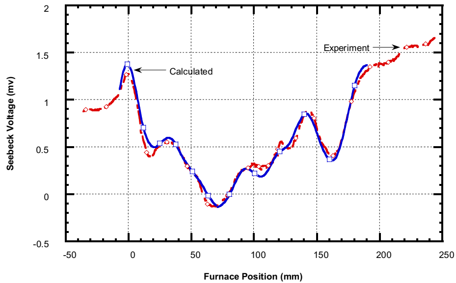
Figure 35. Calculated structural Seebeck voltage compared with experimental data for hot zone at 85°C.
