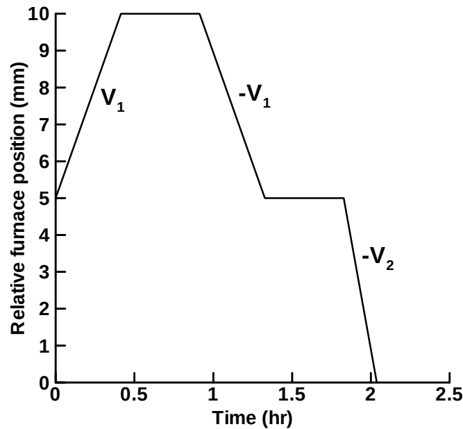
Figure 42. Furnace position as a function of time. V_1 is the furnace velocity during solidification. -V_1 and -V_2 denote melt stages.
