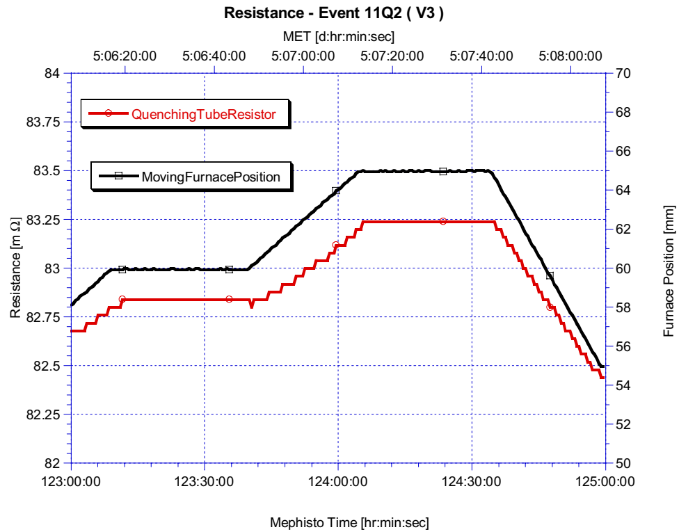
Figure 18. Resistance and furnace position change as a function of processing time during event 11Q2 in MEPHISTO experiment.
