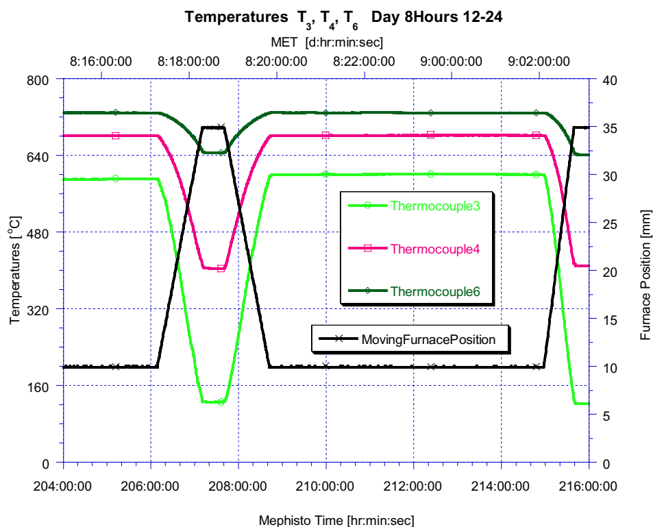
Figure 16. Thermal measurement by three thermocouples placed in the Peltier and Quenching samples.
