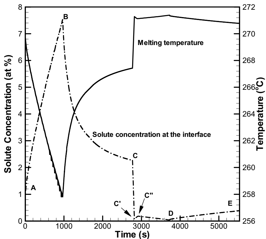
Figure 50. Interface solute concentration and melting temperature at the mid-height of the ampoule.
