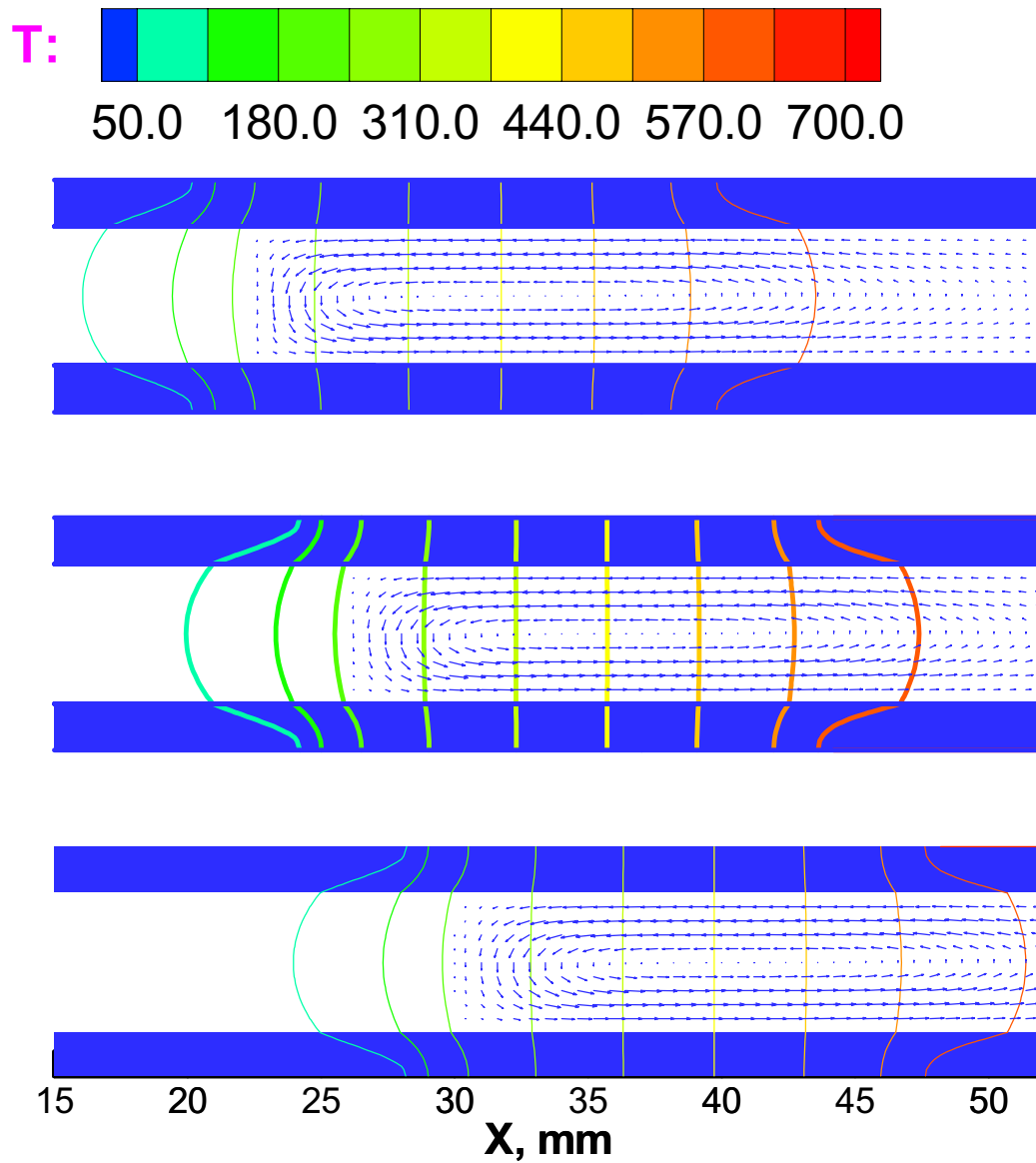
Figure 46(c). Temperature contours and velocity vectors during Event 11E, hold, and Event 11F.
