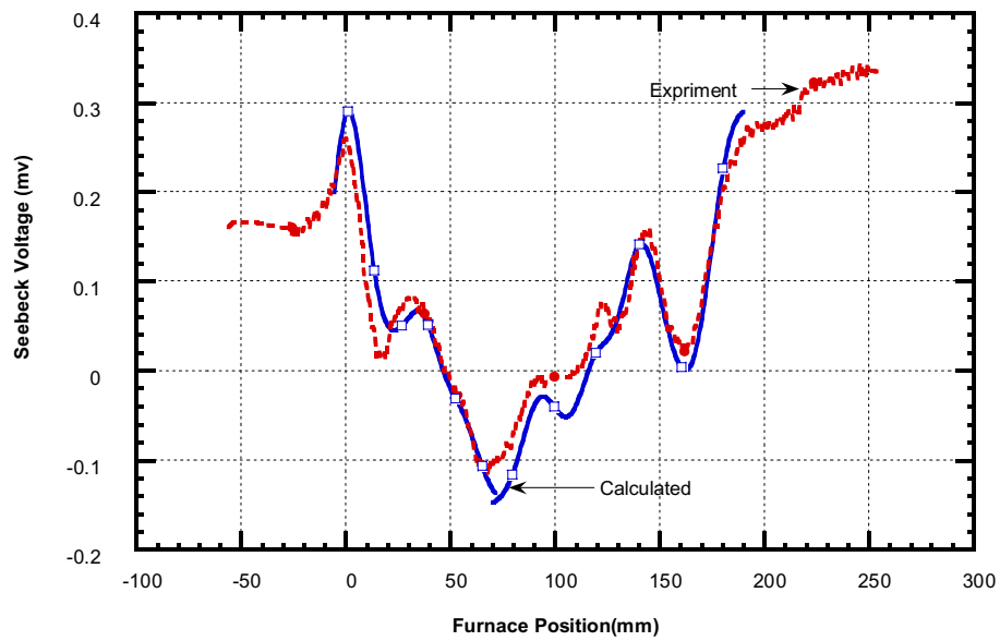
Figure 32. Calculated structural Seebeck voltage compared with experimental data for hot zone at 40°C.
