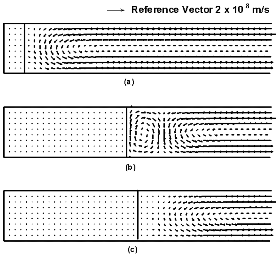
Figure 51. Velocity vectors. (a) early in the solidification; (b) at the end of the solidification; (c) during the first rehomogenization for Event 9w.
