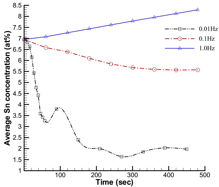
Figure 45. Average concentration at the interface for the disturbances with an amplitude of 10^{-2}g and frequencies of 10^{-2} , 10^{-1} and 1 Hz.
