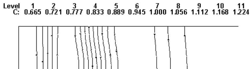
Figure 44. Contours of concentration in the ampoule at the same time as for Figure 43e, showing evidence of transverse (radial) segregation.
