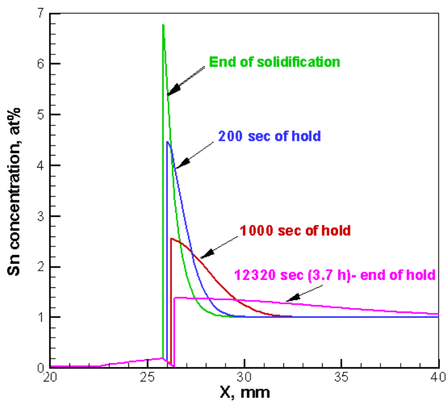
Figure 46(e). Solute decay during extended hold between Event 11E and 11F.
