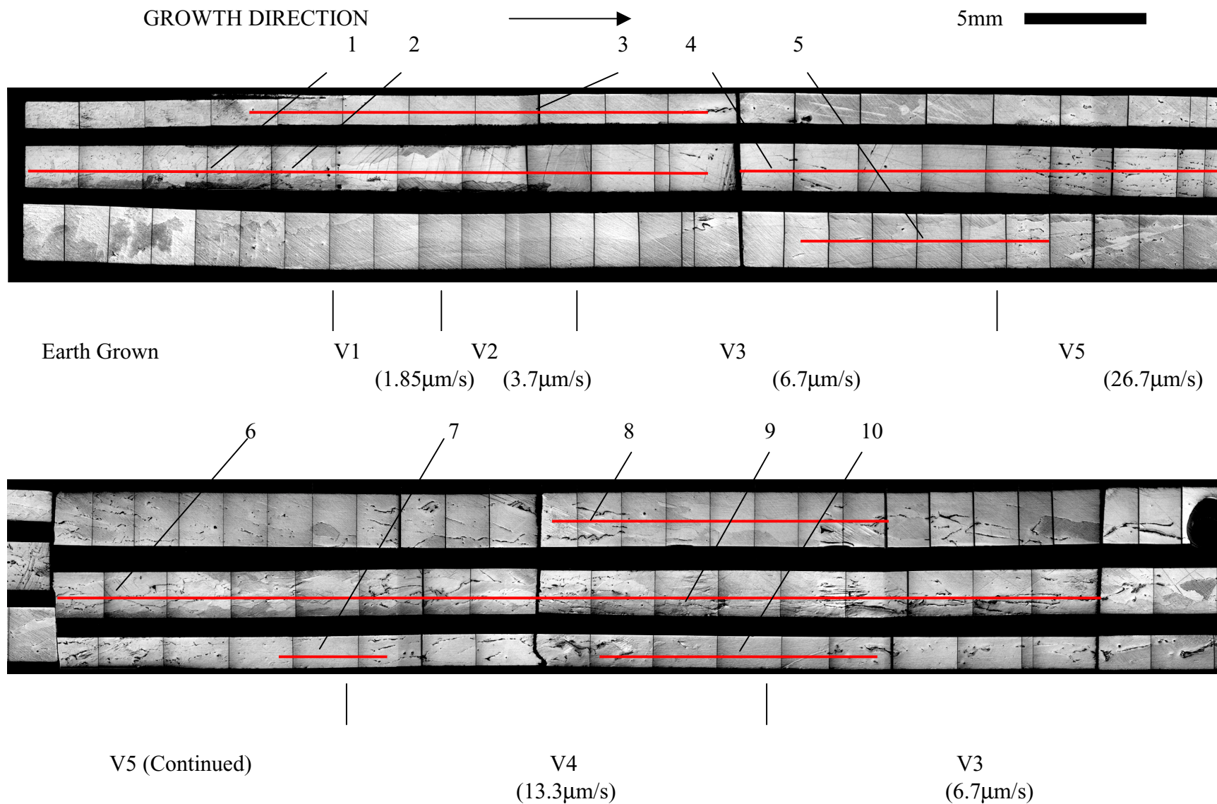
Figure 22(a). Schematic of microprobe analysis position on the Seebeck sample, line numbers included.
