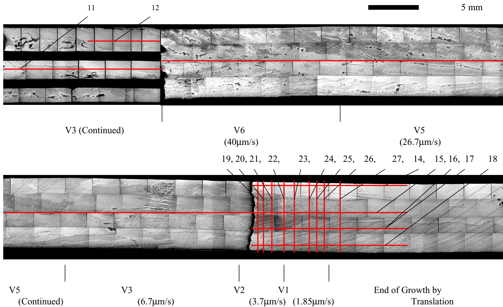
Figure 22(b). Schematic of microprobe analysis position on the Seebeck sample, line numbers included.
