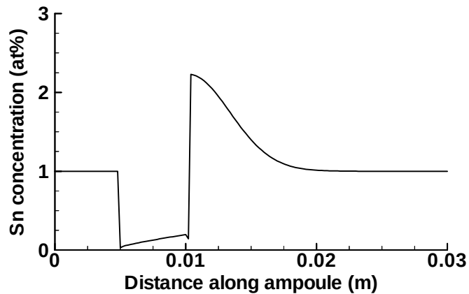
Figure 43(c). Solute concentration along the mid-height of the ampoule following the first 30 min hold.
