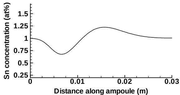
Figure 43(f). Solute concentration along the mid-height of the ampoule after a further 5 mm of solid has been melted at V_2 = -6.6 \mu\text{m s}^{-1} .
