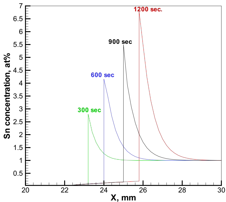
Figure 46(d). Solute build-up during Event 11F solidification.
