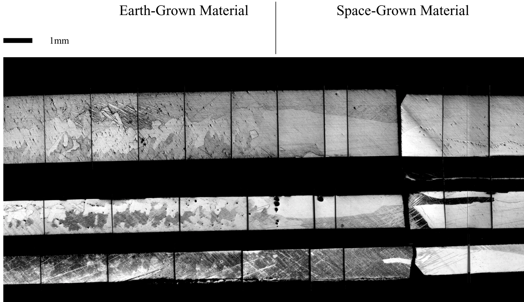
Figure 11(b). Composite image of the initial growth of the Peltier sample showing a similar structure to the quench sample. The break in the micrograph is where the sample was cross sectioned.
