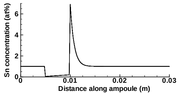
Figure 43(b). Solute concentration along the mid-height of the ampoule after solidification of 5 mm of liquid at V_1 = 3.34 \mu\text{m s}^{-1} .
