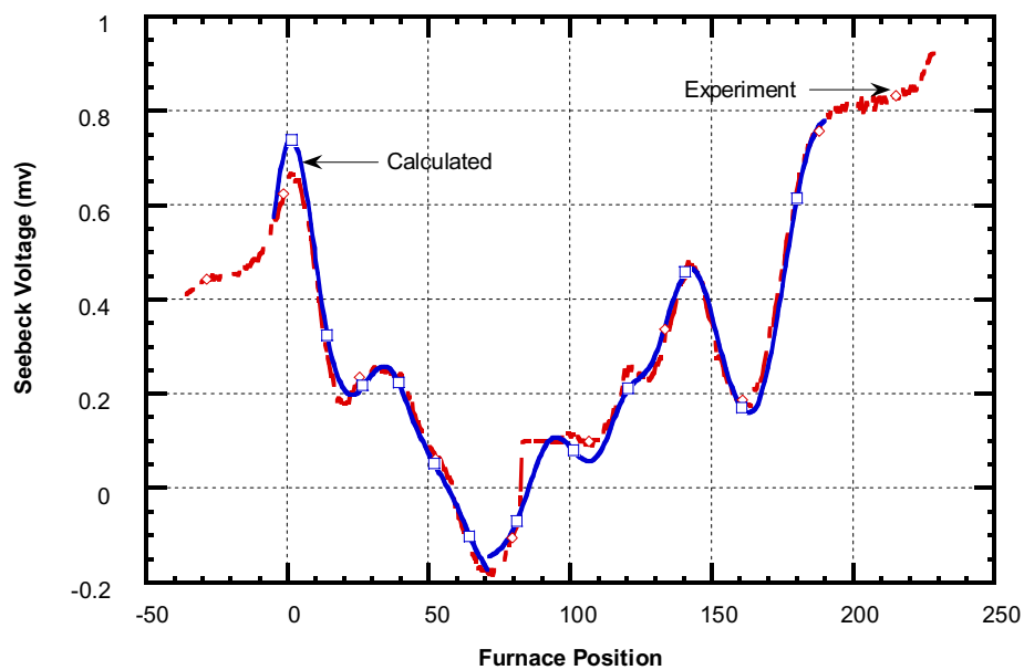
Figure 34. Calculated structural Seebeck voltage compared with experimental data for hot zone at 60°C.
