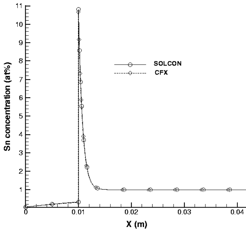
Figure 38. Distribution of solute concentration at the mid-height of the ampoule after 3000 sec of solidification.
