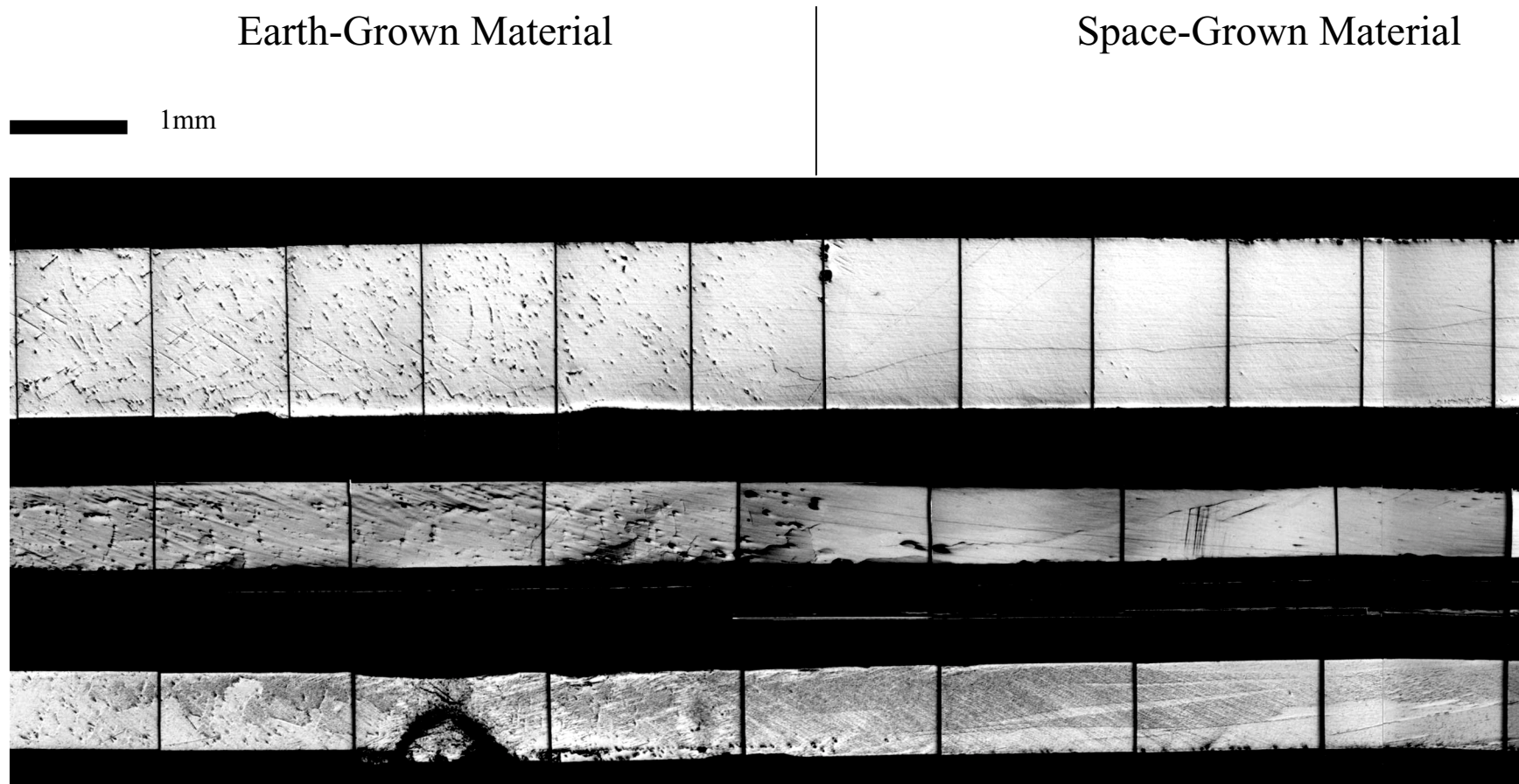
Figure 11(a). Composite image of the initial growth of the quench sample. The initial Earth-grown structure on the left hand side shows a faceted cellular dendritic morphology. The transition to plane-front growth is visible in the space-grown material on the right hand side.
