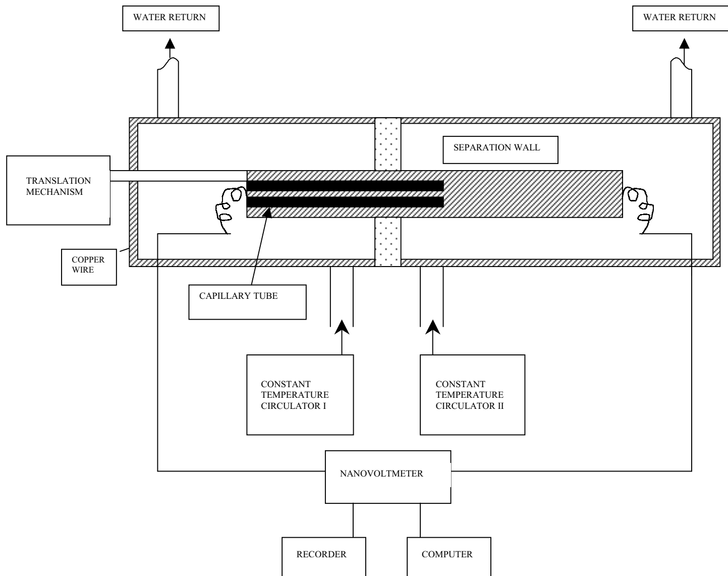
Figure 28. Schematic of Structural Seebeck Measurements.
