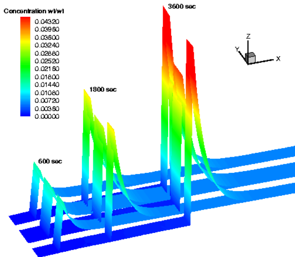
Figure 46(f). Solute build-up inside and outside the capillary.
