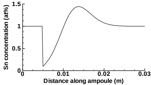
Figure 43(d). Solute concentration along the mid-height of the ampoule after 5 mm of solid has been melted at V_1 = -3.34 \mu\text{m s}^{-1} .
