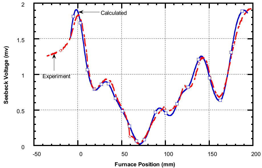
Figure 36. Calculated Structural Seebeck voltage compared with experimental data for hot zone at 95°C.
