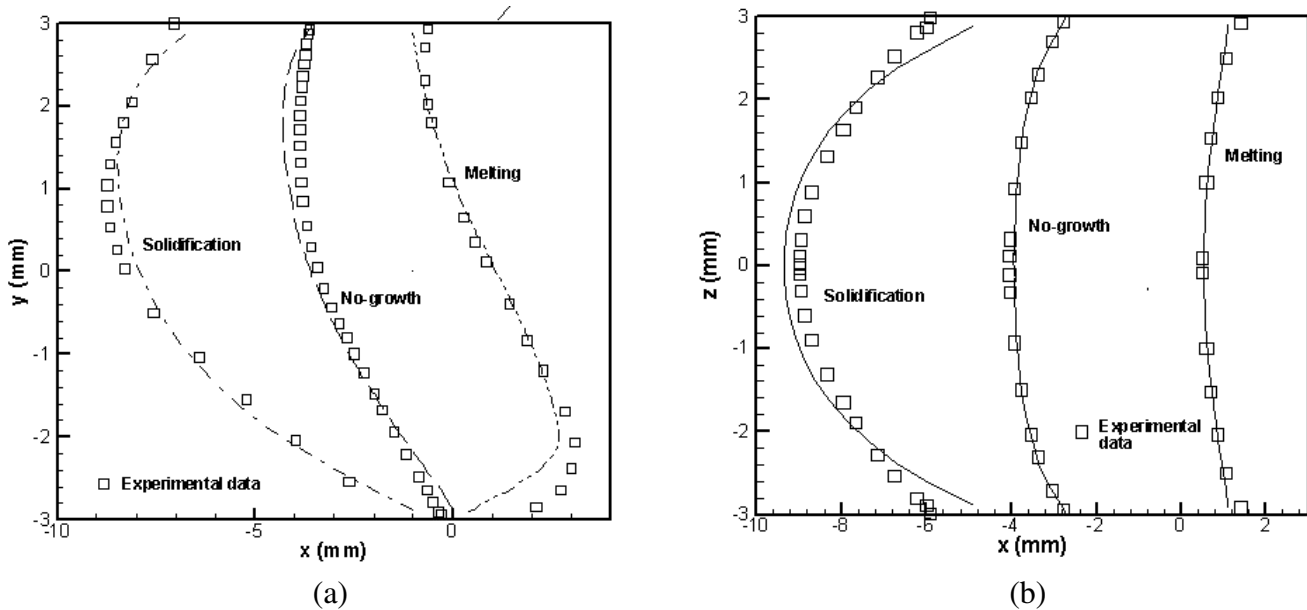
Figure 40. Experimental and computed interface profile at (a) the vertical mid-plane of the ampoule and (b) viewed from above.
