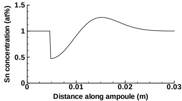
Figure 43(e). Solute concentration along the mid-height of the ampoule following the second 30 min hold.
