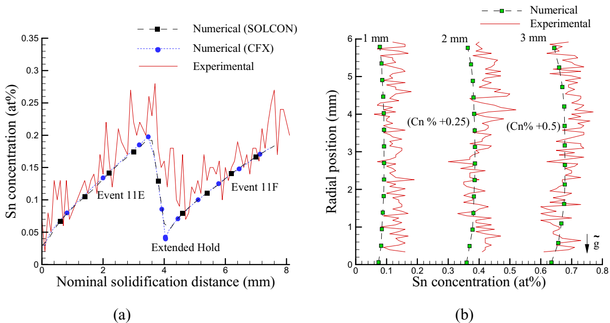
Figure 46. Solute concentration in the solid along the (a) ampoule centre line and (b) across the ampoule for Event 11E and 11F.
