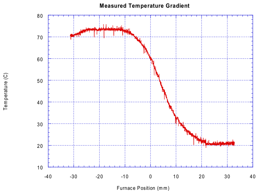
Figure 29. Temperature gradient in the sample for structural Seebeck determination, with the cold and hot ends at 20 and 75°C, respectively.
