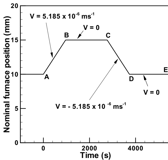
Figure 48. Timeline for the event 9W.
