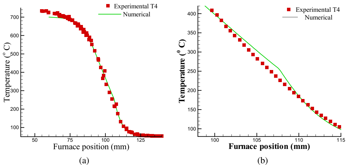
Figure 47. (a) Temperature distribution along the centre line and (b) in the vicinity of interface.
