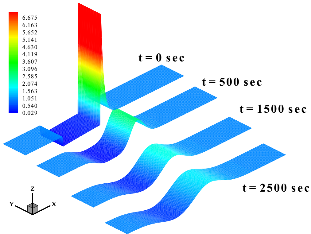
Figure 43(a). Solute concentration decay as a function of time.
