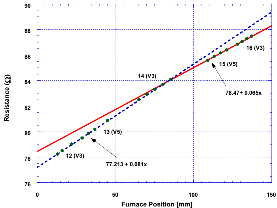
Figure 19. Resistance of Sample versus furnace Position. Crossing of lines is evidence of the end of capillary. Dashed line fits data in the capillary, solid line is fits of data outside.
