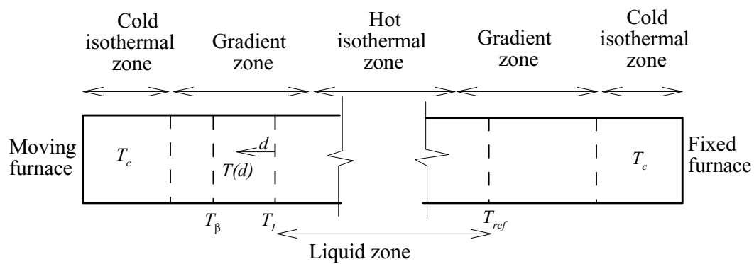
Figure 52. Thermal fields involved in Seebeck signals.
