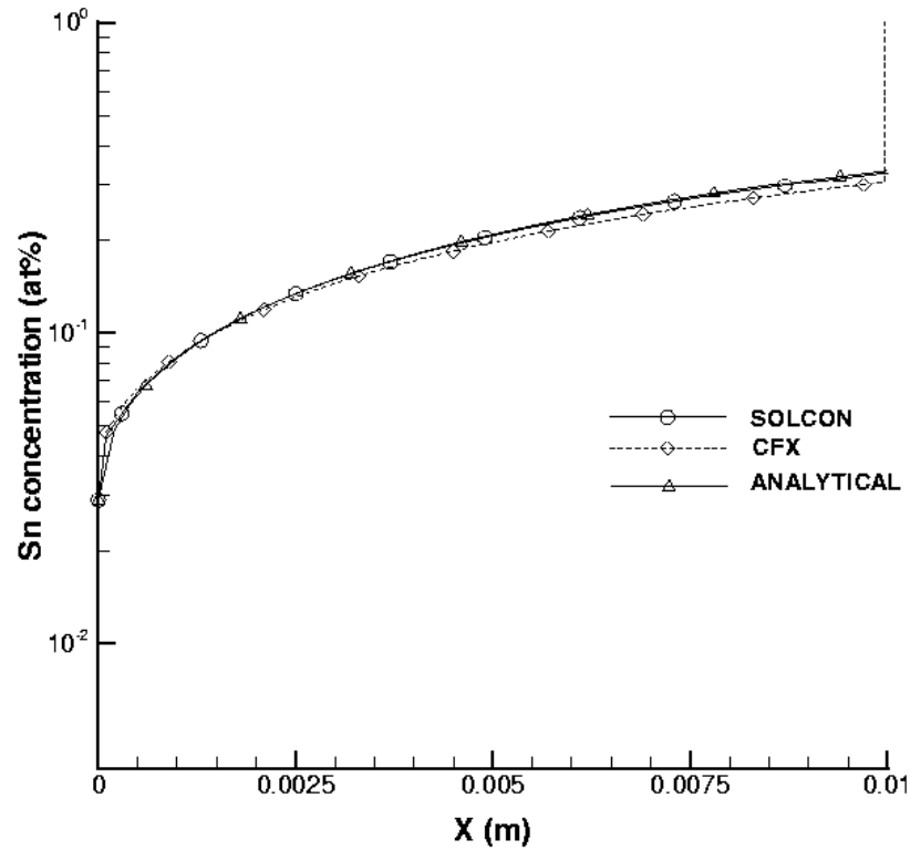
Figure 39. Detailed distribution of solute concentration in the solid part of the sample after 3000 sec of solidification.
