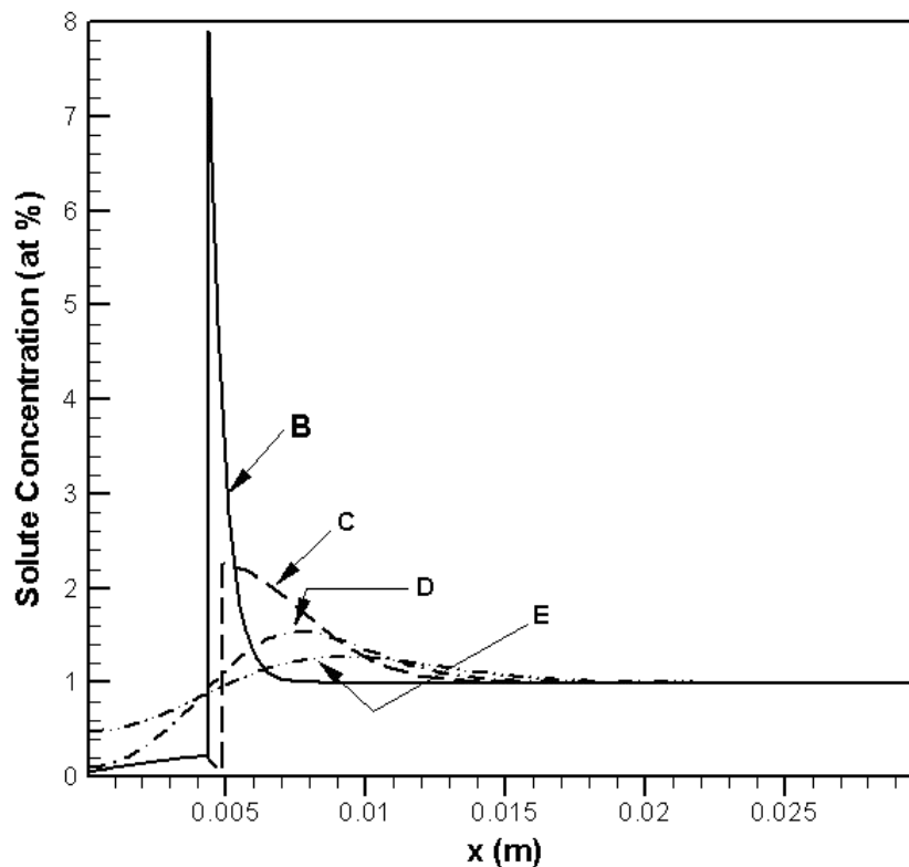
Figure 49. Solute concentration along the horizontal centreline of the ampoule at four different stages of the event.
