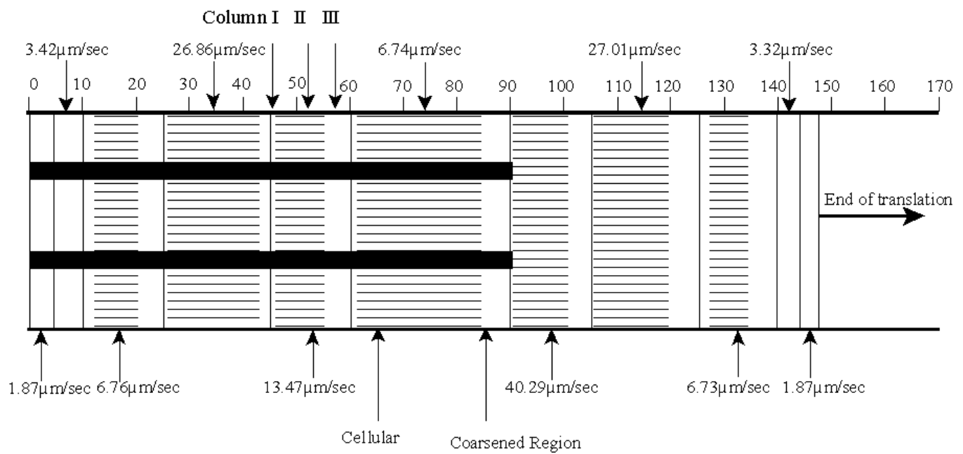
Figure 9. Summary of sample sections preserved during final solidification. Sections with horizontal lines indicate cellular breakdown.
