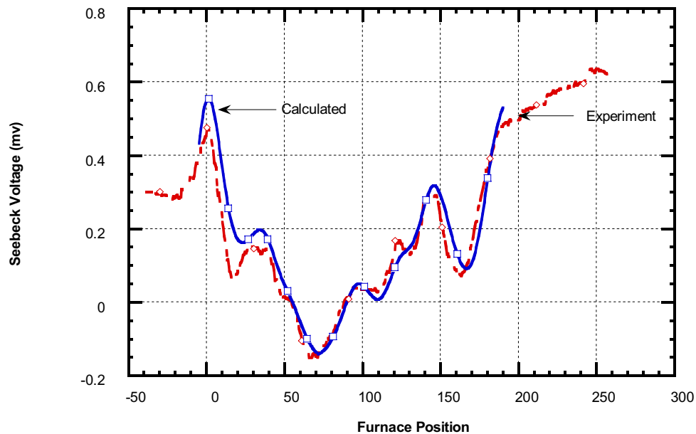
Figure 33. Calculated structural Seebeck voltage compared with the experimental data for hot zone under 50°C.
