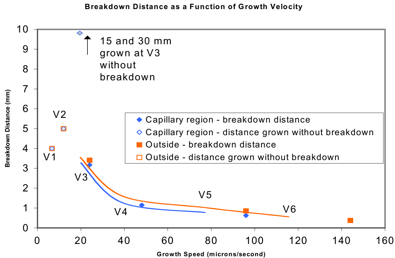
Figure 15. Breakdown distance as a function of growth velocity; solid symbols are the distances solidified to the planar to cellular transition, open symbols indicate planar front growth distances without the planar to cellular transition being reached.
