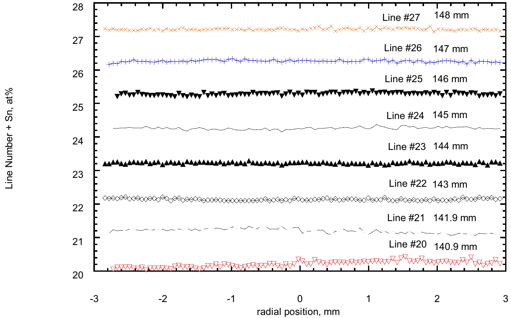
Figure 23. Radial composition profile in the Seebeck sample during solidification at velocity V1, V2.
