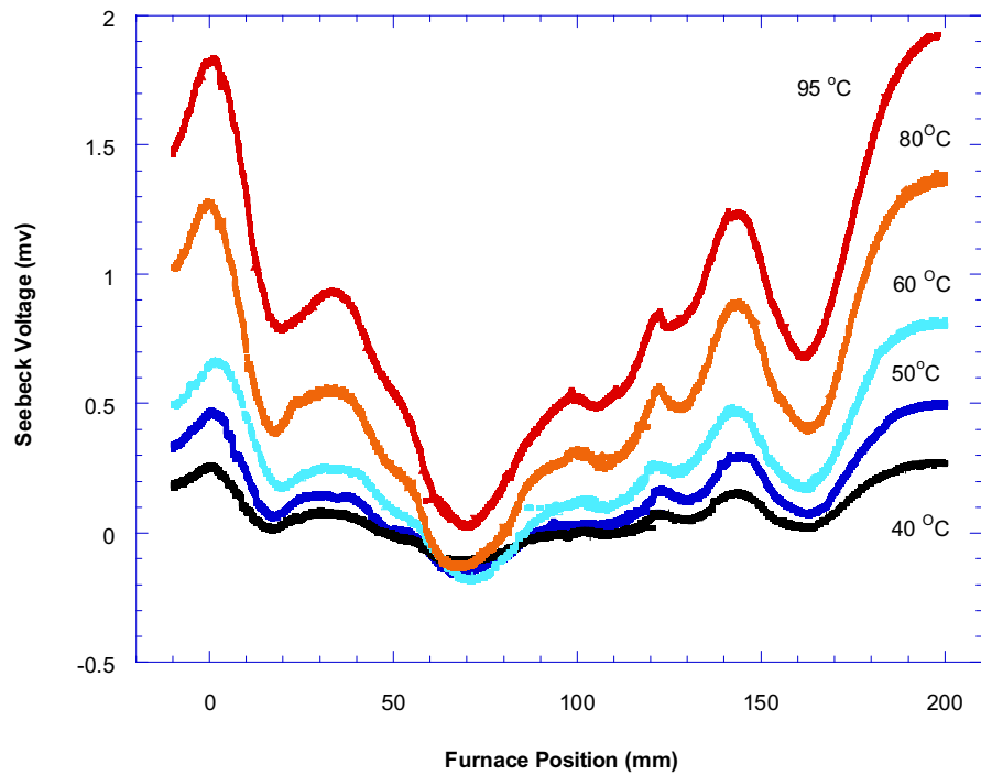
Figure 31. Structural Seebeck voltage under different temperatures, with the cold zone at 20°C and hot zone as indicated.
