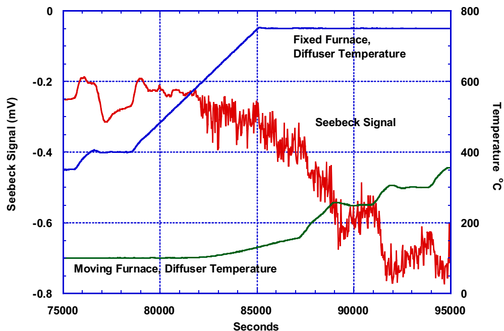
Figure 20. Diffuser temperatures for MEPHISTO furnaces and Seebeck signal during heat-up for ground-based experiments. Fluctuations in the Seebeck signal become apparent as the temperature of the liquid is increased from 400°C to 750°C.
