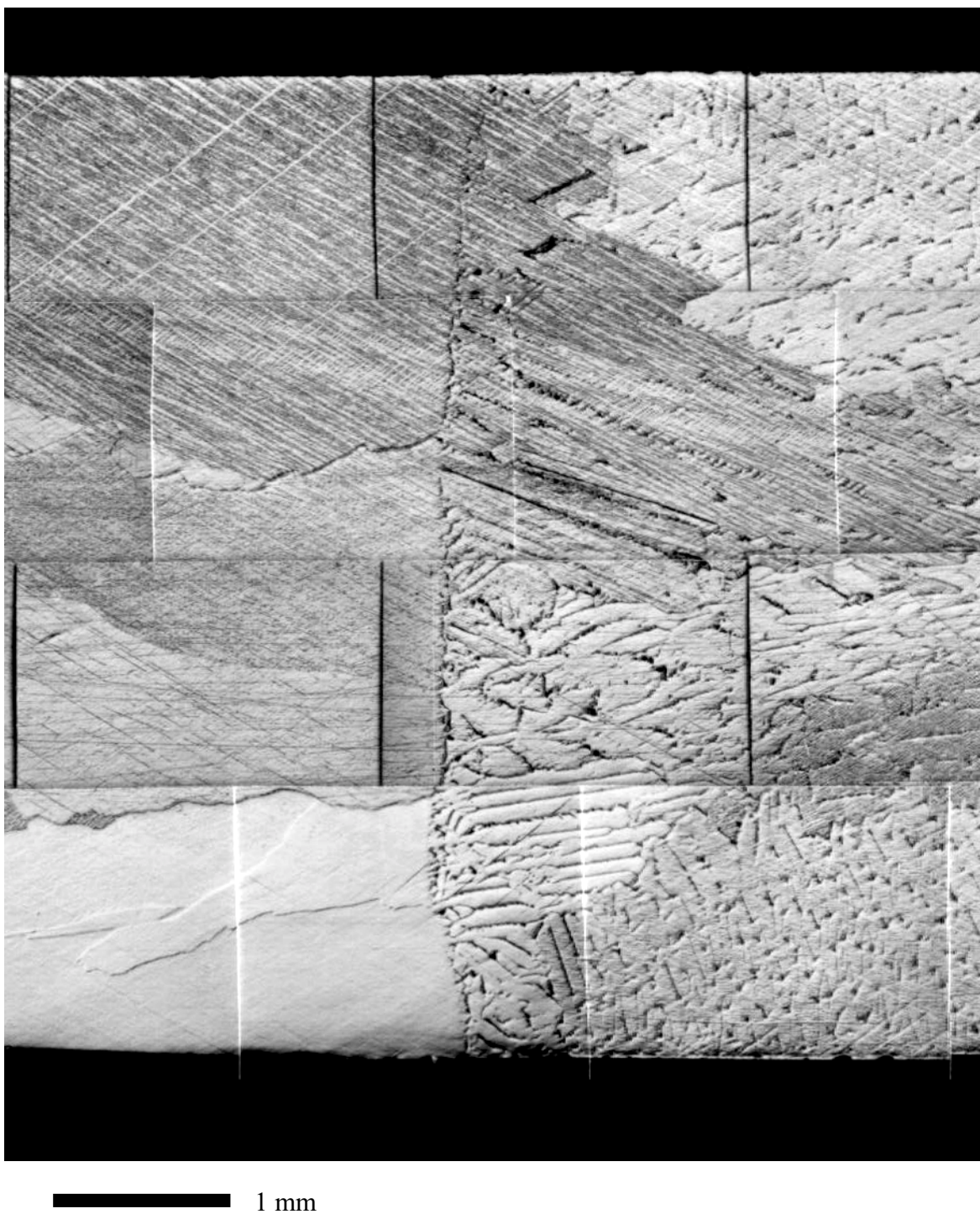
Figure 12. Composite micrograph of quenched section of the quench sample showing the S/L interface shape.
