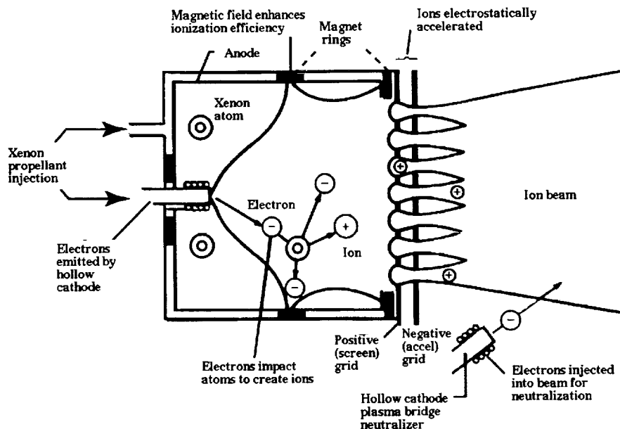
Fig. 3 Ion engine having a ring-cusp magnetic field discharge chamber.
