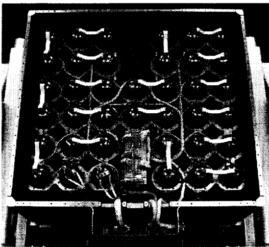
Figure 3. ISS Flight Model Battery Subassembly ORU with Cover Removed
