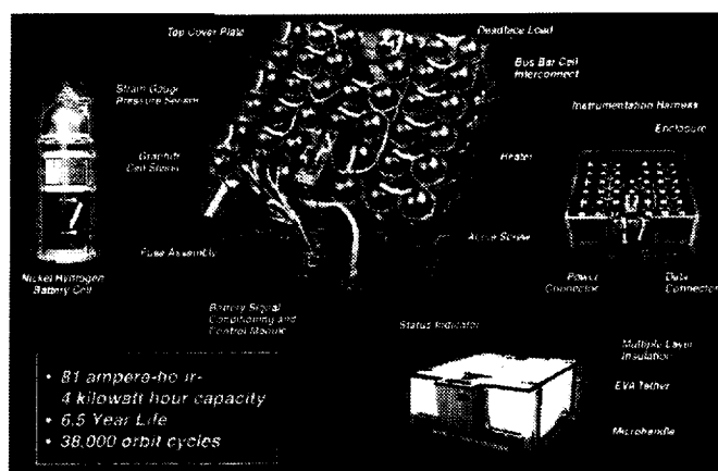
Figure 1. ISS Battery Subassembly ORU
