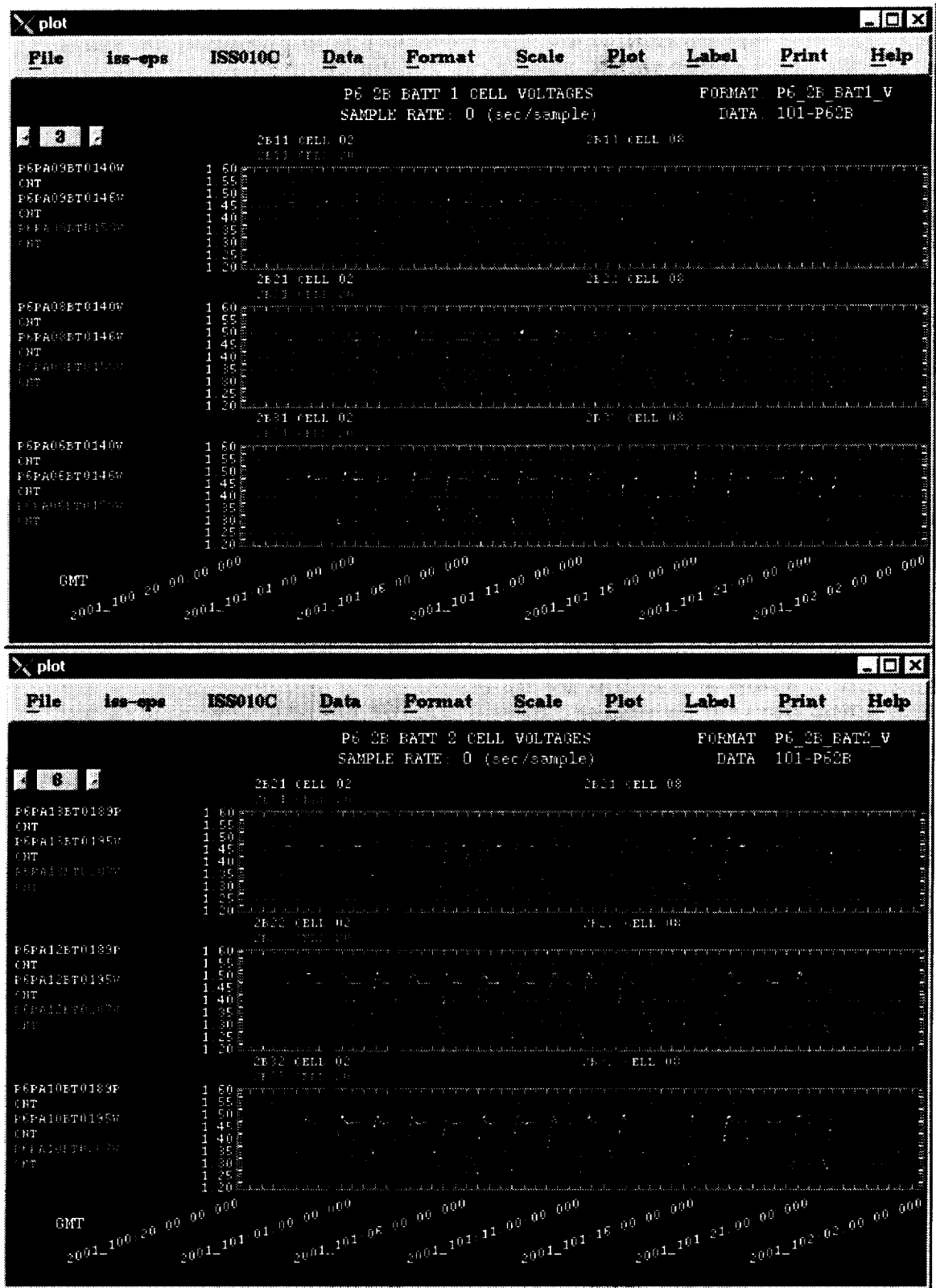
Figure 6: On-Orbit Data, Battery ORU Monitored Cell Voltages (4 cells per ORU 02, 08, 20, and 28)
