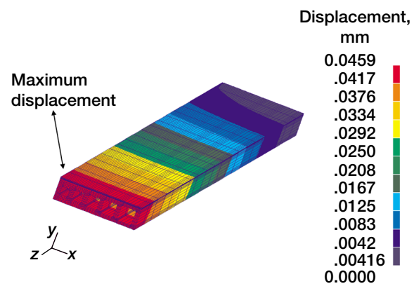
Figure 11.—Displacement profile with air cooling.
