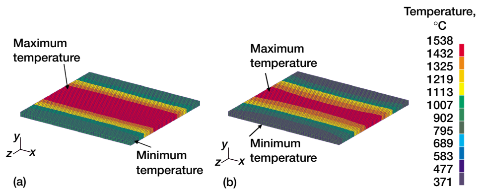
Figure 8.—Temperature distribution. (a) No air cooling. (b) Air cooling (see fig. 3 for hole sizes and shapes).
