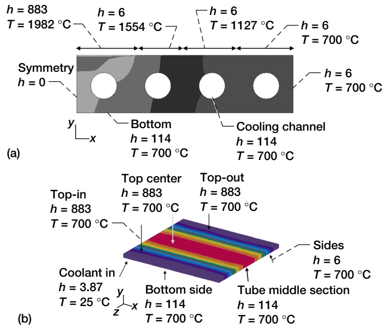
Figure 4.—Thermal boundary conditions showing applied gas temperature and heat transfer coefficient, h which is given in watts per square meters degree Celsius ( \text{W}/\text{m}^2\text{-}^{\circ}\text{C} ). (a) Two-dimensional model. (b) Three-dimensional model.
