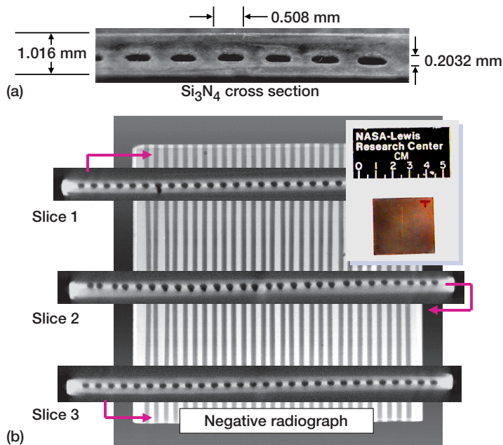
Figure 2.—Cross sections of a cooled silicon nitride panel. (a) Optical photograph of the cross section of a silicon nitride plate with cooling holes. (b) Computed tomographic image and cross-sectional view at three different locations showing inhomogeneity in cooling hole shape and spacing as well as cracks in the walls of the cooling holes.
