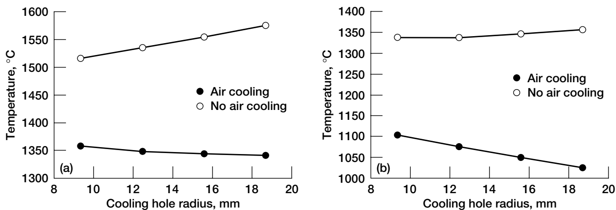
Figure 7.—Temperature variation as a function of hole size. (a) Hot spot temperature. (b) Cold spot temperature.
