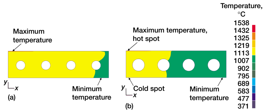
Figure 5.—Influence of cooling hole diameter on predicted ANSYS temperature distribution for \text{Si}_3\text{N}_4 plate internally cooled with air. (a) Hole radius, R , 1.143 mm. (b) Hole radius, R , 1.524 mm.
