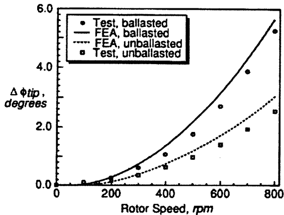
Figure 80. - Change in blade elastic twist at tip as a function of rotor speed.
