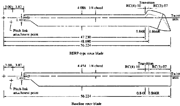
Figure 41. - BERP-type and baseline rotor blade geometries. Linear dimensions are in inches.
