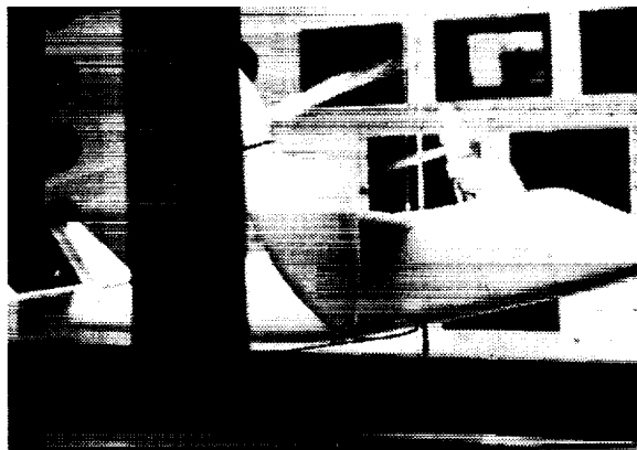
Figure 139. - 1/5-scale model in simulated helicopter autorotational configuration.
