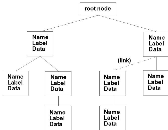
Figure 1: Example CGNS tree-like structure.
