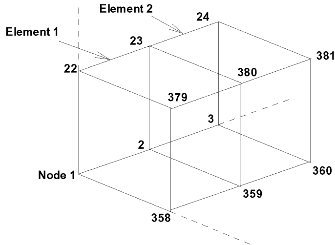
Figure 13: Schematic representation of nodes and elements of unstructured grid.
