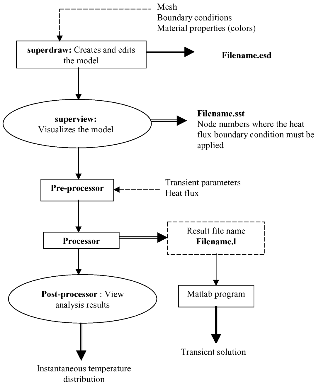
Figure 3.3. Summary of stages used in ALGOR
