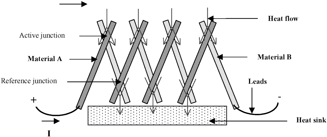
Figure 2.5. Example of a Thermopile
