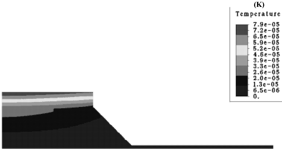
Figure 3.11. Temperature distribution obtained with ALGOR
