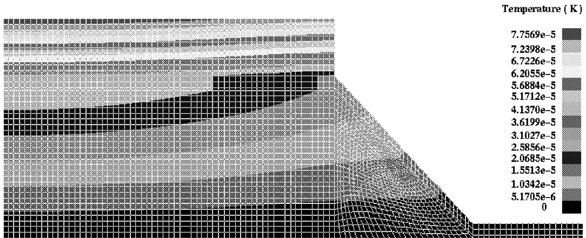
Figure 3.12. Temperature distribution obtained with PATRAN-ABAQUS
