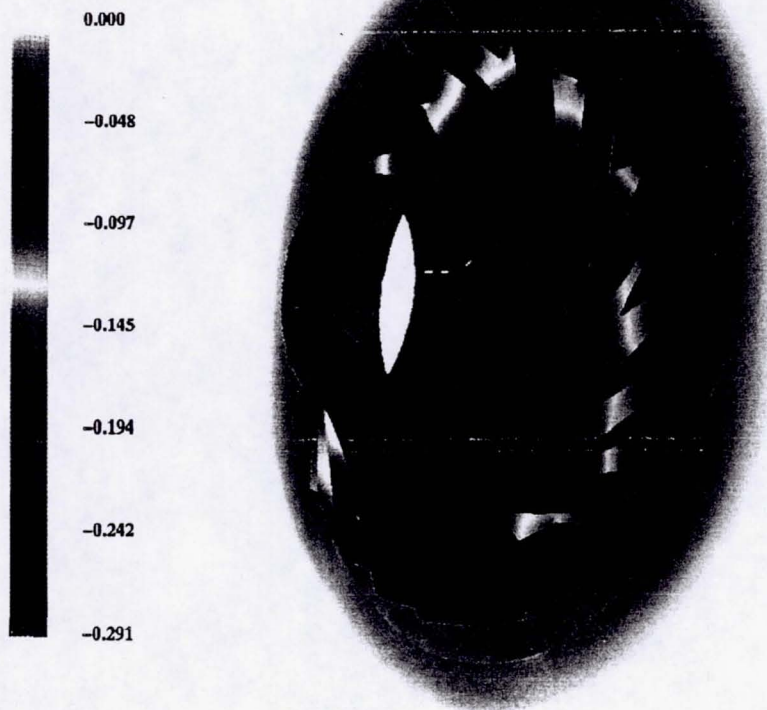
Figure 8. Computed surface pressure for SSME-HPFT impeller.
