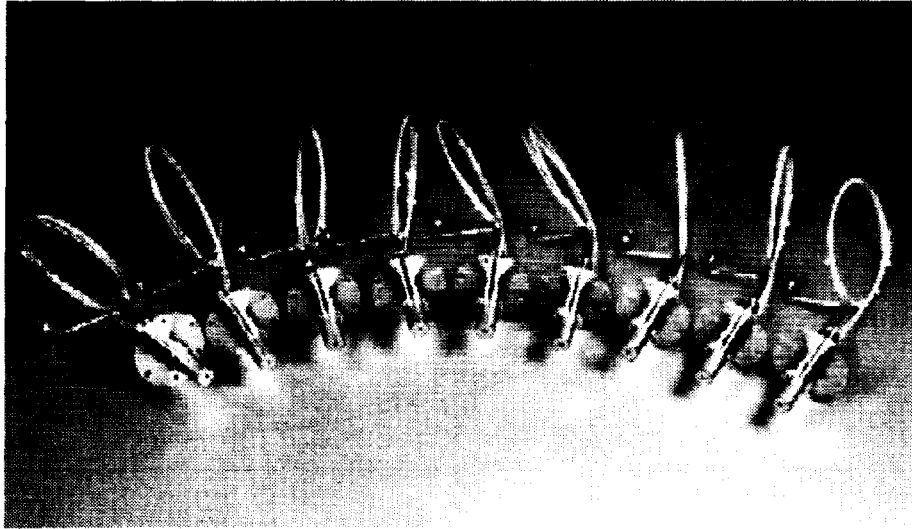
Figure 11. Photograph of 9 out of 12 flight HCA's designed and manufactured by NASA Glenn Research Center in support of the International Space Station plasma contactor program.
