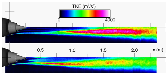
Figure 14. Turbulent kinetic energy measured 3BB (above) and 3A 12 B (below) nozzle systems.
