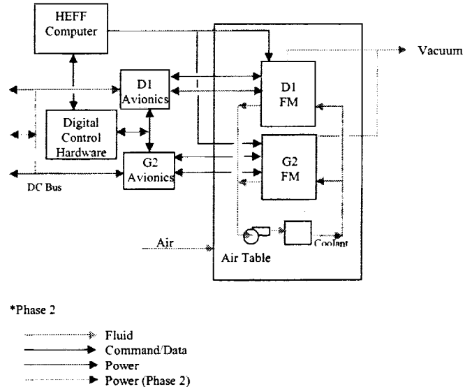
Figure 5. ACESE System Schematic
