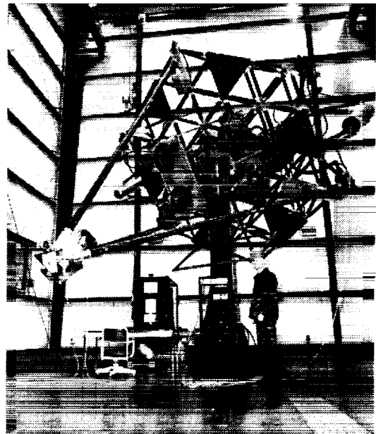
Figure 1 ASTREX Test-Bed at AFRL
