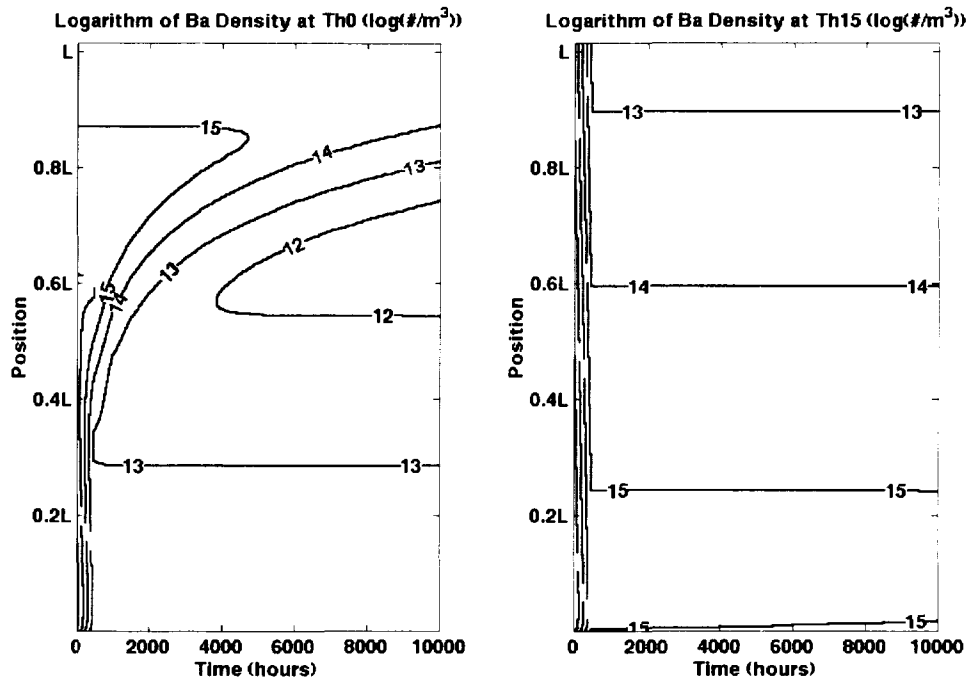
Figure 7. Comparison of gaseous Ba density in the interior of an NSTAR-like discharge cathode modeled at throttle levels TH0 and TH15. Cathode operation over 10,000 hours at each throttle level was modeled. Position given relative to L, which represents the NSTAR emitter insert length.
