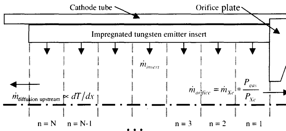
Figure 2. Schematic diagram of the hollow cathode diffusion model. The slices indicate slices of the 1-D diffusion model. Upstream and downstream boundary conditions are indicated. Ba or BaO gas supply from the emitter insert is treated as volume generation within a slice.
