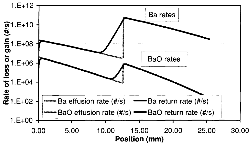
Figure 4. Rate of outward flow of Ba or BaO from the emitter or rate of return of those gases back to the emitter after 2000 hours of model operation. Rates stated in number per second. Discontinuity in outward flow rate is due to a localized phase change after loss of BaO from the impregnate. Dominant BaO producing phase changes from a high vapor pressure phase to a low vapor pressure phase.
