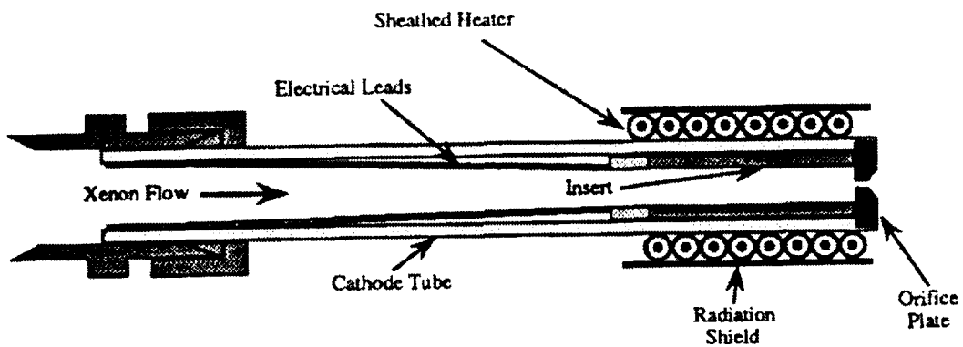
Figure 1. Diagram of a xenon hollow cathode (drawing not to scale) [14]. The direction of xenon flow is indicated.
