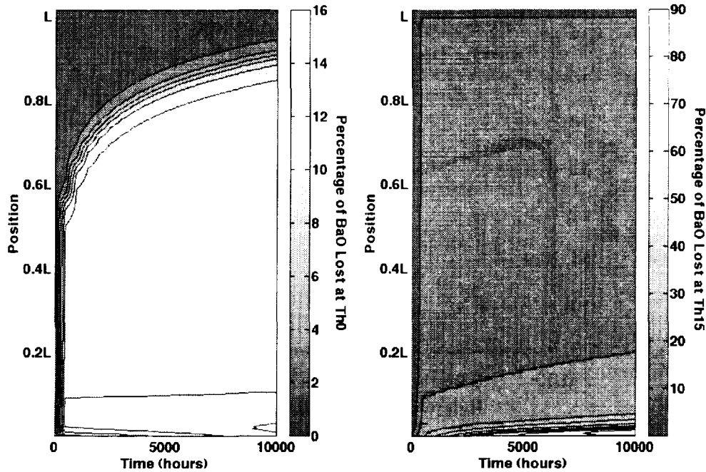
Figure 6. Comparison of BaO loss from the emitter insert of an NSTAR-like discharge cathode modeled at throttle levels TH0 and TH15. Cathode operation over 10,000 hours at each throttle level was modeled. Color keys to the right of each contour plot indicate the percentage of BaO lost. Position given relative to L, which represents the NSTAR emitter insert length.
