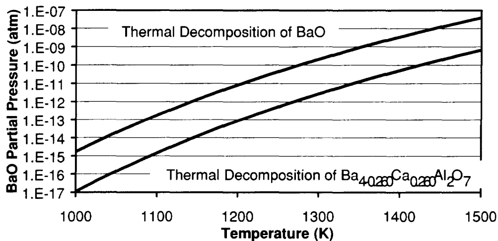
Figure 3. Partial pressure of gaseous BaO for the thermal decomposition of pure BaO and of a Ba_4Al_2O_7 with substitutional Ca. These are the phases in 4:1:1 dispenser cathode impregnates active in production of gaseous BaO.
