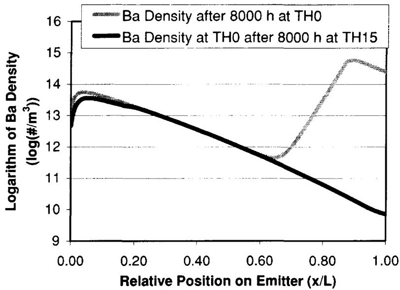
Figure 8. Comparison of gaseous Ba density in the interior of an NSTAR-like discharge cathode modeled at throttle levels TH0 and TH15. Ba densities are produced at TH0 for both cathodes, after 8000 hours of operation at their individual operating points. Position given relative to L, which represents the NSTAR emitter insert length.
