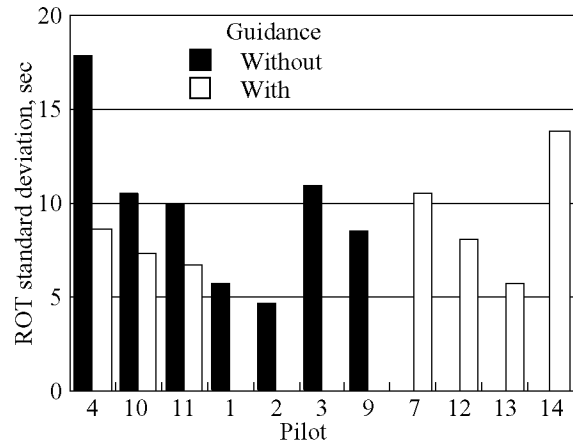
Figure 13. ROT standard deviation for subject pilot for 1200-ft RVR.
