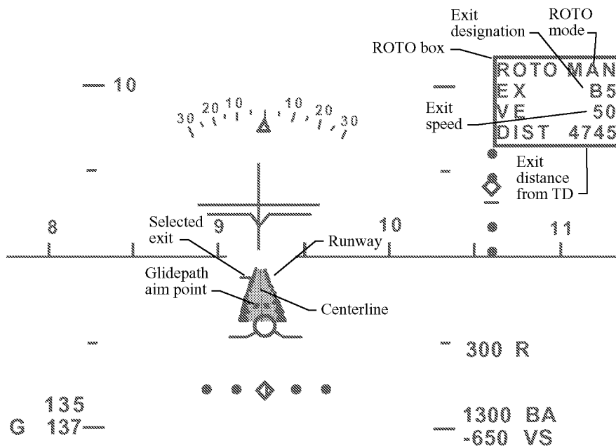
Figure 4. Approach symbology.
