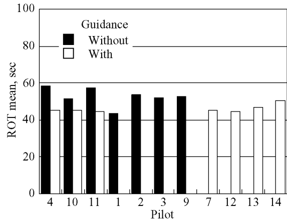
Figure 12. ROT mean for subject pilot for 1200-ft RVR.
