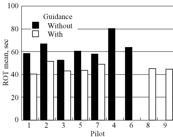
Figure 10. ROT mean for subject pilot for 300-ft RVR.
