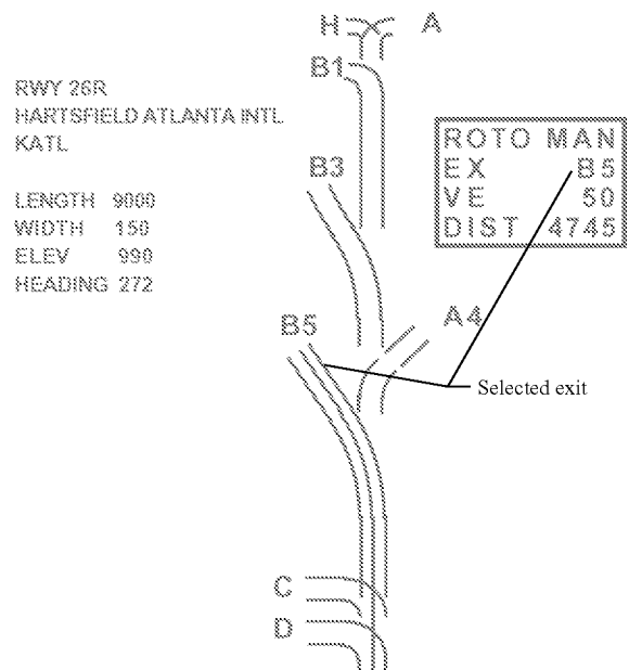
Figure 5. Plan view of runway exits.
