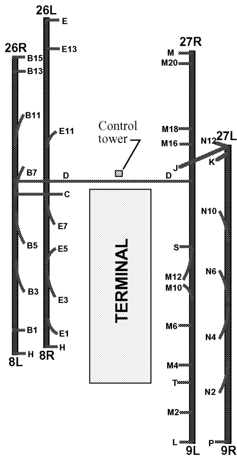
Figure 9. Hartsfield Atlanta runway exits towards terminal.
