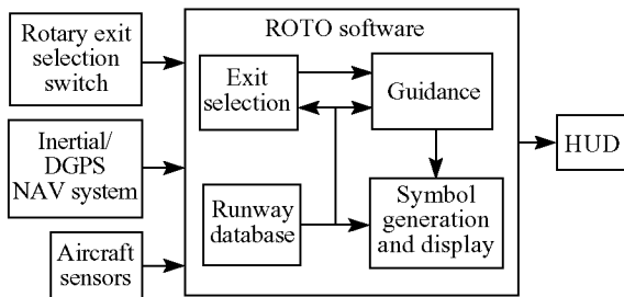
Figure 1. ROTO system.
