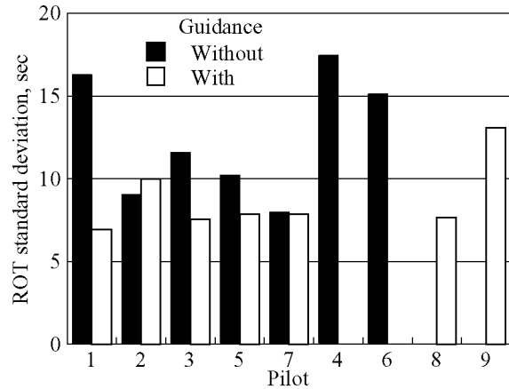
Figure 11. ROT standard deviation for subject pilot for 300-ft RVR.
