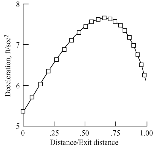
Figure 3. Example of nonlinear deceleration for computed speed profile.
