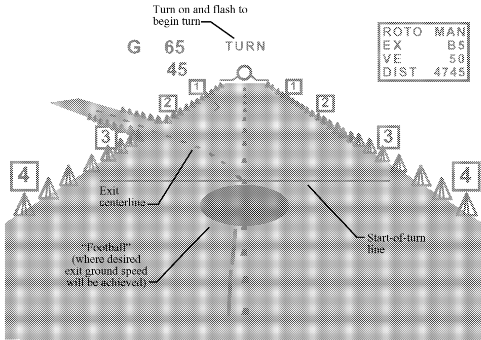
Figure 7. Rollout symbology near exit.
