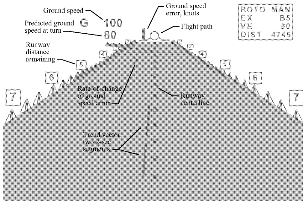
Figure 6. Rollout symbology immediately after touchdown.
