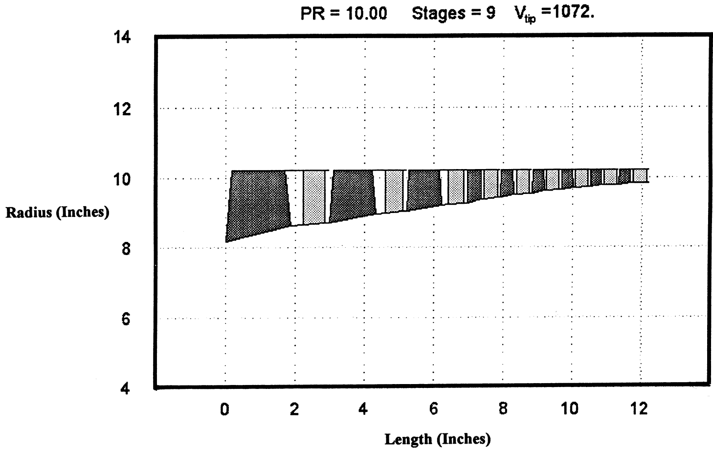
Figure 16. Small-Size Single Spool Exoskeletal Engine – Core Compressor
