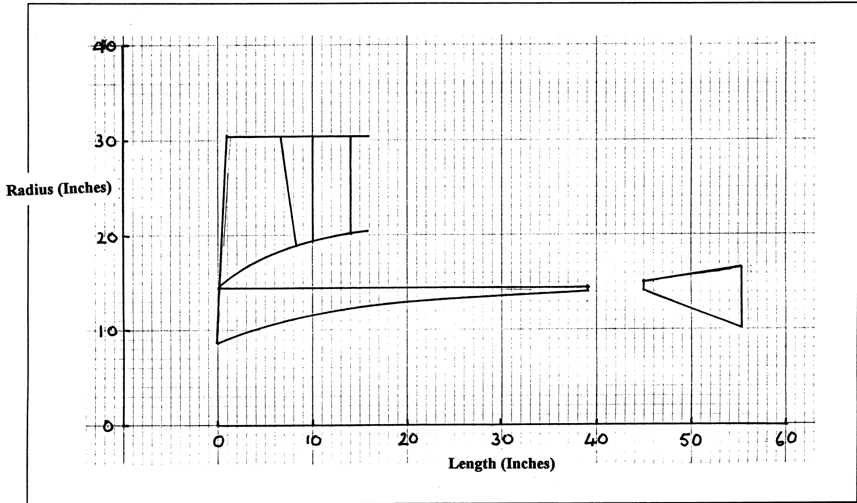
Figure 8. Mid-Size, Single-Spool, Exoskeletal Engine, BPR = 5.1 Engine Layout
