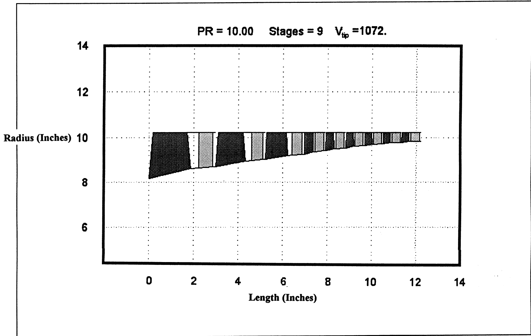
Figure 23. 5,000-lbf Thrust Exoskeletal Turbofan – Core Compressor
