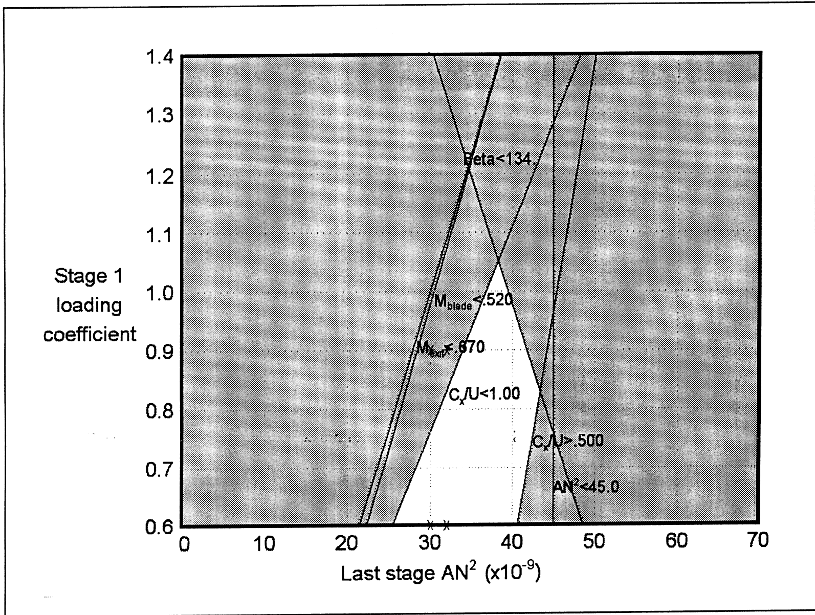
Figure 21. Mid-Size, Single-Spool, Exoskeletal Engine, BPR = 2.0 Design Envelope for the Final Stage of the Uncooled Turbine
