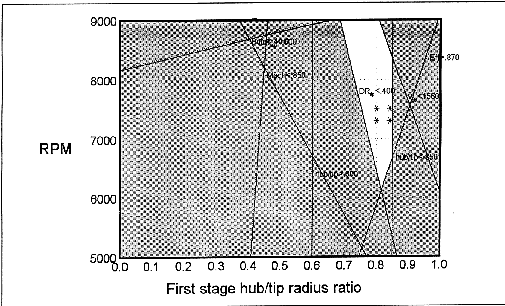
Figure 20. Mid-Size, Single-Spool, Exoskeletal Engine, BPR = 2.0 Design Envelope for the Final Stage of the Core Compressor
