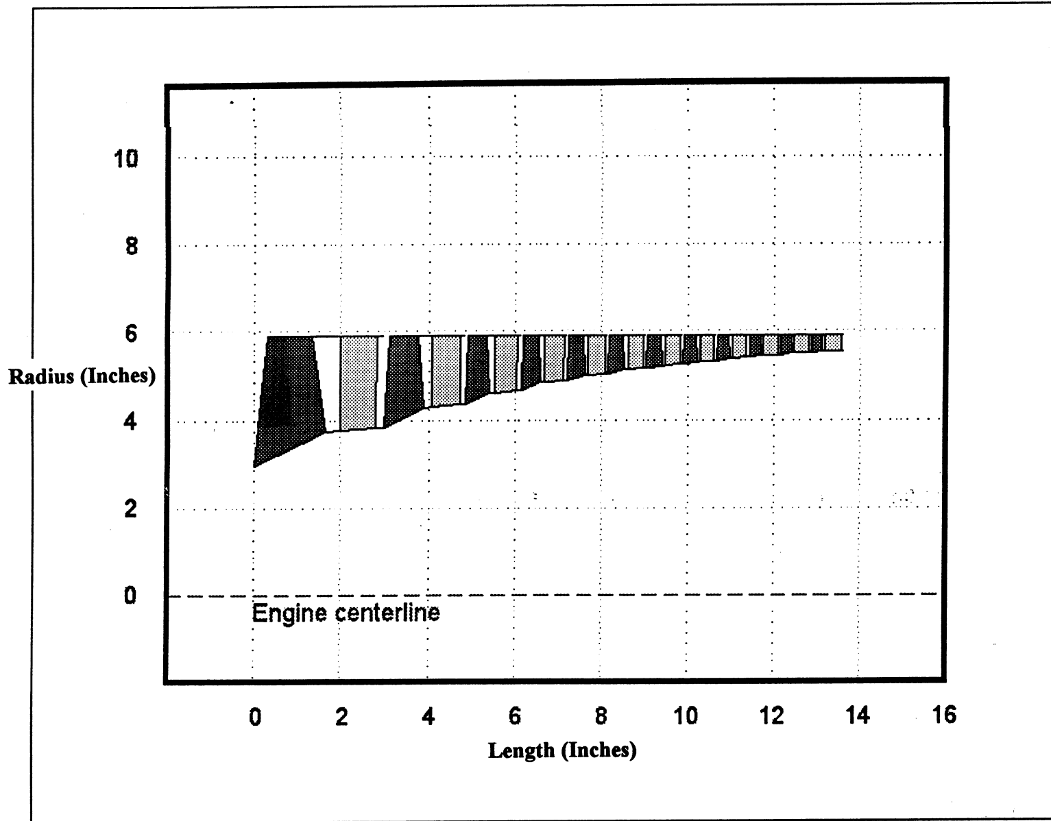
Figure 26. 2,000-lbf Thrust Exoskeletal Turbojet: Compressor
