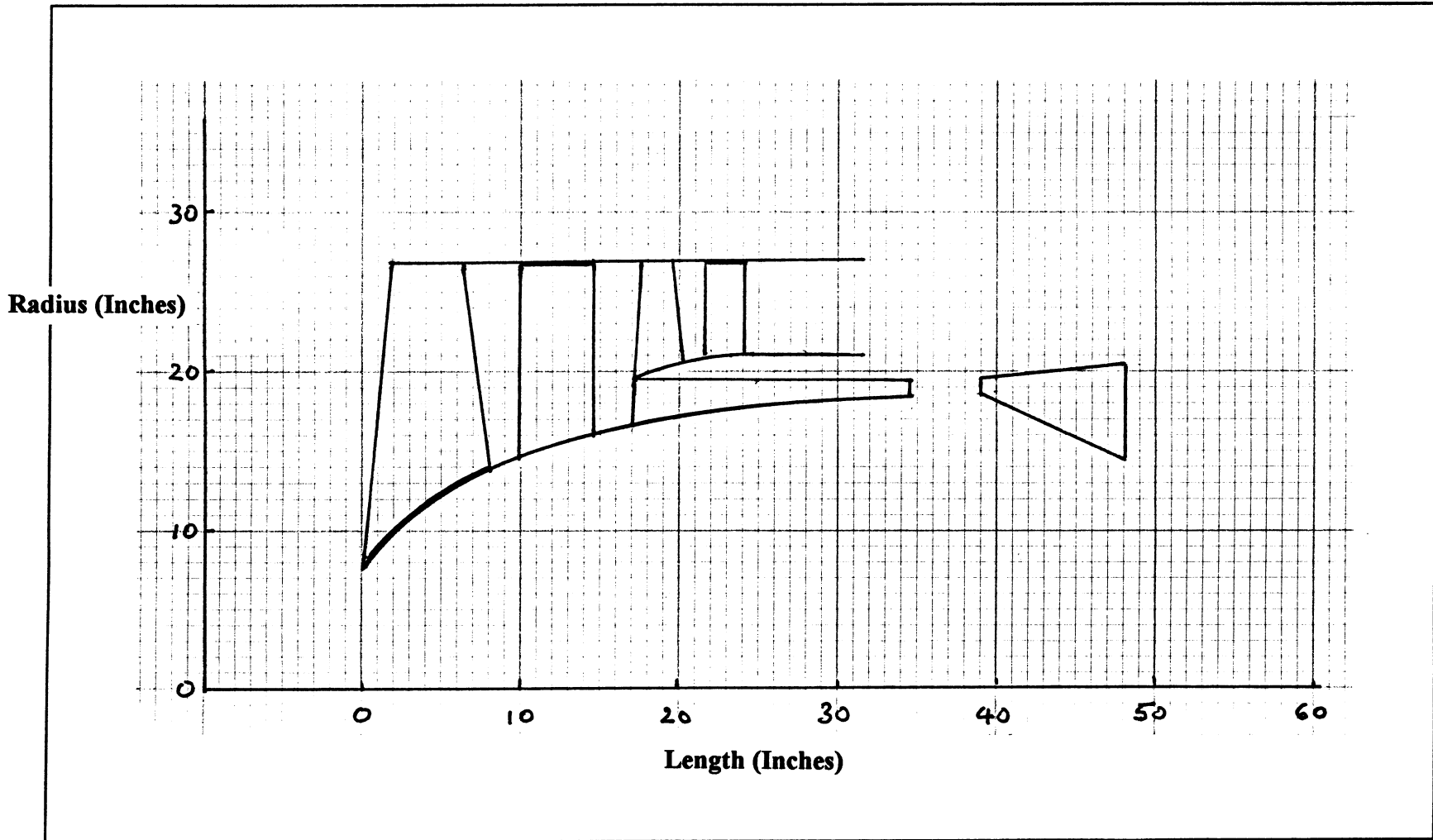
Figure 14. Mid-Size, Single-Spool, Exoskeletal Engine, BPR = 3.0 Engine Layout
