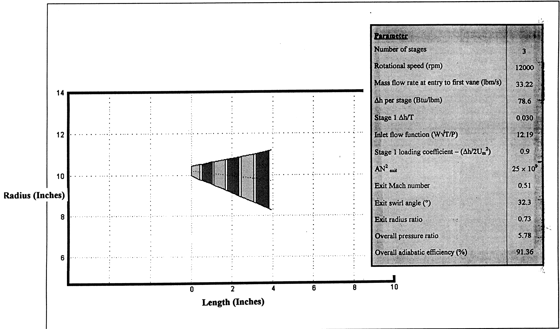
Figure 25. 5,000-lbf Thrust Exoskeletal Turbofan – Uncooled Turbine
