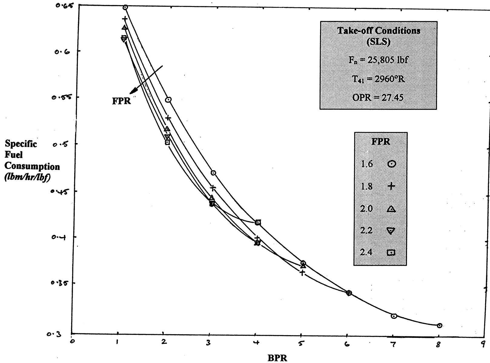
Figure 3. The Effects of Bypass Ratio and Fan Pressure Ratio on Specific Fuel Consumption for a Mid-Size Single-Spool Engine with Separate Exhaust Streams
