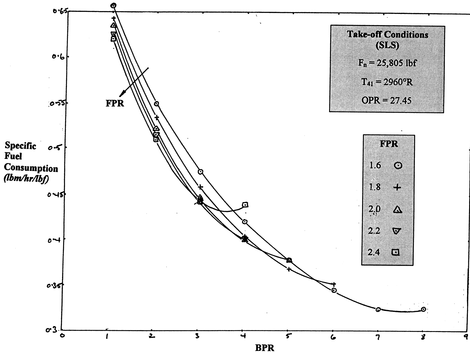
Figure 5. The Effects of Bypass Ratio and Fan Pressure Ratio on Specific Fuel Consumption for a Mid-Size Twin-Spool Engine with Separate Exhaust Streams
