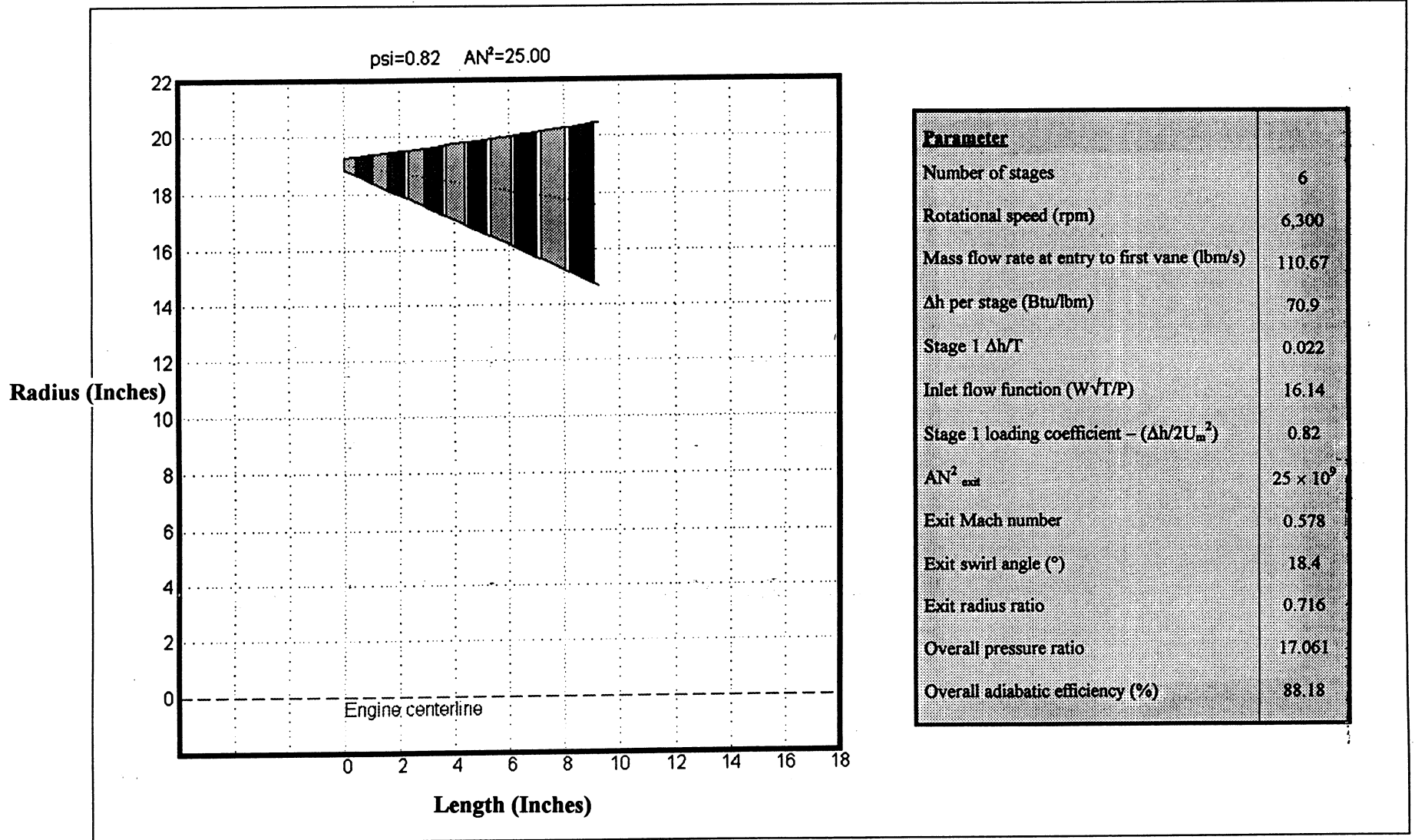
Figure 12. Mid-Size, Single-Spool, Exoskeletal Engine, BPR = 3.0 Cooled Turbine
