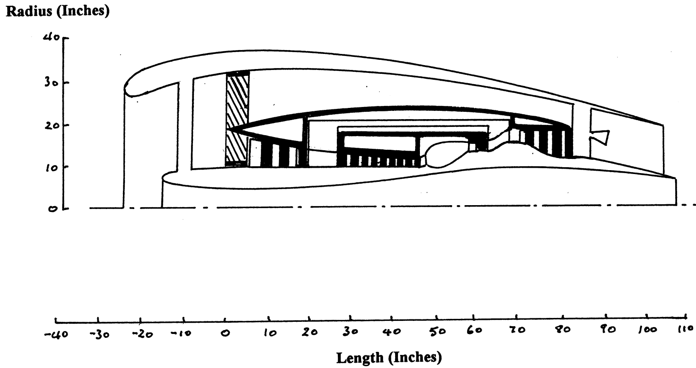
Figure 7. A Possible Twin Spool Configuration for an Exoskeletal Engine
