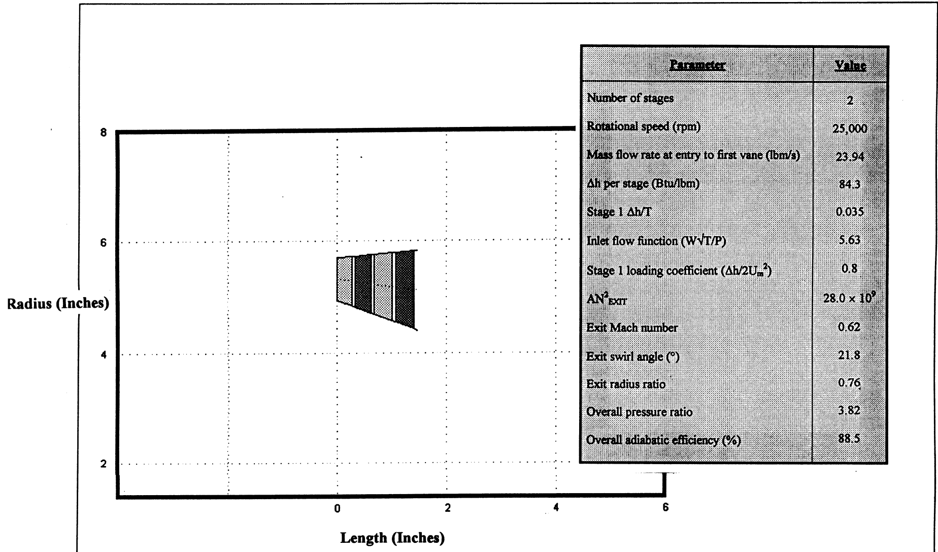
Figure 27. 2,000-lbf Thrust Exoskeletal Turbojet: Turbine (Uncooled)
