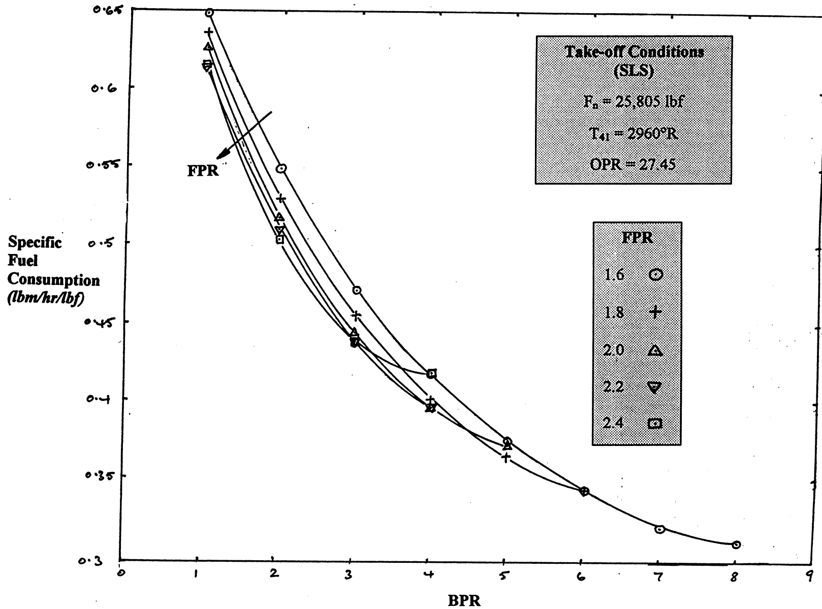
Figure 1. The Effects of Bypass Ratio and Fan Pressure Ratio on Specific Fuel Consumption for a Mid-Size Single-Spool Engine with Separate Exhaust Streams
