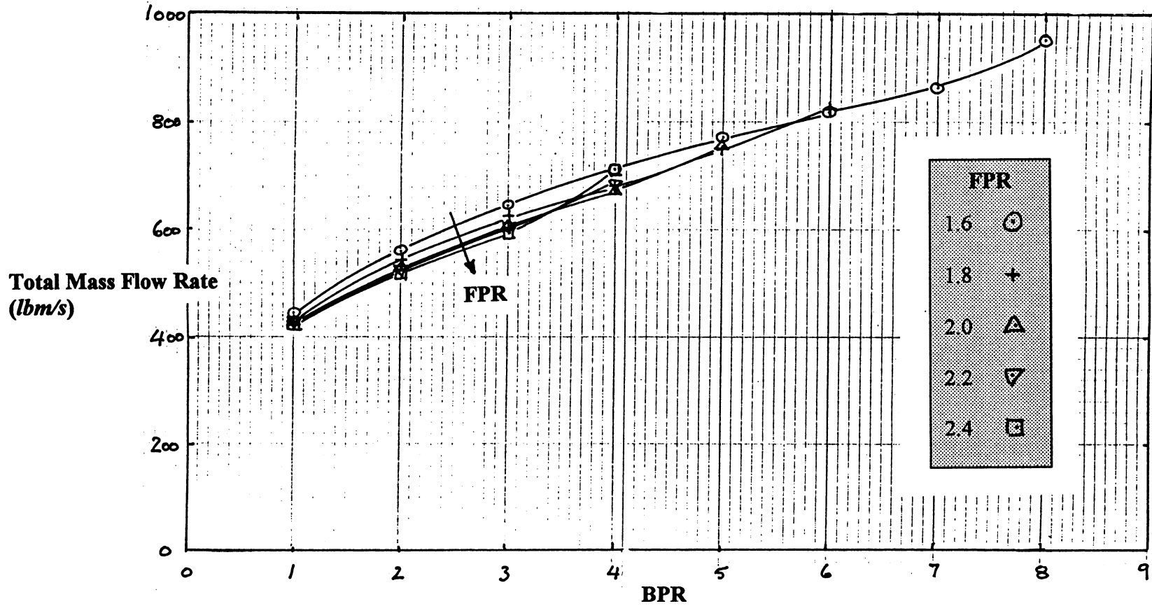
Figure 4. The Effects of Bypass Ratio and Fan Pressure Ratio on Total Mass Flow Rate Required to Produce 25,805 lbf Thrust for a Mid-Size Single-Spool Engine with Separate Exhaust Streams
