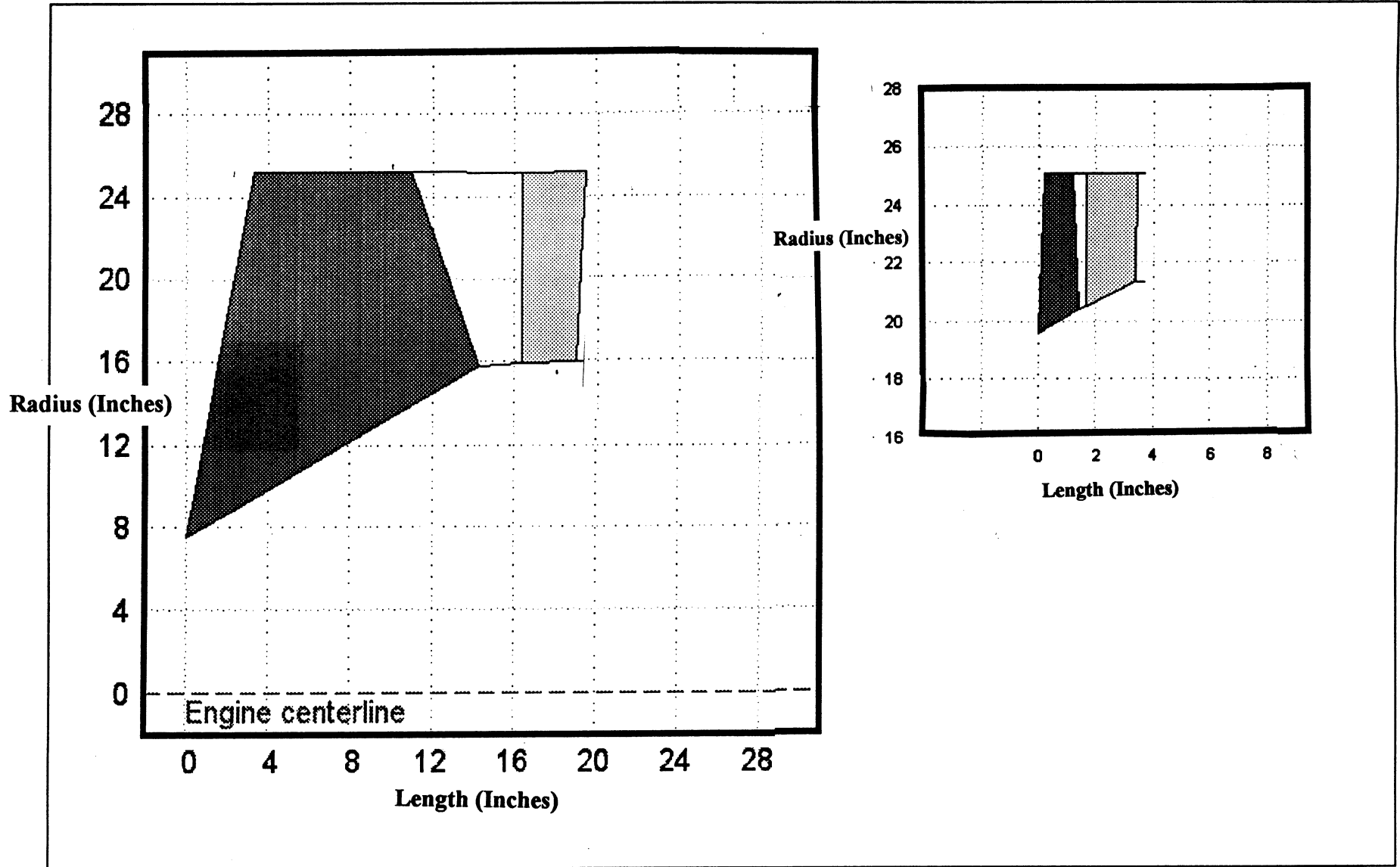
Figure 15. Mid-Size, Single-Spool, Exoskeletal Engine, BPR = 2.0 Fan – Full First Stage & Second Stage Bypass
