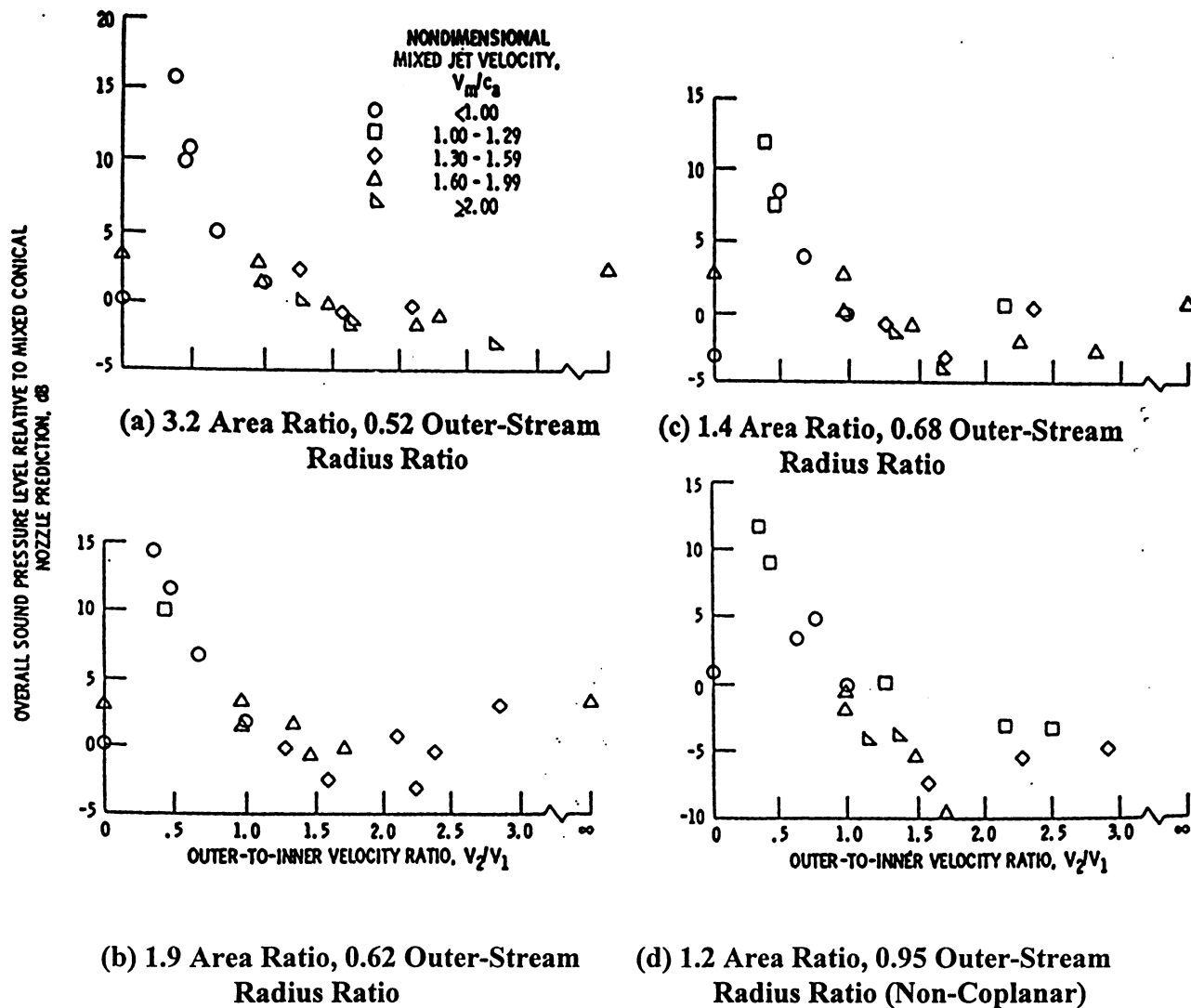
Figure 20. Effect of Velocity Ratio on Noise Relative to Mixed Flow Conical Nozzle Prediction at \theta = 139^\circ (Reference 11)
