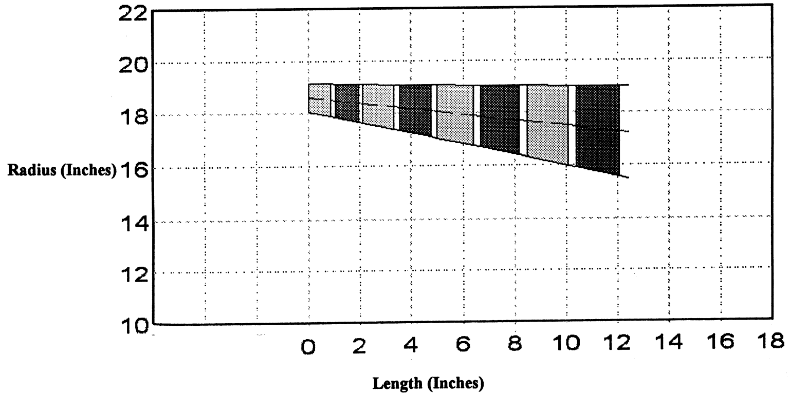
Figure 14. Mid-Size Twin Spool Exoskeletal Engine – 4-Stage LP Turbine
