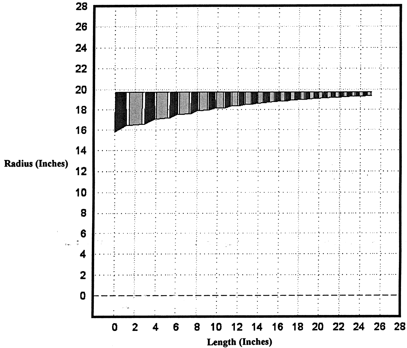
Figure 9. Mid-Size Single Spool Exoskeletal Engine – Core Compressor
