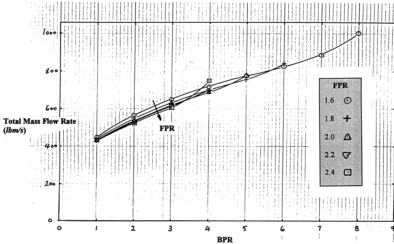
Figure 6. The Effects of Bypass Ratio and Fan Pressure Ratio on Total Mass Flow Rate Required to Produce 25,805 lbf Thrust for a Mid-Size Twin-Spool Engine with Separate Exhaust Streams
