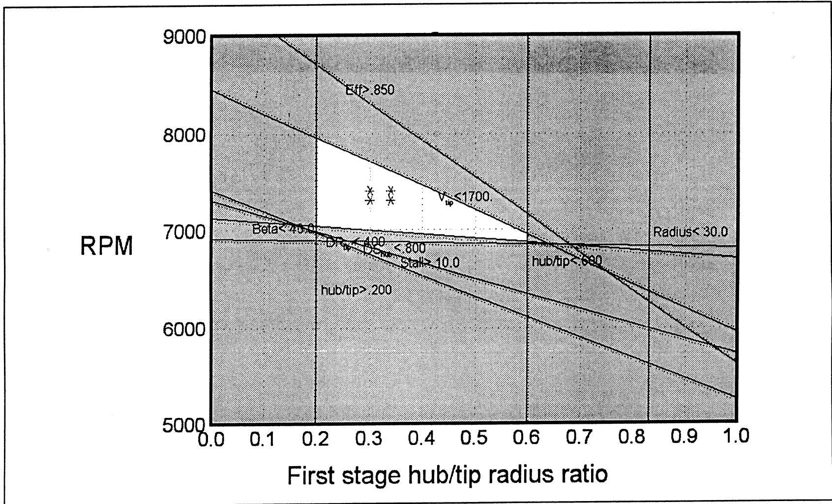
Figure 19. Mid-Size, Single-Spool, Exoskeletal Engine, BPR = 2.0 Design Envelope for the Fan
