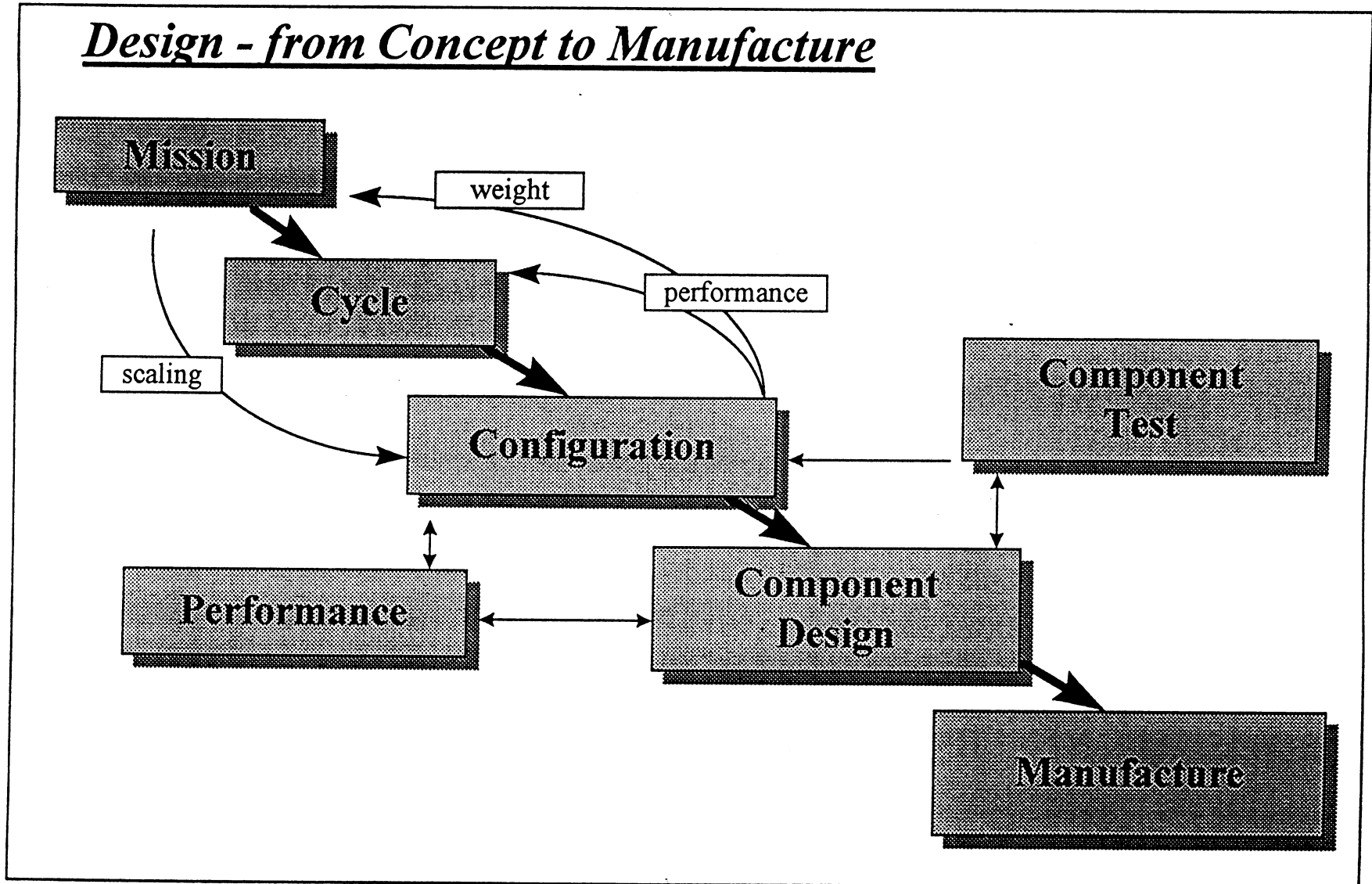
Figure 1. Typical Design Process for a Gas Turbine Engine
