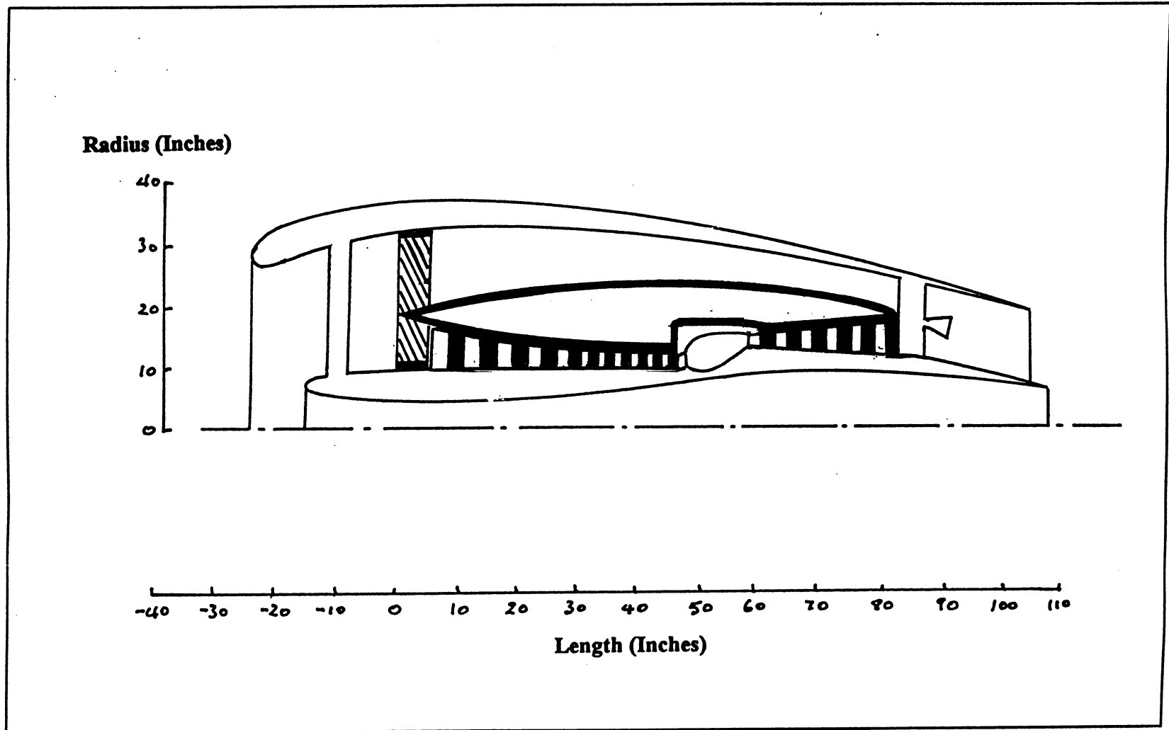
Figure 3. A Possible Single-Spool Configuration for an Exoskeletal Engine
