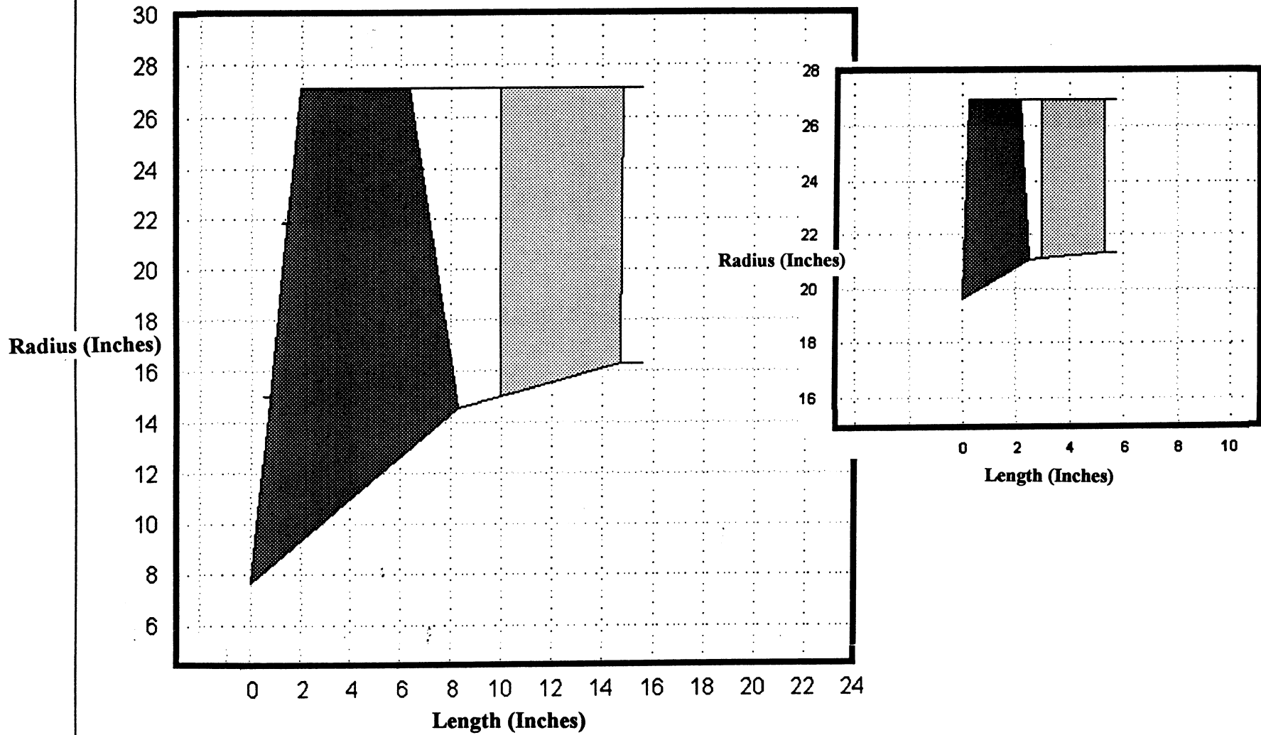
Figure 10. Mid-Size, Single-Spool, Exoskeletal Engine, BPR = 3.0 Fan – Full First Stage & Second Stage Bypass
