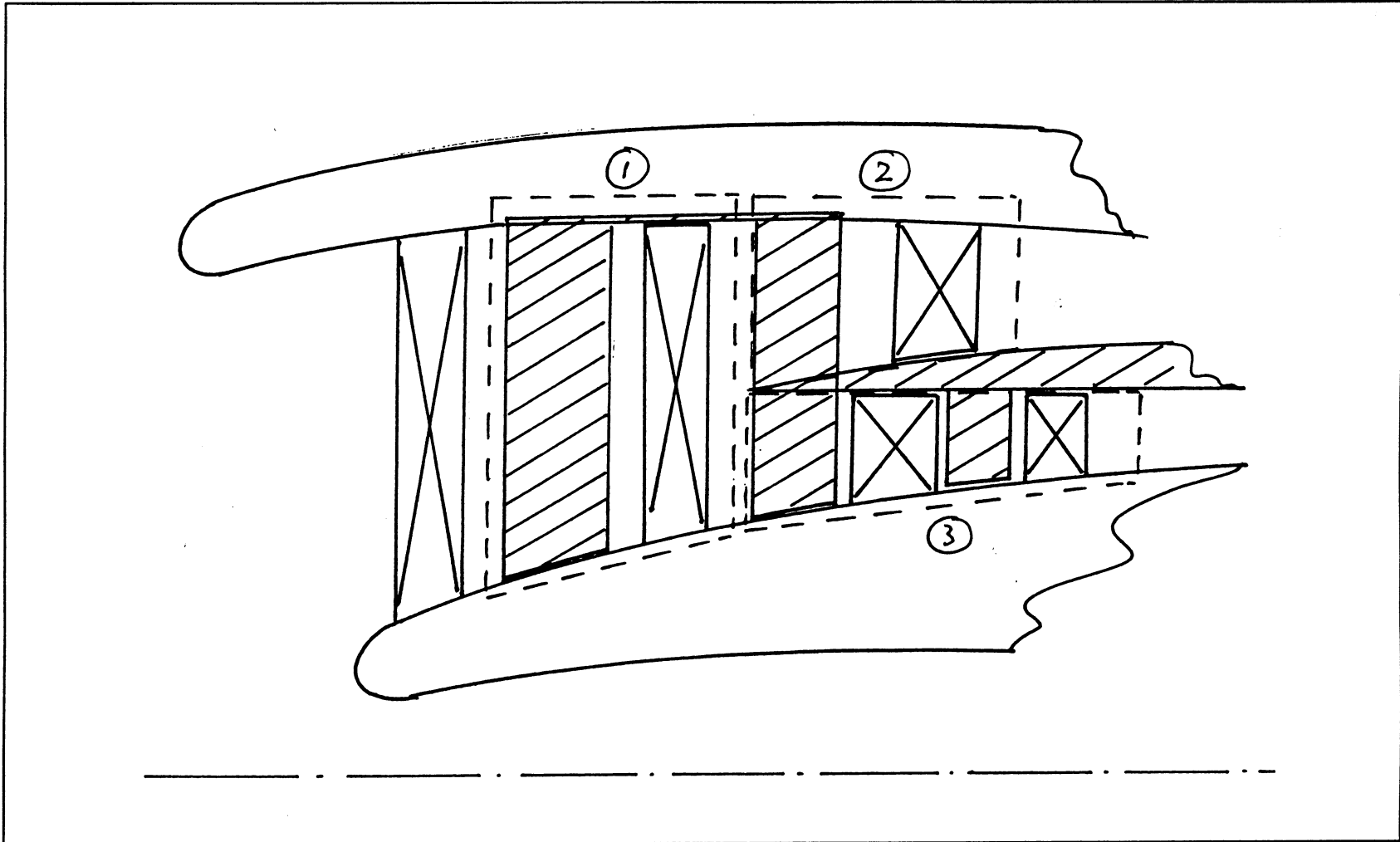
Figure 9. A Possible Split-Fan Configuration for a Low Bypass Ratio, High Fan Pressure Ratio Exoskeletal Engine
