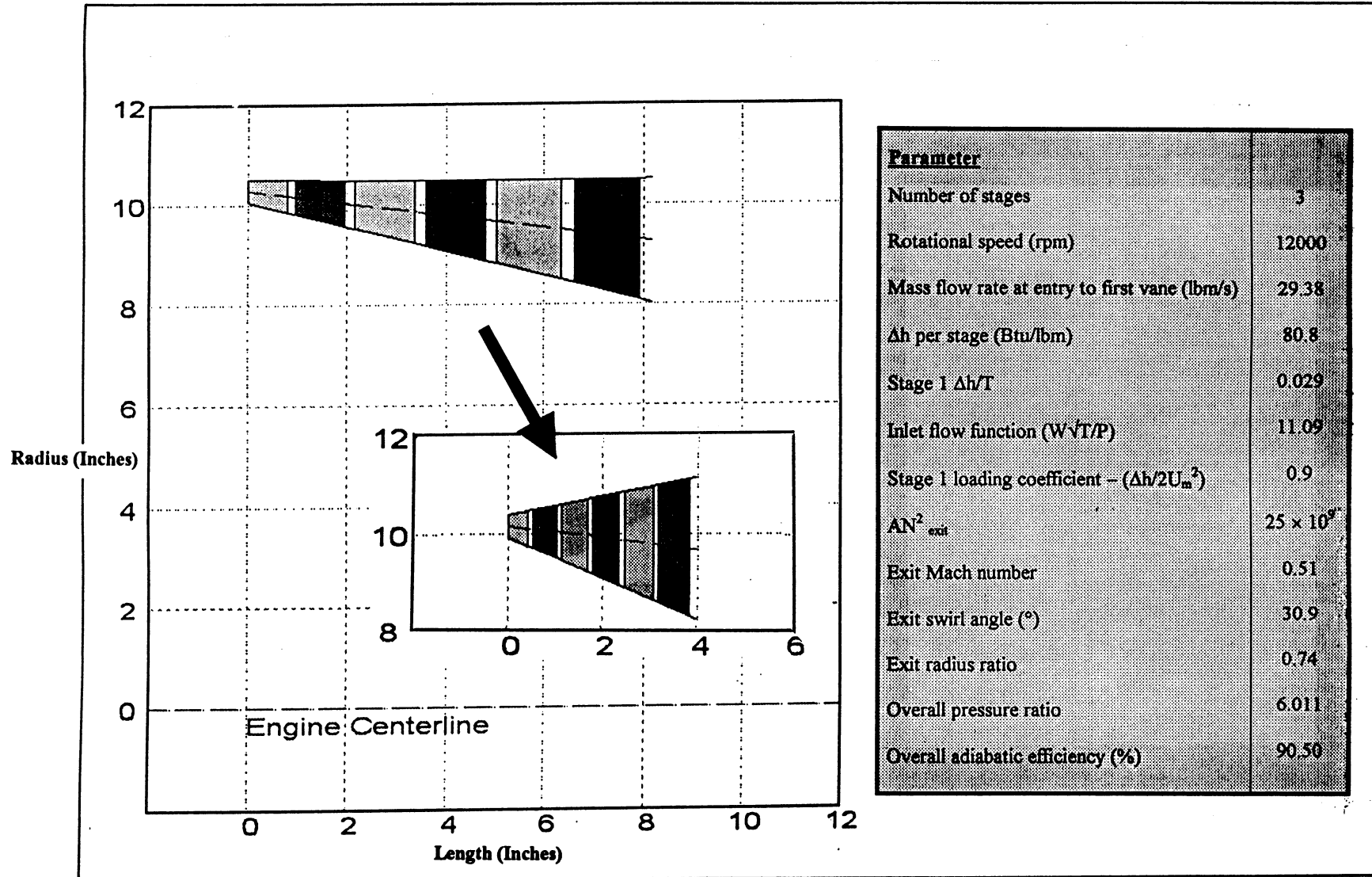
Figure 24. 5,000-lbf Thrust Exoskeletal Turbofan – Cooled Turbine
