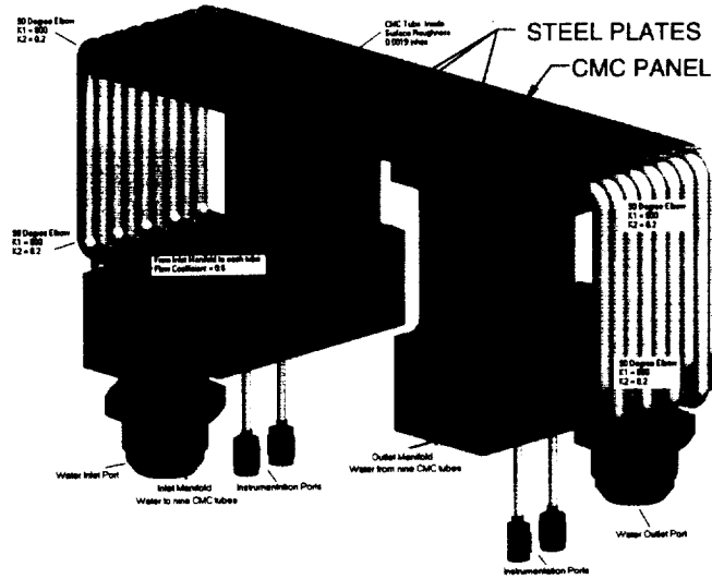
Figure 1: Test Article Assembly with Instrumentation Ports
