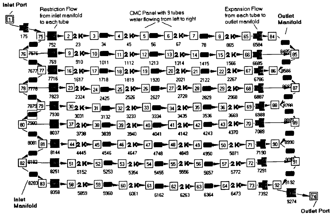
Figure 2: GFSSP model schematic of 9 tube panel with inlet and outlet manifolds
