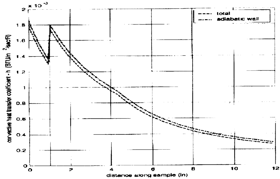
Figure 3: Heat Transfer Coefficient Cell 22 Calorimeter test Results
