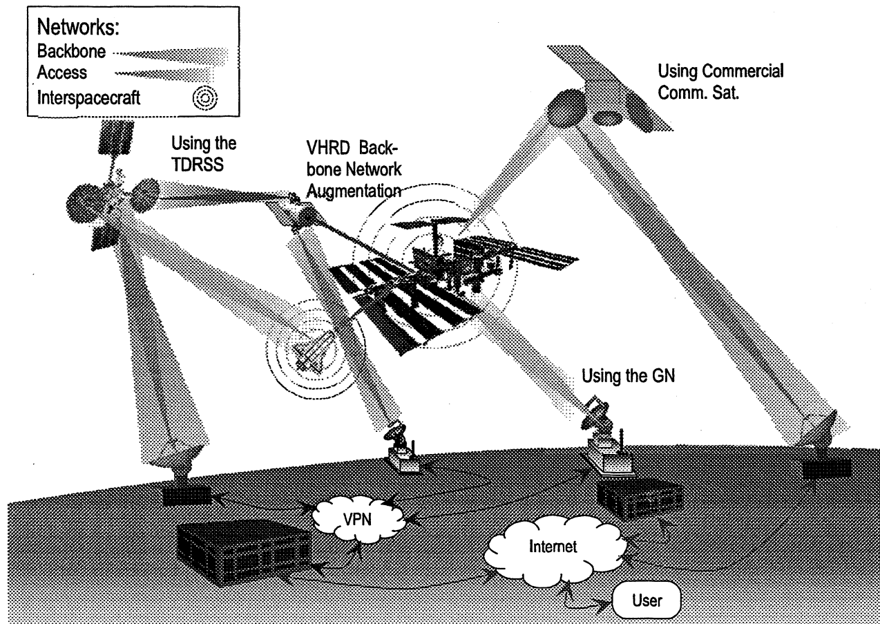
Figure 11, HEDS Architectures
