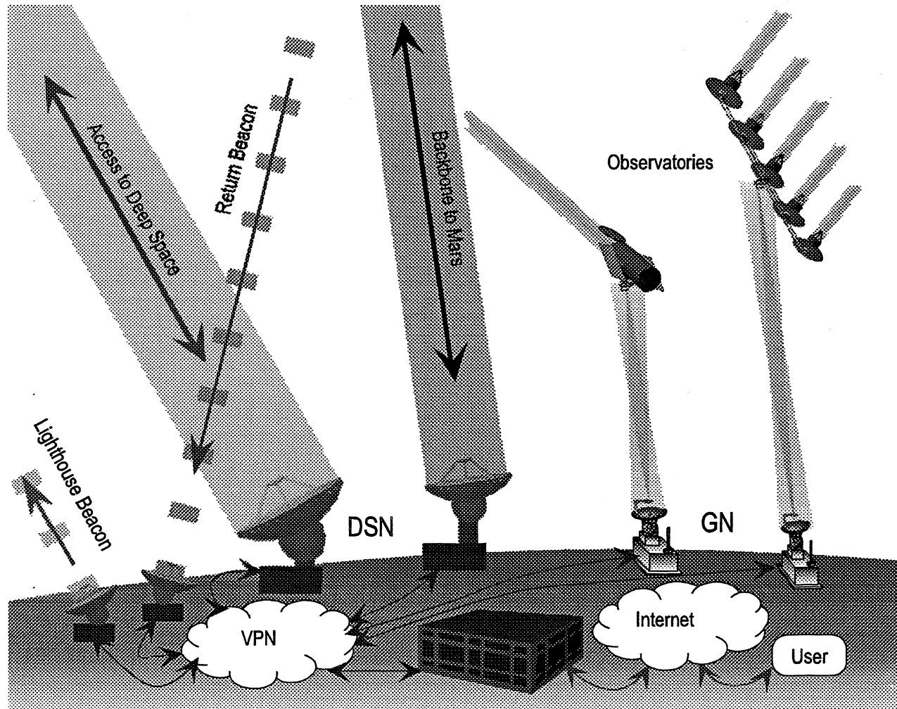
Figure 12, Earth-side Networks for the SSE.
