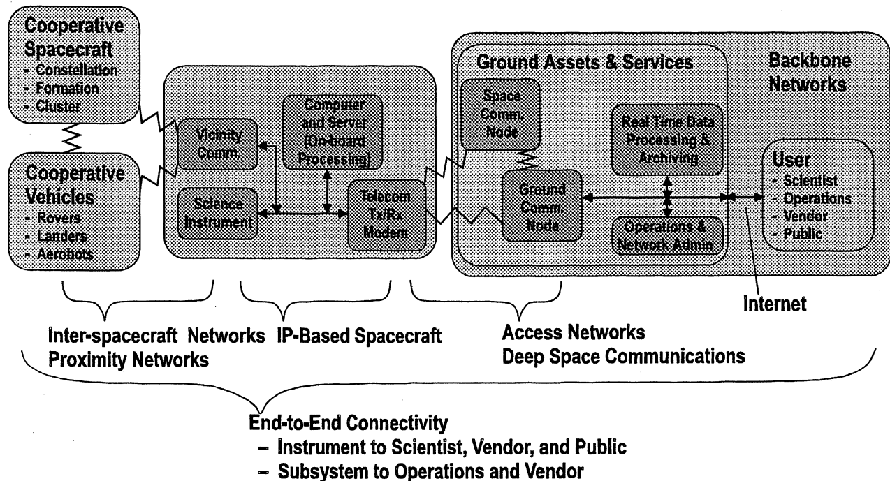
Figure 1, Simplified view of NASA's future communications infrastructure
