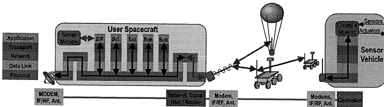
Figure 9, Proximity Network Model – for Sensor Net (Landers/Stations, Rovers, Aero-bots, Airplanes, etc.) and to Relay Spacecraft
