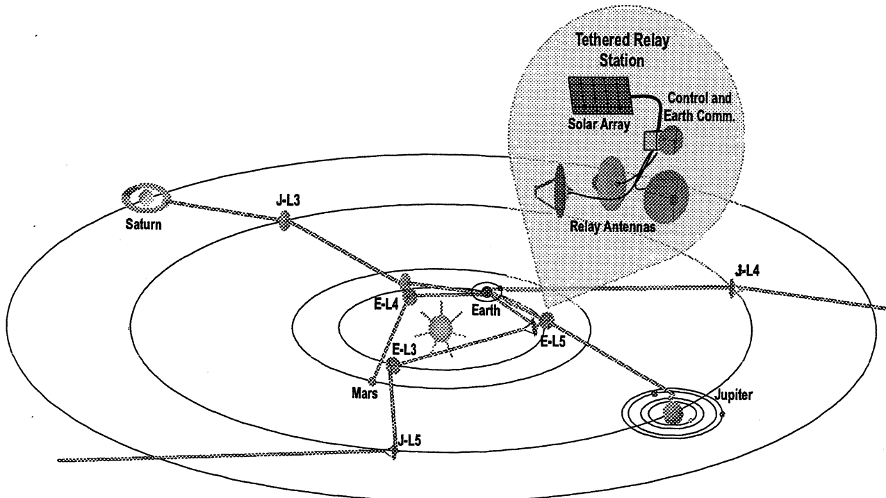
Figure 14, An Architecture for High Data Rate Communications to Deep Space
