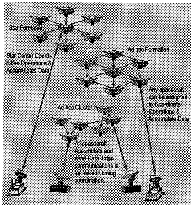
Figure 6, Inter-spacecraft Network Elements
