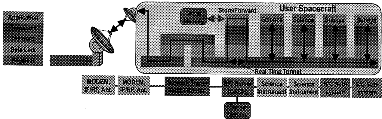
Figure 5, Access Network Model – for Spacecraft to Backbone
