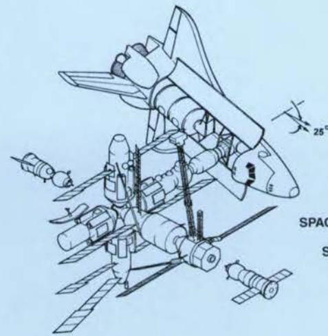
KRISTALL TECHNOLOGY MODULE – 77KST 31 May 1990 19,640 kg (11,270 kg payload) 13.13 m × 4.35 m 60.8 cu m
