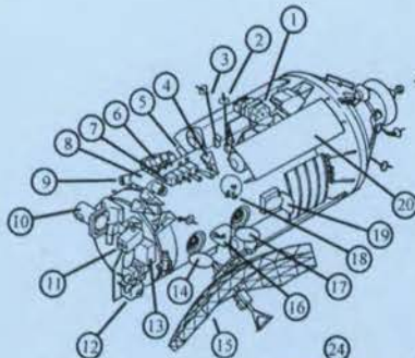
SOYUZ MANNED TRANSPORT Orbital Module 1278 kg Descent Module 2835 kg Instrument Module 3057 kg Spacecraft 7170 kg 6.98 m × 2.72 m, 10.6 m Across Solar Arrays
