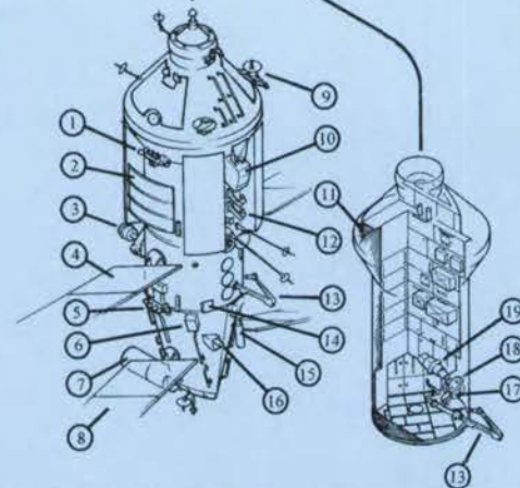
SPEKTR GEOPHYSICAL MODULE – 77KSO 23 May 1995 19,340 kg 14.4 m × 4.36 m 62 cu m
