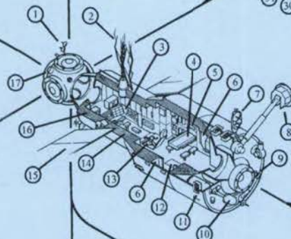
MIR CORE MODULE – 17KS 20 Feb 1986 13.13 m × 4.14 m 20,400 kg 90.0 cu m
