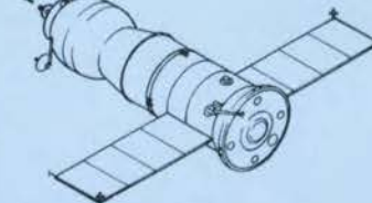
PROGRESS RESUPPLY TRANSPORT Payload 2400 kg Spacecraft 7320 kg 7.23 m × 2.72 m, 10.6 m Across Solar Arrays
