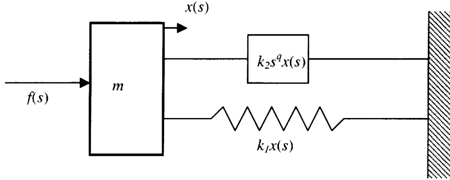
Figure 4.1.1. Spring-mass-viscoelastic system.
