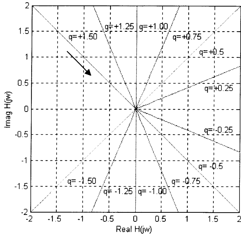
Figure 3.5.2. Nyquist frequency response for fractional-order operators. The arrow shows the direction of increasing frequency.
