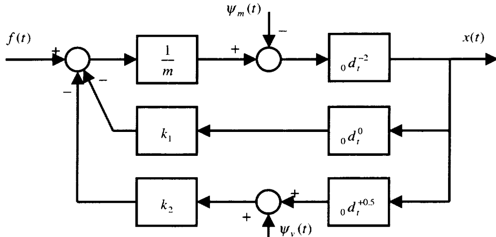
Figure 4.4.1. Integral-form block diagram representation of the mass-spring-visco system.
