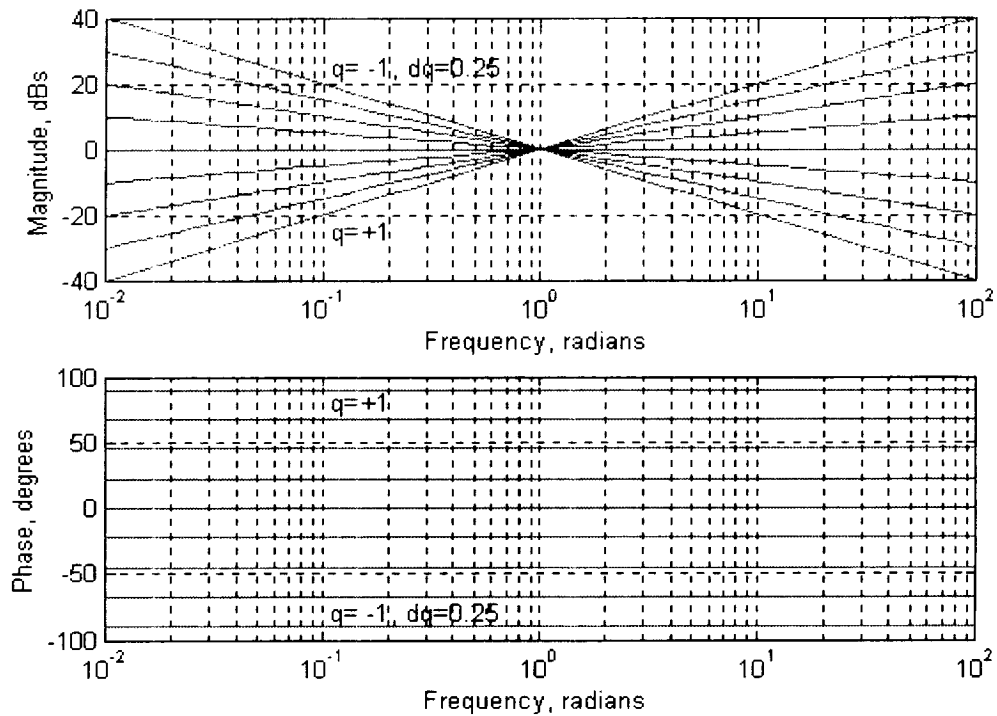
Figure 3.5.1. Bode frequency response for fractional-order operators, with q varying from -1 to +1 in steps of 0.25 .
