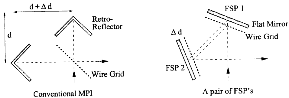
Figure 4: Schematic setup of a conventional MPI and a pair of FSP's. The wires of each grid have an orientation of 45° with respect to the polarization of the incoming radiation.
