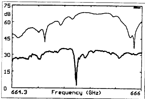
Fig.3. Search for whispering gallery mode resonances in a quartz disc, 18mm diameter, thickness 1mm. The frequency sweep is operated from 664.3 GHz to 666 GHz on the harmonic M=7 of the multiplier (lower trace, resonance found at 665.1 GHz), and, simultaneously, on the harmonic M=6 of the multiplier, from 569.4 GHz to 570.9 GHz (upper trace, resonances found at 569.8 and 570.8 GHz).
