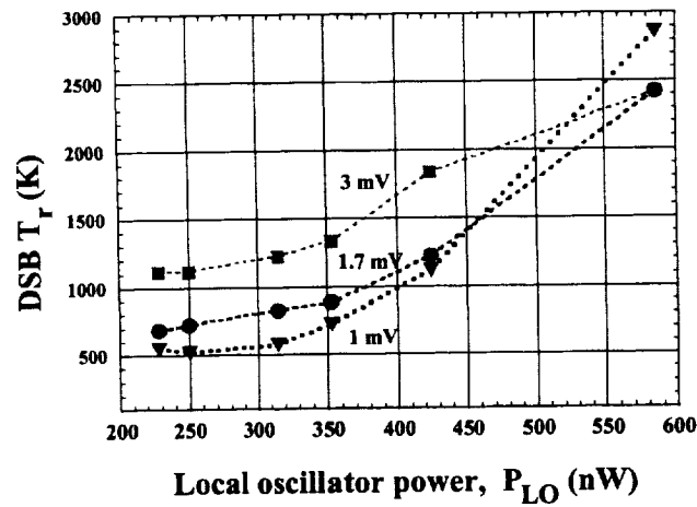
Fig. 3 b DSB receiver noise temperature vs LO power for different bias voltages. Mixer M10-2, width W=4\mu\text{m} , length L=0.4\mu\text{m} . j_c(4.2\text{ K})=1.75 \cdot 10^6\text{ A/cm}^2 , T_c=8\text{ K} .
