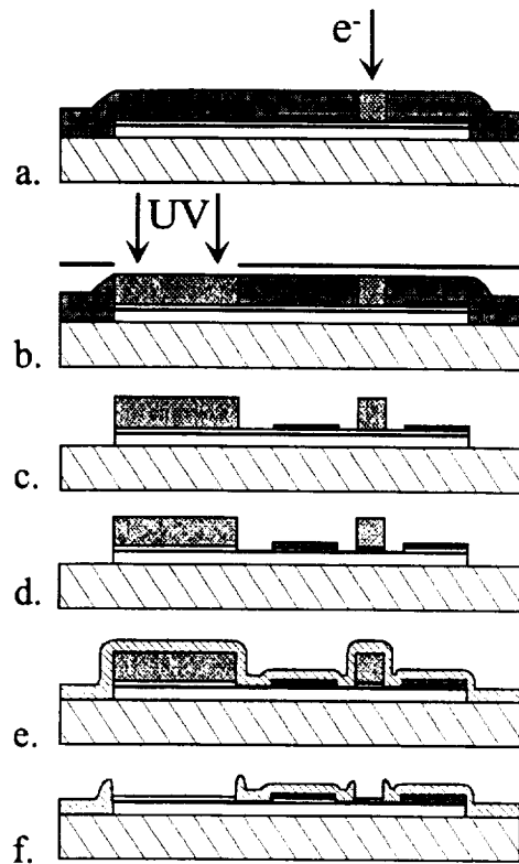
Figure 3. Schematic of the mix & match process: a. e-beam lithography junction definition; b. contact area UV-mask aligner lithography; c. junction and contact pattern after development; d. reactive ion etching of Nb 2 ; e. SiO 2 deposition; f. SiO 2 liftoff.
