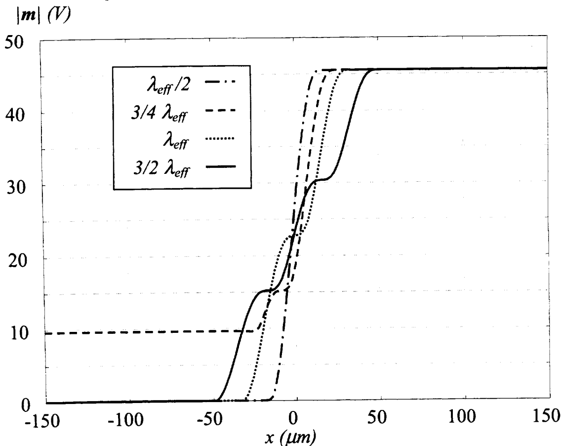
Fig. 3 Magnetic current amplitude on CPW line at the end point of an excitation region indicated in the inset
