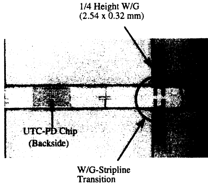
Fig. 3 Waveguide-stripline transition and UTC-PD mounted on a quartz substrate.
