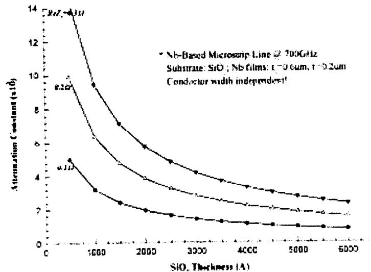
Fig. 1 Attenuation constant vs. substrate thickness.
