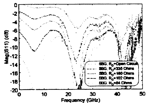
Figure 9: S_{11} measurements of the improved SBG block.
