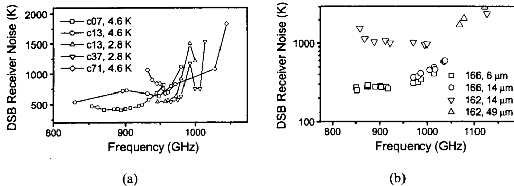
Figure 3 - (a) Measured T_{N,rec} for 4 waveguide devices measured at 4.6 K (c07, c13, and c71) and 2.8 K (c13 and c37). c13, c37, and c71 are measured with a 14- \mu\text{m} beamsplitter, while c07 is measured with a 6- \mu\text{m} beamsplitter (modified from [16]). (b) T_{N,rec} of 2 quasi-optical mixers measured at 2.8 K with 6-, 14-, and 49- \mu\text{m} beamsplitters (modified from [10]).
