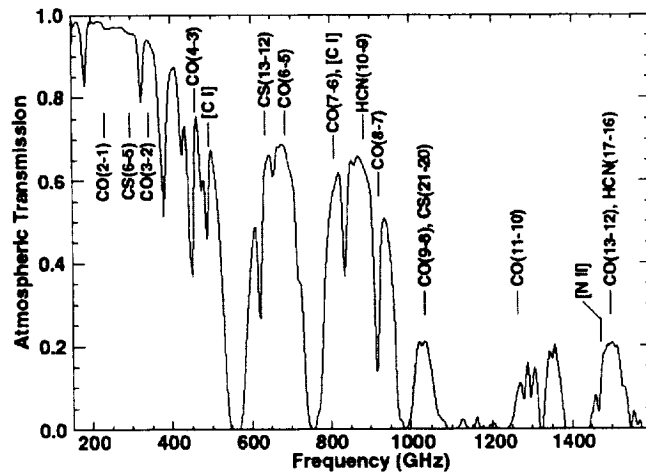
Figure 2: Measured atmospheric transmission spectrum at ASTE site
