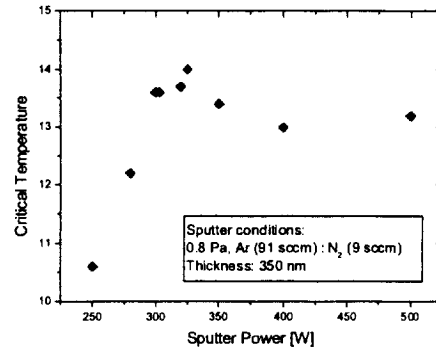
Fig. 1b T c versus sputter power
