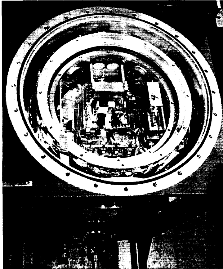
Figure 5: Layout of PoleStar array cryostat.
