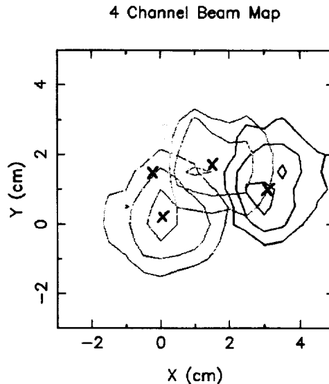
Figure 11: PoleStar beam patterns.
