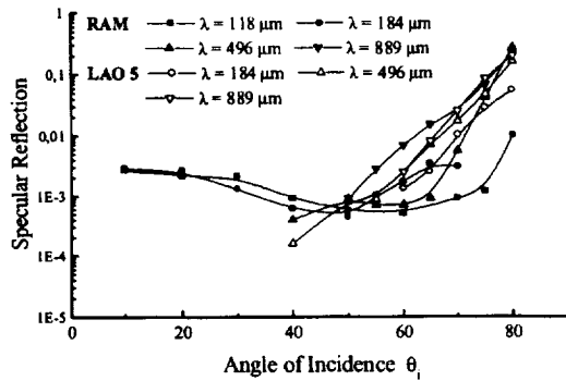
Fig. 3. Specular reflection of RAM and LAO 5
