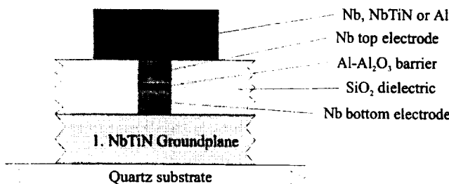
Fig. 3 Sketch of the layer sequence of junction and tuning structure Fig. 4 Microscope photo of a finished device
