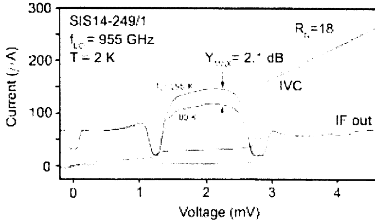
Fig. 5 Unpumped and pumped IV-curves of experimental SIS mixer along with hot/cold response at 955 GHz measured at IF=1.5 GHz. Bath temperature is about 2 K.
