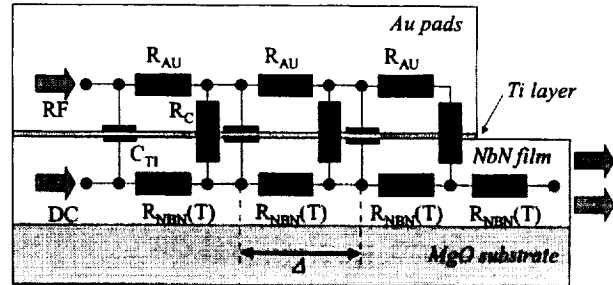
Fig. 1: Equivalent lumped element circuit for the contact resistance problem.
