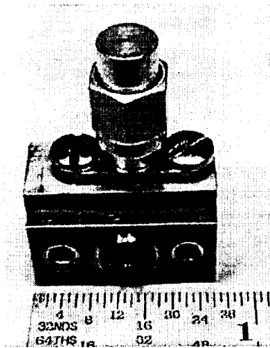
Fig. 3: Assembled MOMED tripler. The outer block dimensions are: HxWxL = 16 x 20 x 10 mm (without the SMA connector).
