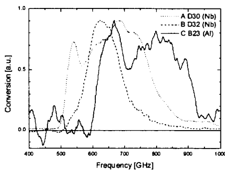
Fig. 8: FTS traces of three devices
