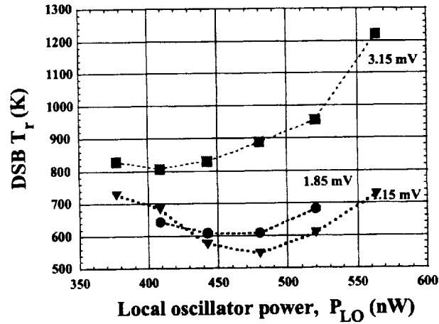
Fig. 3 a DSB receiver noise temperature vs LO power for different bias voltages. Mixer M12-2, width W=4\mu\text{m} , length L=0.4\mu\text{m} . j_c(4.2\text{ K})=2.7 \cdot 10^6\text{ A/cm}^2 , T_c=9.5\text{ K} .
