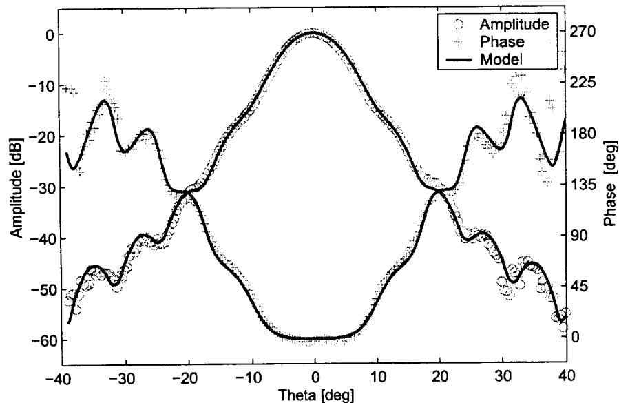
Figure 2: Measured amplitude and phase of the SMILES corrugated horn antenna together with model predictions. This measurement is a cut through the E-plane at a frequency of 602.5 GHz.
