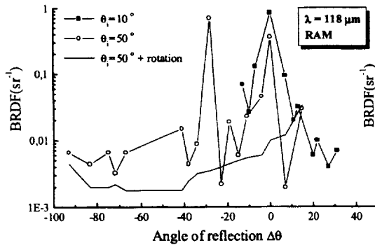
Fig. 5 BRDF of RAM at 118μm
