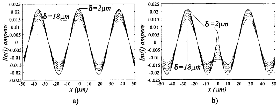
Fig. 3 Current on an example microstrip structure at submillimeter wave frequencies (2.5 THz) obtained using the present direct integration method (equation 2). Real (a) and Imaginary (b) parts are presented for different dimensions of the excitation gap ( \delta varying from 2 to 18 \mu\text{m} ).
