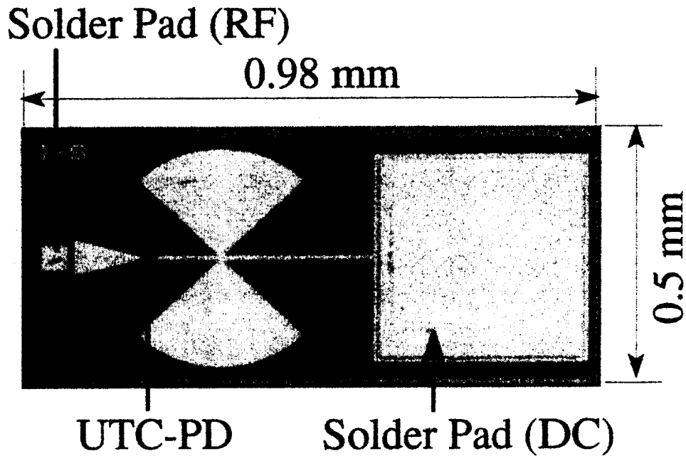
Fig. 2 Photograph of a UTC-PD chip.
