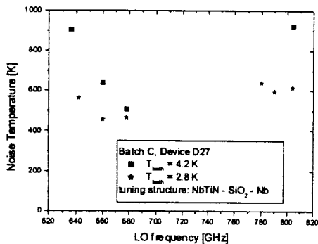
Fig. 9 Results at 2.8 K bath temperature
