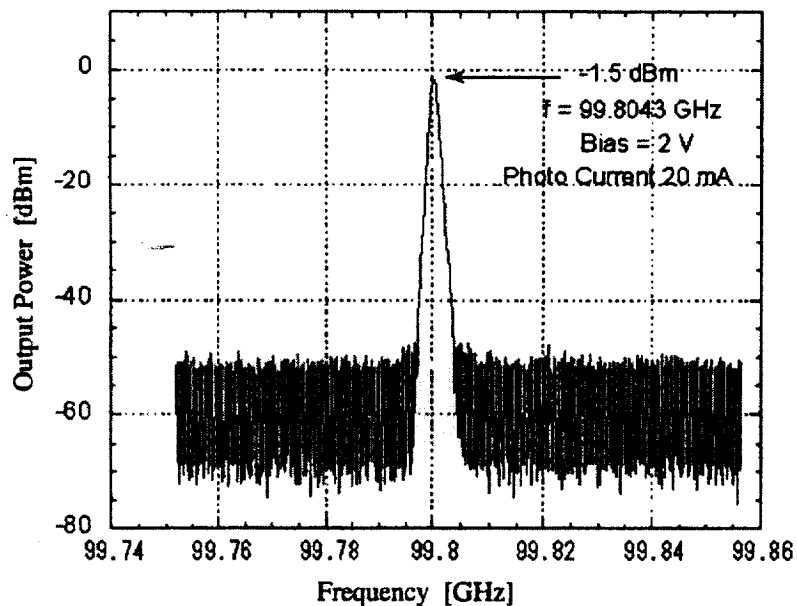
Fig. 8 Spectrum of photomixer output at ~100 GHz.
