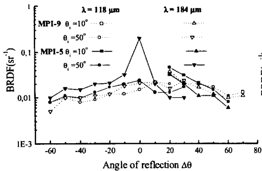
Fig. 9 BRDF of single SiC layer MPI
