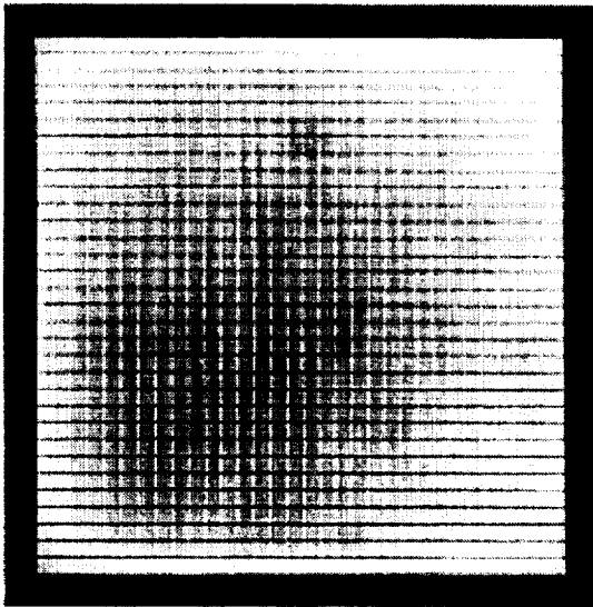
Figure 4 : 32 x 32 array of silicon nitride meshes
