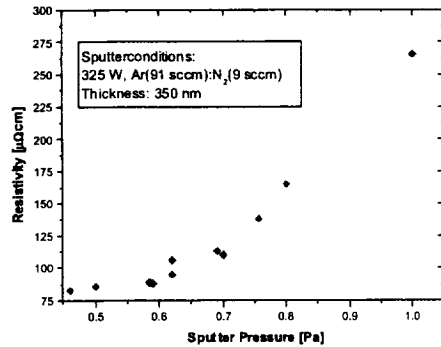
Fig. 1c DC resistivity versus sputter pressure
