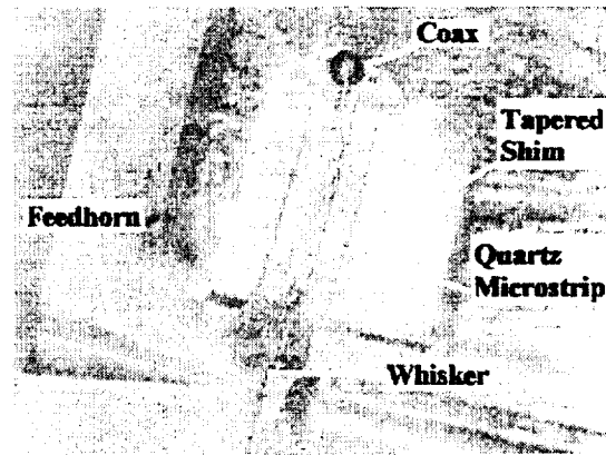
Figure 8: Internal view of the modified SBG block.
