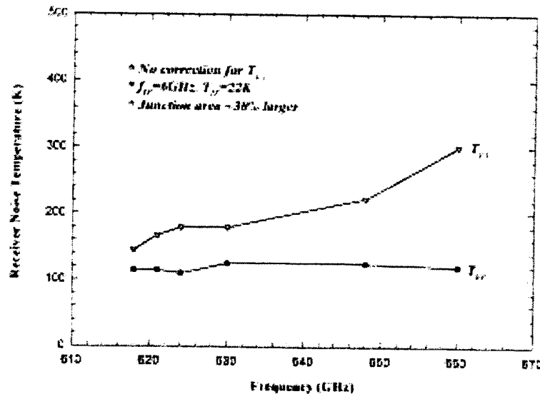
Fig. 6 Measured receiver noise temperature (DSB) for the 660-GHz SIS mixer.
