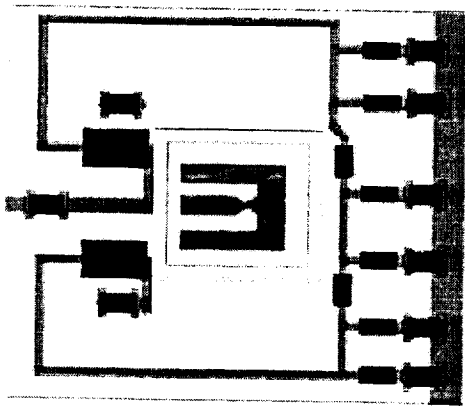
Figure 7. Bias/IF circuit for the TREND NbN receiver
