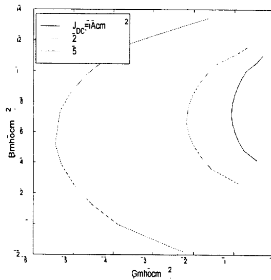
Figure 4: Small Signal G-B Plot, Frequency = 700-1300 GHz, J_{dc} = 100, 200, 500 A/cm^2
