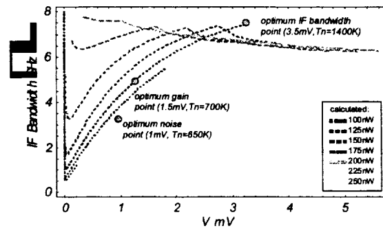
Fig. 8 IF bandwidth for device M2-1. The measured points are obtained for the points with the best noise, the best gain and the best IF gain bandwidth. The measured receiver noises (including optics losses) are indicated.
