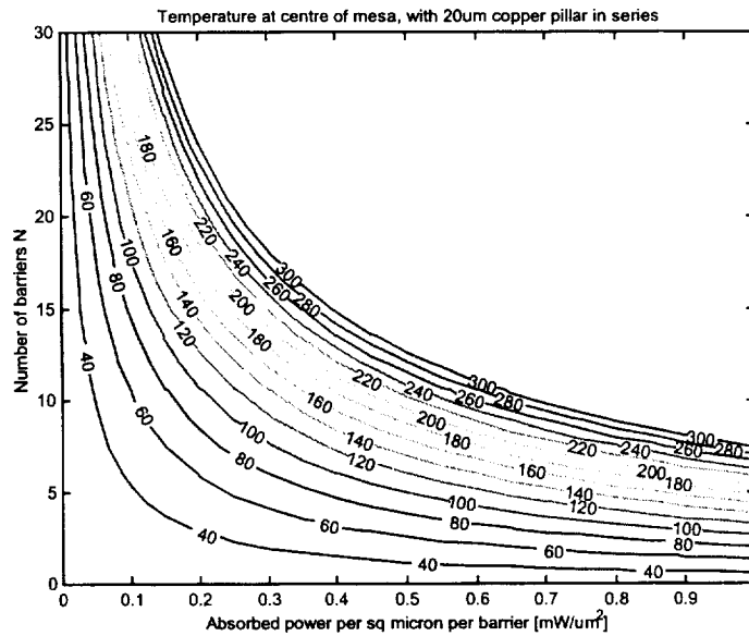
Figure 6) Temperature at the centre of a HBV mesa. The mesa is assumed to be contacted symmetrically by 20 \mu m copper pillars to a perfect thermal conductor at 300K.
