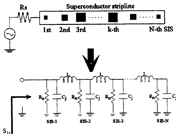
Figure 8: Equivalent circuit of SIS Distributed Junction Array
