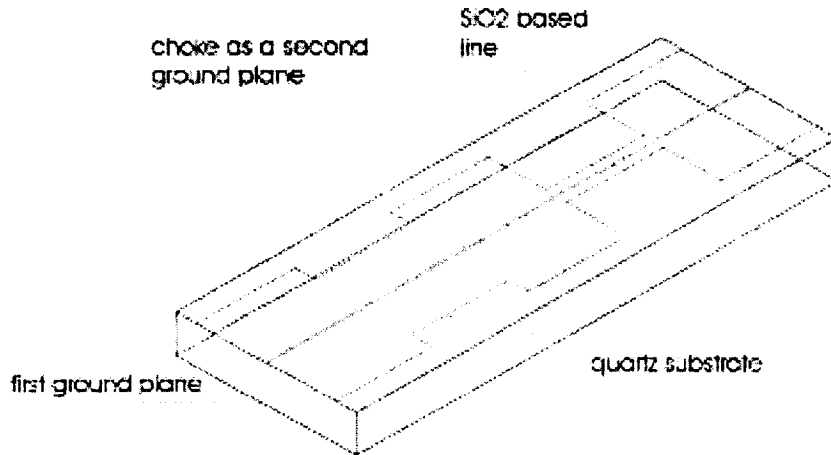
Figure 7 Choke structure on top of the quartz substrate and a line separated by a thin SiO 2 layer (not visible in the picture).
