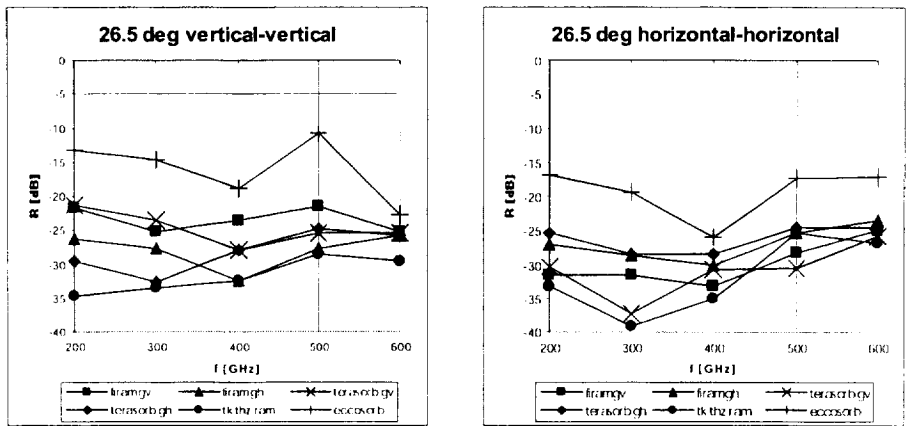
Figure 4. Measured reflectivities for \theta_i = 26.5 degrees.
