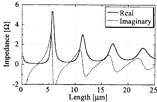
Fig. 1 Calculated real and imaginary parts of the input impedance of a 1.4 μm wide open-ended SIS transmission line. Note that around integer multiples of \lambda_g/2 (6 μm in this case), the reactance vanishes and the resistive part becomes larger.
