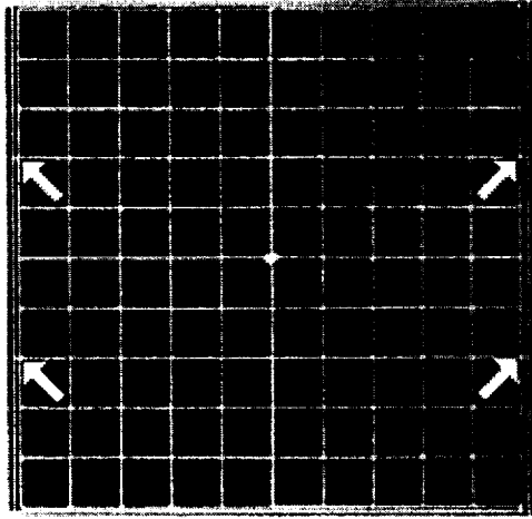
Figure 1 : Prototype single pixel for the filled array design. The absorbing grid is a silicon nitride mesh 1.5 mm on a side. The nitride grid is suspended at four points (arrows) where it is attached to tensioned nitride beams along the left and right sides of the grid. The electrical leads are supported by the nitride beams along the top and bottom of the grid. The leads make contact to the superconducting thermistor on the small patch of nitride at the center of the grid.
