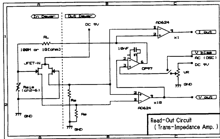
Figure 3: Read-out circuit
