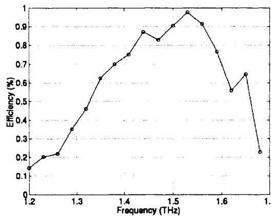
Figure 5. 1.5 THz doubler predicted efficiency vs. frequency at 2 mW input.
