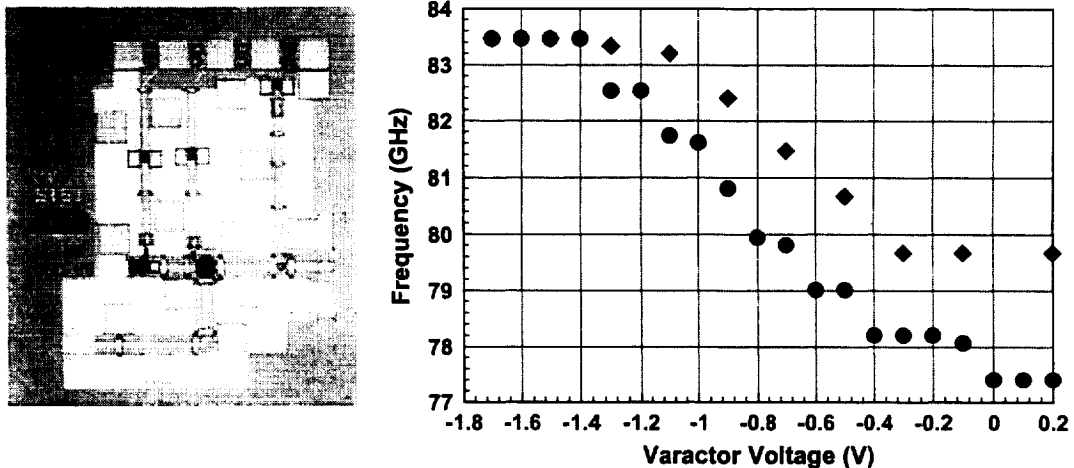
Figure 1. At left, the chip photograph of the 80 GHz VCO is shown. At right, the frequency tuning capability as a function of varactor control voltage is shown. The diamonds and circles represent two stable operating conditions of the VCO, depending on the direction of turning on the varactor voltage.
