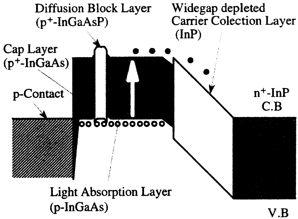
Fig. 1 Schematic energy band diagram of a UTC-PD.
