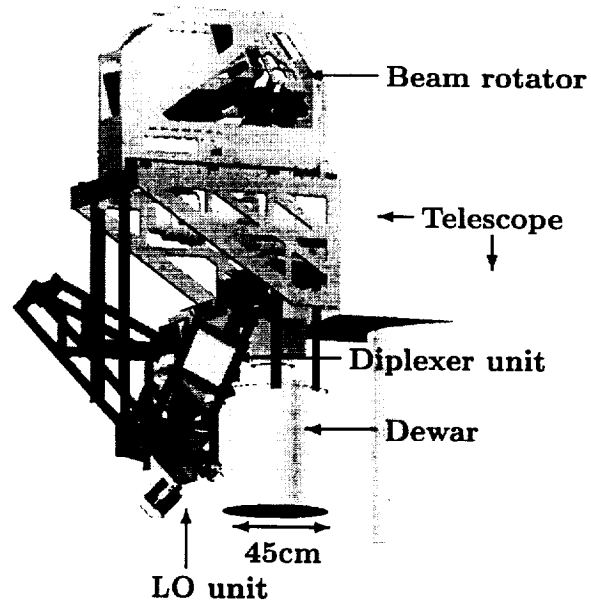
Figure 3. KOSMA Array Receiver 1
