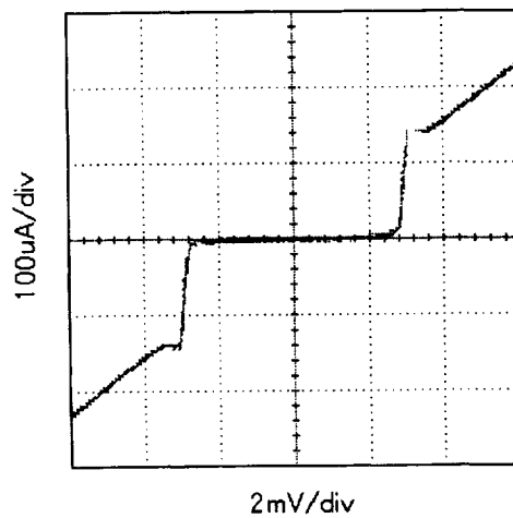
Figure 4: Bias-voltage vs. Leakage-current characteristic
