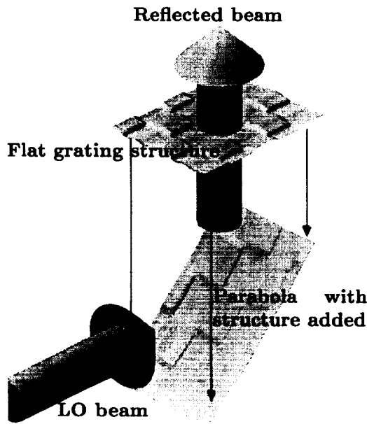
Figure 5. Calculating the grating structure
