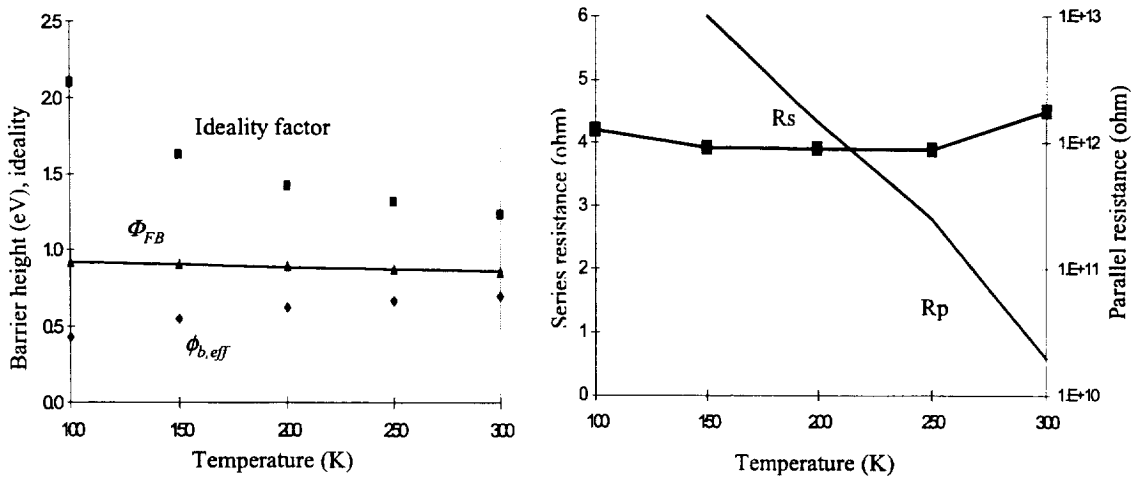
Figure 6. Characteristics of 3e17 diode. (a) Barrier height and ideality. The solid line is a model \Phi_{FB} = 0.95 - 0.0003T \text{ eV} . (b) Series and shunt resistances.
