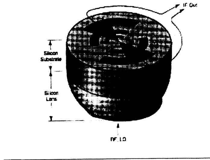
Figure 2. The logperiodic antenna coupled to the silicon lens
