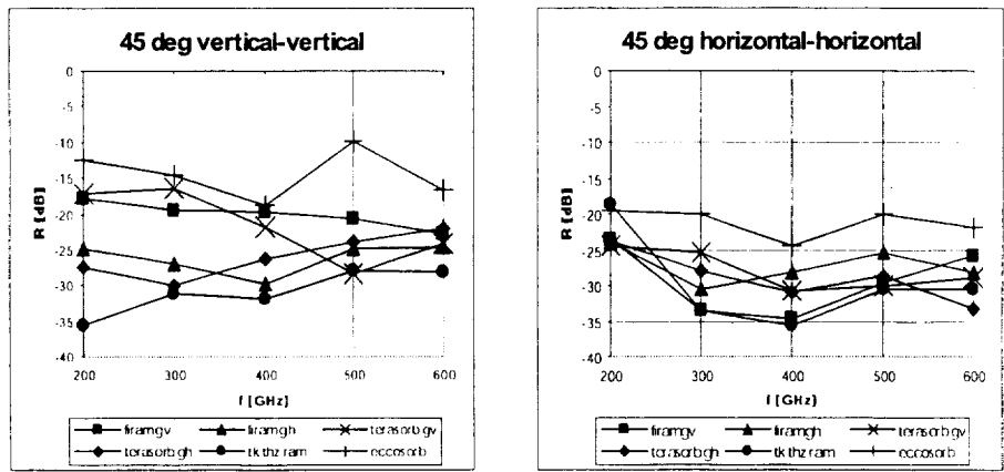
Figure 5. Measured reflectivities for \theta_i = 45 degrees.
