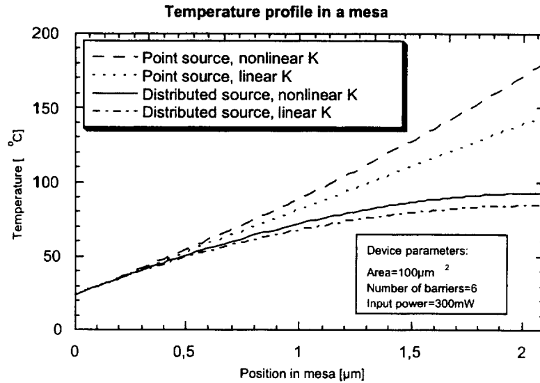
Figure 4) Comparison of thermal models.
