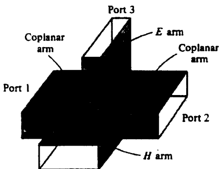
Figure 4: Schematic of magic tee structure (Rizzi, 1988).
