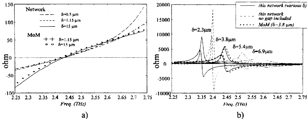
Fig. 9 Impedance of a delta gap excited microstrip as function of the frequency. a) ( l=60 \mu\text{m} ); b) ( l=40\mu\text{m} ). Also a parametric study as a function of \delta and comparison with MoM are shown. The width of the microstrip and the thickness of the dielectric are 2.5 \mu\text{m} and 3 \mu\text{m} respectively. The grounded dielectric is made of Ga-As.
