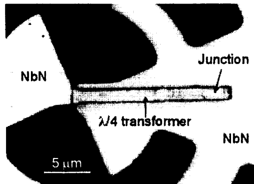
Fig. 1. Optical micrograph of the mixer. A rectangular NbN/AlN/NbN tunnel junction, as a distributed element, and a \lambda/4 NbN/MgO/NbN microstrip-impedance transformer were integrated with a self-complementary NbN log-periodic antenna.
