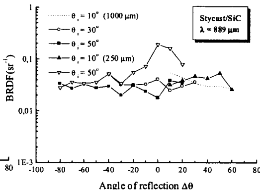
Fig. 18 BRDF of Stycast/SiC at 889 \mu\text{m}
