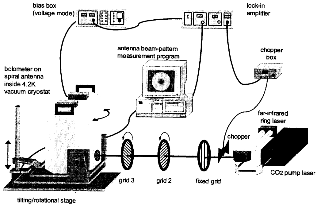
Figure 3. Schematic drawing of the measurement setup. Three submillimeter sources are used for the measurement of polarization and far-field beam pattern, i.e. a BWO at 0.6 THz, a carcinotron + tripler at 1.4 THz, and a CO2 pumped FIR laser at 2.5 THz. Only the laser is shown here.
