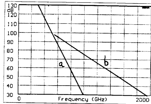
Fig.4. Dynamic range, MVNA-8-350 with extensions. In a): observed with a single pair of extensions (source ESA-1-FC, detection ESA-2-FC) covering continuously the interval 250-1000 GHz. In b): extrapolated from available powers from different multiplication chains, all detected with the single extension ESA-2-FC.
