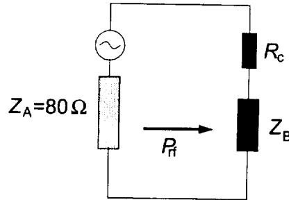
Figure 5: RF circuit model of the antenna integrated bolometer with contact resistance.
