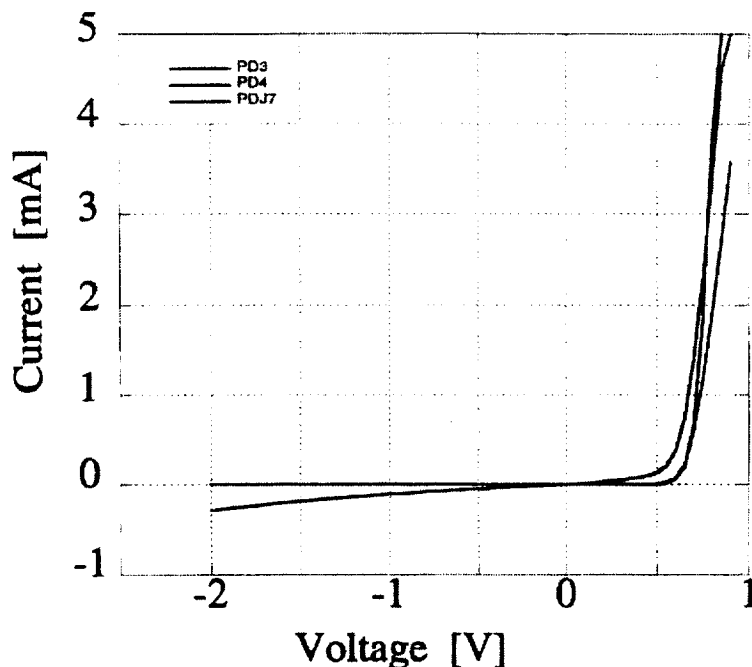
Fig. 6 DC I-V curves of UTC-PD's .
