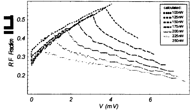
Fig. 6 Fraction of RF power absorbed in the active zone(s) LO heating powers ranging from 100nW to 250nW in steps of 25nW for device M2-1. The calculated points correspond to the points from Fig.4 and 5.
