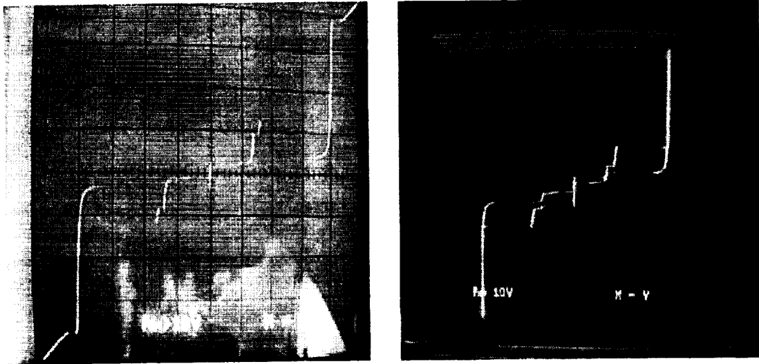
Fig. 7 I-V curves of the twin junctions (a: with a design tuning inductance; b: with a 30% shorter one; 0.677mV/div)
