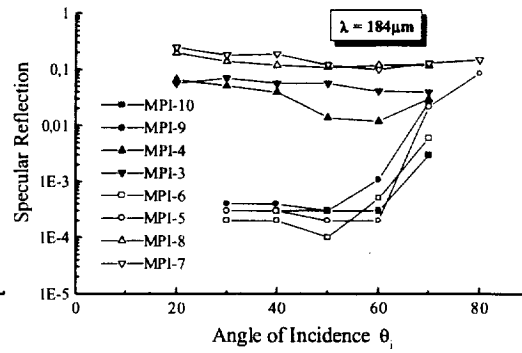
Fig. 8 Specular reflection MPI
