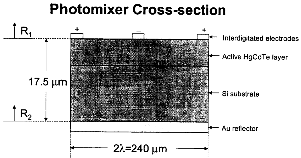
Figure 4: RCE Device Structure
