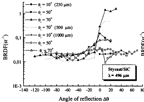
Fig. 17 BRDF of Stycast/SiC samples at 496 \mu\text{m}
