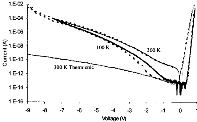
Figure 5. Tunneling/avalanche current calculations compared with measurement. The solid lines are measured currents, broken lines are calculated.
