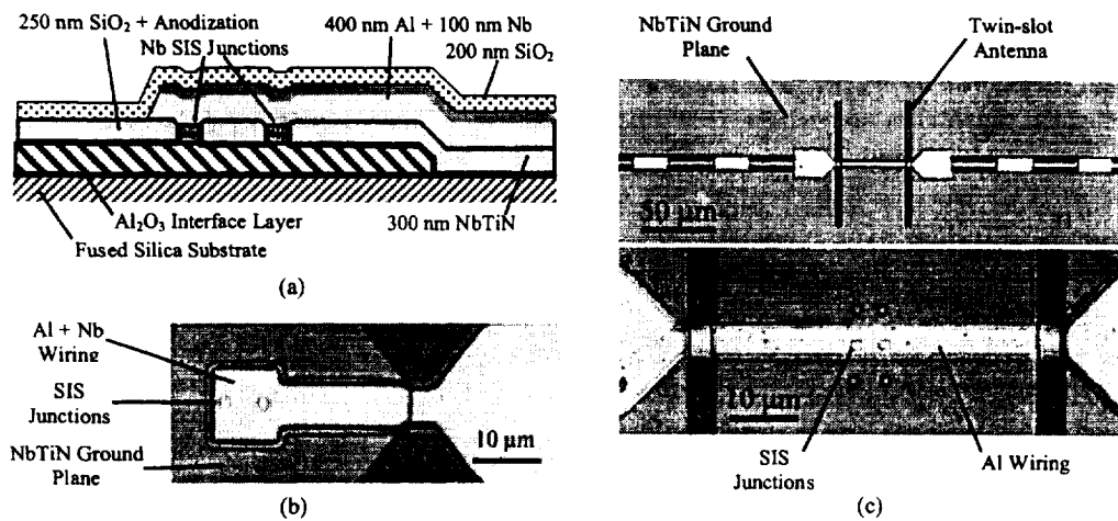
Figure 1. (a) cross-section of the NbTiN/SiO 2 /Al tuning circuit (modified from [16]), (b) microscope image of the waveguide device geometry used here (modified from [16]), and (c) microscope images of the quasi-optical device geometry used here (modified from [10]).
