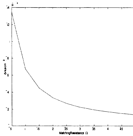
Figure 6: Small Signal Device Area J_{DC} = 1000 A/cm^2
