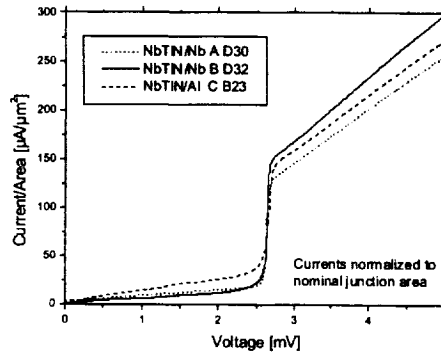
Fig. 6 Comparison between the unpumped IV curves scaled to the nominal junction areas of different batches
