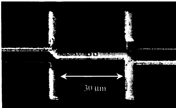
Fig. 2 Photograph of the double-dipole antenna SIS mixer fabricated on silicon substrate. The light metal strips are Al wiring; the darker ones are NbTiN strips at the bottom.
