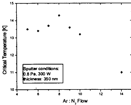
Fig. 1a T c versus Ar/N 2 flow
