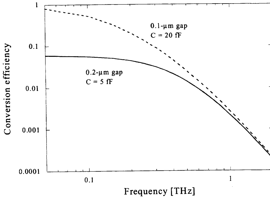
Fig. 3: The conversion efficiency of the photomixer receiver. The solid and dashed curves represent the estimation for the self-complementary broadband antenna ( R_A=72 \Omega ) device with 0.2- \mu\text{m} and 0.1- \mu\text{m} gap electrodes, respectively.
