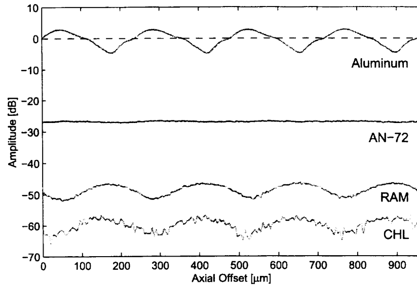
Figure 9: Reflection measurements at 625 GHz of the CHL and other absorbing materials at different axial offsets.
