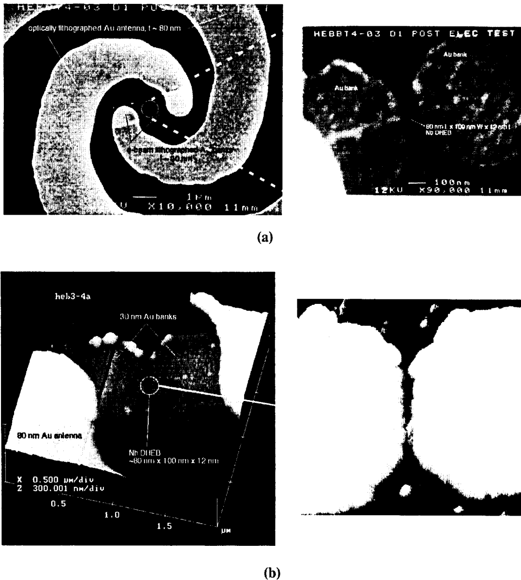
FIG.5. (a) SEM pictures of the DHEB, (b) AFM pictures of the DHEB.
