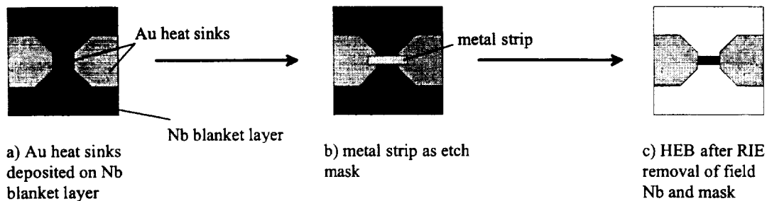
Fig. 2: Outline of self-aligned fabrication process (top view)
