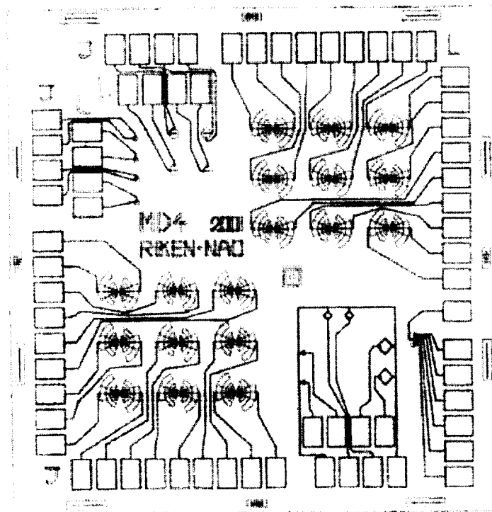
Figure 11: Mask design for 3x3 array
