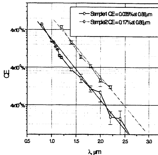
Fig. 7. Spectral dependence of quantum efficiency (meander-type devices).
