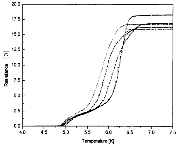
Fig. 5 : RT-characteristics of similar-sized HEBs on one wafer ( \varnothing 22 mm), nominal device dimensions: 240 \times 200 \times 14 \text{ nm}^3 , R_{\text{sheet}} = 14 - 15 \Omega . The spread in the R/T curves is probably due to small size variations of the bolometers.
