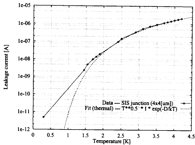
Figure 6: Temperature vs. Leakage-current characteristic
