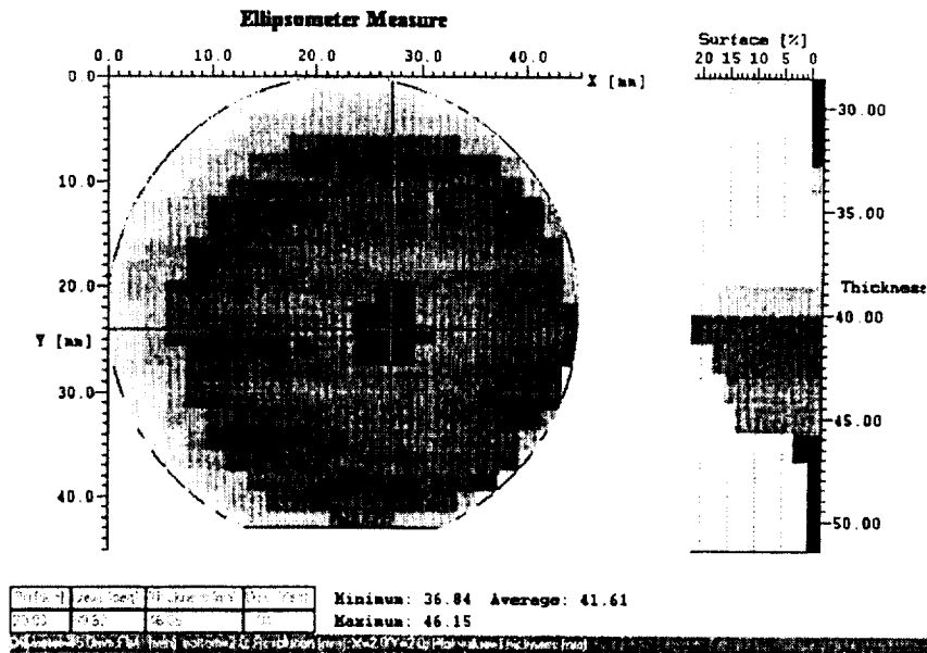
Fig.2.1.: MgO film thickness control by ellipsometry. Mapping of the hole 2" Si wafer.
