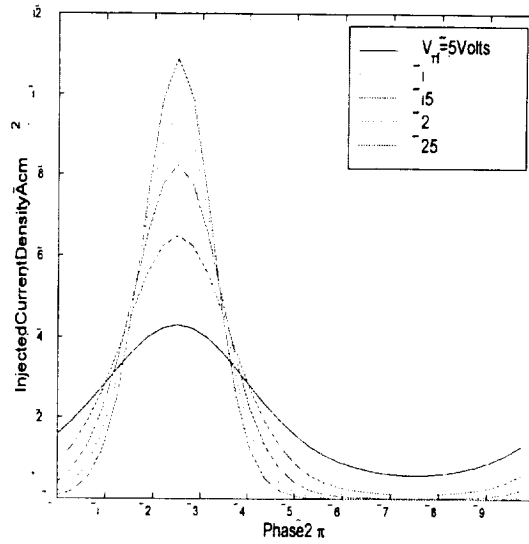
Figure 3: Example Injected Current Waveform
