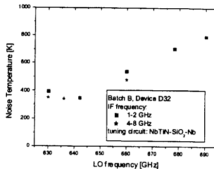
Fig. 10 Results with different IF frequencies
