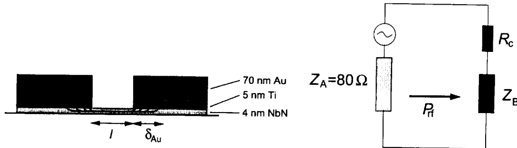
Figure 5: RF circuit model of the antenna integrated bolometer with contact resistance.
