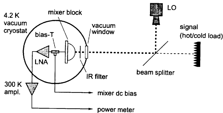
Figure 1: Schematics of the measurement set-up. The radiation coupling optics consists of “hot” (beam splitter, vacuum window) and “cold” (IR filter, lens + antenna) parts.
