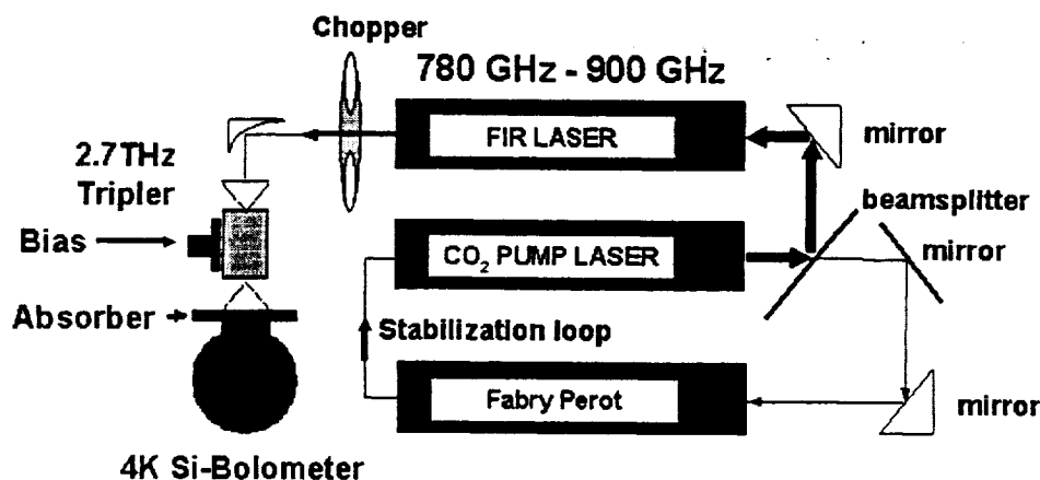
Fig. 7: FIR laser tripler test setup.
