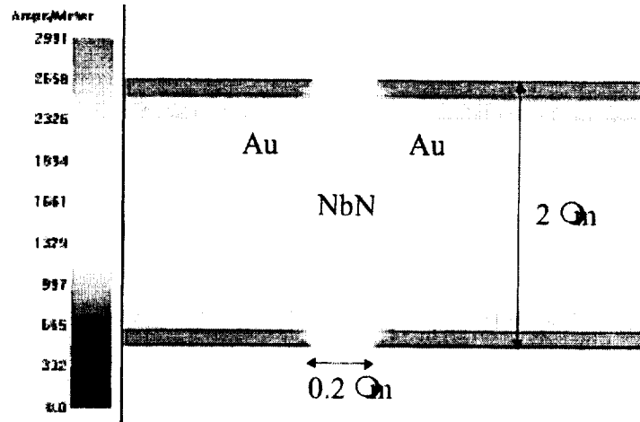
Figure 8. RF current distribution simulated by Sonnet ® .
