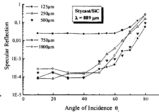
Fig. 14. Specular reflection at 889 \mu\text{m}
