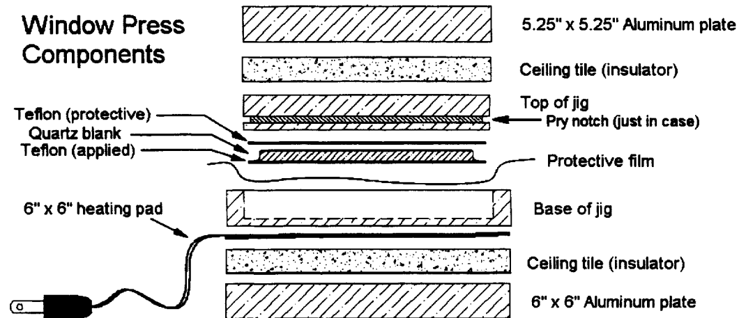
Figure 8. Components of the window press, in cross-section.
