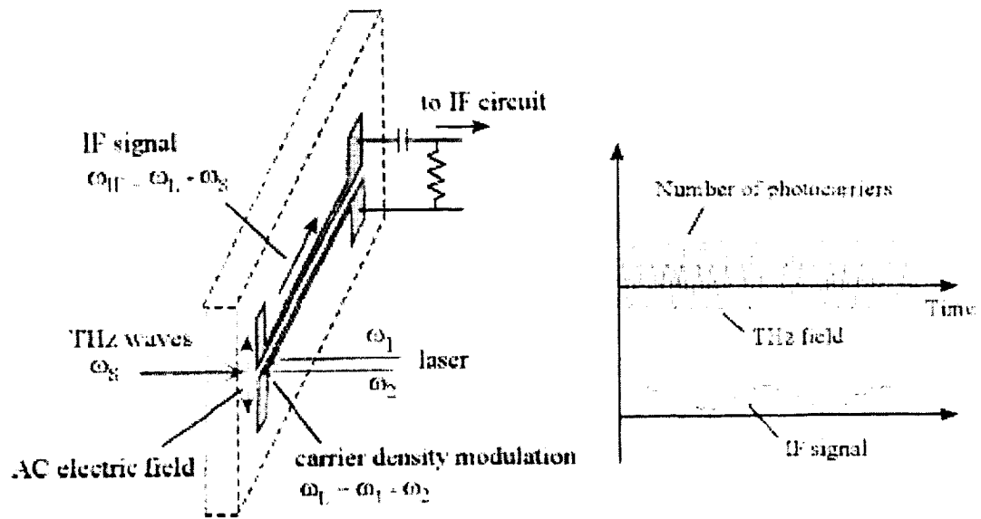
Fig. 2: The principle of the photomixer receiver.
