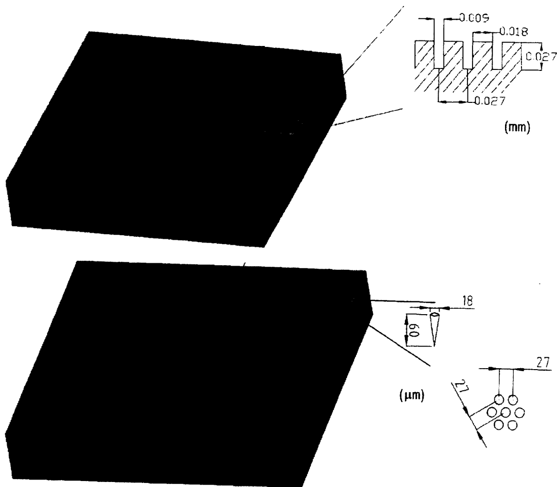
Figure 10: Conceptual 3D rendering of 1.5 THz AR matching layers in silicon. 10-a (top) Using concentric rectangular grooves. 10-b (bottom) Using conical holes.
