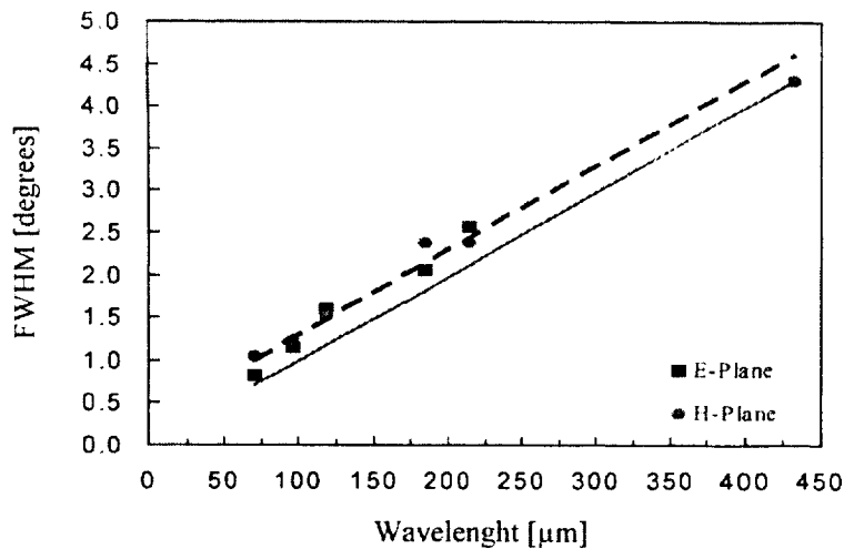
Fig. 4: FWHM as a function of the wavelength. The solid line represents the diffraction limit as given by the diameter of the lens while the dashed line is a linear fit to the measured FWHM.
