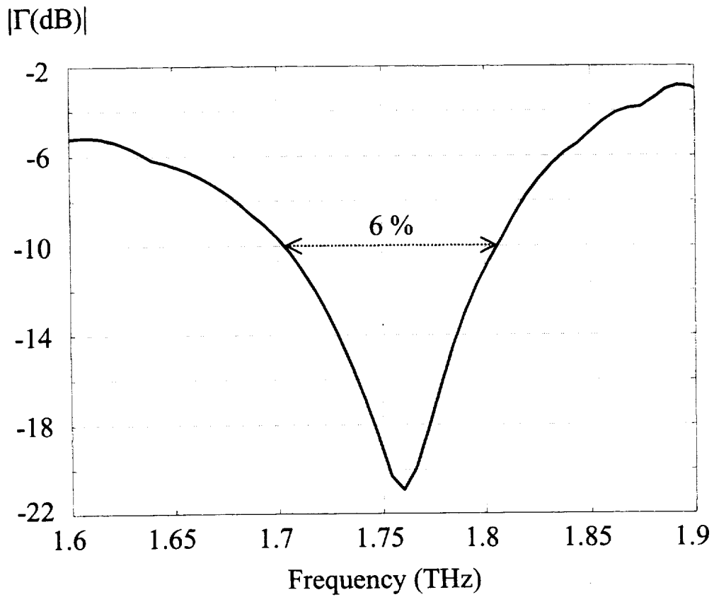
Fig. 4 Reflection Coefficient for a double slot antenna
