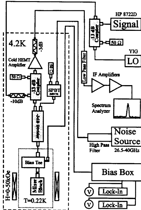
Figure 2: Measurement Setup
