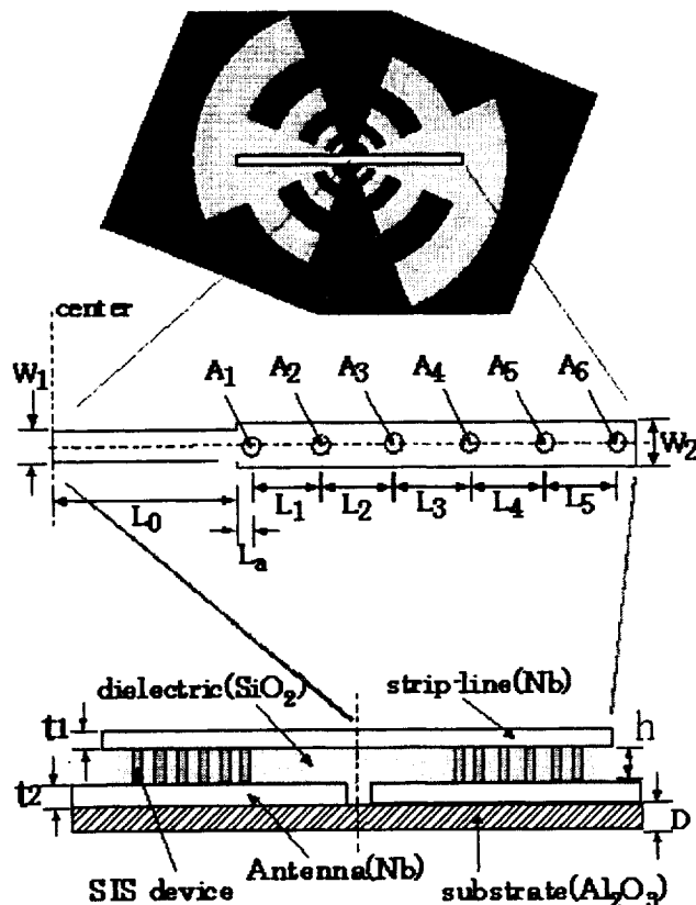
Figure 10: Design of superconducting direct detectors
