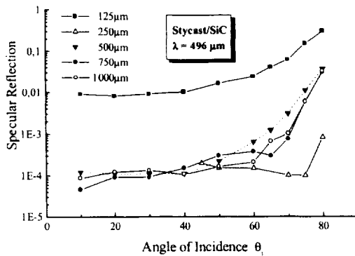
Fig. 13 Specular reflection at 496 \mu\text{m}
