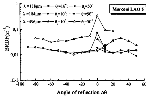
Figure 4. BRDF of LAO 5
