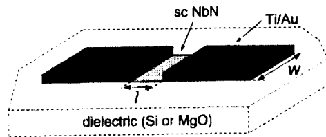
Figure 2: Schematics of the bolometer. The NbN strip with, is contacted by normal metal pads made of 5 nm Ti + 70 nm Au. The width w and length l are of the order \mu\text{m} .
