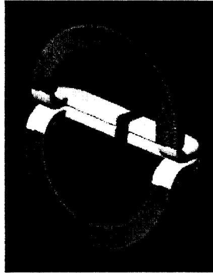
Figure 8. One half of the cryoperm electromagnet designed for Band 1 (1100 turns); artist's view.
