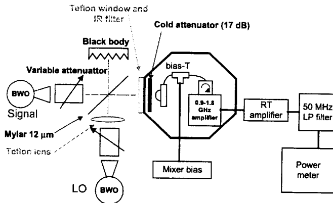
Fig. 2 Experimental set-up used for saturation measurements of HEB mixers. For the receiver noise temperature measurements, the cold attenuator in the cryostat was removed, signal BWO was replaced by 300K/77K black body.
