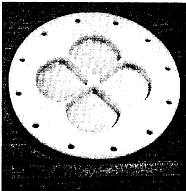
Figure 6: HDPE vacuum window for PoleStar.
