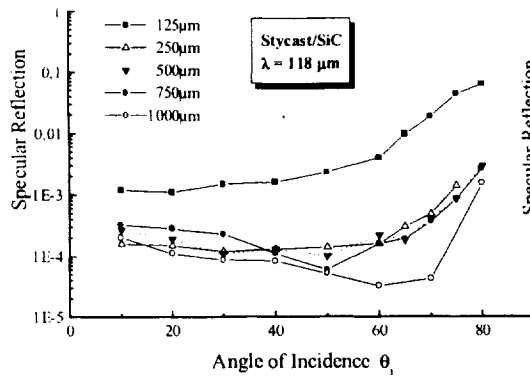
Fig. 11 Specular reflection at 118 \mu\text{m}
