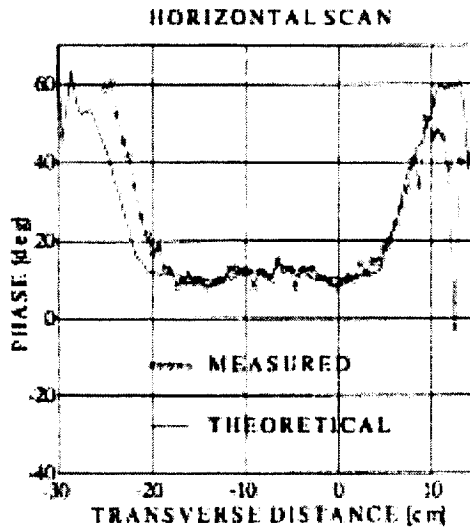
Figure 4. Measured and theoretical phases in horizontal direction.
