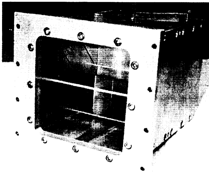
Figure 4: PoleStar's quasioptical LO power splitter.
