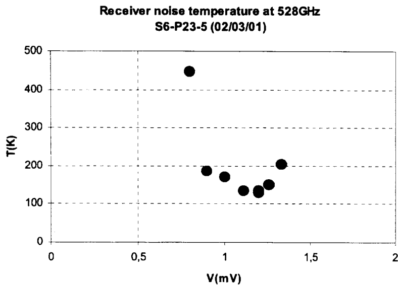
Figure 7. Measured receiver noise temperature versus bias voltage at 528 GHz for device # S6-P23-5 ( 15 \text{ kA/cm}^2 ).
