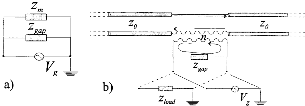
Fig. 5 Equivalent network for \delta gap excited microstrip structure. a) admittance decomposition ( y_{inf} = y_{gap} + y_m ); b) Interpretation of the modal impedance interms of transformer connected equivalent transmission line.
