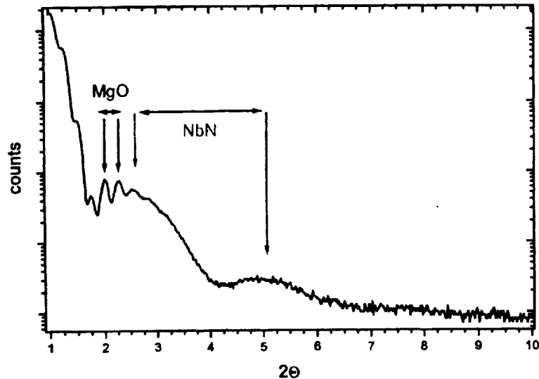
x-ray reflectometry, NbN/MgO bilayer on crystalline quartz substrate
