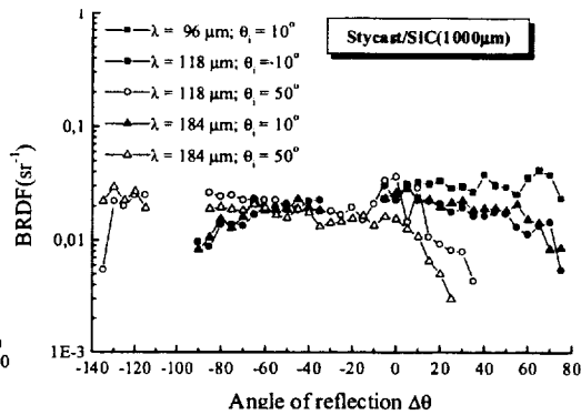
Fig. 16. BRDF of 1000 \mu\text{m} sample at 3 wavelengths
