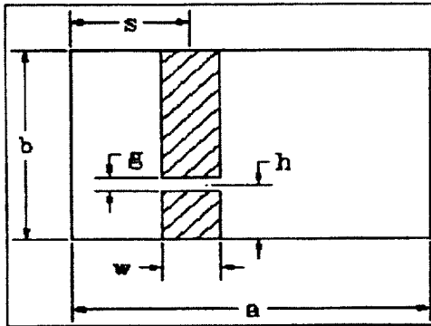
Figure 21: Waveguide/post physical model. a and b are the dimensions of the waveguide (160 x 40 μm); s is the distance from the waveguide wall to the diode post (80 μm); g is the gap between the waveguide post and the end of the wide section of the whisker (10 μm); and h is the height of the diode mounting post – ½ g (0.4 μm), and w is the width of the post and whisker end section just prior to the narrowed contact area (taken to be 40 μm in this model for improved performance at higher frequencies).
