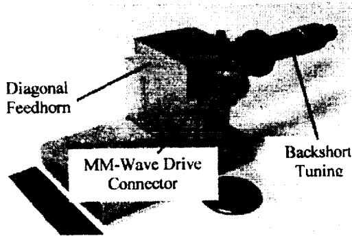
Figure 4: Photograph of the SBG mixer block.
