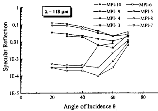
Fig. 7 Specular reflection of MPI coatings
