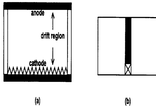
Figure 1: BT^3D (a) Structure (b) Waveguide Mount
