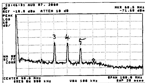
Fig.1. Vertically : 10dB/div. Horizontally : 10 MHz/div, Span 0-100 MHz. Signal detected by the SIMUHAE with a Gunn at 103 GHz feeding a single-Schottky multi-harmonic multiplier with a F > 285 GHz high-pass filter at its output. The successive harmonics M=3-4-5 , observed at 30- 40-50 MHz, correspond to the microwaves at 309-412-515 GHz.
