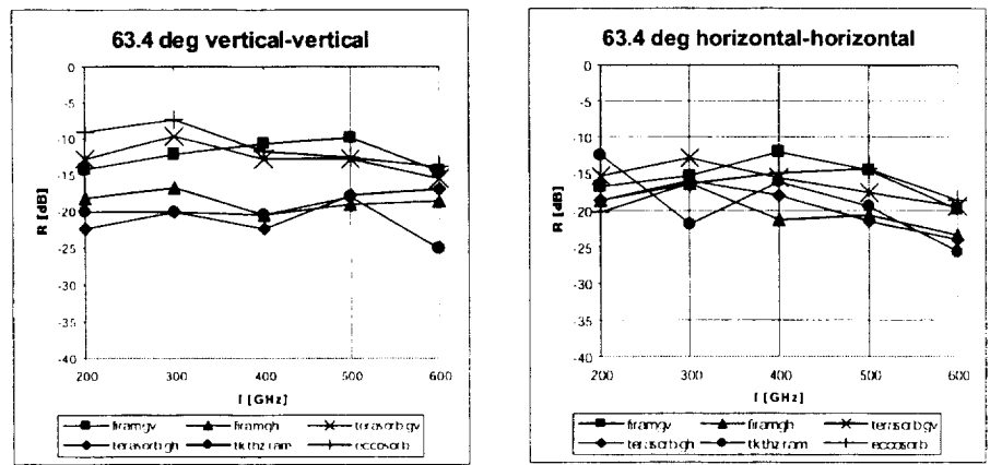
Figure 6. Measured reflectivities for \theta_i = 63.4 degrees.
