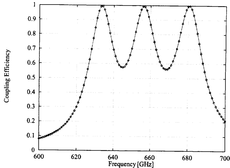
Figure 9: Coupling efficiency of SIS Distributed Junction Array
