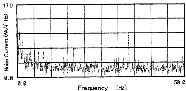
Figure 7: Noise Characteristic
