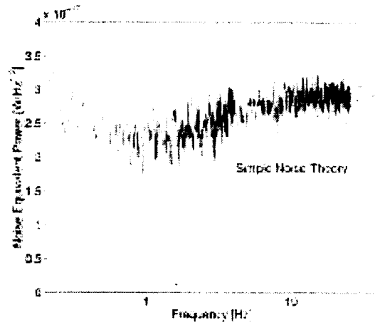
Figure 2 : Measured noise equivalent power for prototype bolometer
