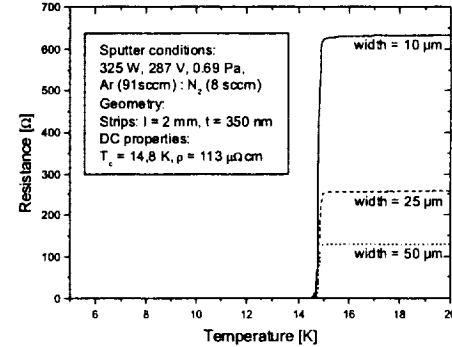
Fig. 2: Typical R-T curves of NbTiN test structures
