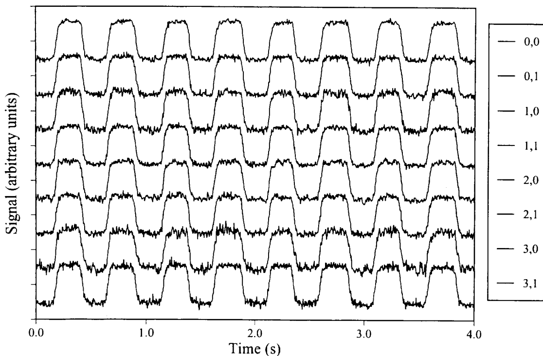
Figure 9. Multiplexed detection of 8 detectors viewing a chopped hot/cold load, read out simultaneously and demultiplexed on-the-fly.
