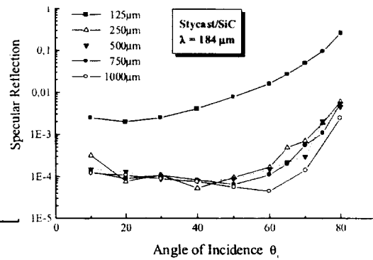
Fig. 12 Specular reflection at 184 \mu\text{m}
