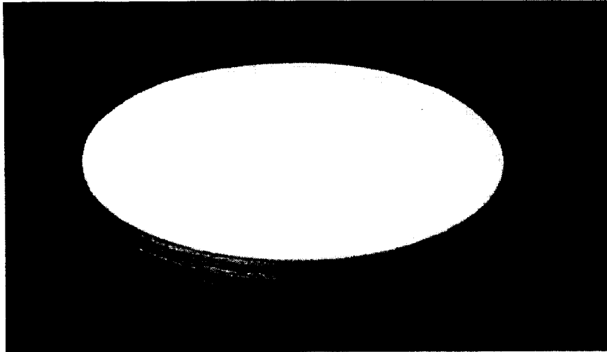
Figure 10. A nearly completed 4.5" diameter, three-layer window for the VLBA. The outer surfaces are PTFE, which has not yet been trimmed for the o-ring seal.
