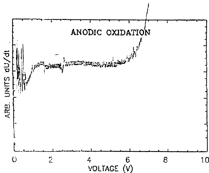
Fig.2.2.: NbN film thickness control by anodization. The plot shows the curve of a ~5 nm NbN thin film.
