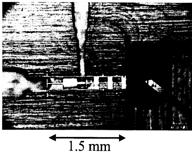
Figure 5: Inside of the 400 GHz balanced doubler with the top half of the split block removed. The output guide is shown in the top half of the photograph. The chips are made with the substrateless technology that requires only a simple assembly process.
