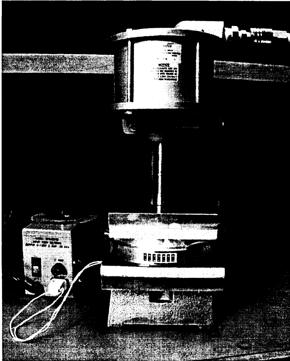
Figure 9. Photograph of the assembled window press. The Variac and heating pad are used to increase the temperature of the jig and so decrease the curing time of the epoxy. Note the thin film thermometer on the lower half of the jig.
