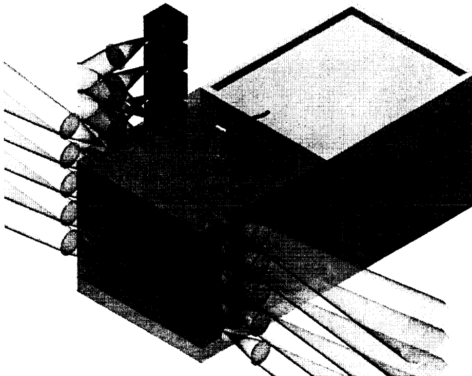
Figure 6: Conceptual 3D rendering of an interferometric array proposed for the Large Binocular Telescope (LBT). The split block uses laser micro machined feedhorns and magic tees to coherently combine the beams from two telescopes. A directional coupler is used to inject LO power.
