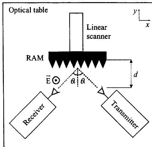
Figure 1. Schematic drawing of the test instrumentation.
