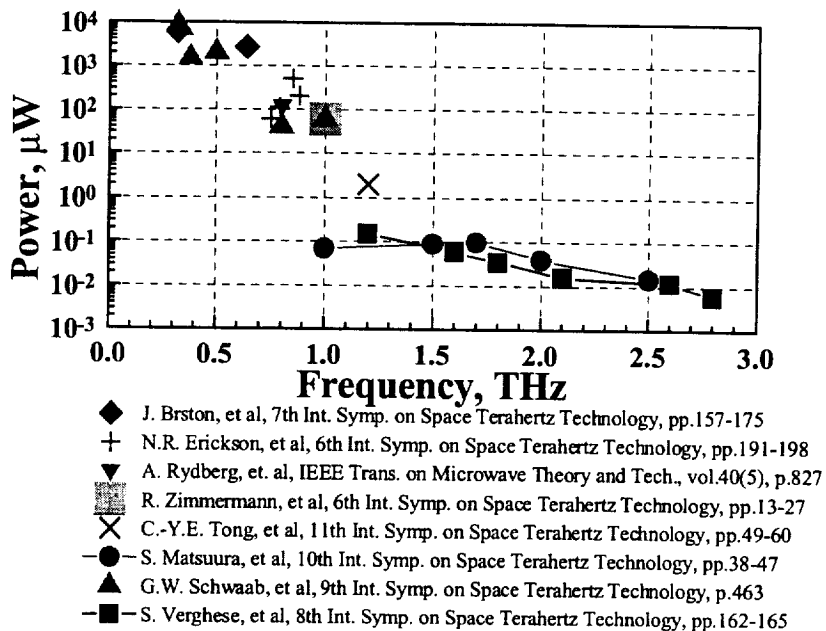
Fig. 1 Output power available from local oscillator sources reported in press.
