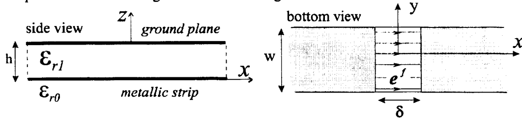
Fig.1 Infinitely extended microstrip excited with by an impressed electric field distributed over a gap of dimensions (\delta, w) .
