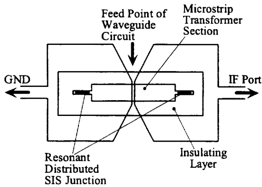
Fig. 2 Layout of the resonant SIS mixer chips.
