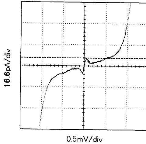
Figure 5: Bias-voltage vs. Leakage-current characteristic (magnified)
