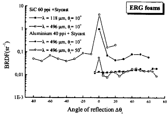
Fig. 19 BRDF of Stycast coated foams
