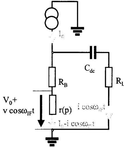
Fig. 3: Small signal circuit for the active zone mode: The heating power sensitive active zone resistor r(\rho) is in series with the resistance of the passive rest of the HEB R_B . The HEB is in parallel with a load resistance R_L . The bias current is I_0 .
