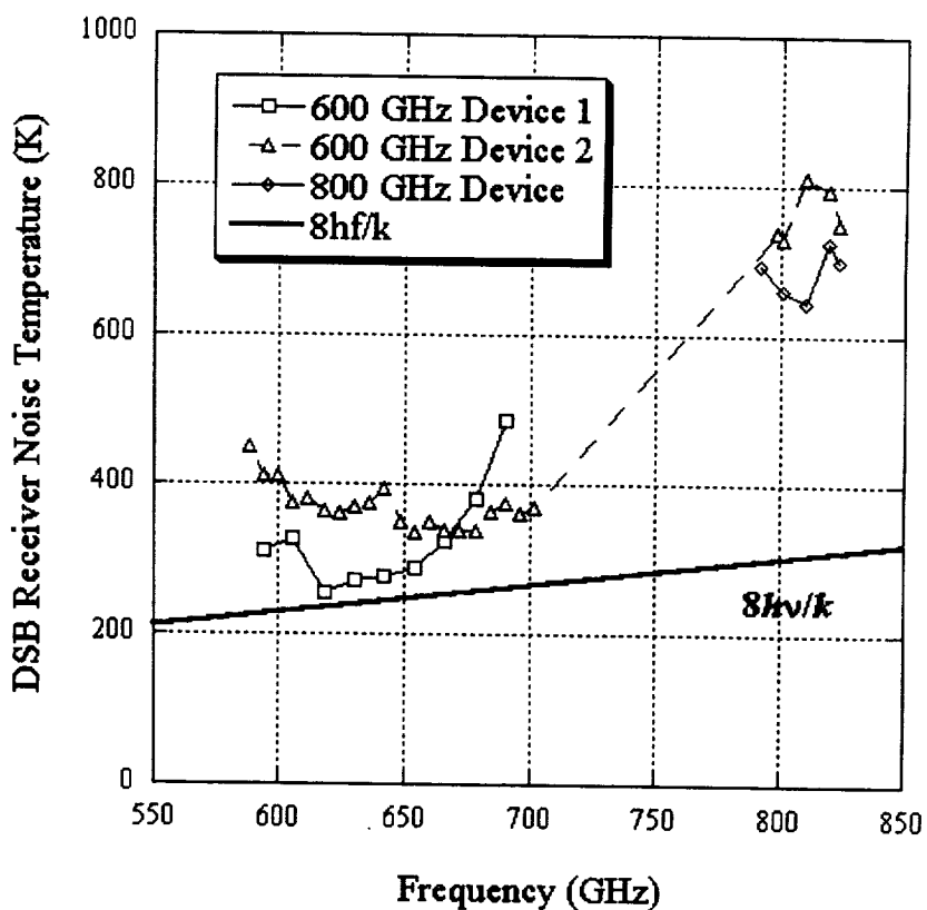
Fig. 5 Double-side-band receiver noise temperature measured for two 600 GHz and one 800 GHz NbTiN mixer chips.
