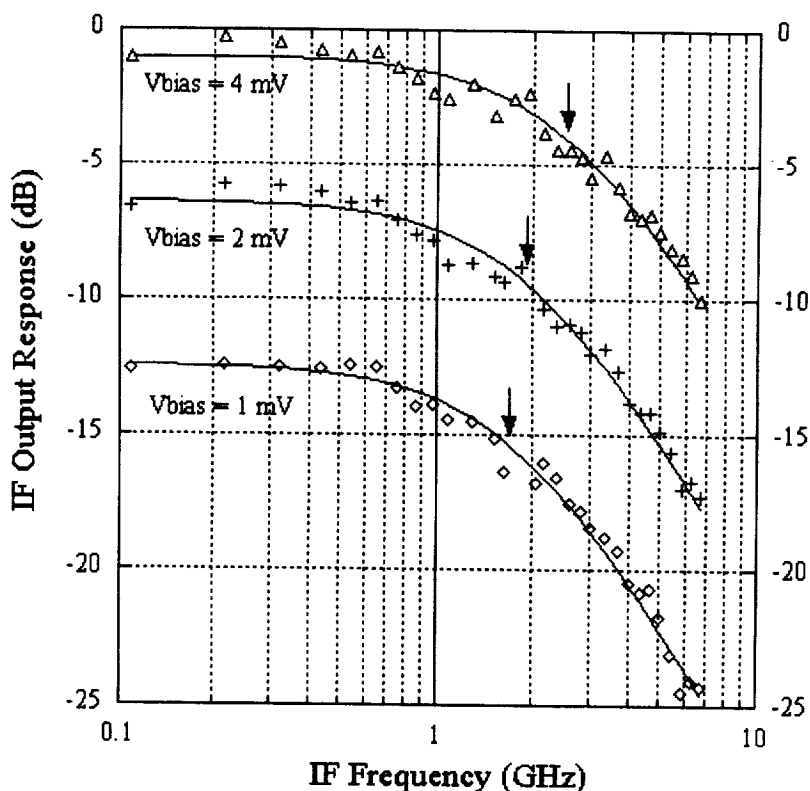
Fig. 3 IF Gain Bandwidth measurement of NbTiN HEB mixers operating at around 600 GHz. The solid curves are the best fit single pole roll-off response for each bias voltage setting. Note that the curves are shifted vertically relative to each other for display purposes only. The 3-dB rollover frequencies are marked by arrows. The error of the fit is about 0.2 GHz.
