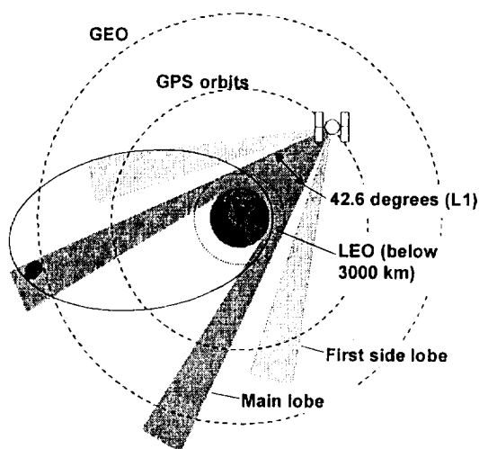
Figure 4-7. Satellite Orbital Geometry With Respect to GPS Signal
