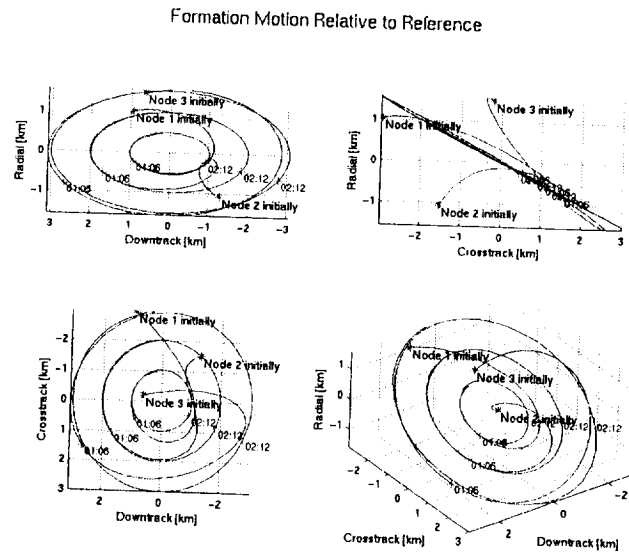
Figure 4-17. Formation Motion Relative to Reference
