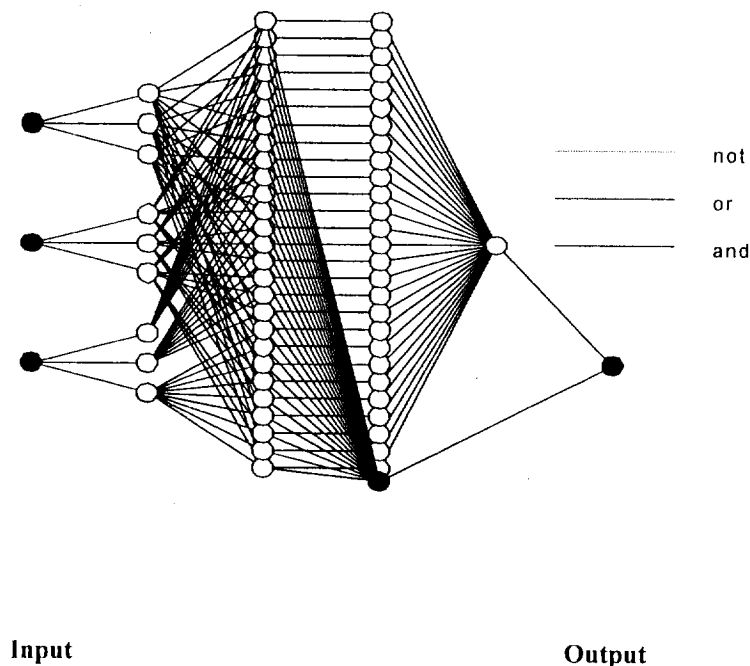
Figure 4-9. Diagram of a Three-Input ANFIS with 27 Rules
