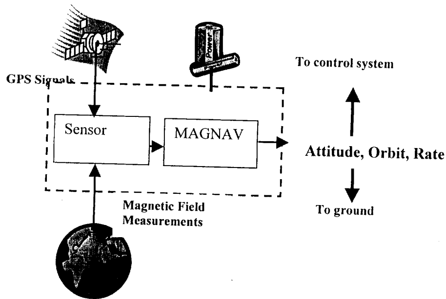
Figure 4-10. High Level Overview of Onboard Operation
