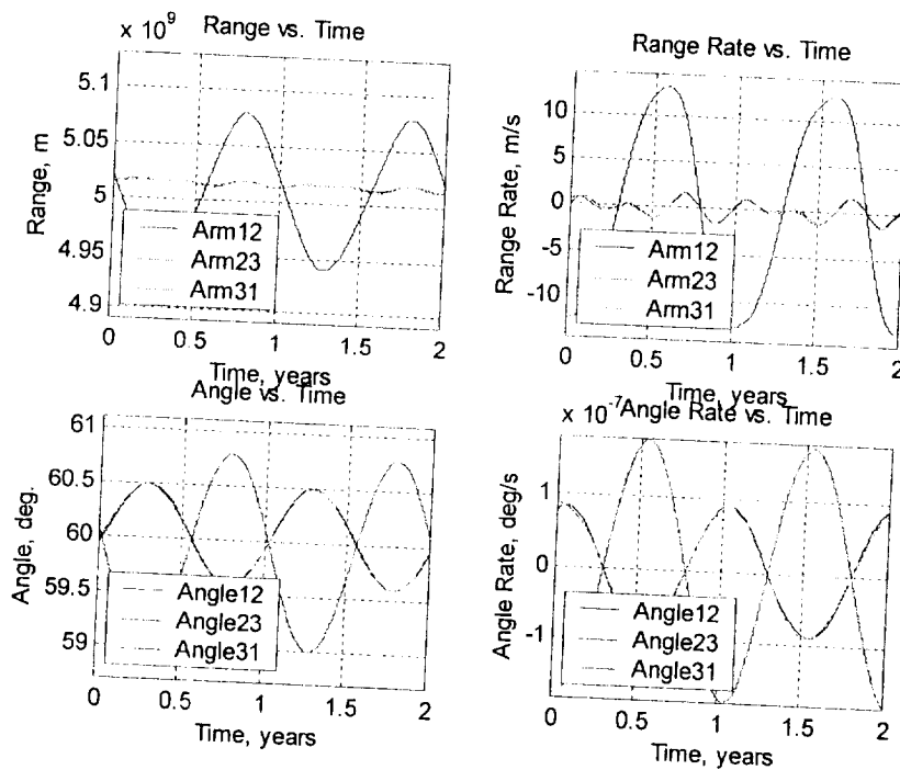
Figure 4-3. Relative Geometry Evolution
