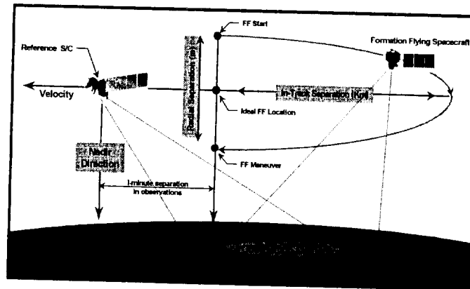
Figure 4.12. Orbit Mechanics of EO-1 Formation Flying
