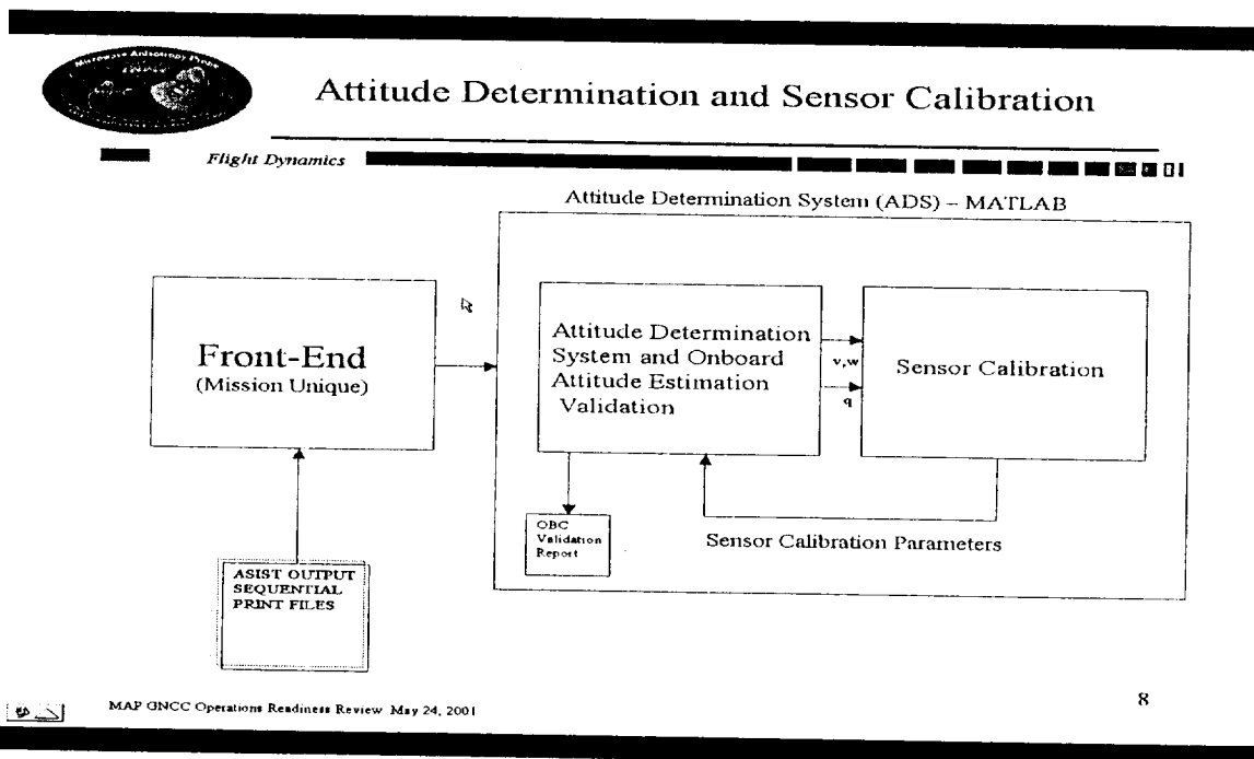
Figure 4-25. ADS-MATLAB Overview
