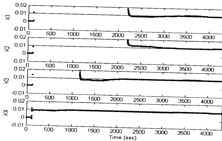
Figure 4-23. AQUA Gyro Scale Factor Estimates (bold) versus Truth (thin)
