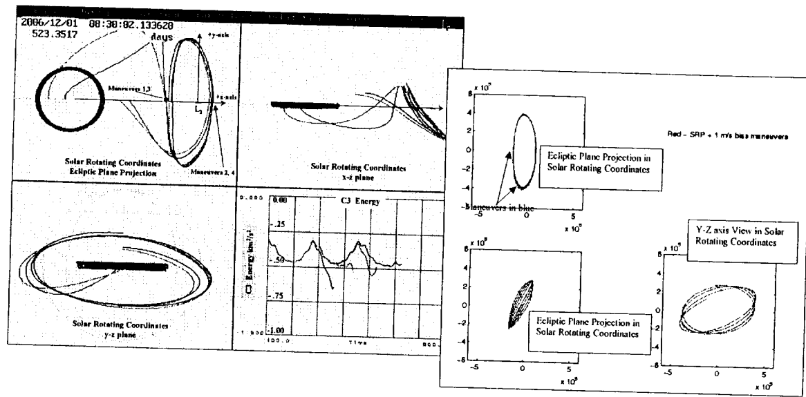
Figure 3-9 NGST Trajectory Planning
