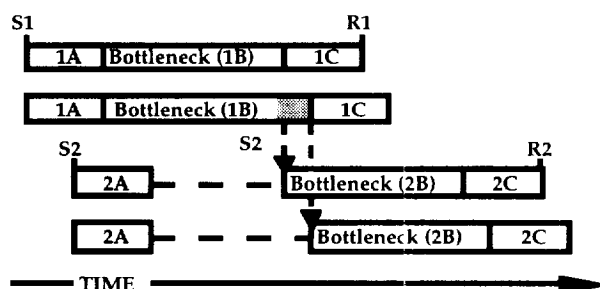
Figure 2. At the short SOA, but not the long SOA, Task 1 difficulty carries-over onto RT2. At the long SOA (top panel), lengthening Task 1 bottleneck processing (shaded 1B) does not affect Task 2 response times because Task 2 processing is independent of Task 1 processing. At the short SOA (bottom panel), lengthening Task 1 bottleneck processing (shaded 1B) lengthens RT2 because Task 2 processing at stage 2B is held up while waiting for bottleneck processing for Task 1 at stage 1B to be completed.
