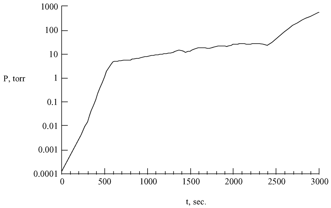
Figure 3. Typical re-entry pressure profile.
