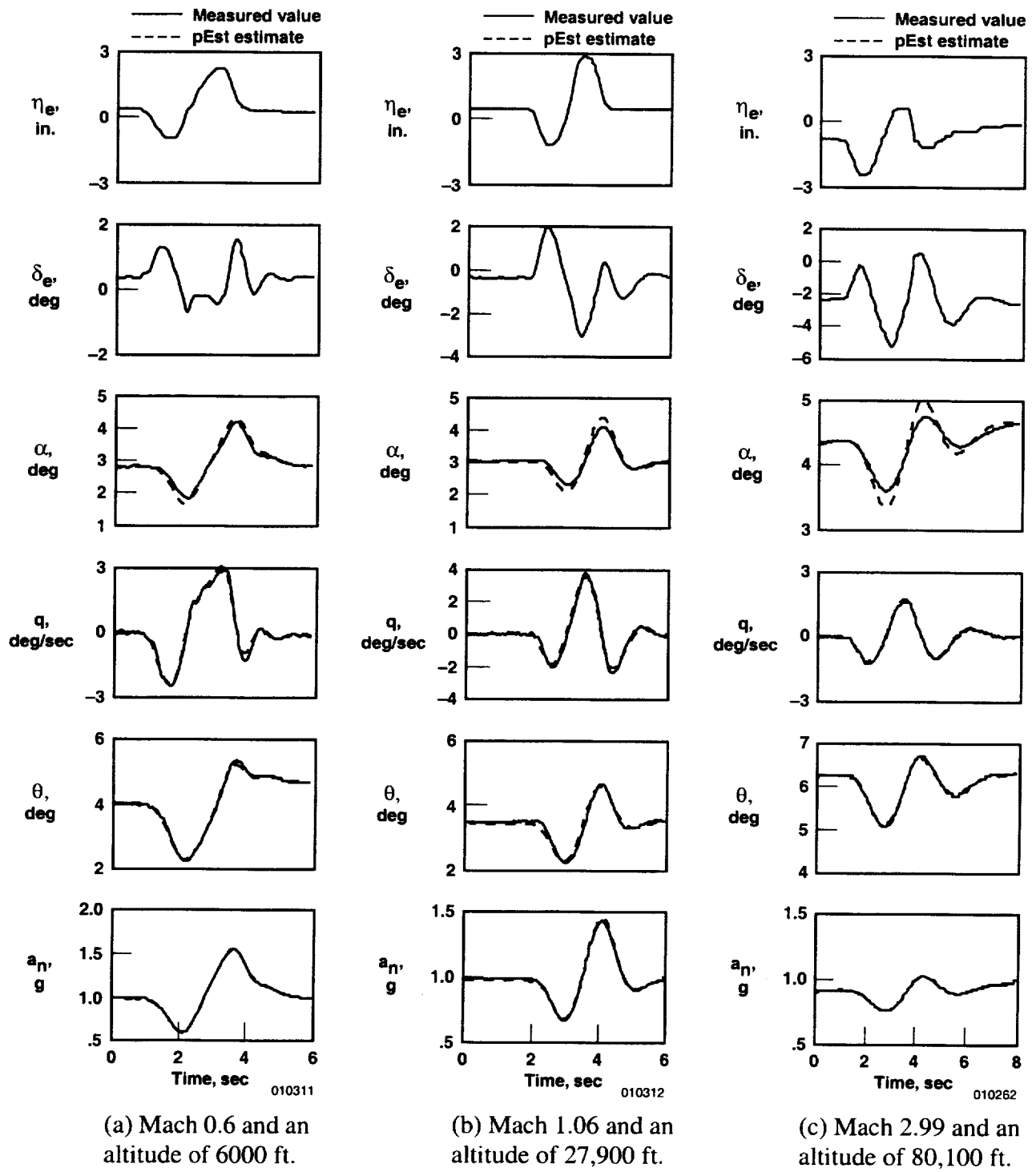
Figure 14. Baseline configuration longitudinal maneuver time histories.
