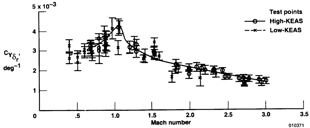
(a) C_{Y_{\delta_r}}
