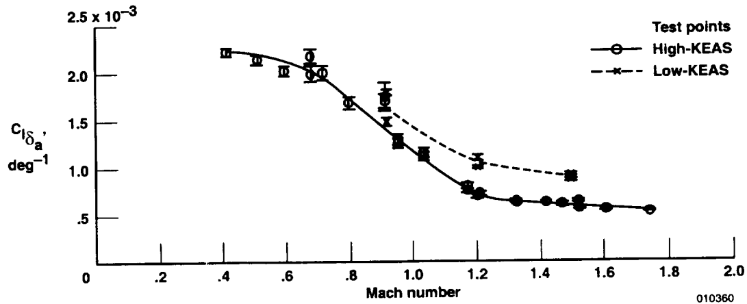
(b) C_{l_{\delta_a}}
