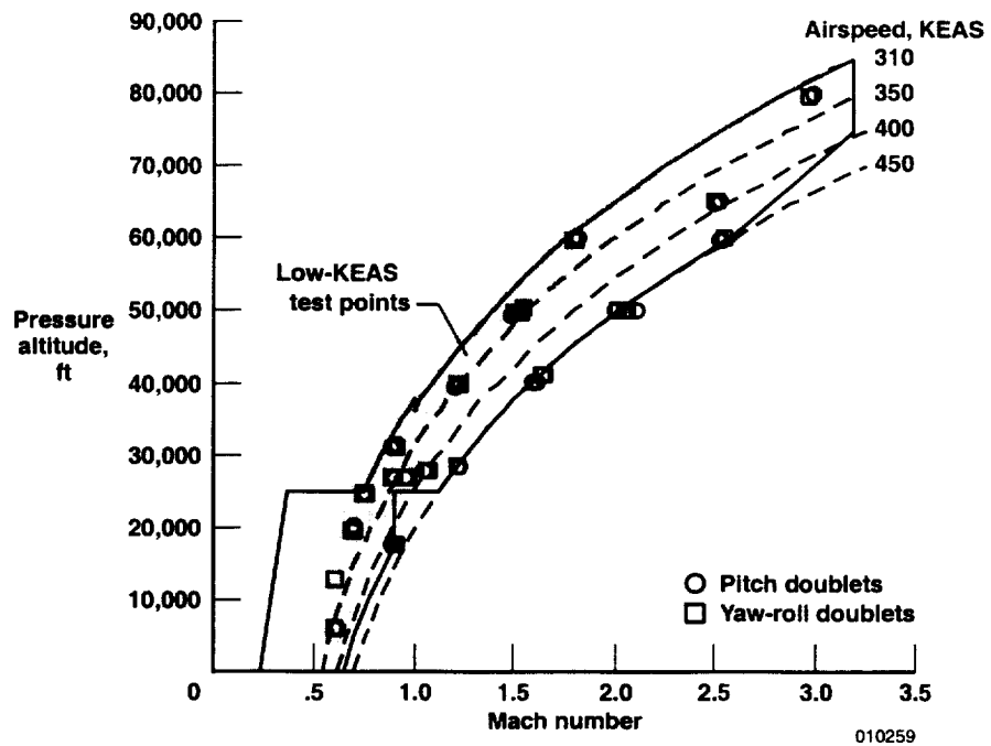
Figure 11. Flight conditions for stability and control test points (baseline configuration).
