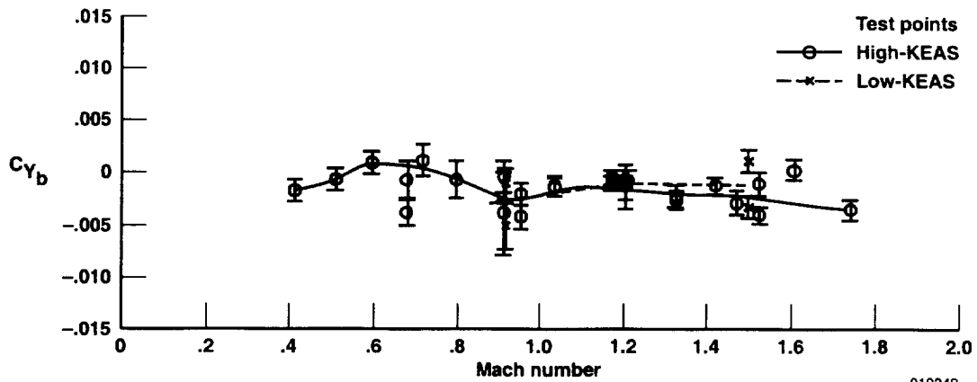
(a) C_{Y_b} .
