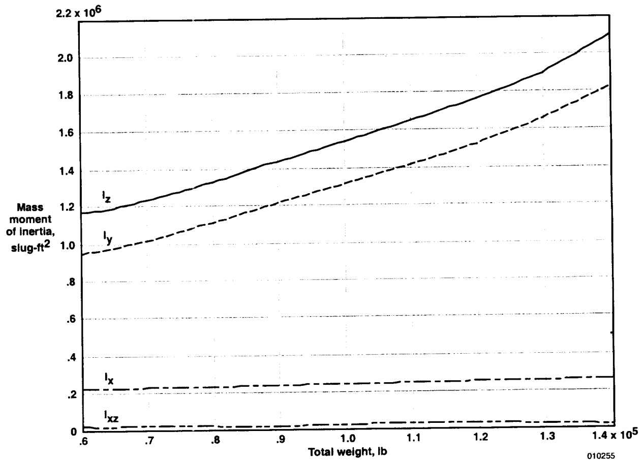
Figure 7. Body-axis mass moments of inertia for the baseline configuration using the standard fuel burn schedule.
