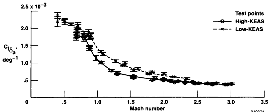
(b) C_{l\delta_a} .
