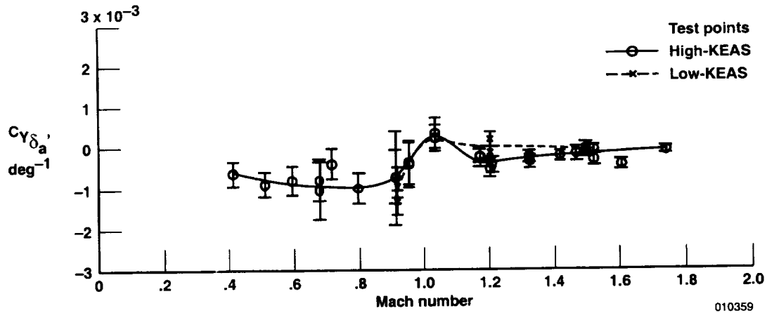
(a) C_{Y_{\delta_a}}
