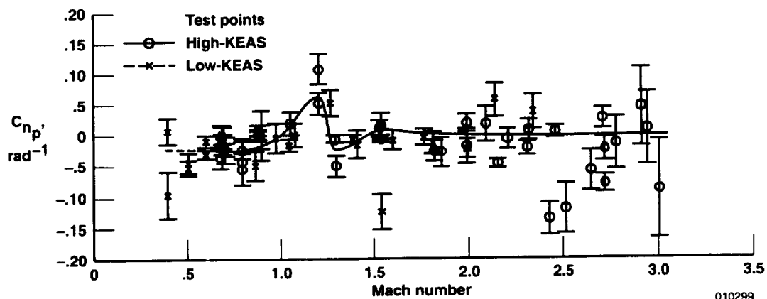
(c) C_{n_p} (moment reference at 0.25 c).
