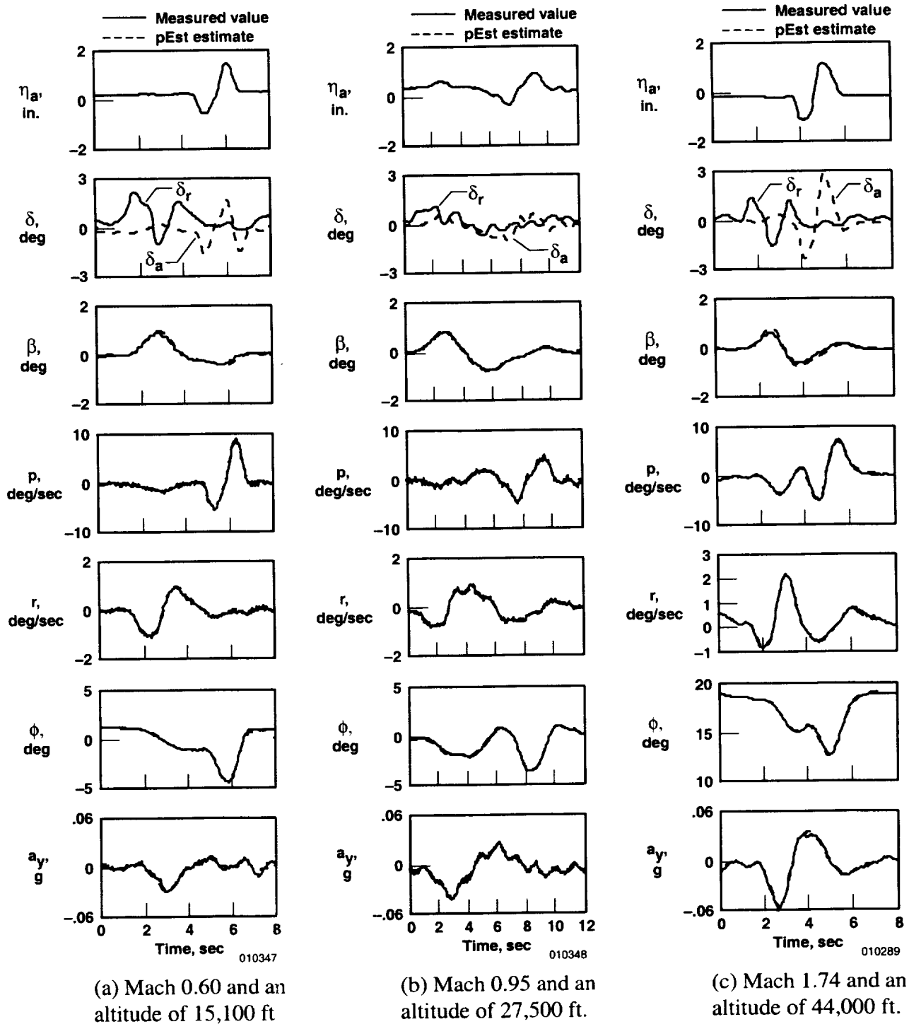
Figure 41. LASRE configuration lateral-directional maneuver time histories.
