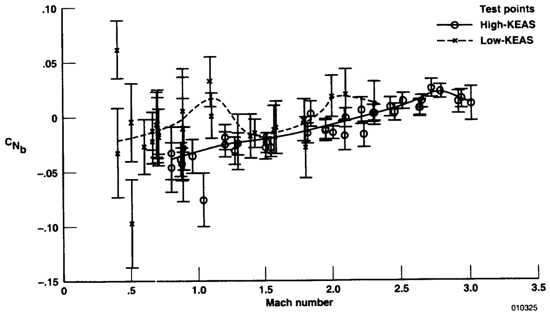
(a) C_{N_b} .
