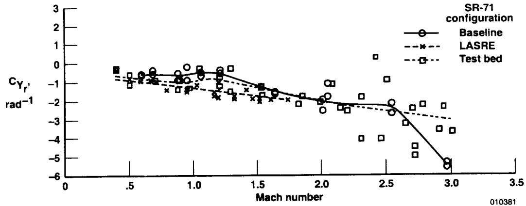
(a) C_{Y_r}' .
