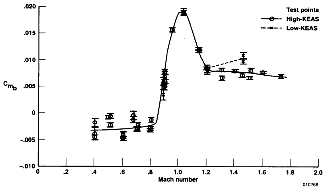
(b) C_{m_b} .
