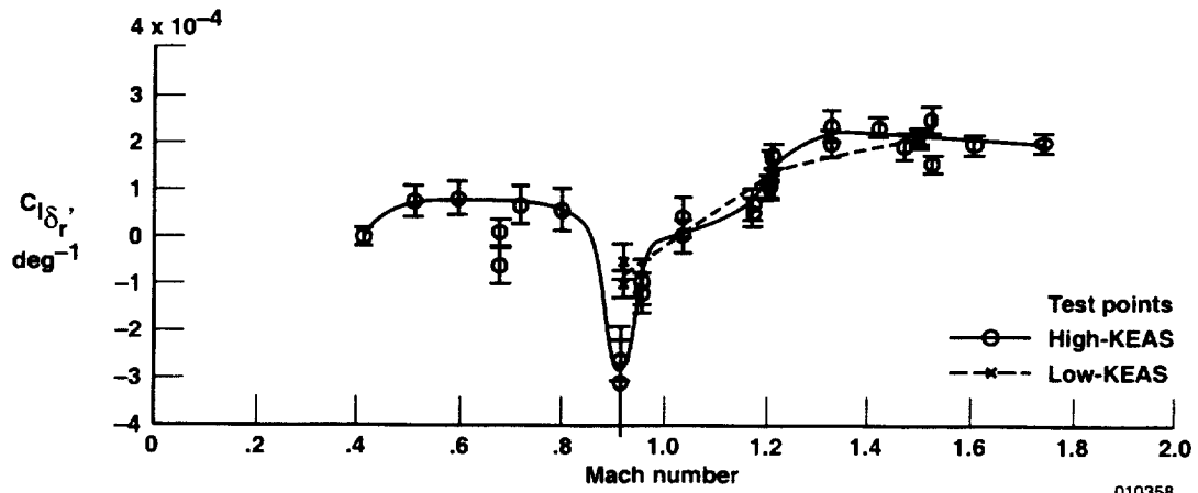
(b) C_{l_{\delta_r}}
