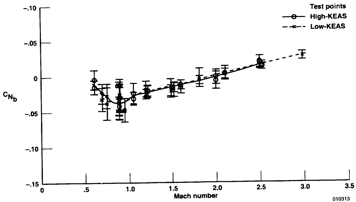
(a) C_{N_b} .
