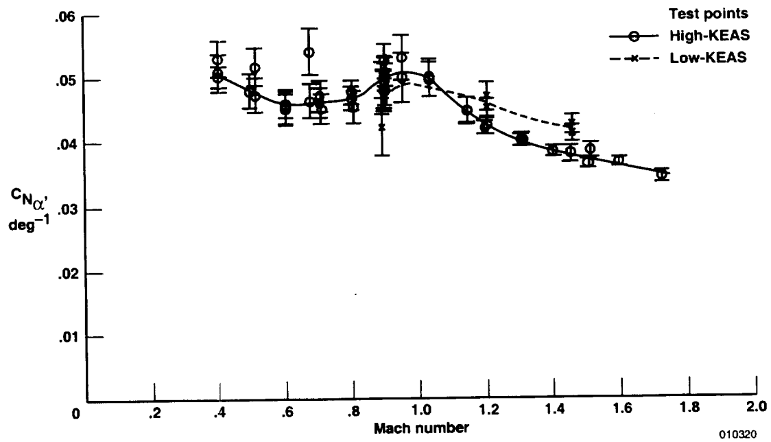
(a) C_{N_{\alpha}}
