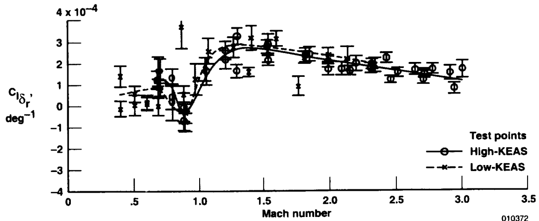
(b) C_{l_{\delta_r}}
