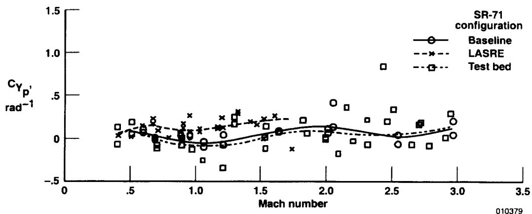
(a) C_{Y_p} .
