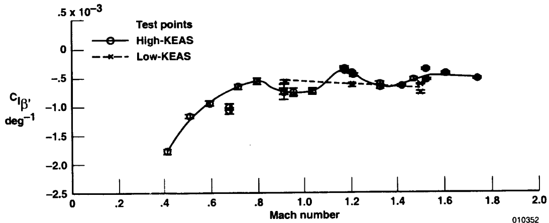
(b) C_{l\beta} .
