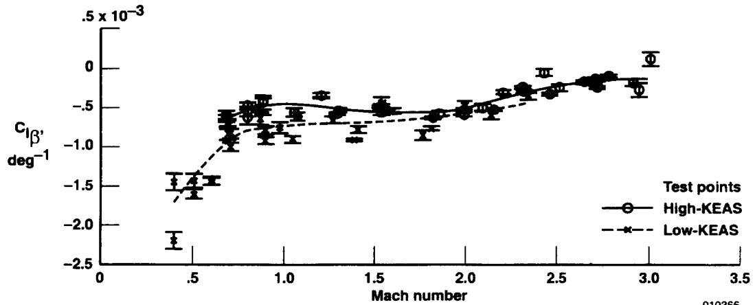
(b) C_{l\beta} .
