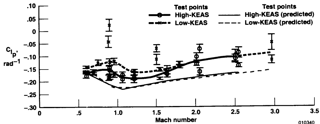
(b) C_{l_p} .
