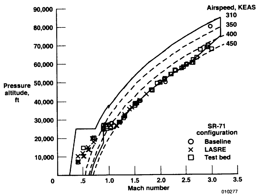
Figure 29. Flight conditions for comparison of configuration longitudinal stability and control derivatives.
