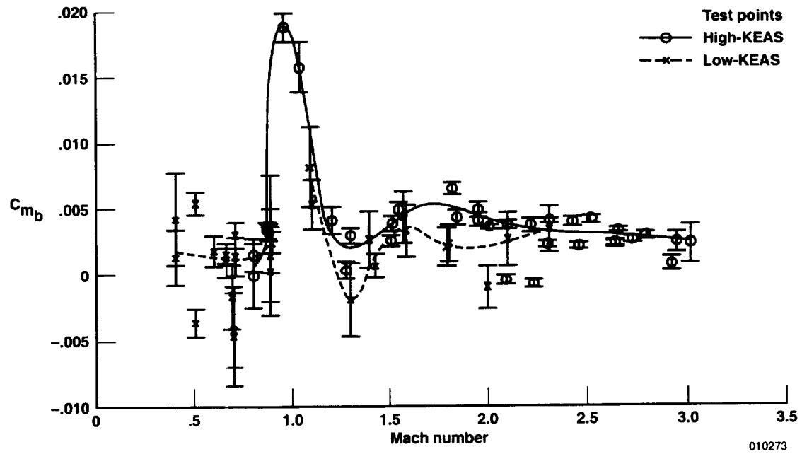
(b) C_{m_b} .
