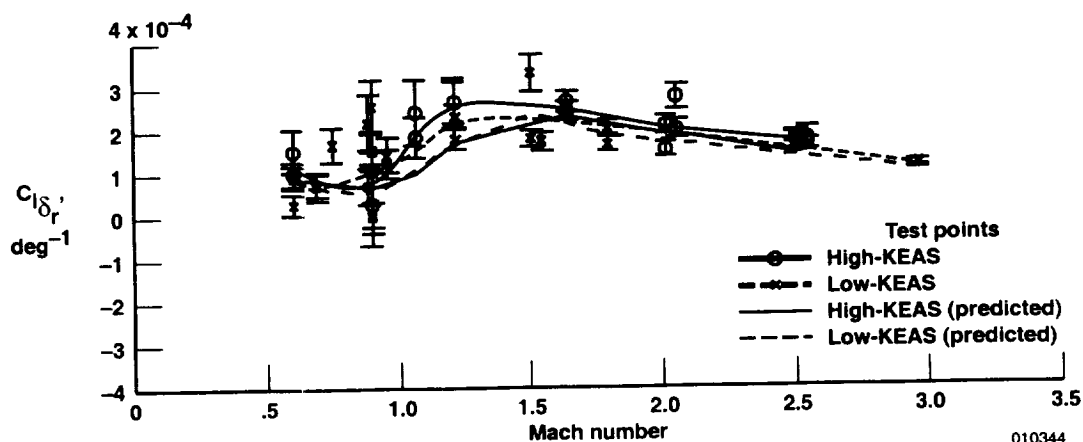
(b) C_{l\delta_r}'
