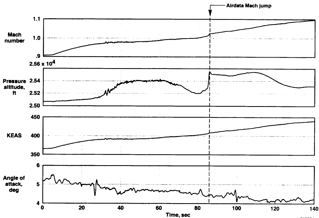
Figure 6. Time history of an acceleration from subsonic to supersonic flight (test bed configuration).
