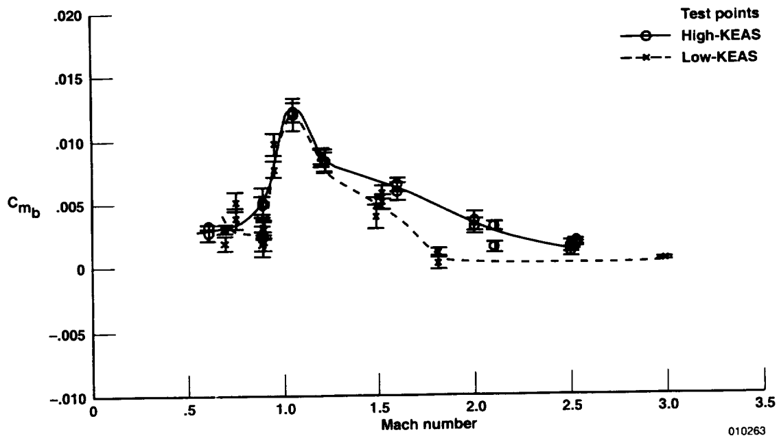
(b) C_{m_b} .
