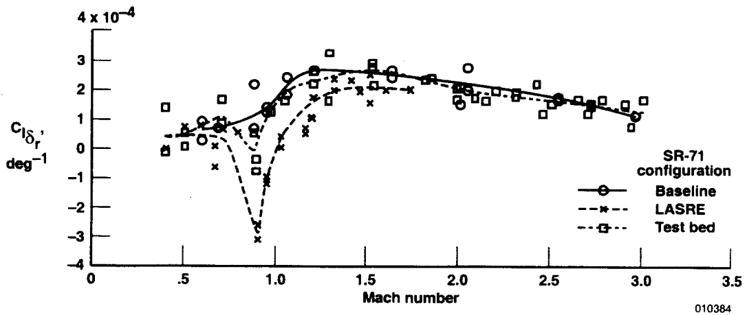
(b) C_{l_{\delta_r}}
