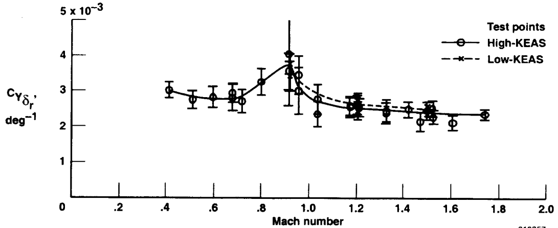
(a) C_{Y_{\delta_r}}
