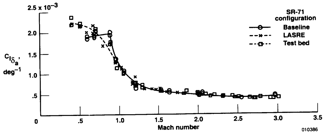
(b) C_{l_{\delta_a}}
