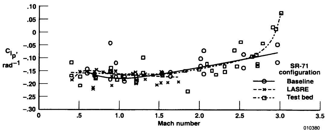
(b) C_{l_p} .
