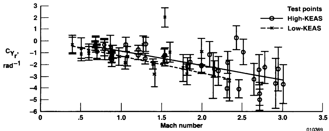
(a) C_{Y_r} .
