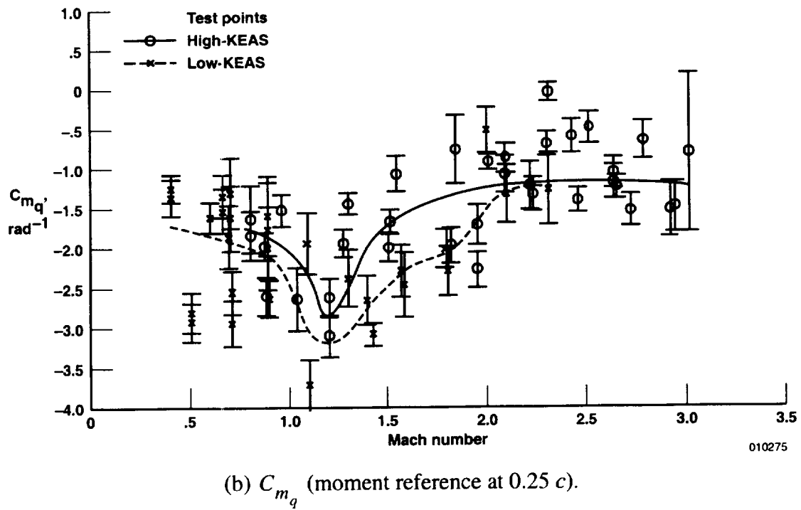
Figure 27. Flight-determined pitch-rate derivatives (test bed configuration).
