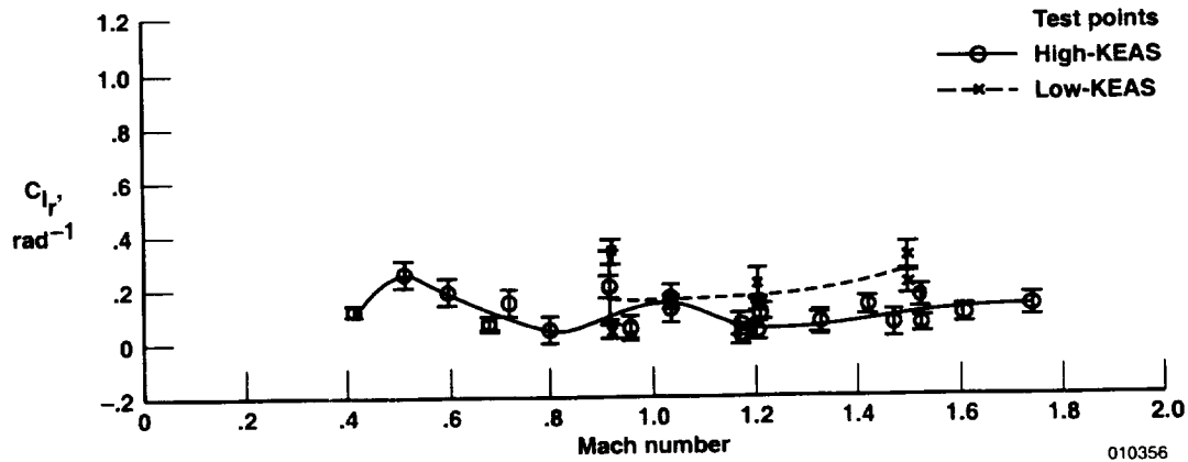
(b) C_{l_r} .
