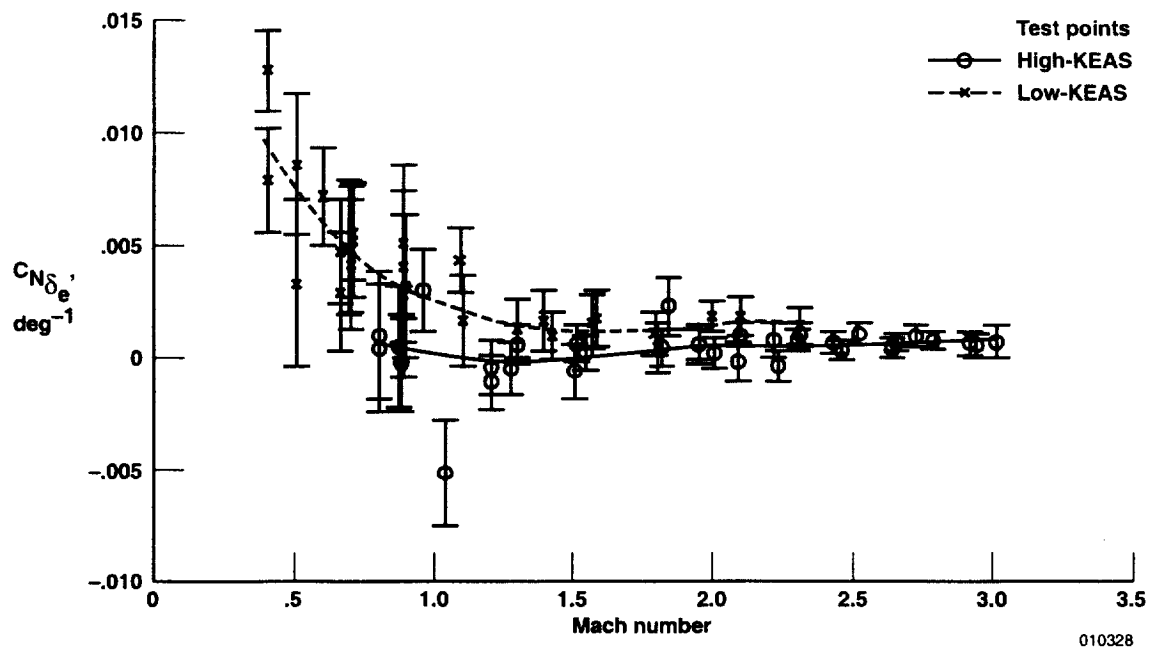
(a) C_{N_{\delta_e}}
