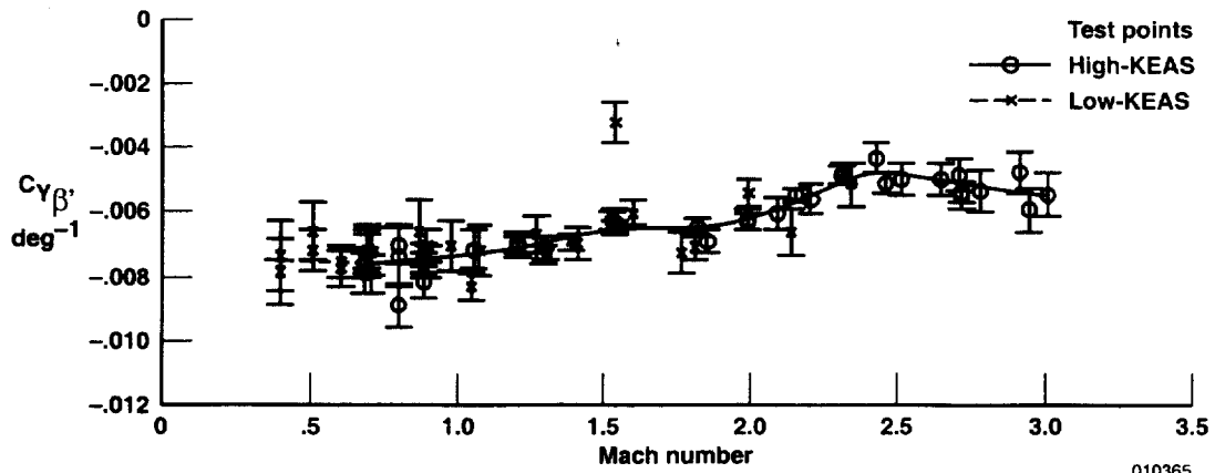
(a) C_{Y\beta} .
