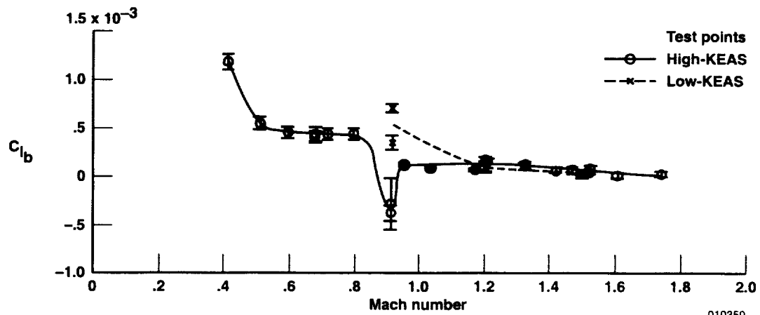
(b) C_{l_b} .
