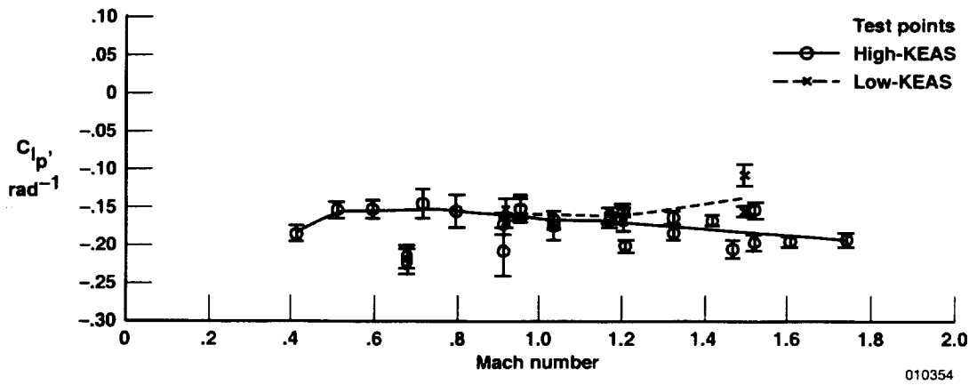
(b) C_{l_p} .
