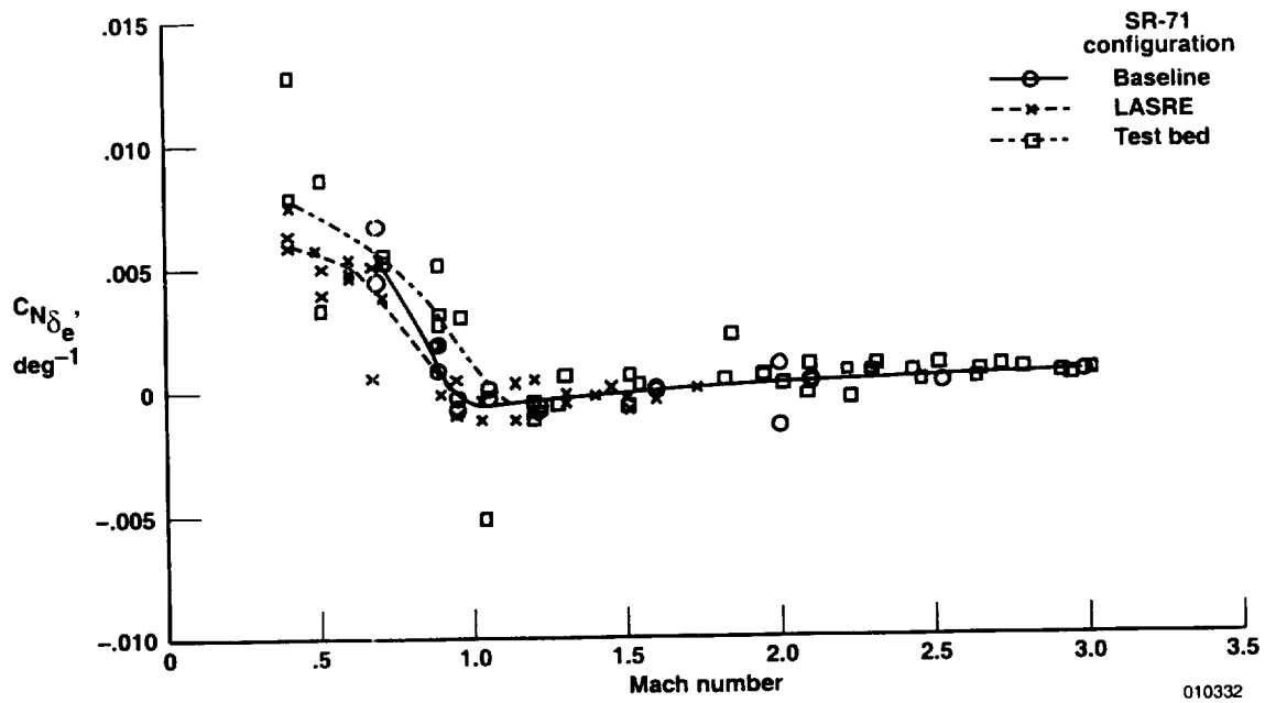
(a) C_{N_{\delta_e}}
