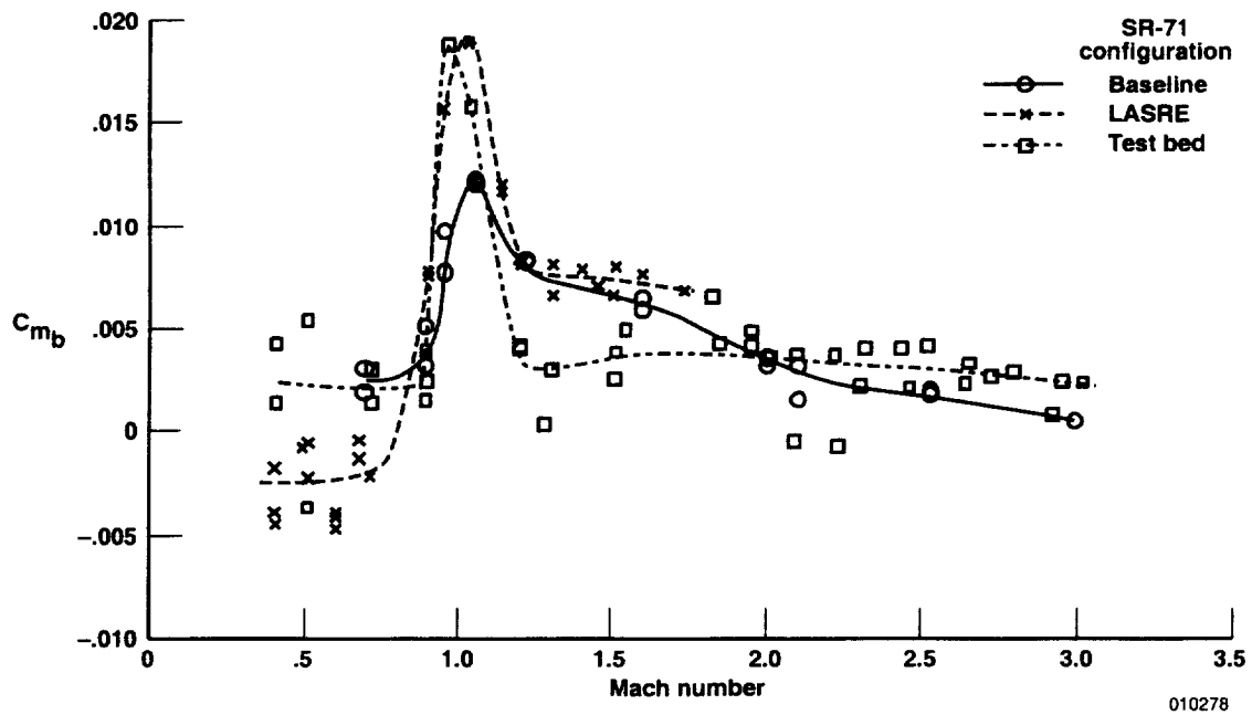
(b) C_{m_b} .
