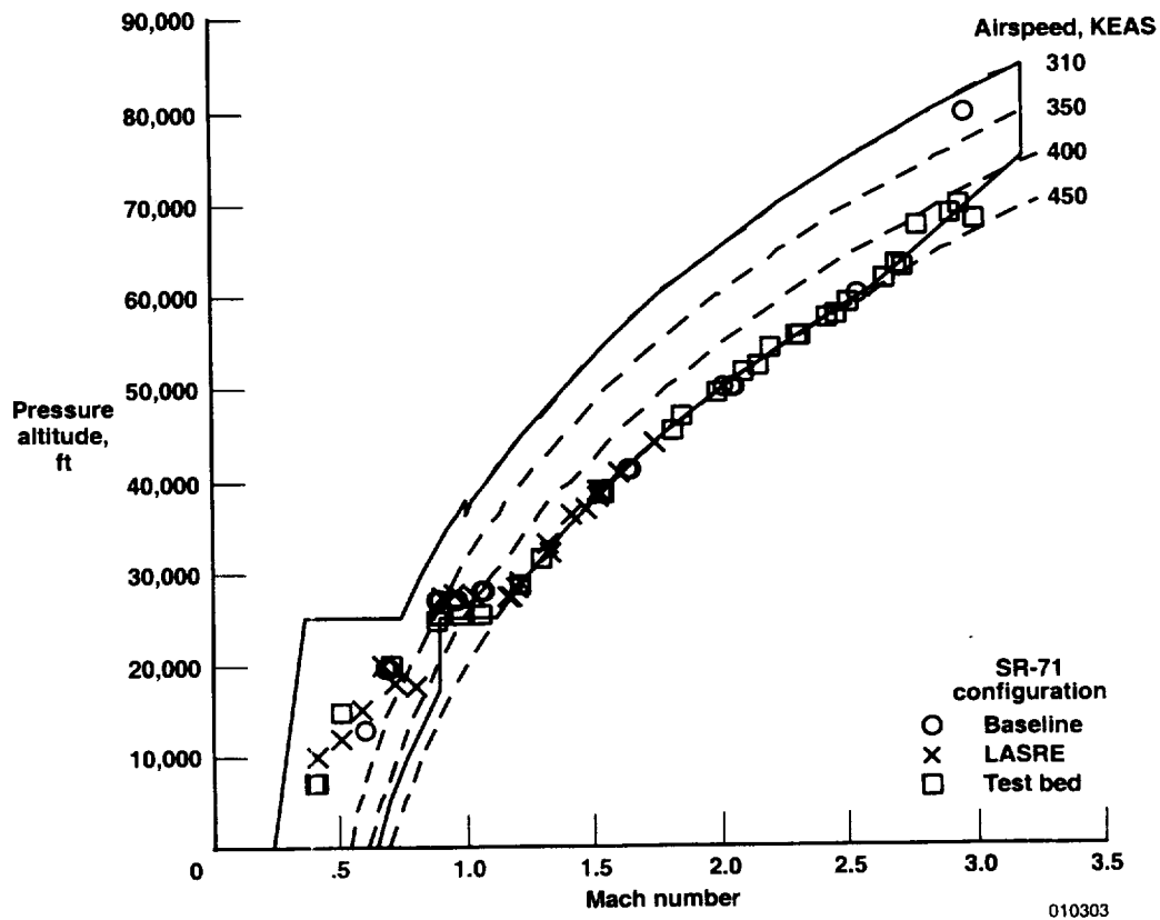
Figure 55. Flight conditions for comparison of configuration lateral-directional stability and control derivatives.
