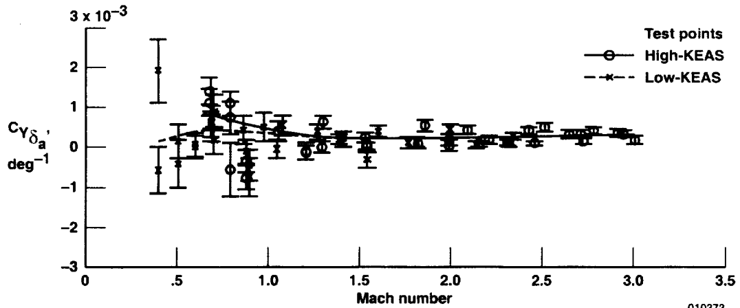
(a) C_{Y\delta_a} .
