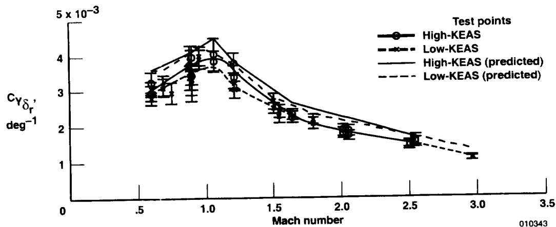
(a) C_{Y\delta_r}'
