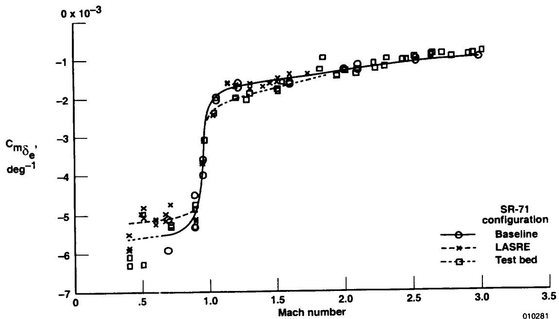
(b) C_{m_{\delta_e}} (moment reference at 0.25 c).
