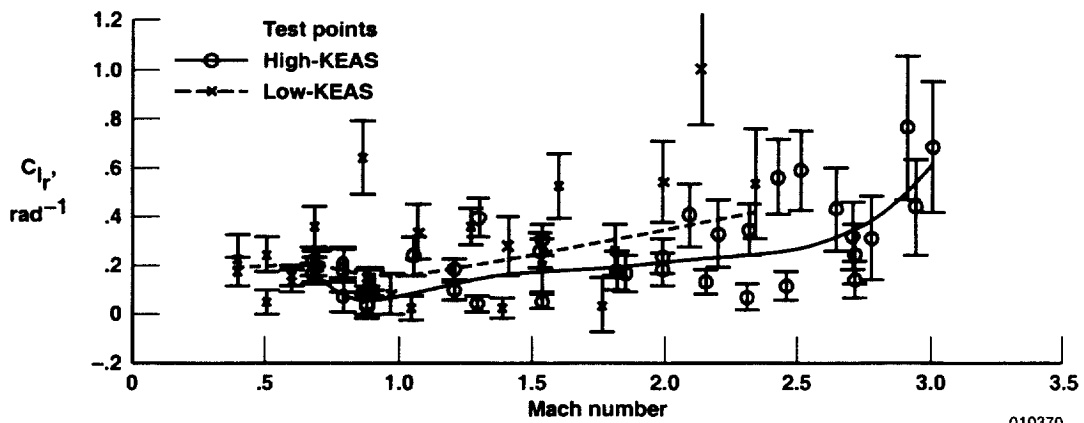
(b) C_{l_r} .
