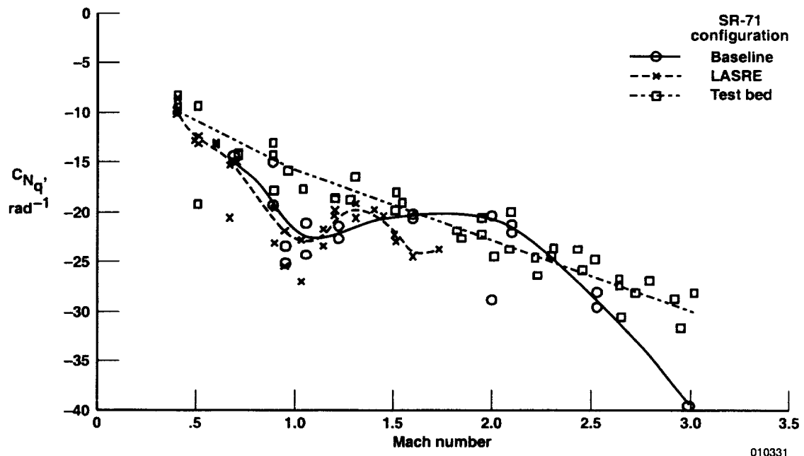
(a) C_{N_q} .
