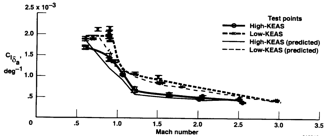
(b) C_{l_{\delta_a}}
