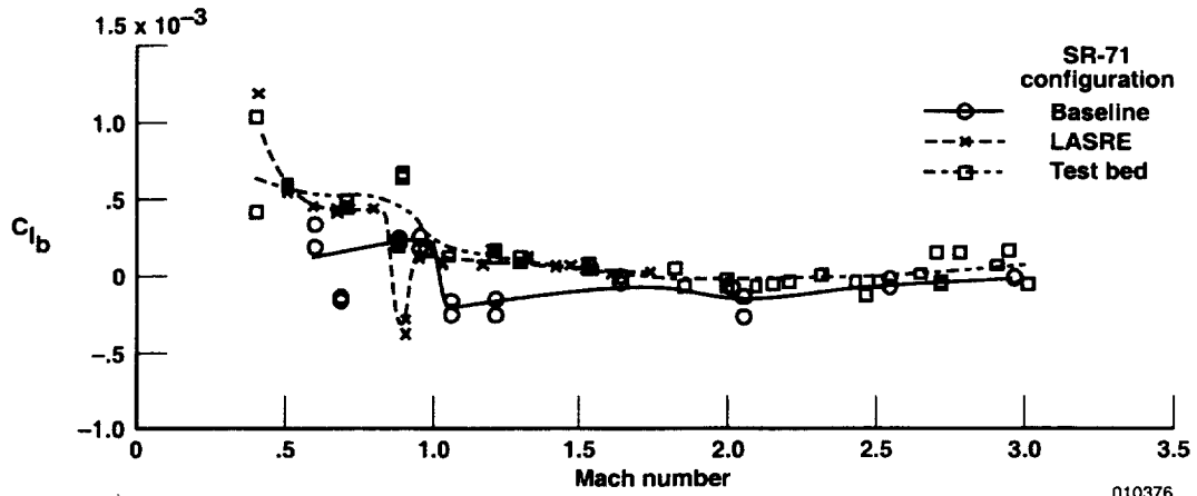
(b) C_{l_b} .
