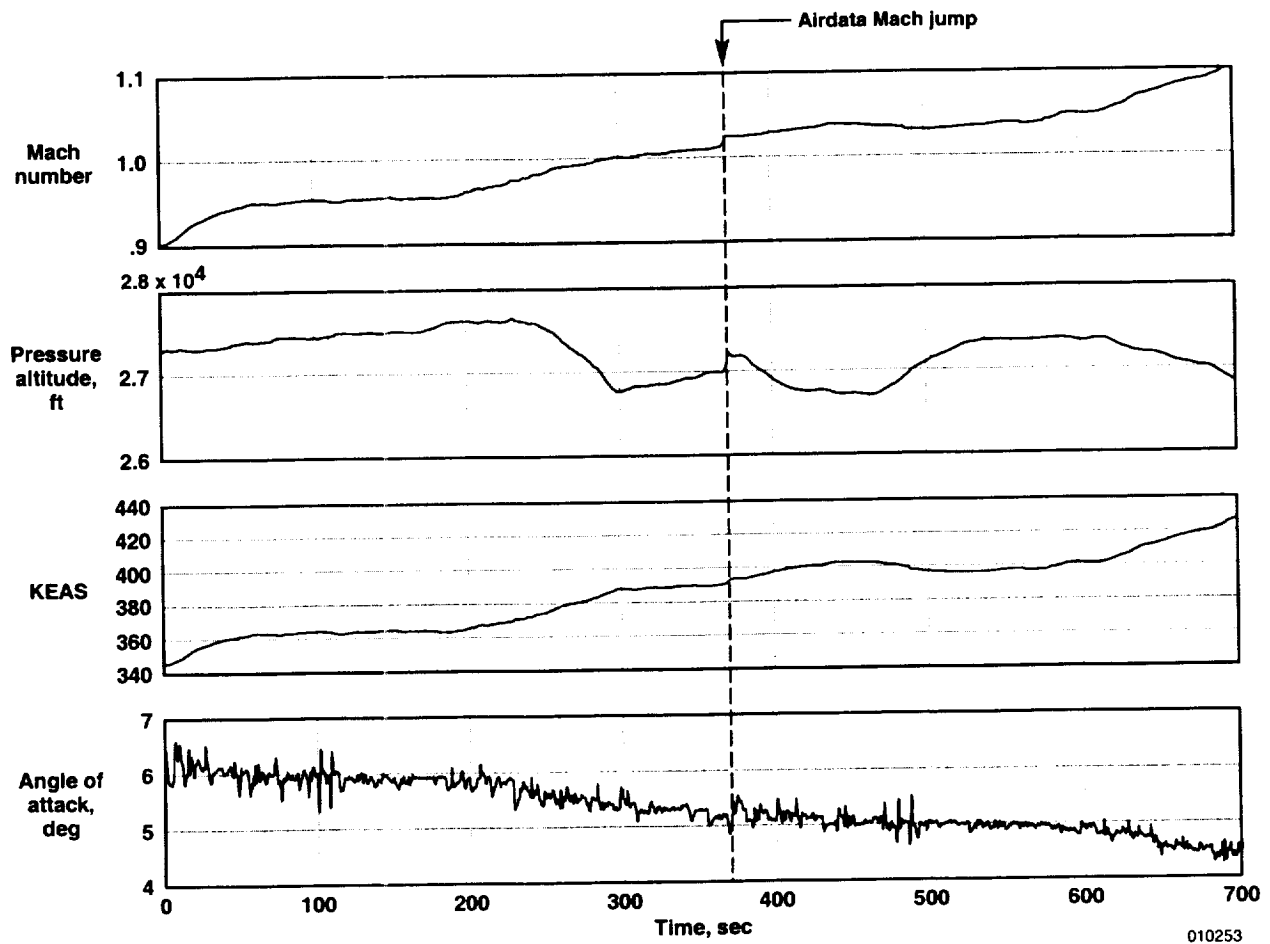
Figure 5. Time history of an acceleration from subsonic to supersonic flight (LASRE configuration).
