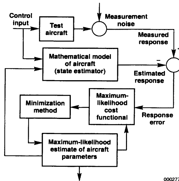
Figure 8. Maximum-likelihood parameter estimation process.
