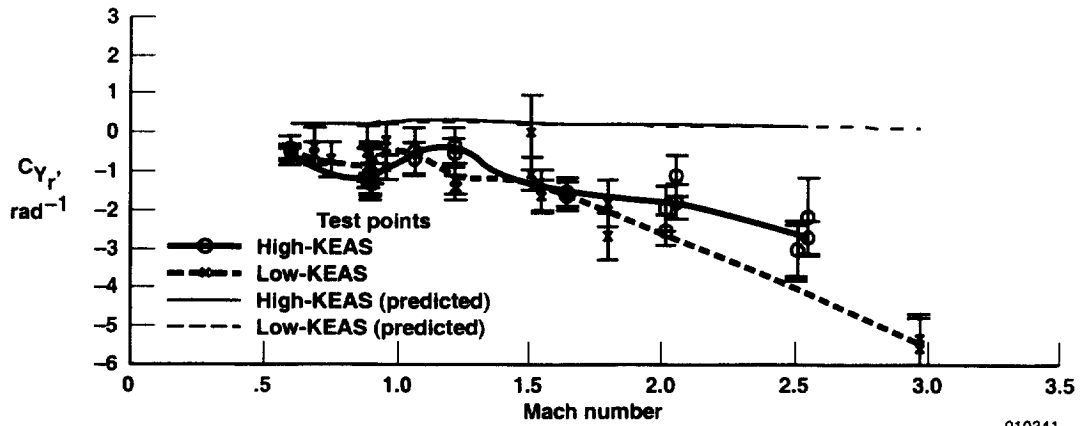
(a) C_{Y_r} .
