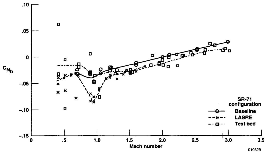
(a) C_{N_b} .
