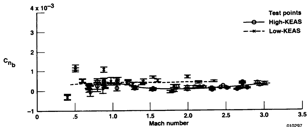
(c) C_{n_b} .
