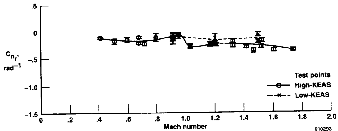
(c) C_{n_r} (moment reference at 0.25 c).
