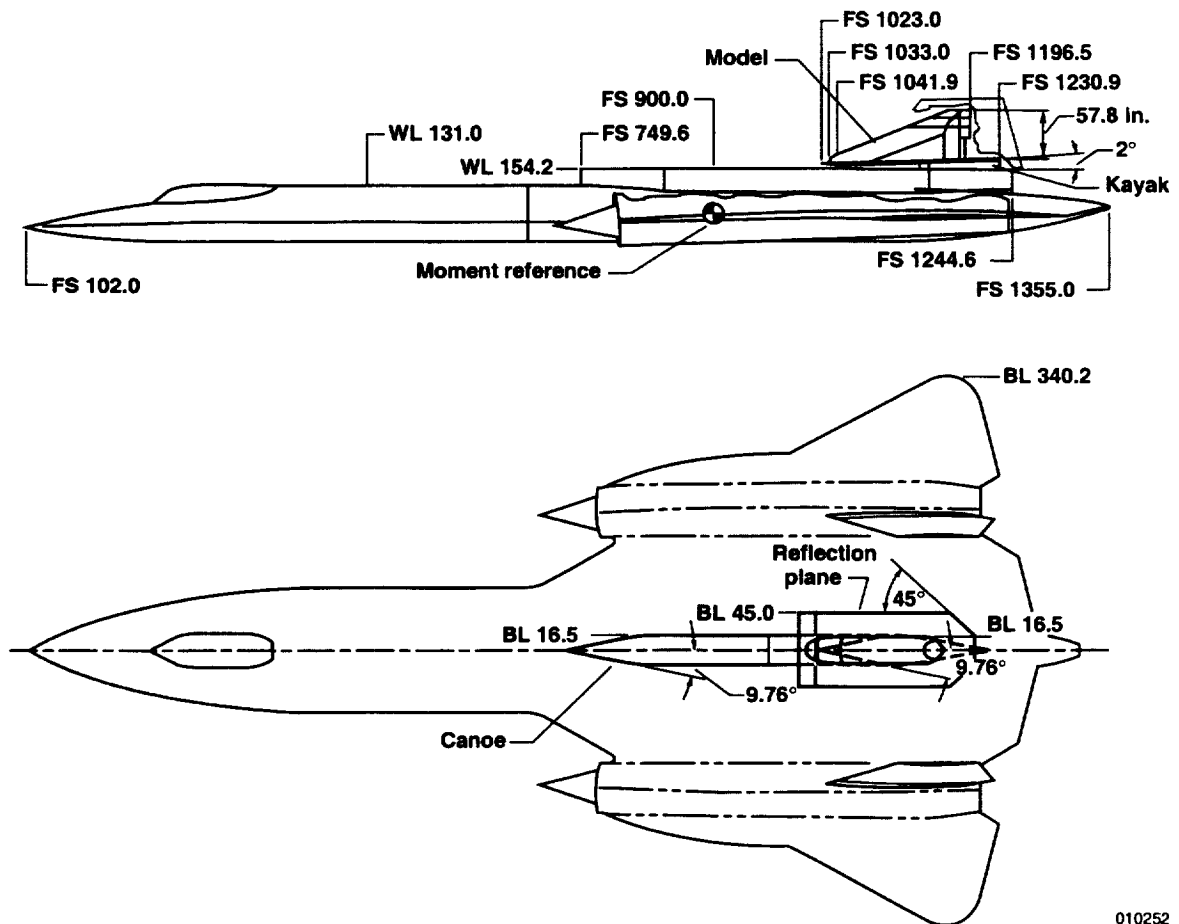
Figure 4. Side and planform views of the LASRE configuration.
