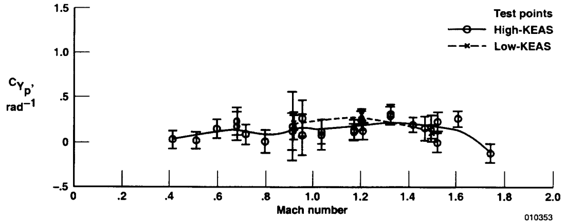
(a) C_{Y_p} .
