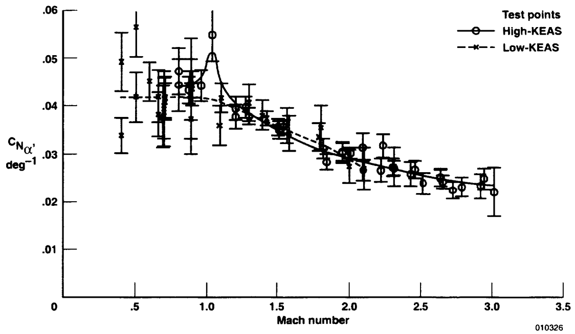
(a) C_{N_{\alpha'}}
