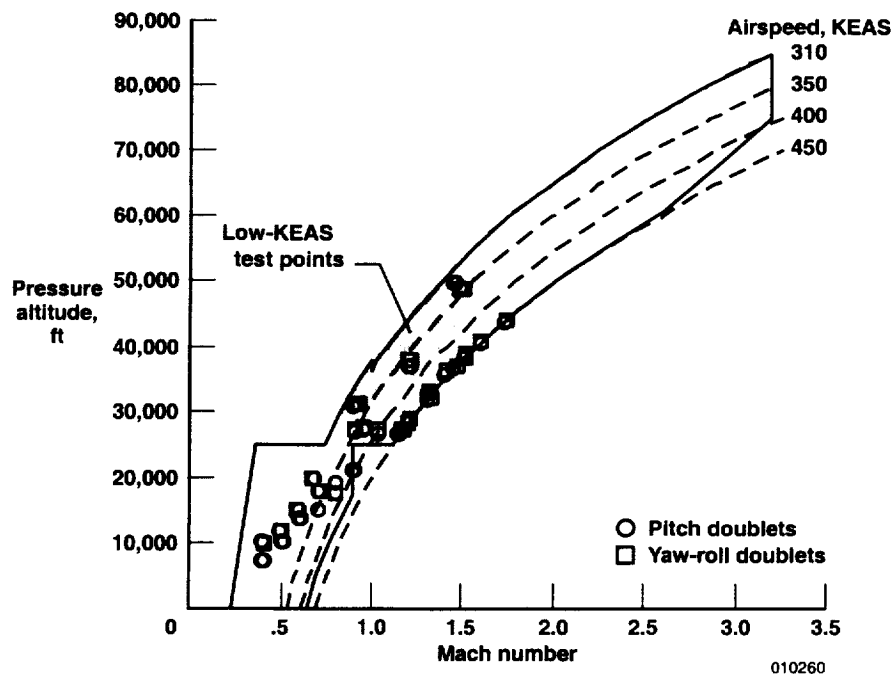
Figure 12. Flight conditions for stability and control test points (LASRE configuration).
