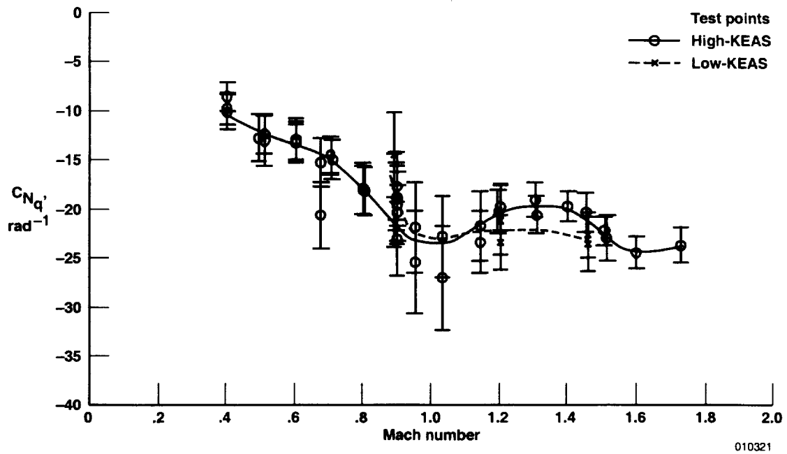
(a) C_{N_q} .
