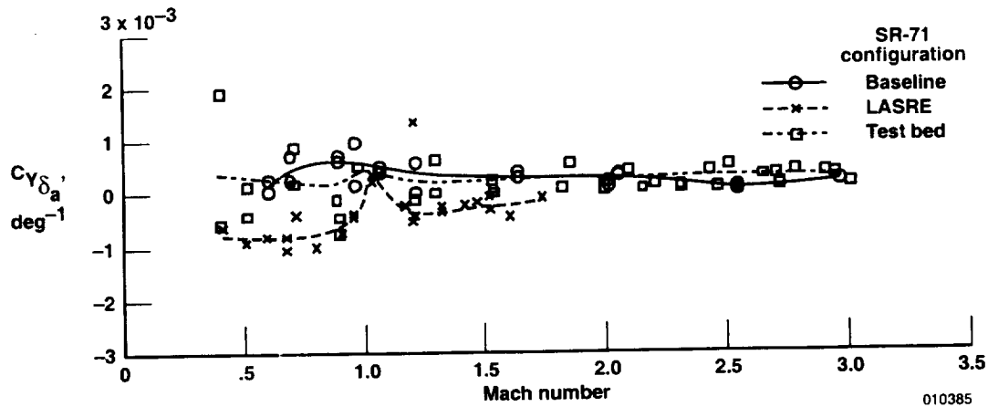
(a) C_{Y_{\delta_a}}
