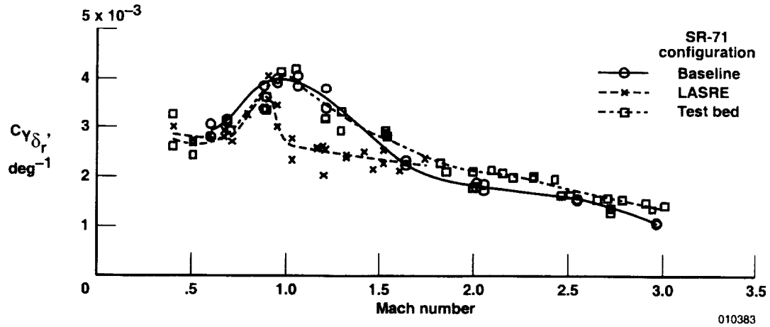
(a) C_{Y_{\delta_r}}
