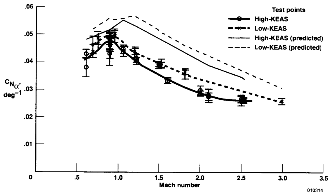
(a) C_{N_{\alpha'}}
