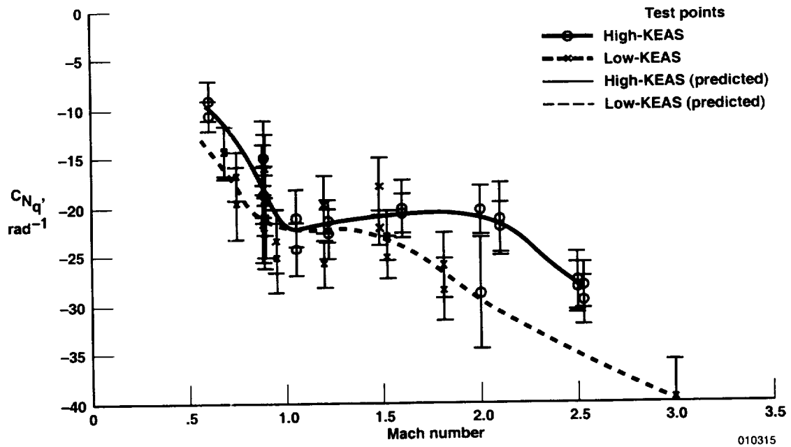
(a) C_{N_q} .
