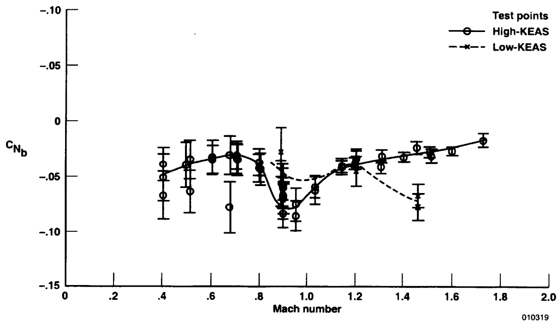
(a) C_{N_b} .
