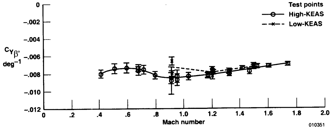
(a) C_{Y\beta} .
