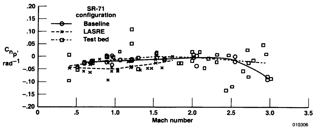
(c) C_{n_p} (moment reference at 0.25 c ).
