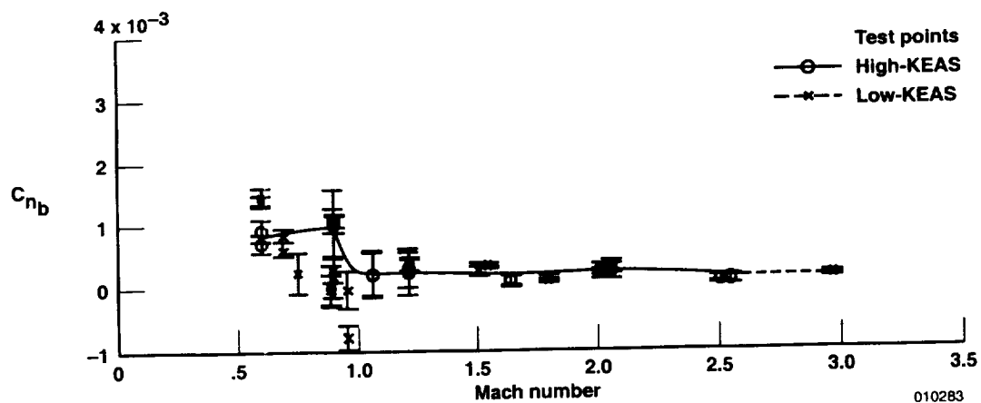
(c) C_{n_b} .
