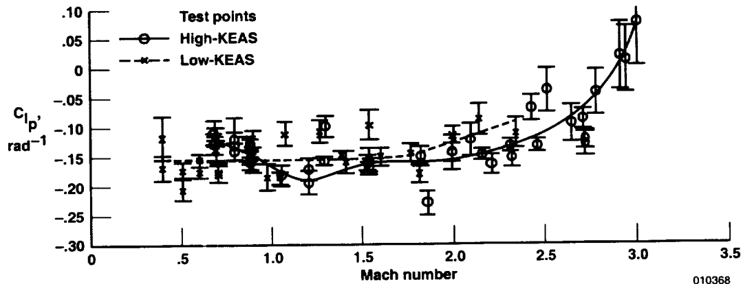
(b) C_{l_p} .
