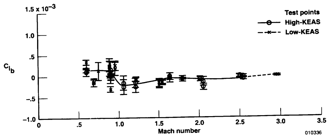
(b) C_{l_b} .
