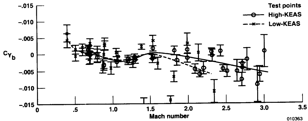
(a) C_{Y_b} .
