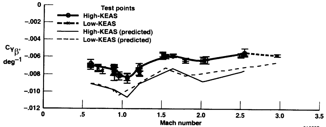
(a) C_{Y_{\beta}} .
