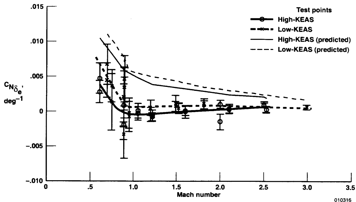
(a) C_{N_{\delta_e}}
