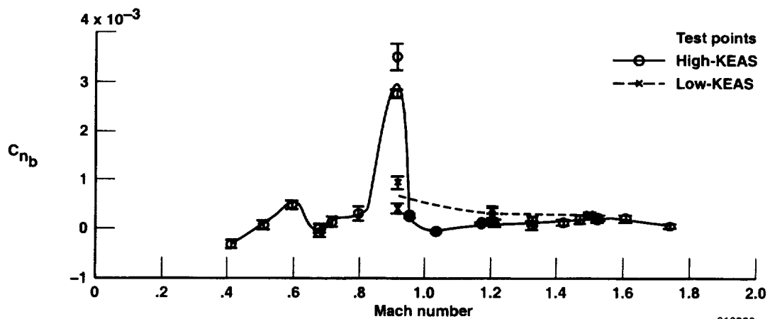
(c) C_{n_b} .
