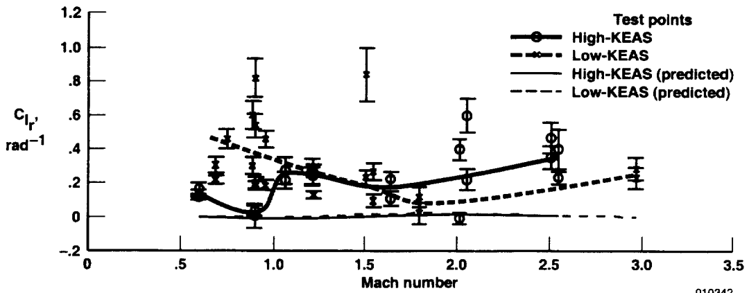
(b) C_{l_r} .
