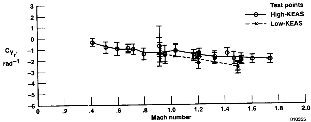
(a) C_{Y_r} .
