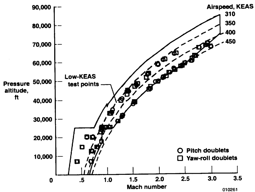
Figure 13. Flight conditions for stability and control test points (test bed configuration).
