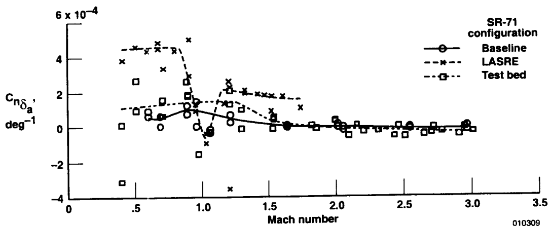
(c) C_{n_{\delta_a}} (moment reference at 0.25 c ).
