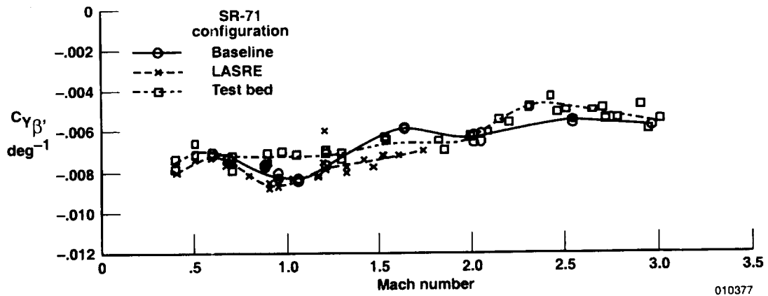
(a) C_{Y\beta} .
