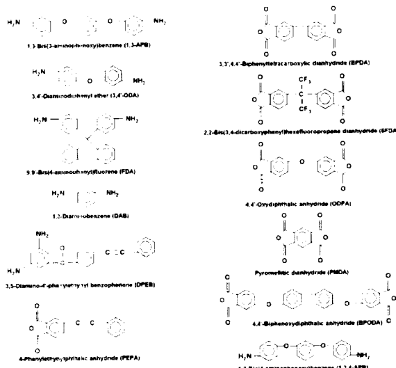
Fig. 1 Examples of chemical structures of the monomers used in this method to prepare high performance resins for RTM and/or RI
