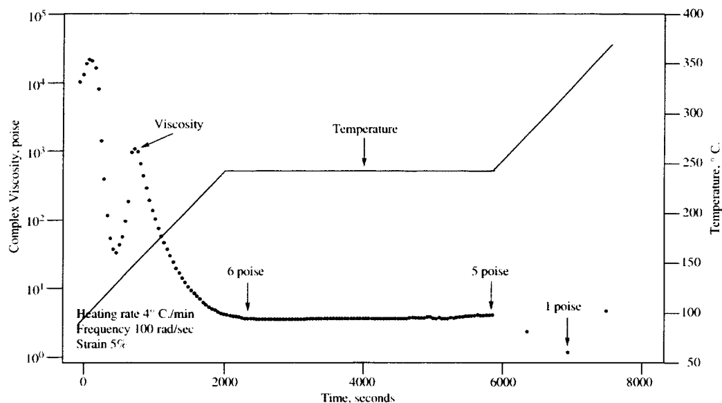
(Isothermal melt viscosity at 250° C. of material described in Example 1)
