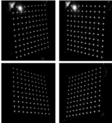
d) 0.7-m oscillating Kapton membrane with retroreflective targets
