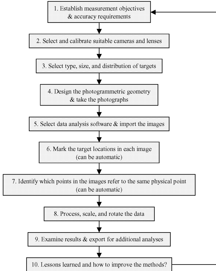
Fig. 2. The 10 steps of photogrammetry.
