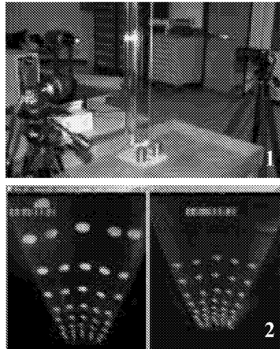
b) 1-m flexible Fresnel lens (1-projected dots, 2-adhesive targets)
