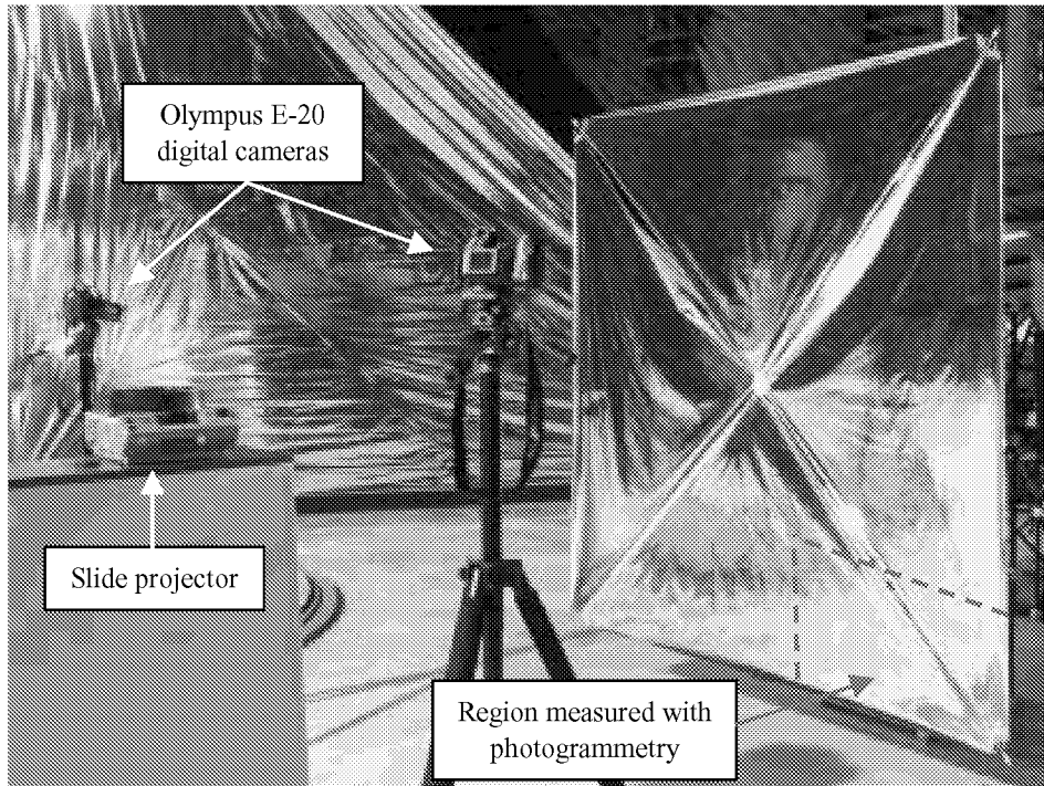
Fig. 6. Equipment for photogrammetry of 2-m solar sail model using projected dots.
