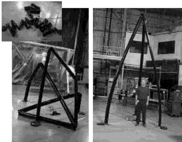
f) 4.5-m inflatable tripod
