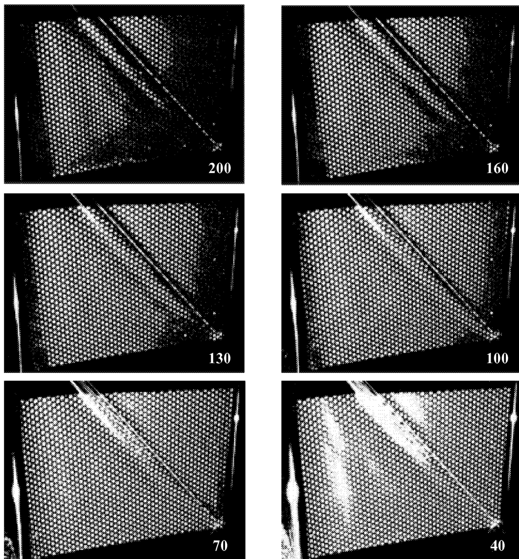
Fig. 8. Left image displayed at various binary intensity thresholds.
