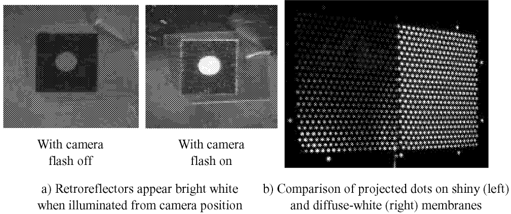
Fig. 5. Retroreflective and projected circular targets.
