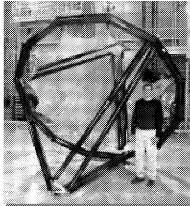
e) 3-m hexapod reflector for active control experiments (projected dots on stretched membrane reflector)
