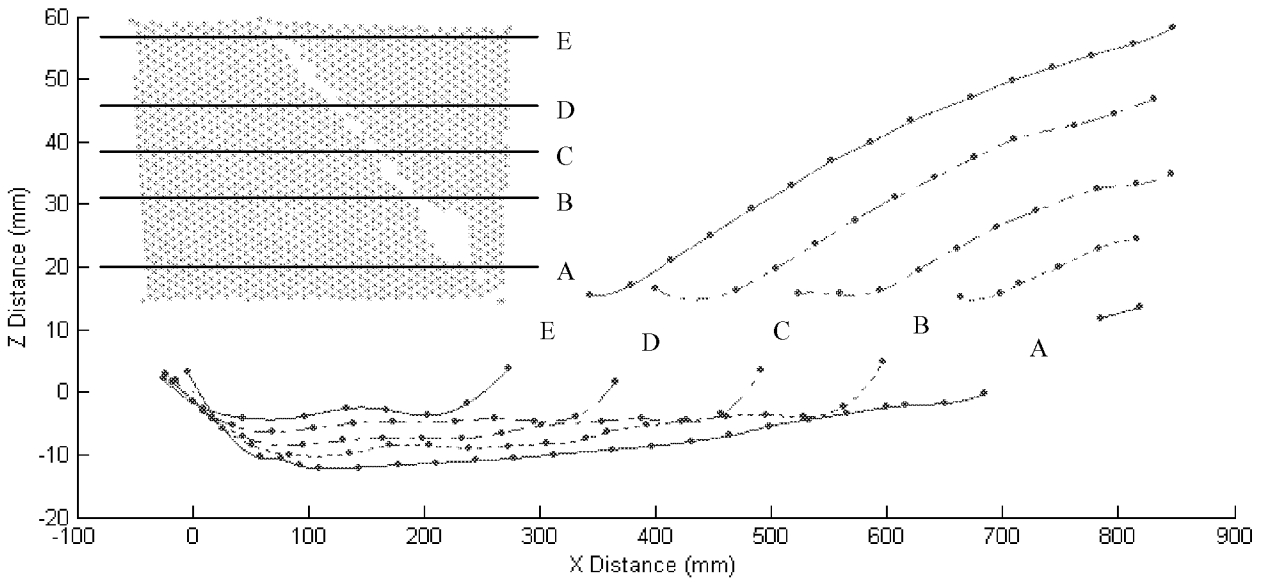
Fig. 12. Out-of-plane membrane shape at various elevations.
