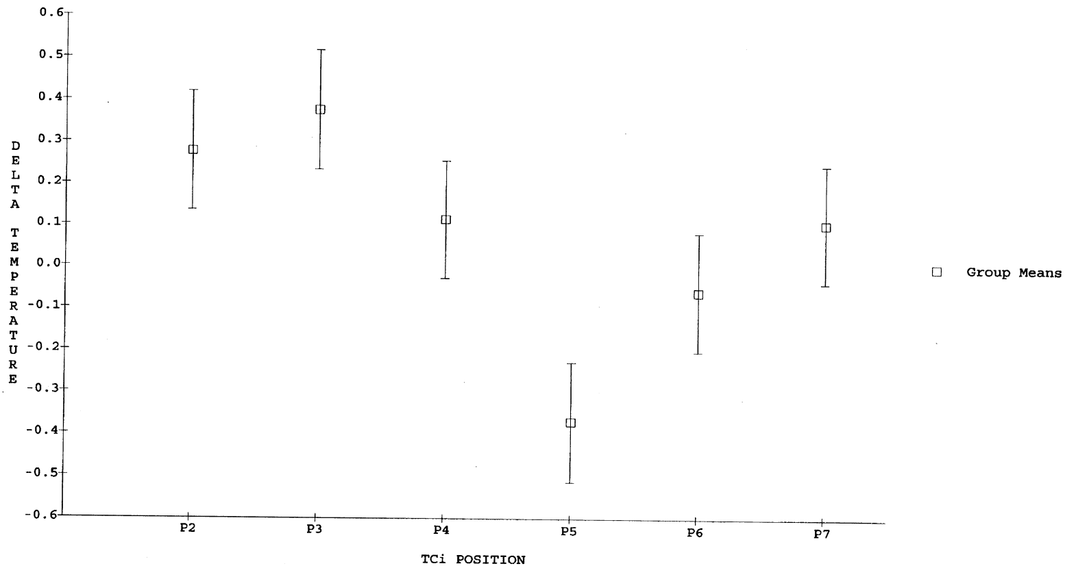
FIGURE C2 METAL BLOCK METHOD OF CALIBRATING UNSHEATHED THERMOCOUPLES BONFERRONI MULTIPLE COMPARISON OF MEANS PROCEDURE
