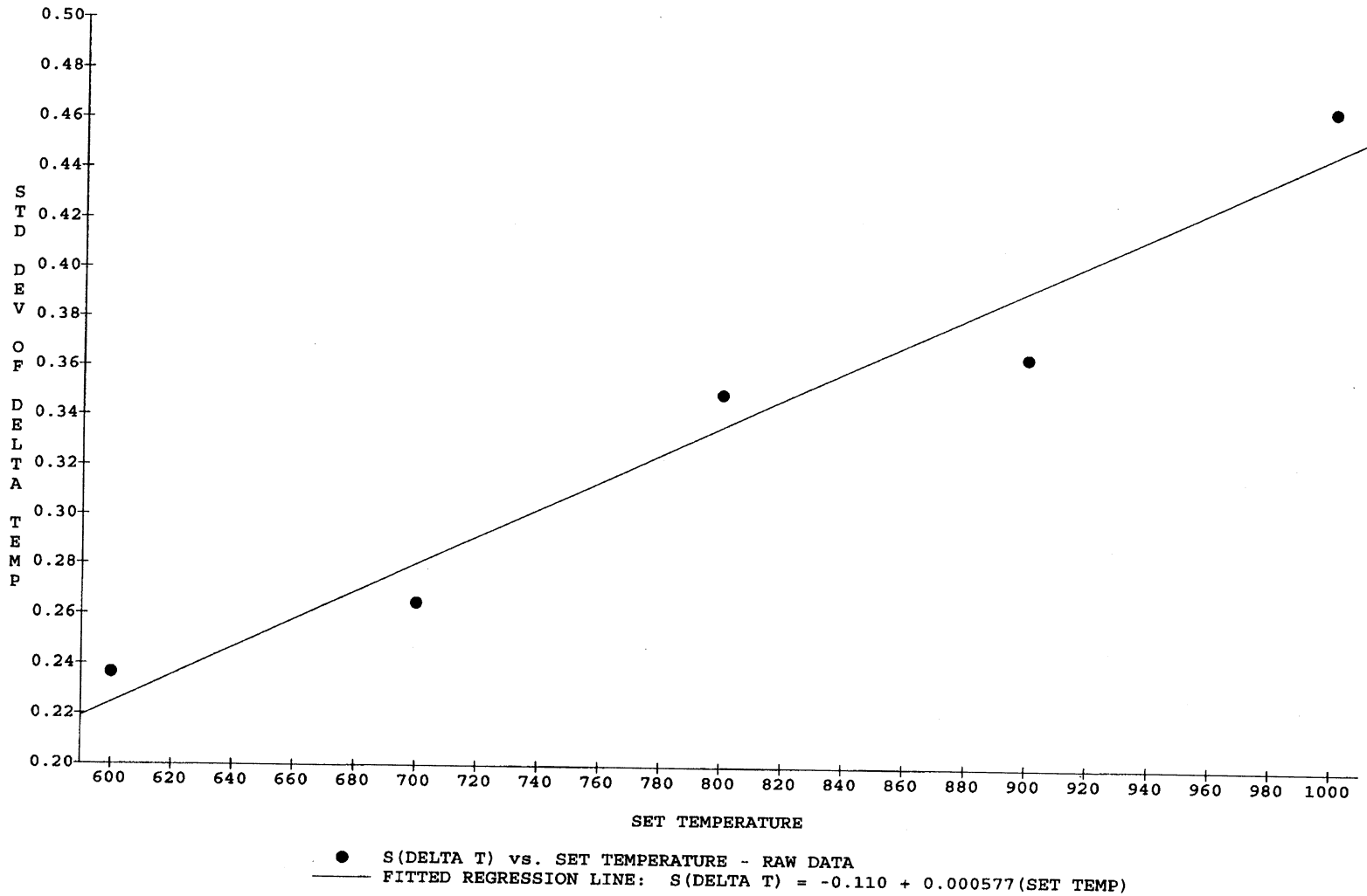
FIGURE D1 TEST ERROR STRUCTURE FOR TYING METHOD OF CALIBRATING UNSHEATHED THERMOCOUPLES
