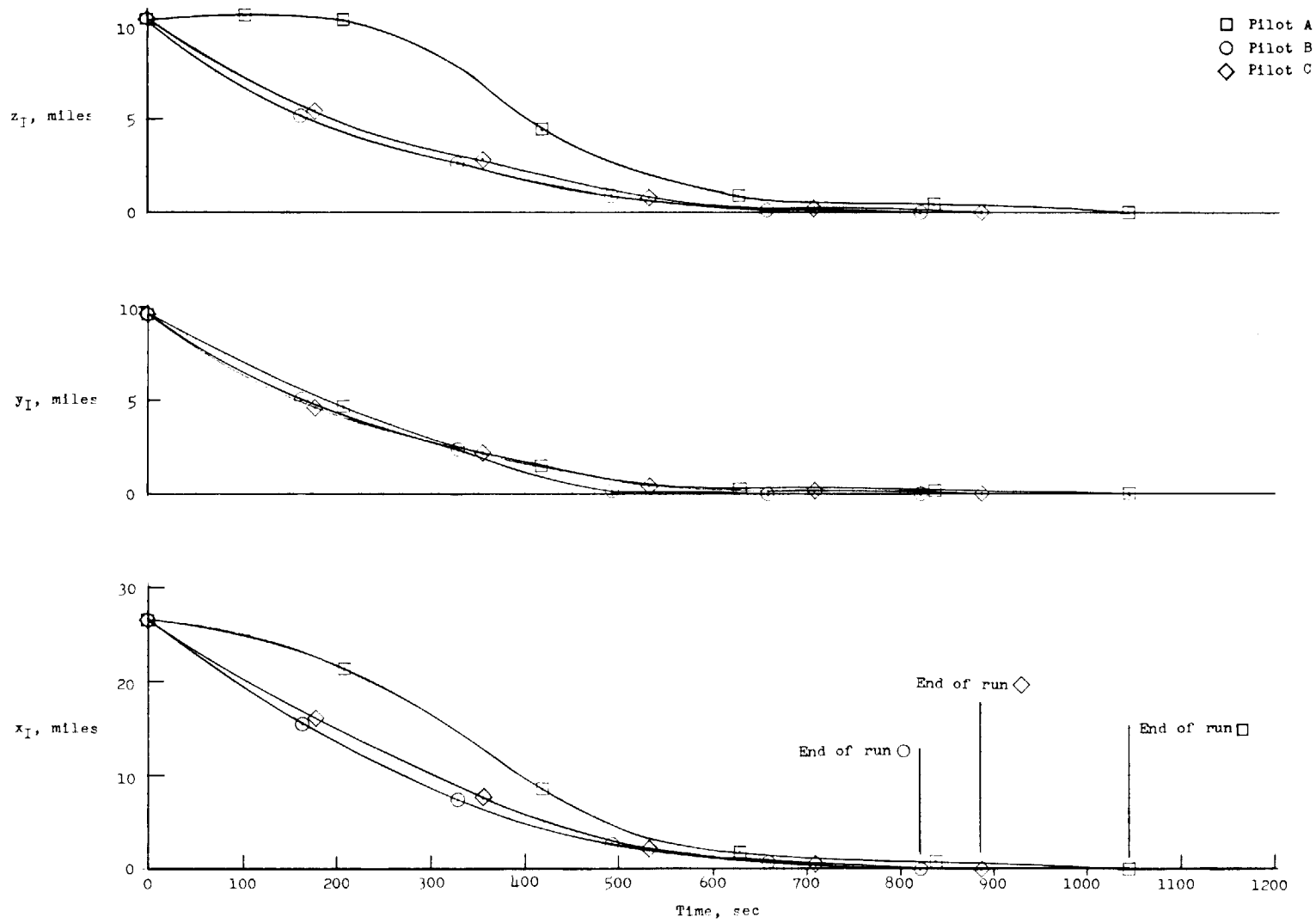
Figure 17.- Position-time trajectories of near-orbital rendezvous (case 6).
