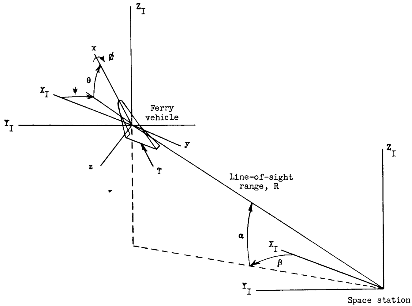
Figure 2.- Line-of-sight and Euler angle relations between rendezvous vehicle and space station.
