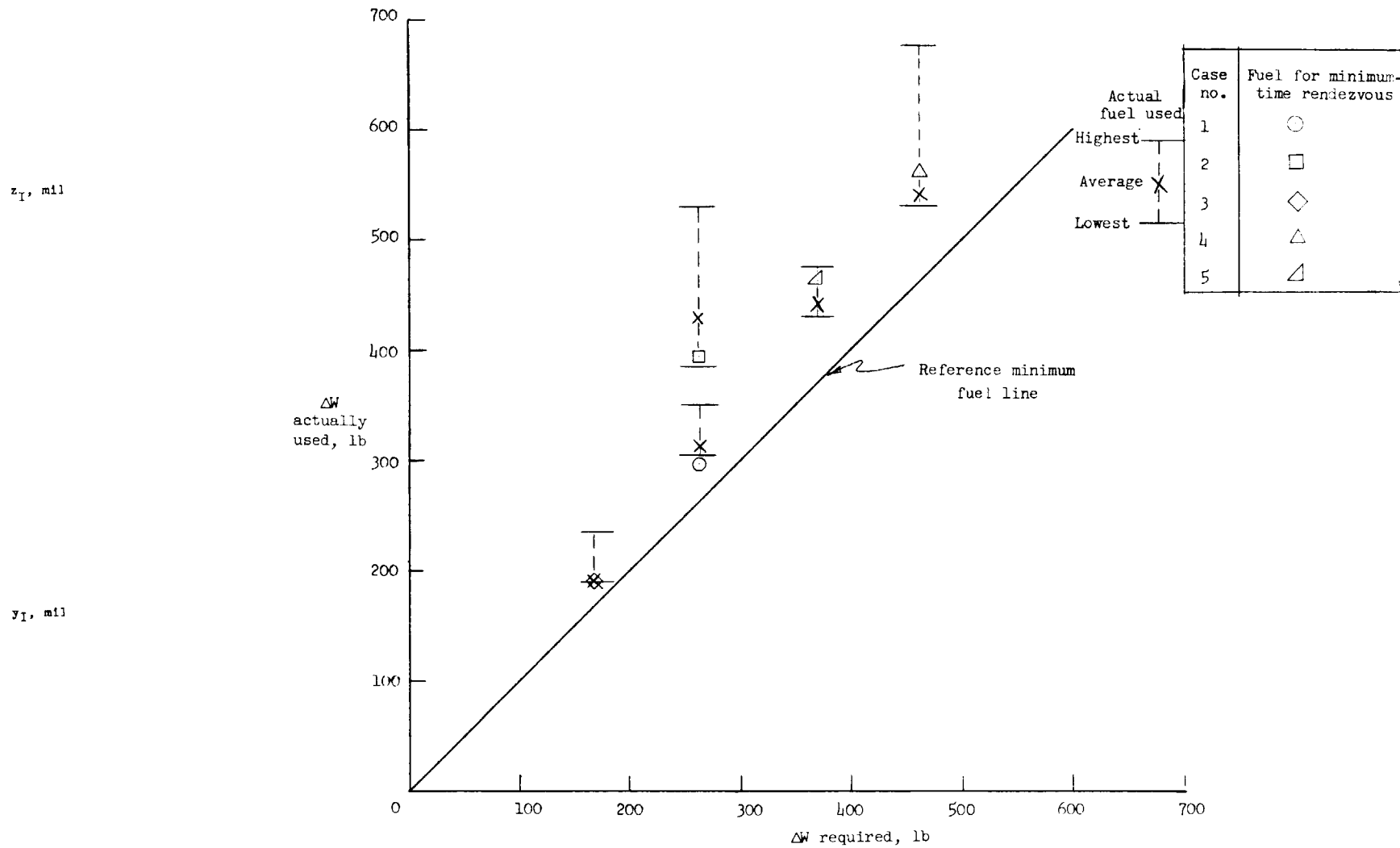
Figure 14.- Weight of fuel used relative to fuel required for rendezvous with cases 1 through 5 (table 1).
