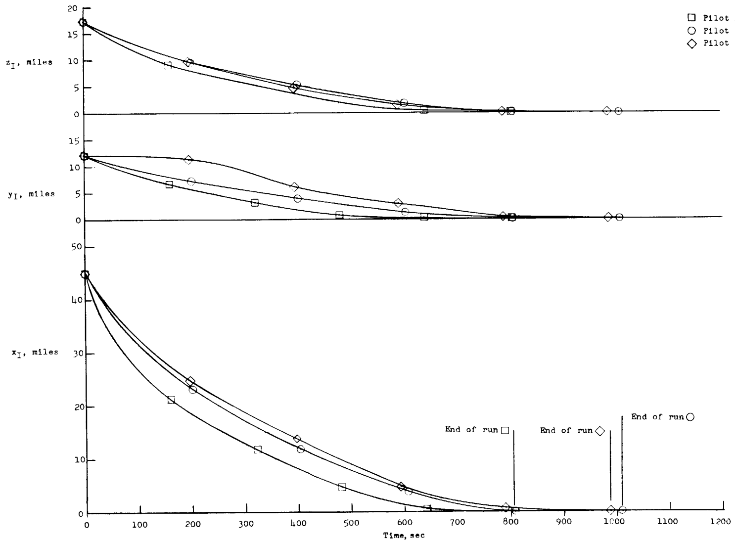
Figure 12.- Position-time trajectories of pilots for rendezvous conditions of case 4 (table 1).
