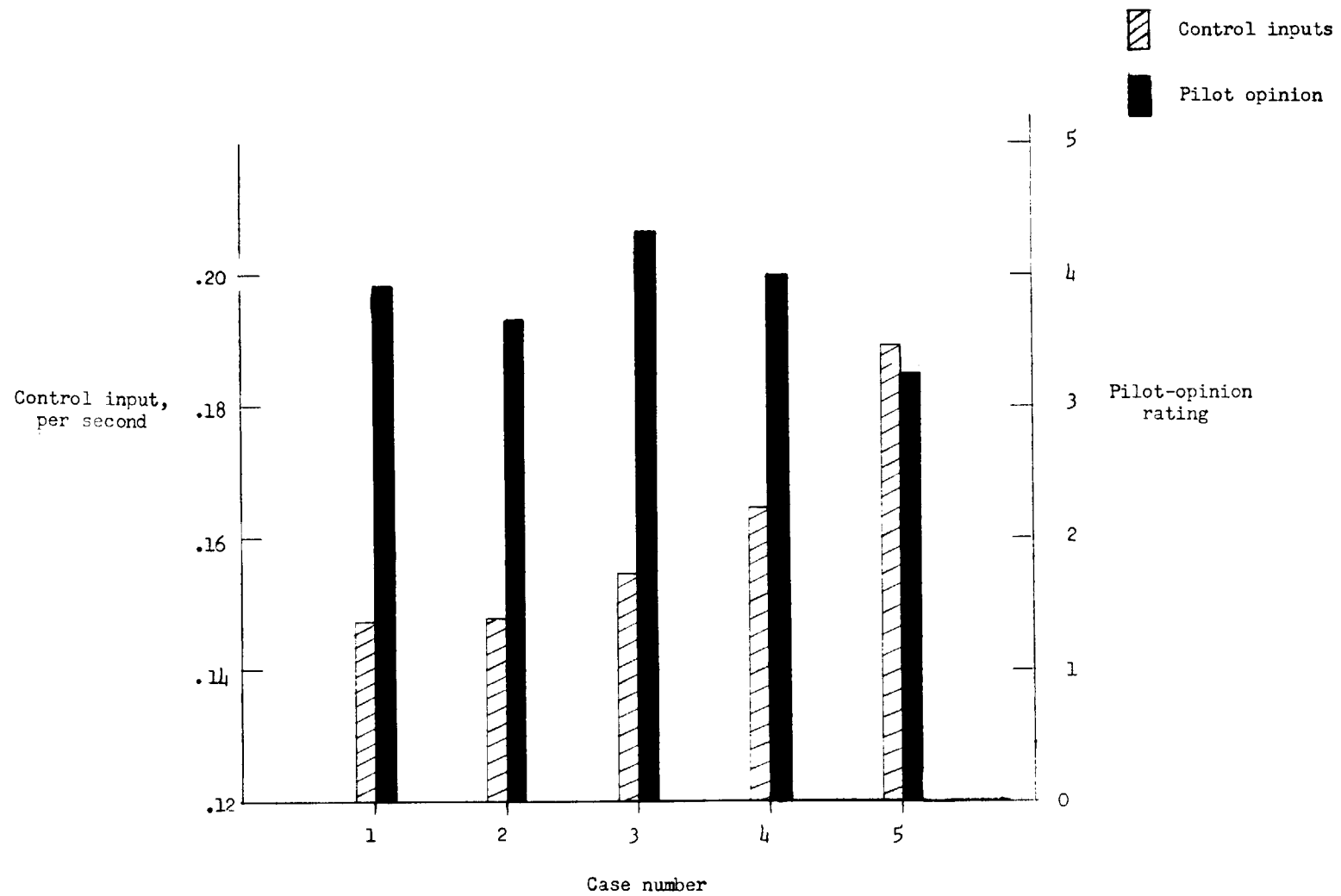
Figure 8.- Bar graph of pilot-opinion ratings and control inputs for all rendezvous cases. (Conditions for each case listed in table 1.)
