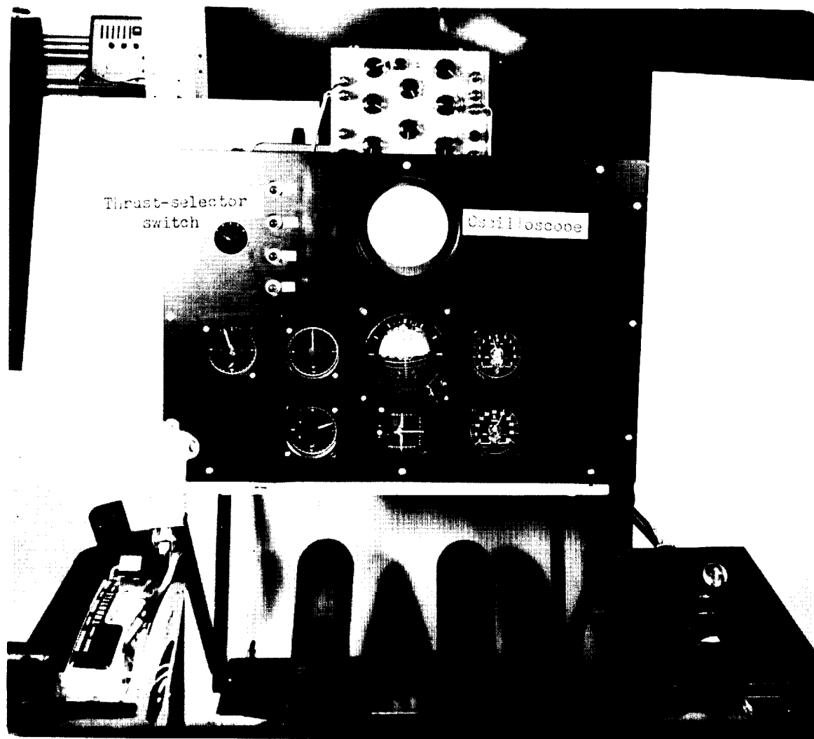
Figure 5.- Instrument panel 1 showing oscilloscope display. L-60-3092
