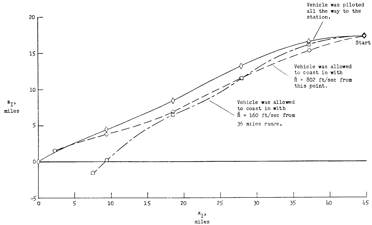
Figure 19.- Trajectories of vehicle showing effects of gravity and orbital ellipticity.
