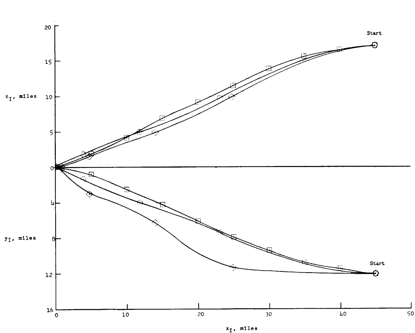
Figure 11.- Position trajectories of pilots for rendezvous conditions of case 4 (table 1).
