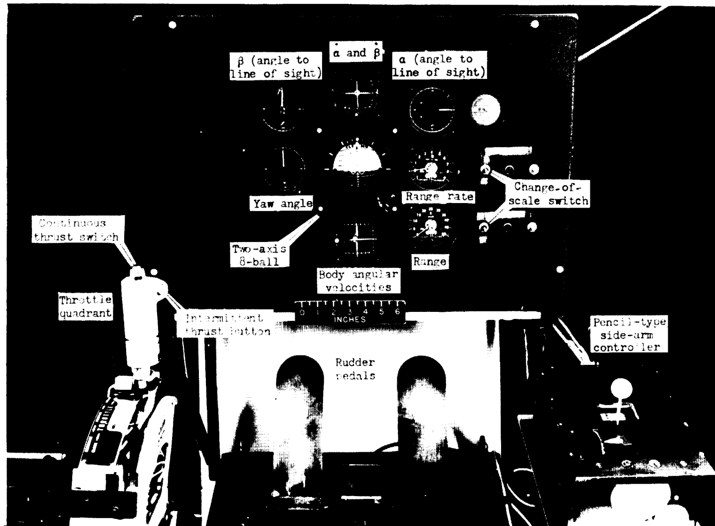
Figure 4.- Photograph of cockpit display.
