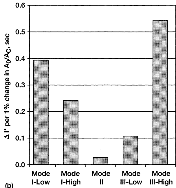
Figure 12.—Reference vehicle air capture. (a) Air capture ratio at free stream and station 1 showing the effect of forebody compression. (b) Sensitivity of I^* to a 1% change in air capture.
