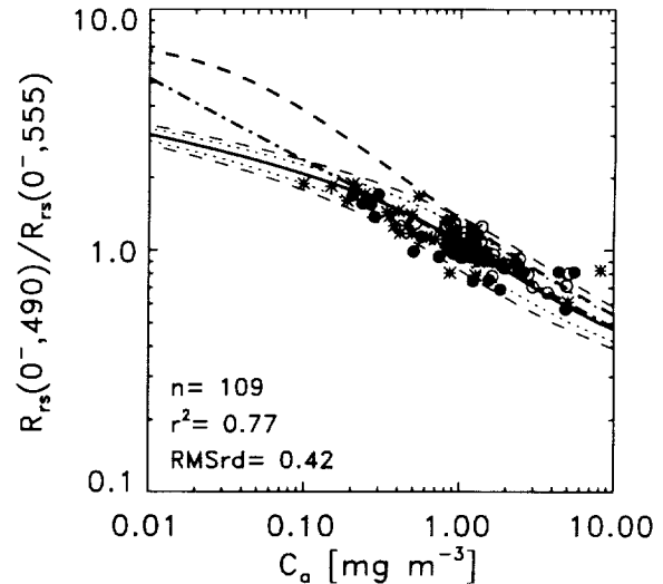
Fig. 11. Relationships between the remote sensing reflectance ratio ( 0^- depth) R_{rs}(490)/R_{rs}(555) and C_a . Filled and empty circles represent the Case-2 and Case-1 situations, respectively (according to Loisel and Morel 1998), whereas the stars represent the unidentified situations. The thick solid line represents the polynomial fit (see text), the thick dotted-dashed line the linear fit. The dotted and dashed thin lines represent a factor of \pm 1.5 and \pm 2 around the fit, respectively. The thick dashed line is the SeaWiFS OC2v4 algorithm.
