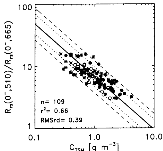
Fig. 12. Relationships between the remote sensing reflectance ratio (0 - depth) R_{rs}(510)/R_{rs}(665) and C_{TSM} . The solid line represents the linear fit (see text). The thin dotted and dashed lines and symbols are as in Fig. 11.
