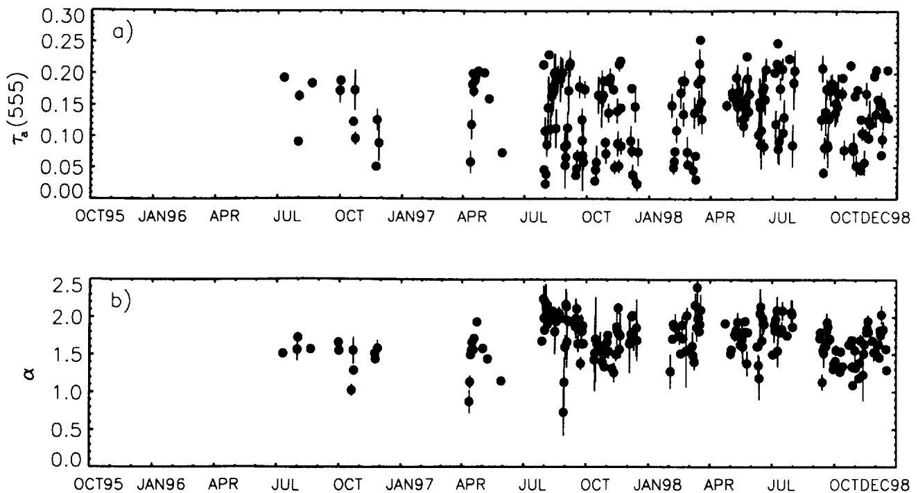
Fig. 3. Time-series of a) the aerosol optical thickness \tau_a , at 555 nm, and b) the Ångström exponent \alpha . Filled circle and black lines represent the daily averages and standard deviations, respectively.
