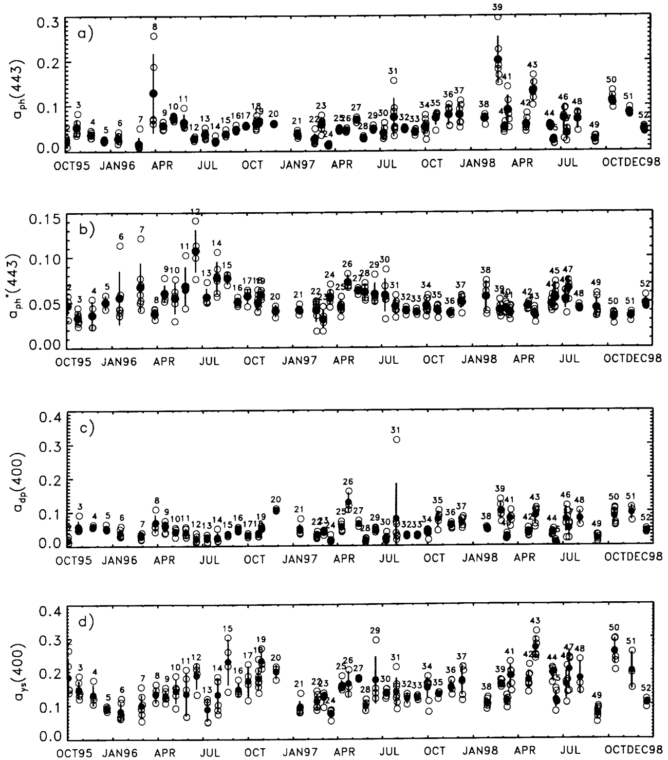
Fig. 7. Time series, for near-surface samples, of a) the absorption coefficient of pigmented particulate matter a_{ph} , at 443 nm in per unit meters; b) the corresponding chlorophyll a -specific absorption coefficient a_{ph}^*(443) in meters square per milligram of chlorophyll a ; c) the absorption coefficient of nonpigmented particulate matter a_{dp} at 400 nm in per unit meters; and d) the absorption coefficient of colored dissolved organic matter a_{ys} , at 400 nm in per unit meters. The symbols and lines are as in Fig. 1.
