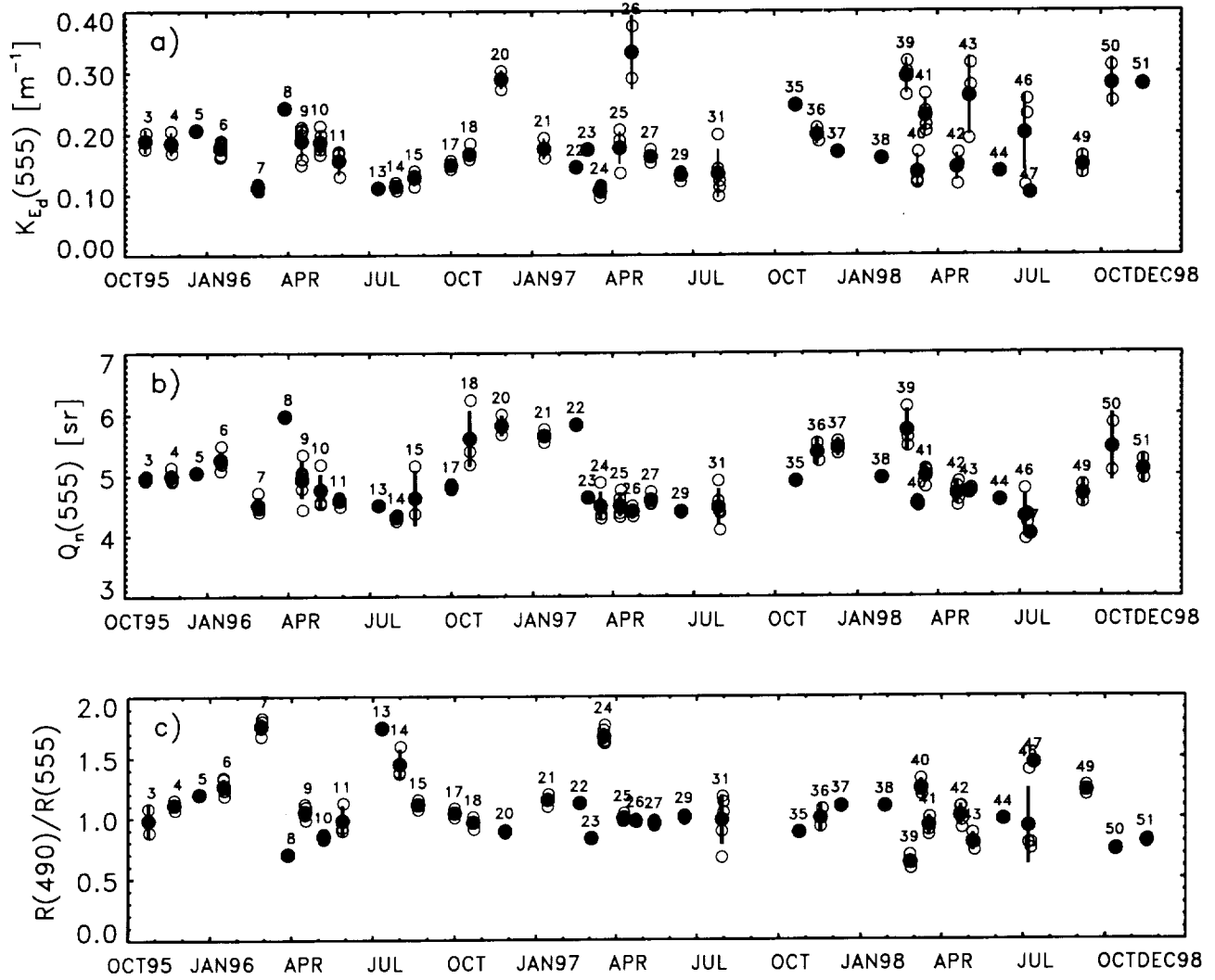
Fig. 9. The time-series' of a) K_{E_d}(555) computed for an optically homogeneous near-surface layer; b) the surface ( 0^\circ ) Q_n factor at 555 nm, and c) the surface ( 0^\circ ) reflectance ratio R(490)/R(555) . The symbols and lines are as in Fig. 1.
