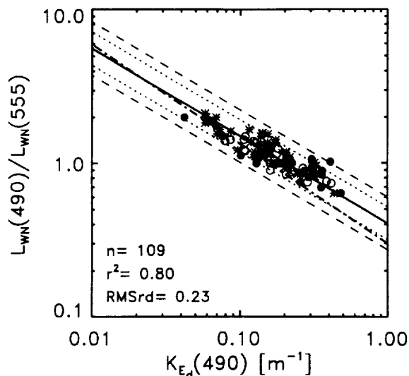
Fig. 13. The relationship between the normalized water-leaving radiance ratio L_{WN}(490)/L_{WN}(555) and the diffuse attenuation coefficient K_{E_d}(490) . The solid line represents the fitted power function, the dotted and dashed lines represents a factor of \pm 1.5 and \pm 2 around the fit, respectively. The dotted and dashed line represents the Mueller (2000) algorithm. The symbols are as in Fig. 11.
