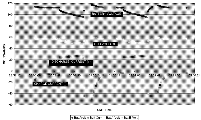
FIGURE 7. BATTERY 4B2 VOLTAGE AND CURRENT
