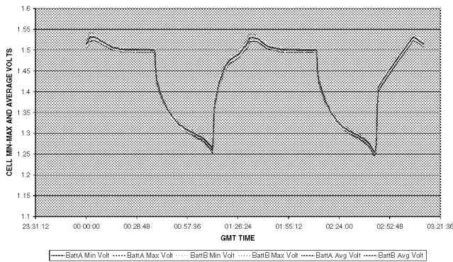
FIGURE 8. BATTERY 2B2 CELL VOLTAGES
