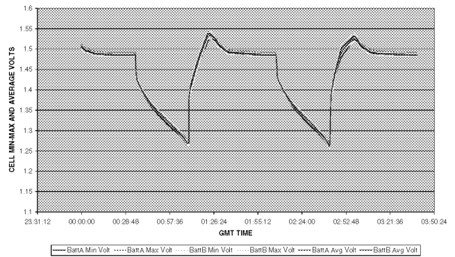
FIGURE 9. BATTERY 4B2 CELL VOLTAGES
