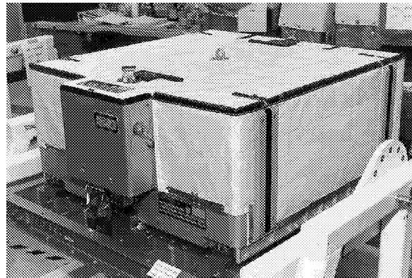
FIGURE 2. ISS BATTERY SUBASSEMBLY ORU WITH MLI BLANKET
