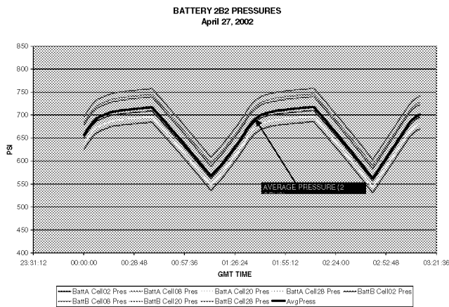
FIGURE 12. BATTERY 2B2 PRESSURES
