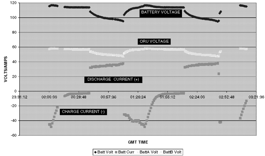
FIGURE 6. BATTERY 2B2 VOLTAGE AND CURRENT
