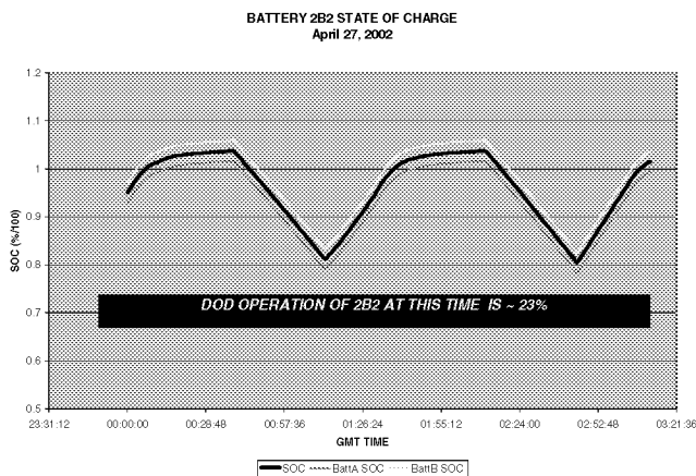
FIGURE 14. BATTERY 2B2 SOC
