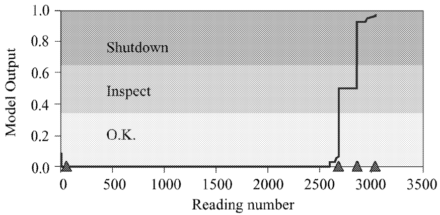
Figure 9: Experiment 3 Features and Model Output
