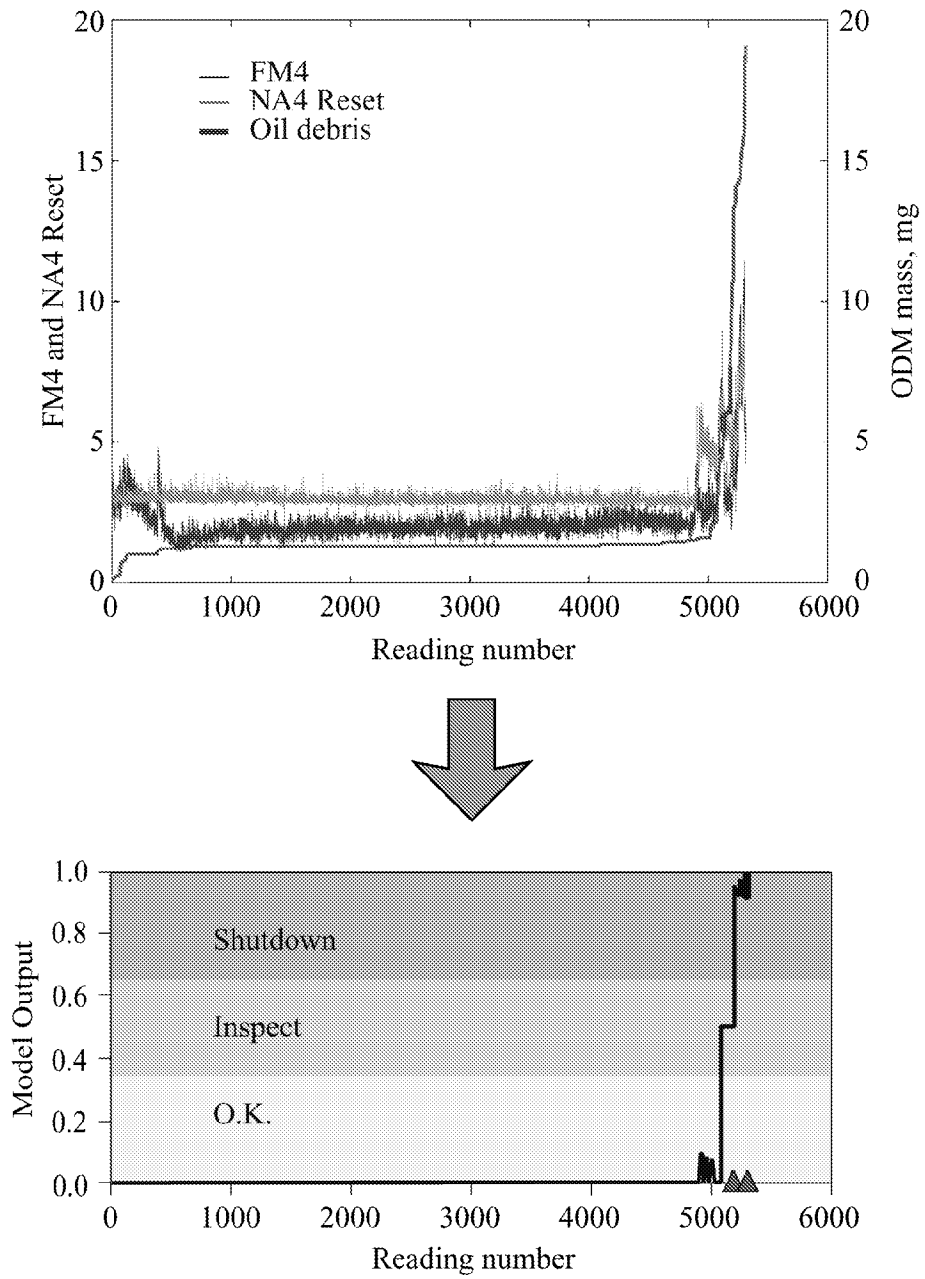
Figure 11: Experiment 8 Features and Model Output
