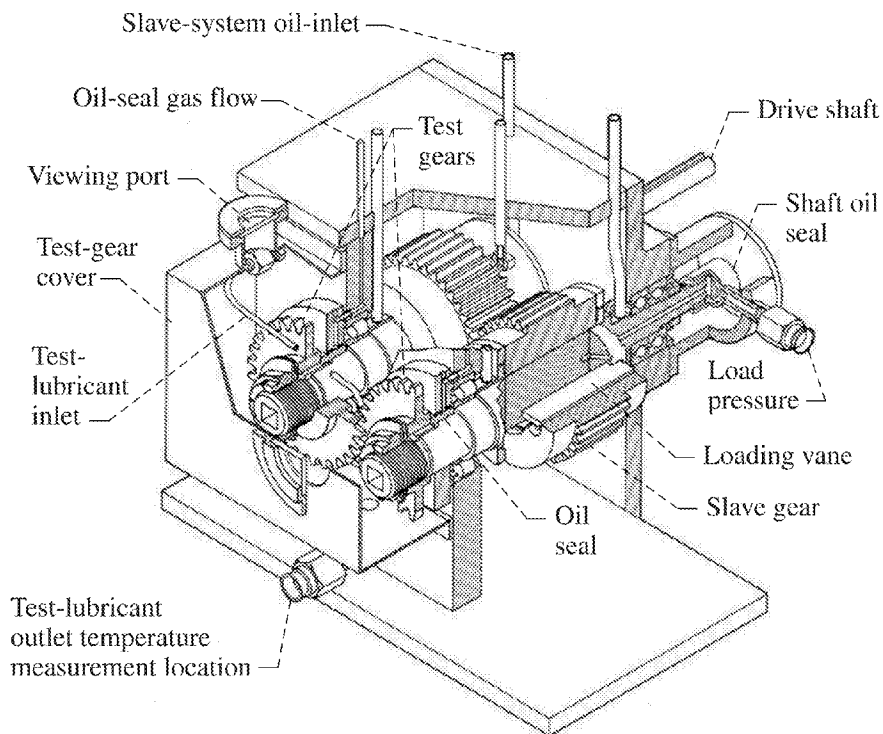
Figure 1: Spur Gear Fatigue Rig Gearbox
