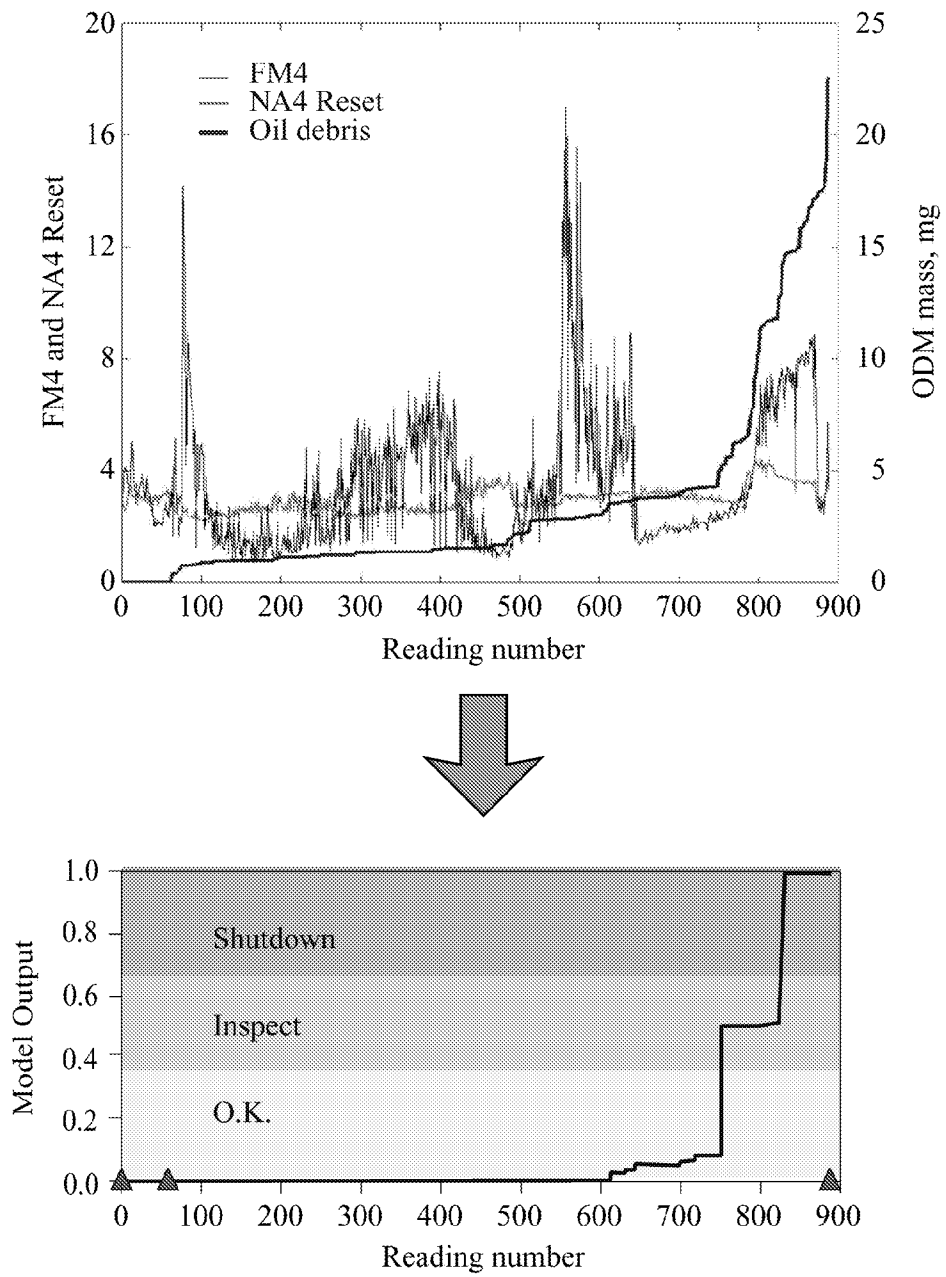
Figure 12: Experiment 18 Features and Model Output
