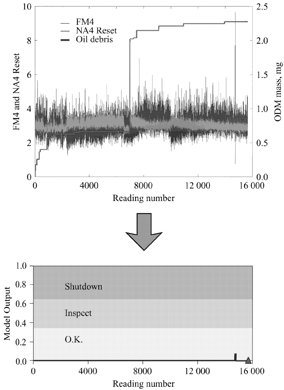
Figure 10: Experiment 12 Features and Model Output
