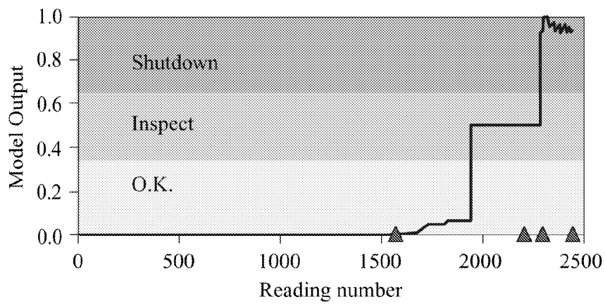
Figure 8: Experiment 2 Features and Model Output
