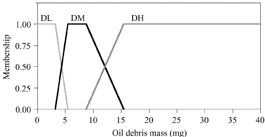
Figure 4: Membership Values for Oil Debris Feature
