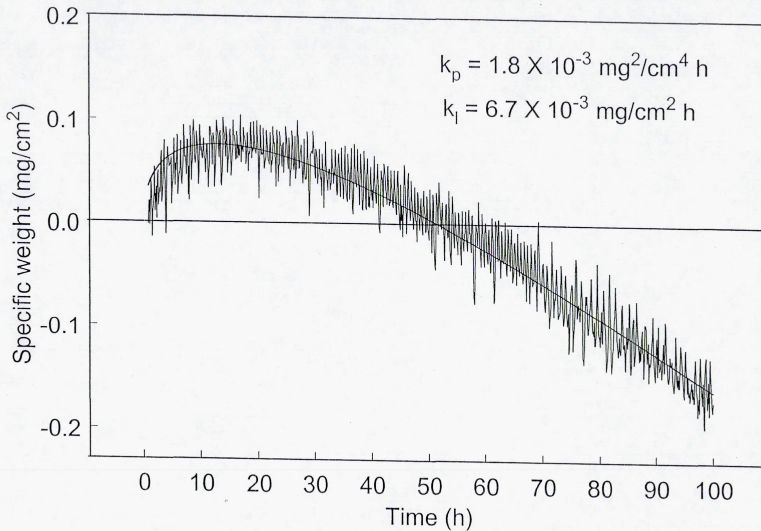
Fig. 7. Parabolic weight change kinetics for AS800 \text{Si}_3\text{N}_4 at 1200^\circ\text{C} in 50% \text{H}_2\text{O} - 50% \text{O}_2 flowing at 4.4 cm/s.
