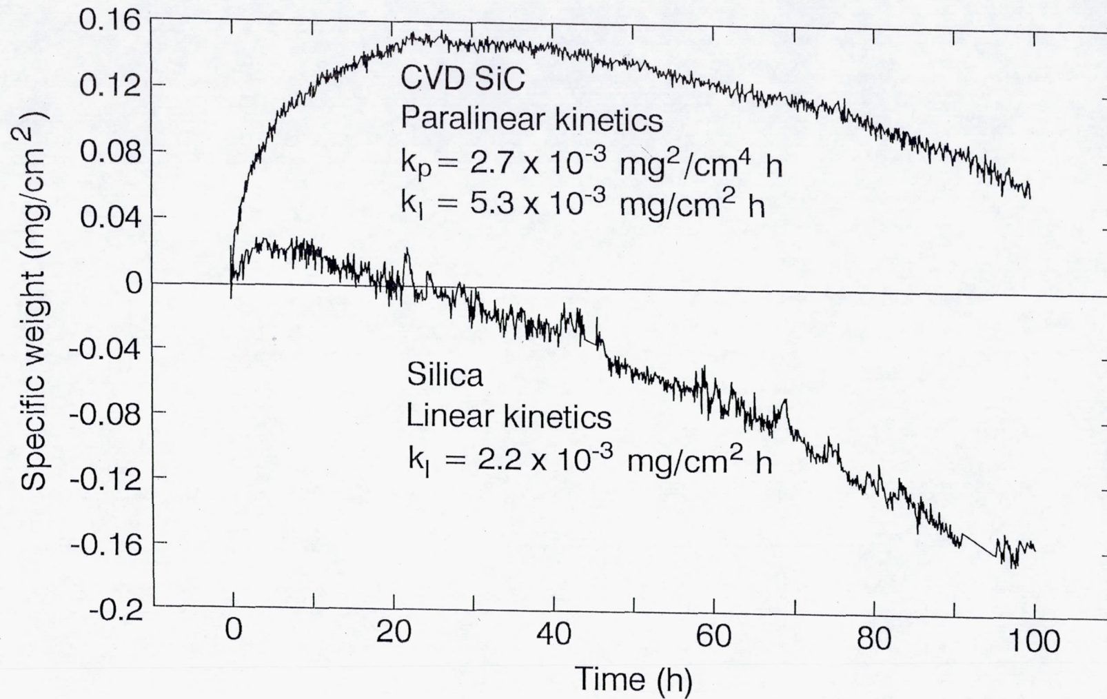
Fig. 1. Paralinear kinetics of CVD SiC and linear kinetics of fused quartz at 1200°C in 50% H 2 O - 50% O 2 flowing at 4.4 cm/s (adapted from Ref. 13).
