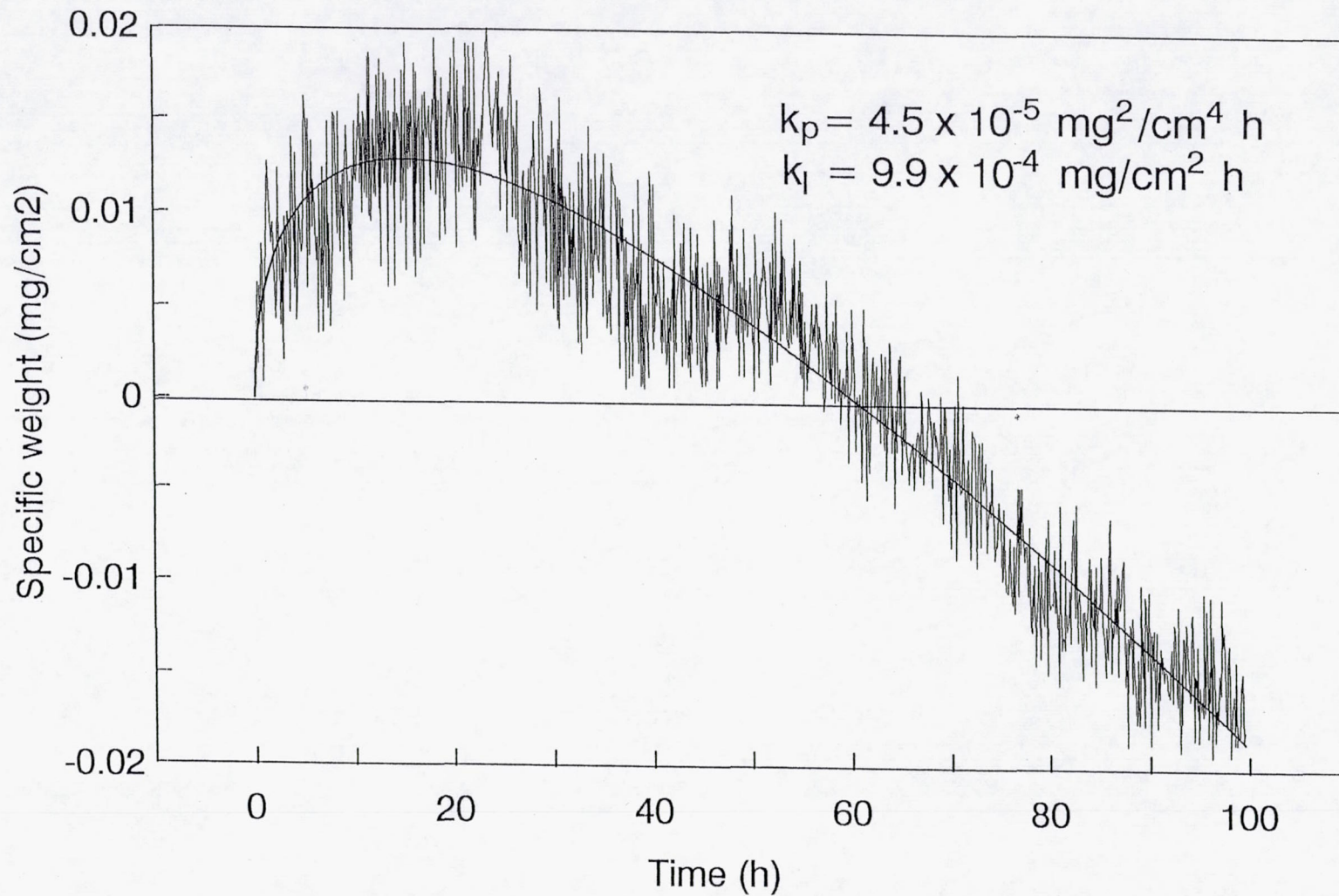
Fig. 6. Paralineer weight change kinetics for SN282 Si 3 N 4 at 1200°C in 50% H 2 O - 50% O 2 flowing at 4.4 cm/s
