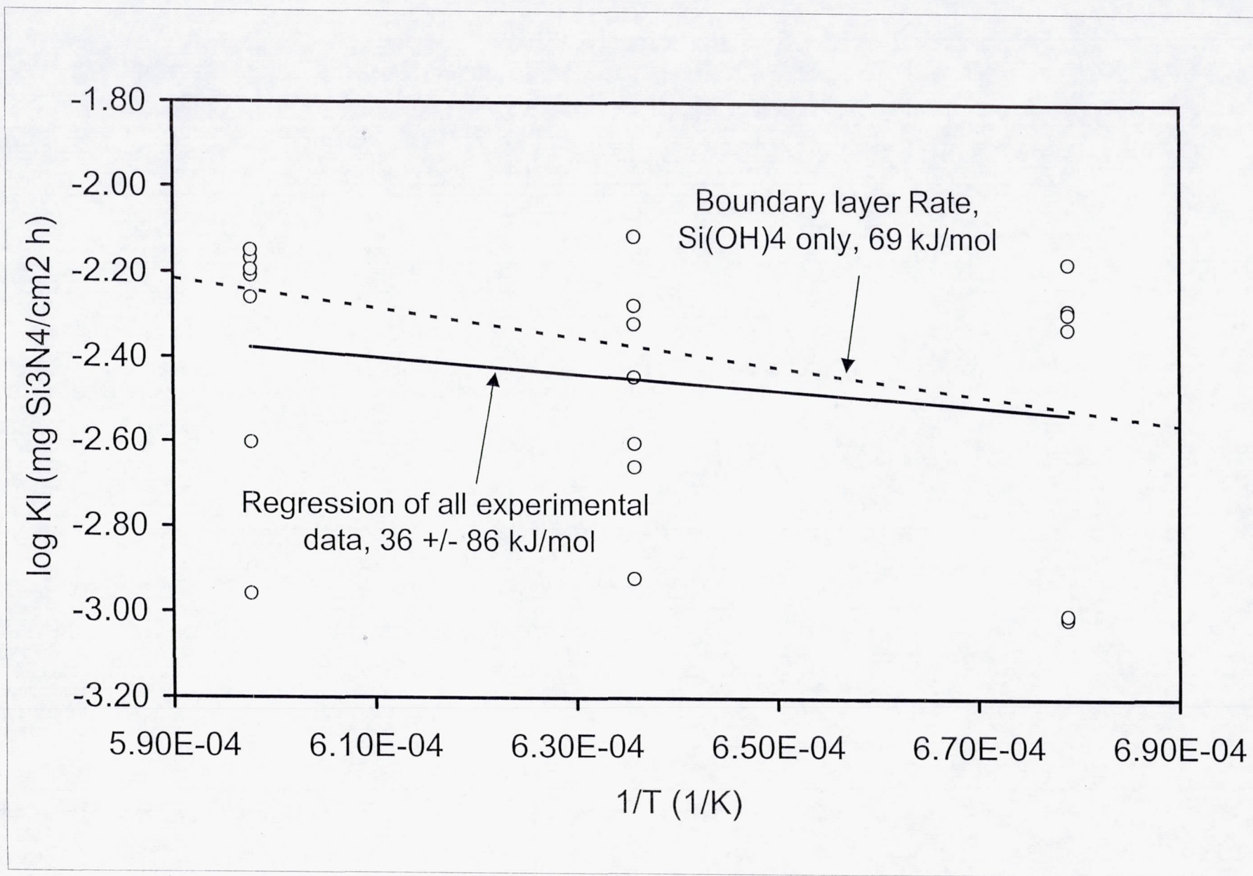
Fig. 8. Linear rate constants ( k_1 ) for all three \text{Si}_3\text{N}_4 materials in 50% \text{H}_2\text{O} - 50% \text{O}_2 flowing at 4.4 cm/s.
