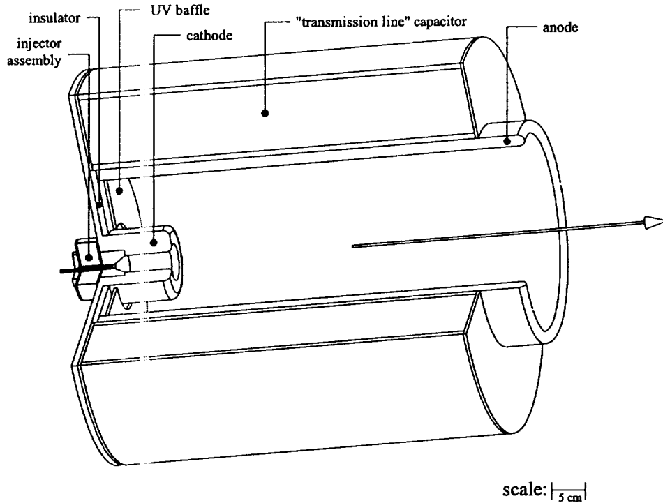
Figure 1: Schematic of the PRC-PPT1 geometry and components (sectioned to show inner detail.)
