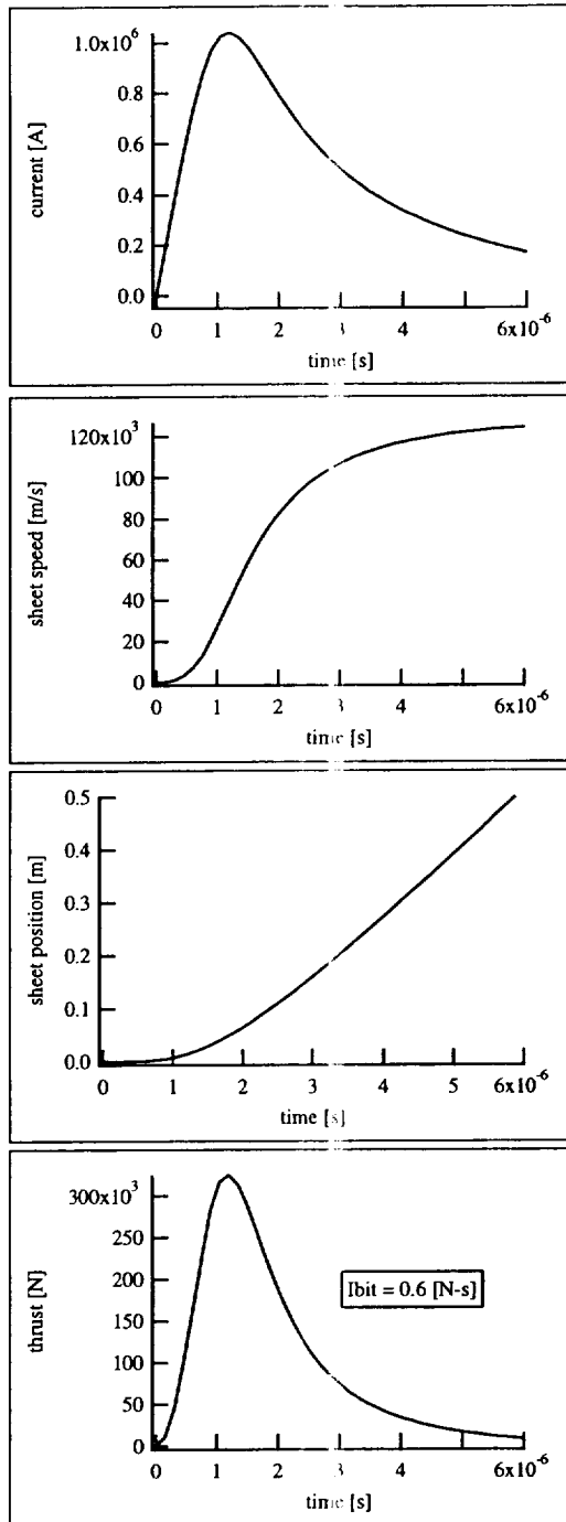
Figure 6: Results of 0-d analysis: current, sheet speed, sheet position, and thrust as a function of time.
