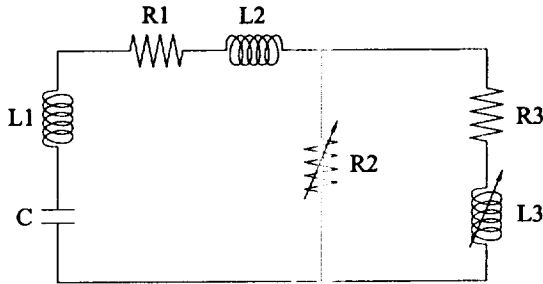
Figure 5: Computational circuit elements of PTC1.
