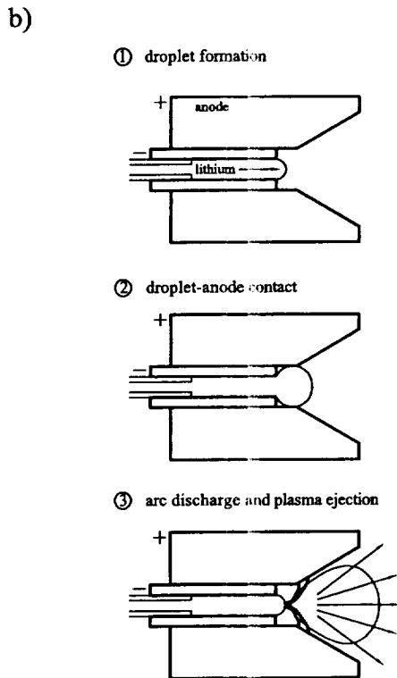
Figure 2: PRC-PPT1 propellant feed system: a) diagram of liquid lithium feed system, b) first stage droplet formation and plasma ejection sequence.
