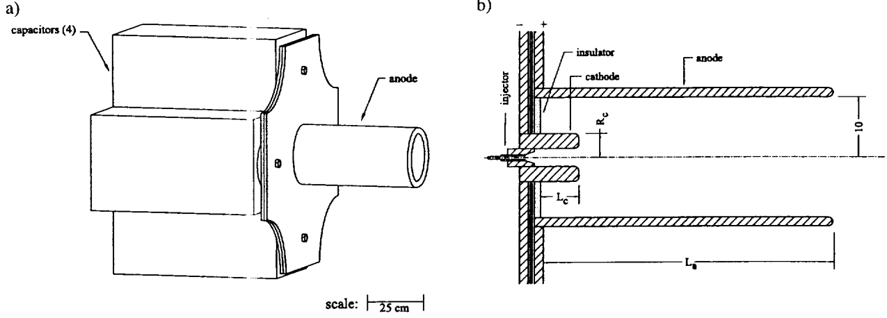
Figure 4: a) Isometric view of complete PRC-PPT1a assembly, b) Cross-section of PRC-PPT1a discharge chamber.
