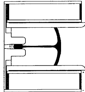
Figure 3: Conceptual evolution of current sheet in second stage of PRC-PPT1: initiation, pinching, and acceleration with virtual cathode.
