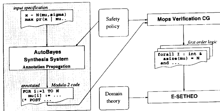
Fig. 1. The AUTOBAYES/CC system architecture
