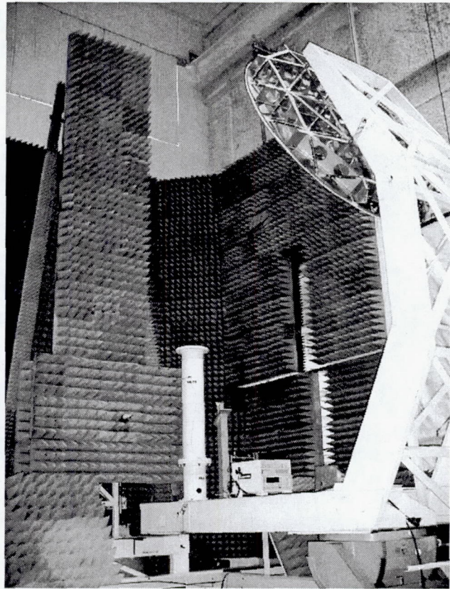
Figure 2 - 2.7m Reflector Antenna in the Planar Near-Field Facility.
