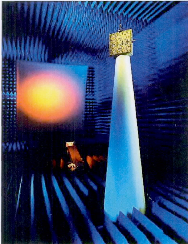
Figure 9 - Interior of the Compact Range Facility.
