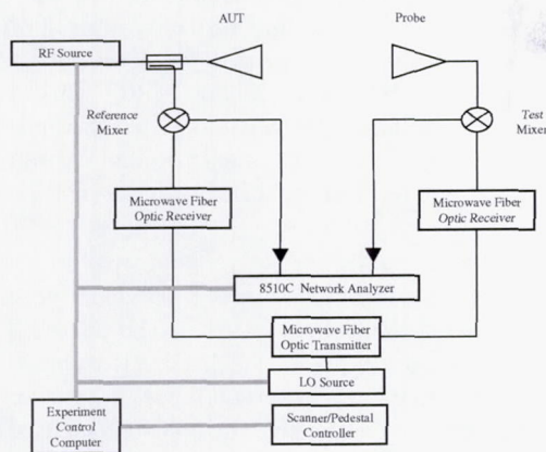
Figure 3 - Measurement Configuration for the Planar Near-Field Facility.
