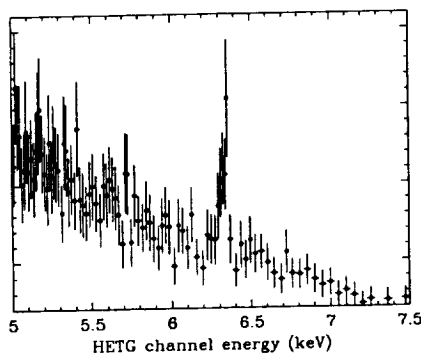
Figure 4. HETG spectrum of the Fe K\alpha line in MCG–5-23-16.
