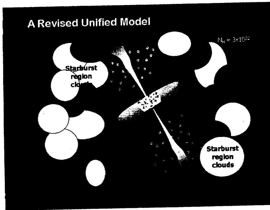
Figure 18. Cartoon of a revised unified model, which includes a central AGN surrounded by the standard pc-scale Compton-thick torus plus an obscuring region of \sim 50 pc diameter of dense molecular clouds ( N_H = 10^{22-23} \text{ cm}^{-2} ) associated with a circumnuclear starburst.
