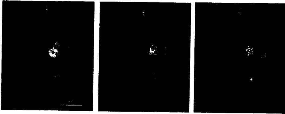
Figure 11. Soft, medium and hard-band adaptively smoothed (false-color) images of NGC 253. Image size is 1.1' \times 1.4' . Ultraluminous X-ray point sources are numbered, including the core (#2).
