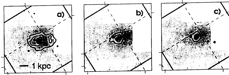
Figure 9. ACIS-S contours overlaid on an optical HST image of NGC 4579. Image size is \sim 1.2' \times 1.2' ( \sim 10 \text{ kpc} \times 10 \text{ kpc} ). Energy bands are a) 0.2–1.5 keV, b) 1.5–2.5 keV and c) 2.5–8.5 keV.
