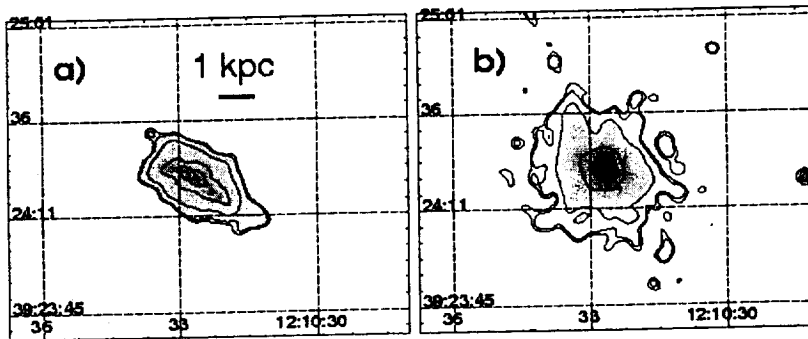
Figure 7. Unbinned and adaptively smoothed greyscale Chandra images of NGC 4151 with contours overlaid. Image sizes are 1.8' \times 1.4' ( 9.7 \text{ kpc} \times 7.6 \text{ kpc} ) and are shown for energy bands a) 0.2–1.5 keV (soft) and b) 2.5–8.5 keV (hard).
