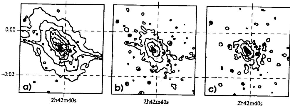
Figure 2. Contours for adaptively smoothed images of NGC 1068 for energy bands a ) 0.2–1.5 keV, b ) 1.5–2.5 keV and c ) 2.5–8.5 keV. Image size is 4' \times 4' ( 26.4 \text{ kpc} \times 26.4 \text{ kpc} for H_0 = 50 \text{ km s}^{-1} \text{ Mpc}^{-1} ).
