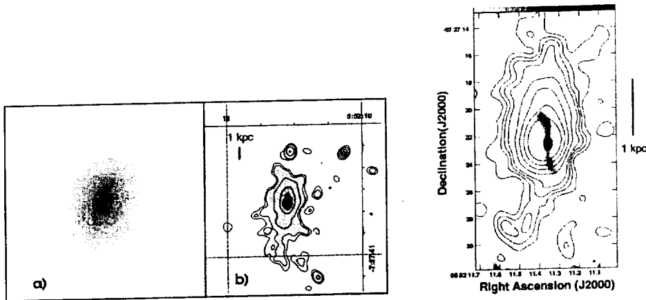
Figure 3. a) HST WFPC image of NGC 2110 compared with b) the soft X-ray Chandra contours (0.2–1.5 keV). The image sizes are 60'' \times 63'' and the X-ray image in b) is smoothed to a resolution of 2'' . c) Enlargement of the central region showing the nuclear soft X-ray contours overlaid on the 6 cm radio map (Ulvestad & Wilson 1983).
