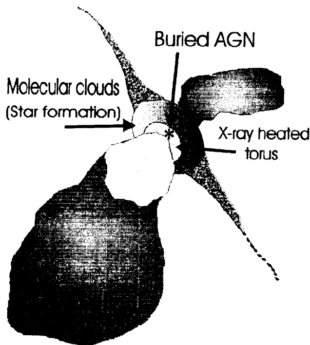
Figure 17. Cartoon of the central kpc of a starburst-AGN composite (“energetic”) galaxy.
