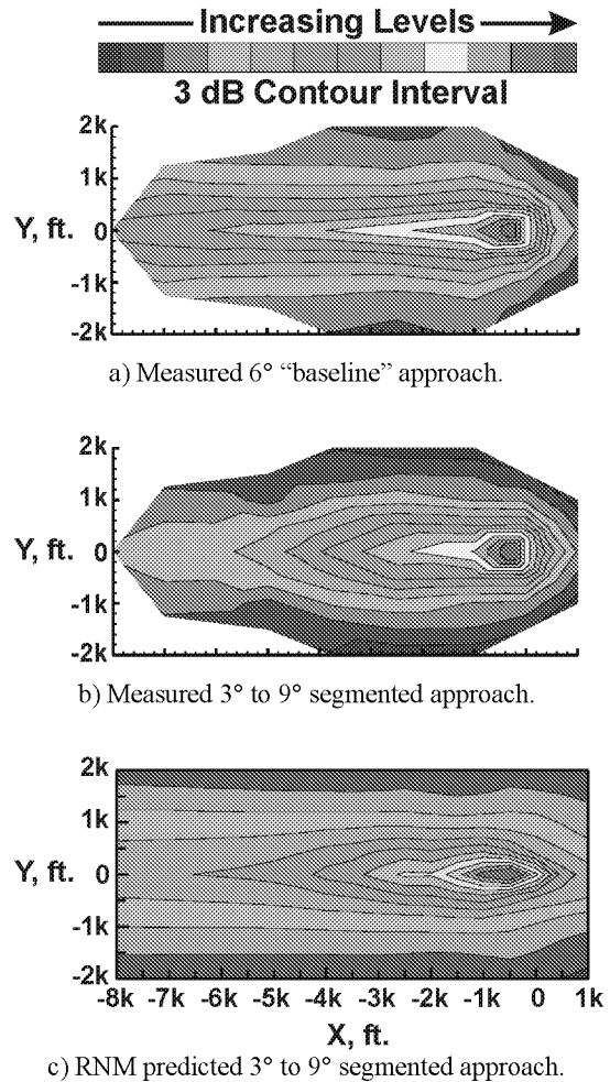
Figure 7. XV-15 ground noise footprints.
