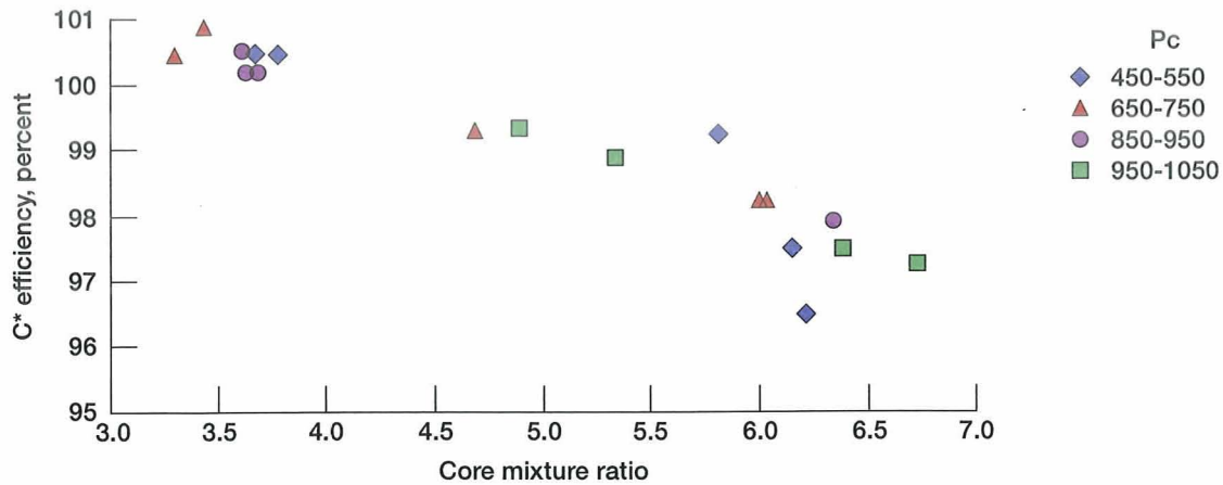
Figure 8.—C* efficiency as a function of core mixture ratio for the fully mixed analysis with data grouped by chamber pressure range.
