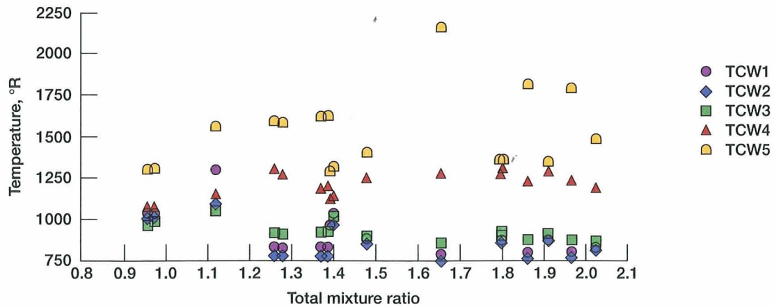
Figure 12.—Wall temperatures as a function of total mixture ratio.
