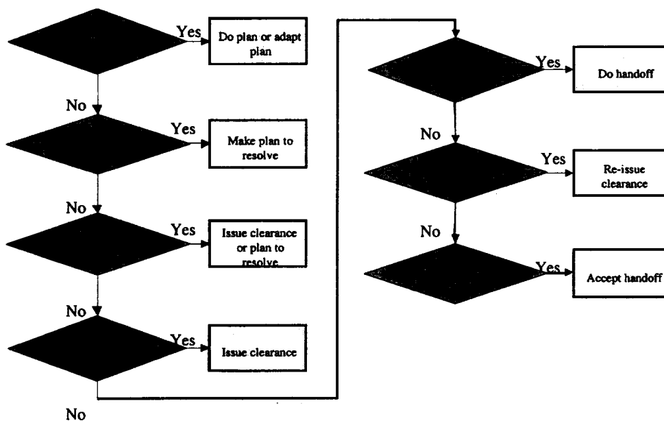
Figure 8. Flow of control resulting from the CATS model used by the CATS ATC agents.
