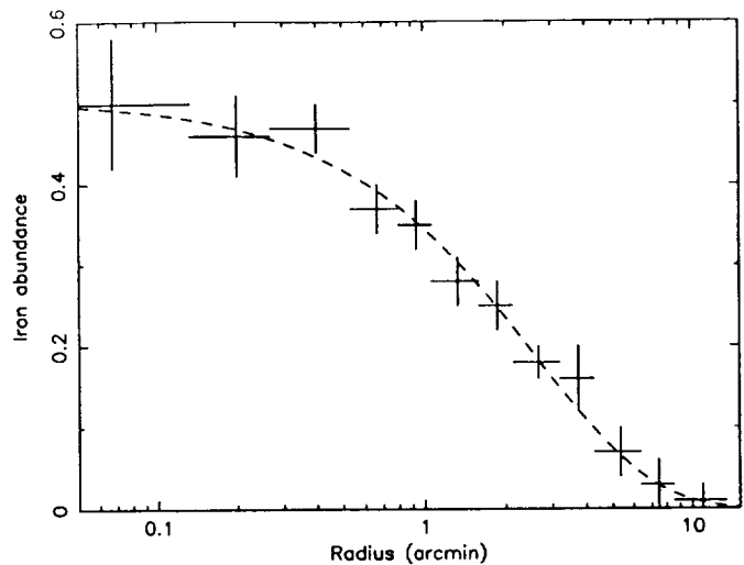
Fig. 2. Radial abundance profile of Sérsic 159-03. The dashed line is the best-fit exponential model (see text).
