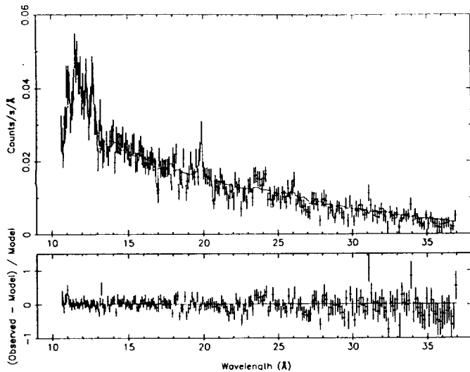
Fig. 6. RGS1 spectrum of Sérsic 159-03 with the best fit two components model.
