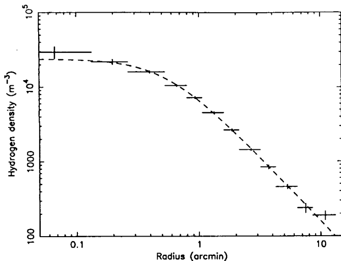
Fig. 1. Radial density profile of Sérsic 159-03. The dashed line is the best-fit \beta -model (see text).
