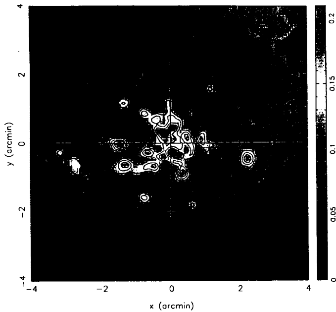
Fig. 4. Fe-L equivalent line width in keV. Contours are separated by 0.02 keV. The statistical uncertainty is about 0.02, 0.05 and 0.1 keV at a distance of 0, 1 and 2' from the core, respectively, for a box of 16'' \times 16'' .
