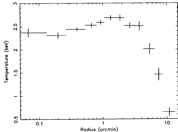
Fig. 3. Radial temperature profile of Sérsic 159-03.
