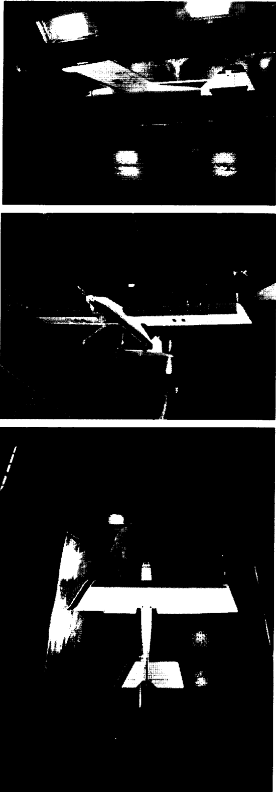
Figure 1 Free-flying Airplane for Sub-scale Experimental Research (FASER) in the NASA Langley 12 ft Low-Speed Wind Tunnel
