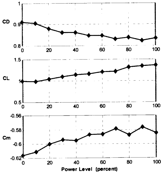
Figure 5 Power Sweep for Subspace Boundary Definition, \alpha=40 , \beta=0
