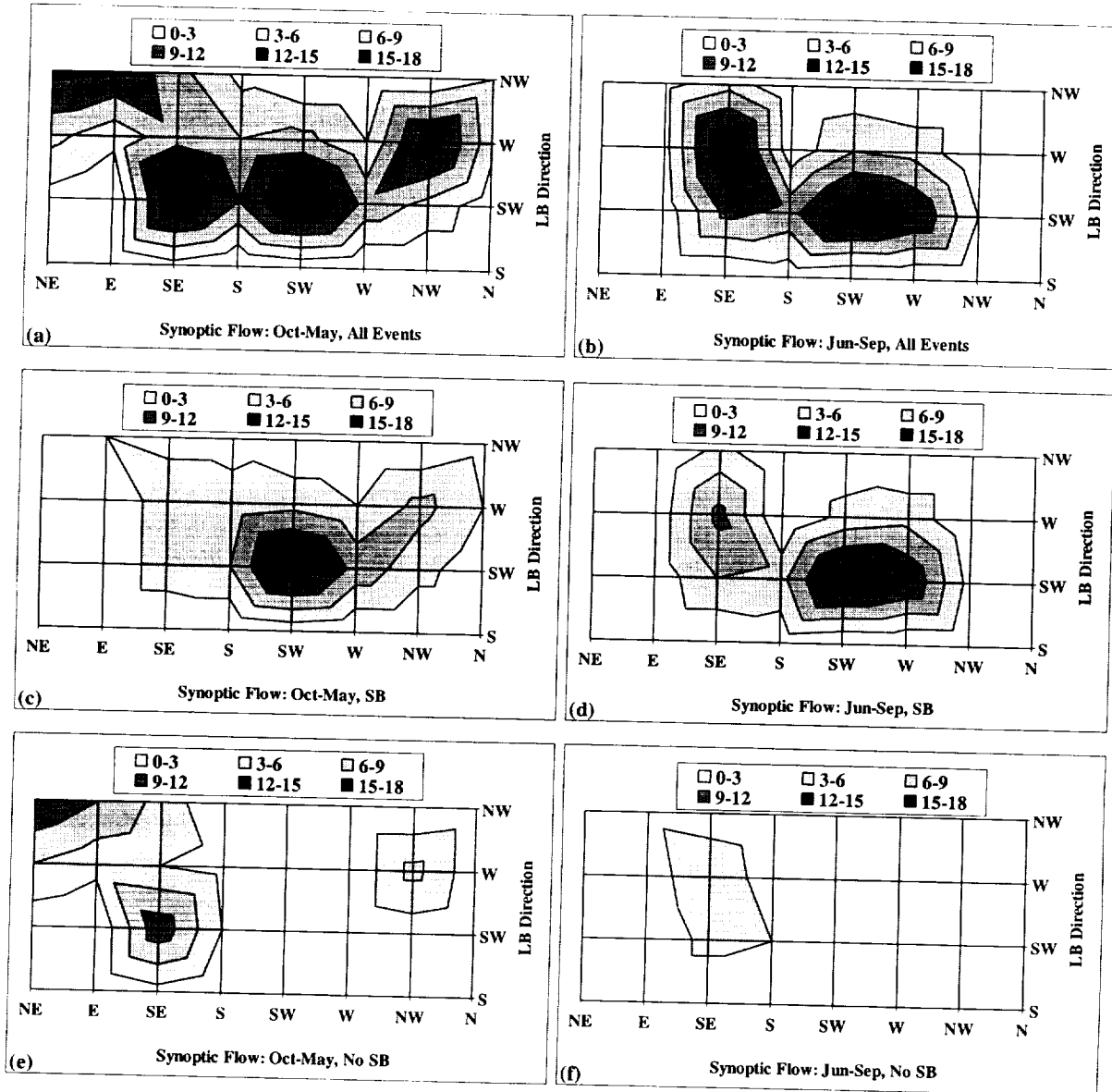
Figure 5.5. The frequency distributions of land-breeze directions from February 1995 to January 2002 as a function of the synoptic flow direction, based on a categorization of events into MC (October to May) versus PC months (June to September) and events with and without a preceding sea breeze (SB). All events are shown for the months of (a) October to May, and (b) June to September. Events preceded by a sea breeze are shown in (c) October to May, and (d) June to September. Events without a preceding sea breeze are shown in (e) October to May, and (f) June to September.
