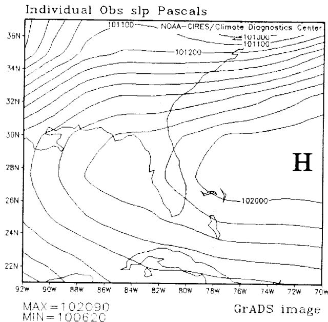
Figure 3.9. NCEP/NCAR reanalysis map of mean sea-level pressure over the southeastern U.S. at 0000 UTC 7 April 2000. The contour interval is 100 Pa (1 mb) with the maximum and minimum values indicated in the lower left.
