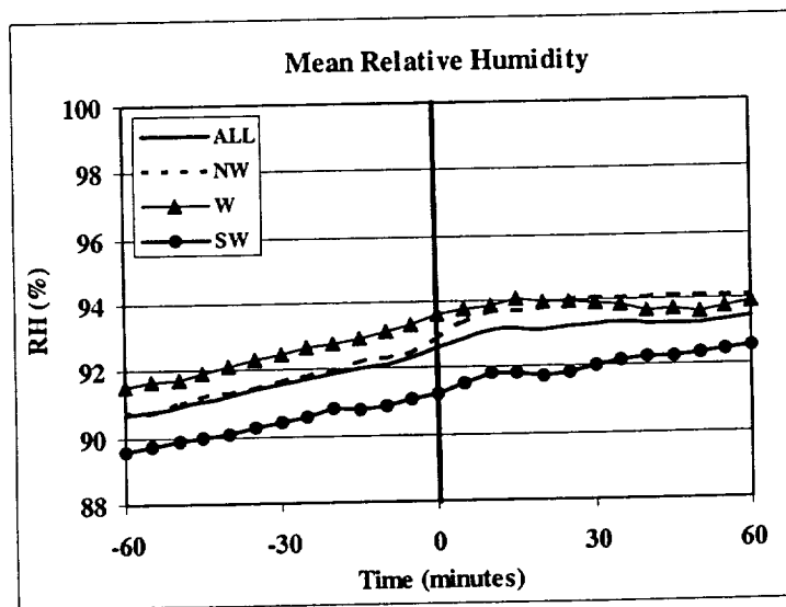
Figure 4.9. Five-minute mean 6-ft relative humidity variations at \pm 60 minutes relative to land-breeze passages for all land breezes (ALL), and for events with post-land breeze winds from the northwest (NW), west (W), and southwest (SW), valid during October to May. The bold vertical line at 0 minutes in each panel represents the time of the land-breeze passage.
