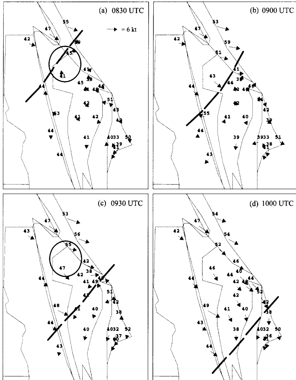
Figure 3.6. KSC/CCAFS tower observations of winds and 6-ft temperatures for 6 April 2000, valid at (a) 0830 UTC, (b) 0900 UTC, (c) 0930 UTC, and (d) 1000 UTC. The winds are given by arrows, with the tail centered on each station [speed scale provided in panel (a)], and 6-ft temperatures are plotted above the wind arrows. Thick dashed lines denote the location of the land-breeze front. The circled towers are discussed in the text.
