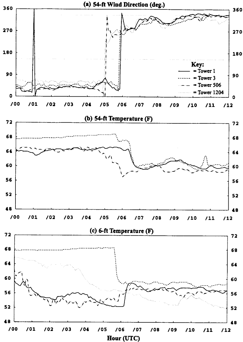
Figure 3.3. Time series plots for KSC/CCAFS Towers 1, 3, 506, and 1204, from 0000 to 1200 UTC 6 March 2000. Variables plotted are (a) 54-ft wind direction, (b) 54-ft temperature, and (c) 6-ft temperature. Note that 54-ft temperatures are not available for Tower 1204. The horizontal dotted lines in panel (a) differentiate between onshore and offshore wind direction. The key is provided in panel (a) and tower locations are shown in Fig. 3.2a.
