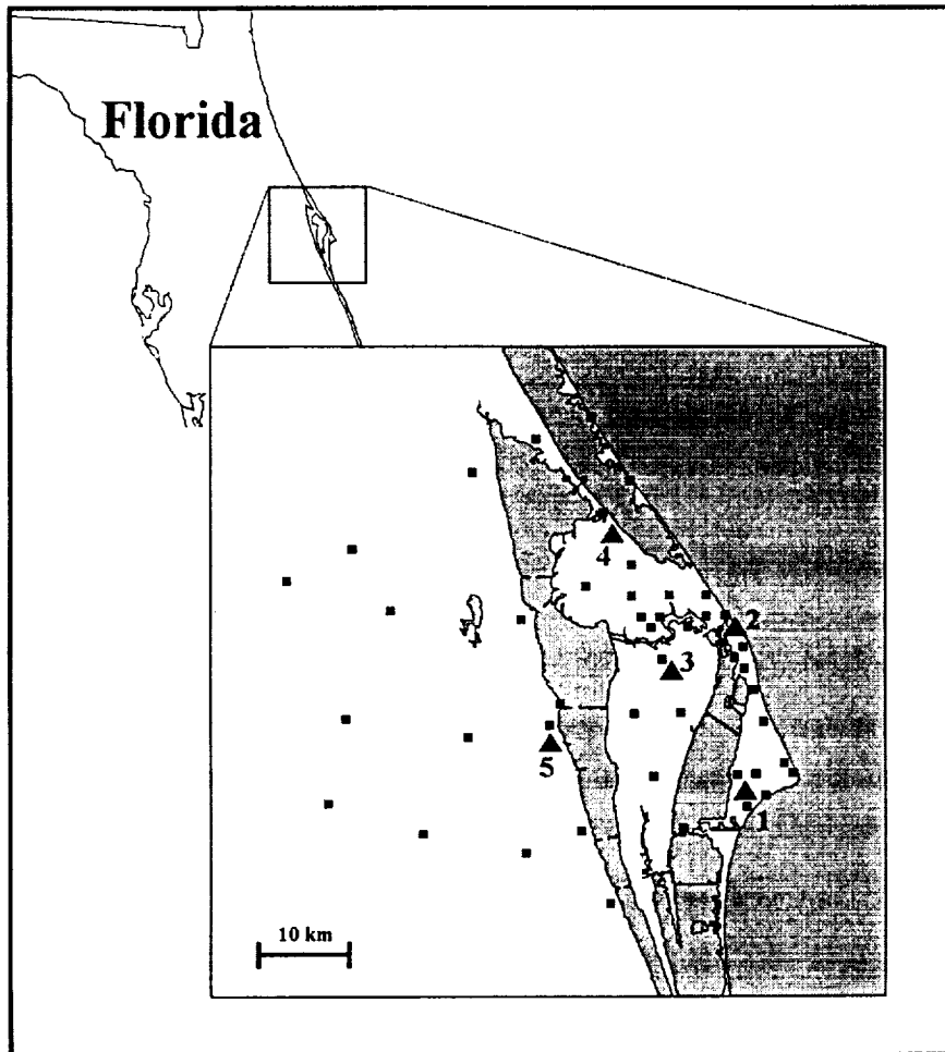
Figure 2.1. The locations of the 44 KSC/CCAFS observational towers (squares) used to study land breezes and develop the seven-year land-breeze climatology over east-central Florida. The locations of the five 915-MHz DRWP sensors are given by triangles and labeled with numbers 1–5.
