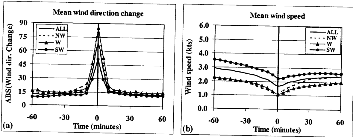
Figure 4.11. Five-minute mean wind variations at \pm 60 minutes relative to land-breeze passages during the PC months (June to September) for all land breezes (ALL), and for events with post-land breeze winds from the northwest (NW), west (W), and southwest (SW). (a) the absolute value of 54-ft wind direction changes (degrees), and (b) the 54-ft wind speed (kt). The bold vertical line at 0 minutes in each panel represents the time of the land-breeze passage.
