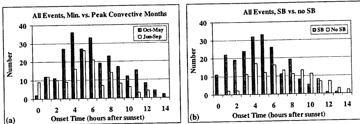
Figure 4.4. The frequency distribution of land-breeze onset times in hours after sunset for (a) minimal convective (October to May) versus peak convective months (June to September), and (b) land-breeze events with a sea breeze during the previous afternoon (SB) versus events without a sea breeze during the previous afternoon (No SB).
