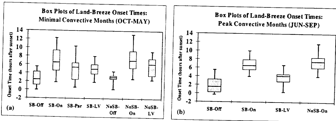
Figure 5.4. Box-plot distributions of the land-breeze onset times under various surface flow regimes during the (a) minimal convective months, and (b) peak convective months. The gray shading in each box plot indicates the onset times that occurred between the 1st and 3rd quartiles of the distribution, and the hatch marks at the top and bottom of each box plot indicate the maximum and minimum, respectively. Box plots are shown only for regimes that had a sample size of at least 10 occurrences according to the data provided in Tables 5.1 and 5.2. The flow regime notations are: SB occurrence with offshore synoptic flow (SB-Off), SB with onshore flow (SB-On), SB with shore-parallel flow (SB-Par), SB with light and variable flow (SB-LV), no SB with offshore flow (NoSB-Off), no SB with onshore flow (NoSB-On), and no SB with light and variable flow (NoSB-LV).
