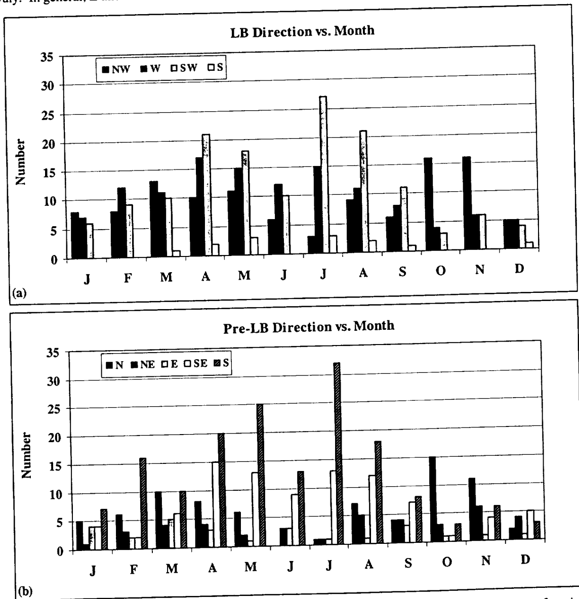
Figure 4.2. The distributions of the post-land breeze and pre-land-breeze wind direction as a function of month. (a) The monthly distributions of post-land-breeze directions for all events, and (b) the monthly distributions of pre-land-breeze directions for all events from February 1995 to January 2002. The land-breeze direction is given by the mean wind for one hour following the land-breeze frontal passage at all towers that experienced a land-breeze frontal passage.
