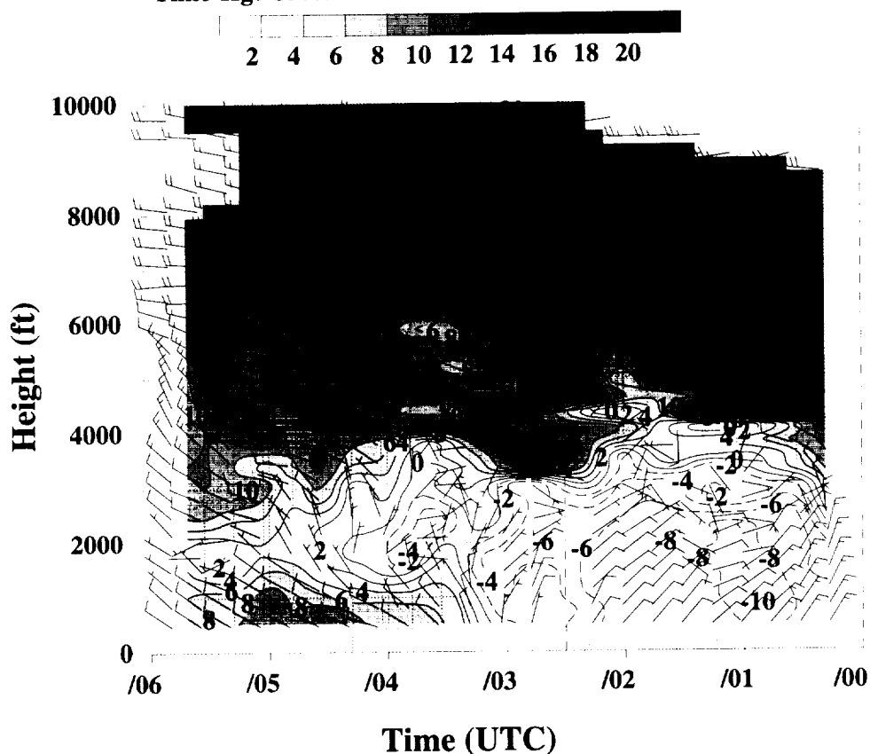
Figure 3.16. Time-height cross section of wind vectors and contoured u-wind component at the 915-MHz DRWP #3 from 0000 to 0600 UTC 27 April 2000. Time along the x-axis increases from right to left and height along the y-axis is given in feet. The u-wind component is contoured in 2-kt increments, with positive (westerly) u-winds greater than 2 kt shaded according to the scale provided.
