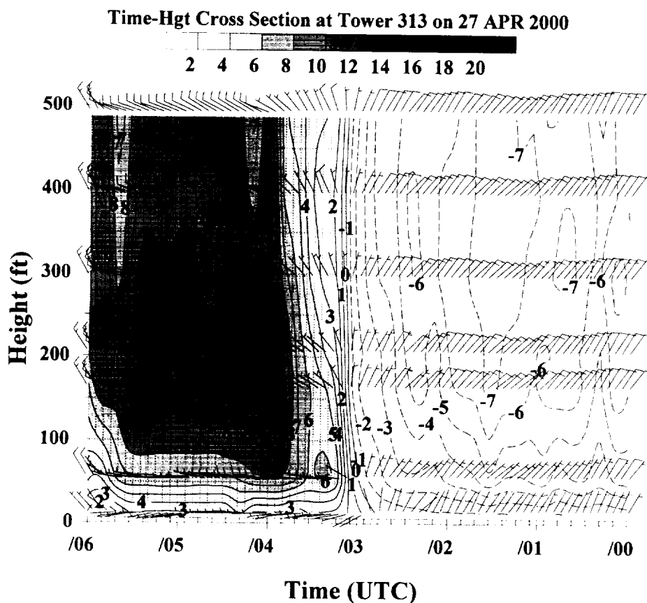
Figure 3.15. Time-height cross section of wind vectors and contoured u-wind component at Tower 313 from 0000 to 0600 UTC 27 April 2000. Time along the x-axis increases from right to left and height along the y-axis is given in feet. The u-wind component is contoured in 1-kt increments, with positive (westerly) u-winds greater than 2 kt shaded according to the scale provided.
