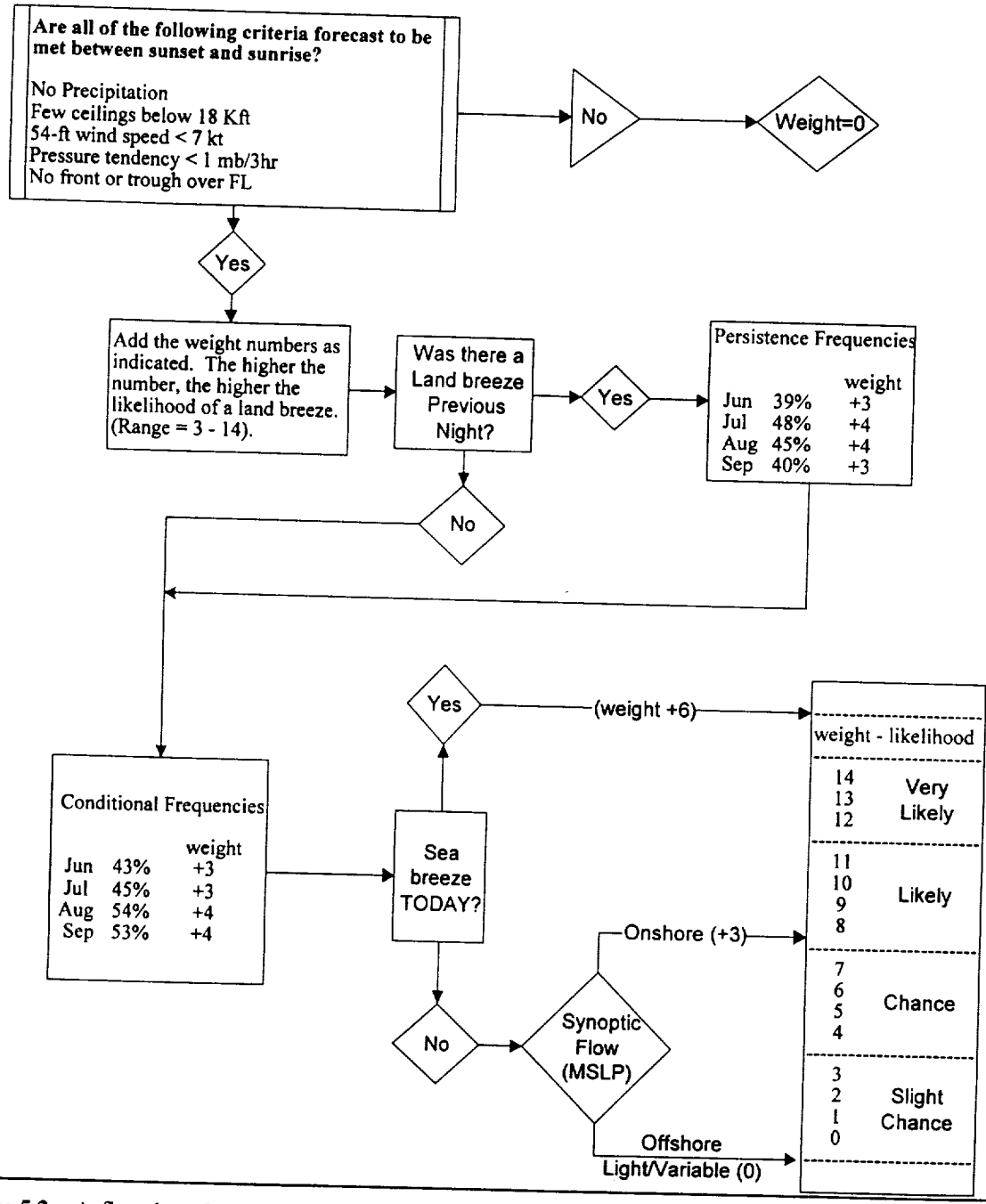
Figure 5.2. A flowchart for determining whether a night has the potential for a land breeze during the PC months. If all initial meteorological conditions are met, then the forecaster follows the logic of the chart and adds all weights together. The final number represents a qualitative measure of the likelihood of a land breeze, ranging from 0 (land breeze least likely) to 14 (land breeze most likely). The flowchart also provides the persistence and conditional frequencies for general land-breeze occurrence during each month, provided that all initial meteorological criteria are met.
