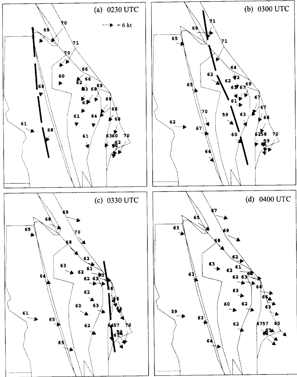
Figure 3.14. KSC/CCAFS tower observations of winds and 6-ft temperatures for 27 April 2000, valid at (a) 0230 UTC, (b) 0300 UTC, (c) 0330 UTC, and (d) 0400 UTC. The winds are given by arrows, with the tail centered on each station [speed scale provided in panel (a)], and 6-ft temperatures are plotted above the wind arrows. Thick dashed lines denote the location of the land-breeze front.
