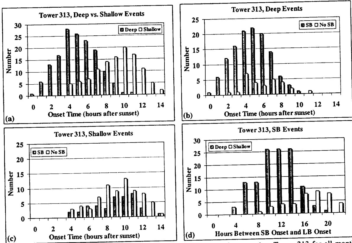
Figure 4.5. The distributions of land-breeze onset times (in hours after sunset) at Tower 313 for all months from February 1995 to January 2002. The distributions are shown for (a) deep (> 492 ft depth) versus shallow (< 150 m depth) circulations, (b) the occurrence (SB) / absence (No SB) of a sea breeze during the afternoon preceding the land breeze for all deep circulations, and (c) SB / No SB during the afternoon preceding the land breeze for shallow circulations. In (d), the distribution of elapsed times between the SB and LB onset times are shown for deep versus shallow events for all land breezes that had a sea breeze during the preceding afternoon.
