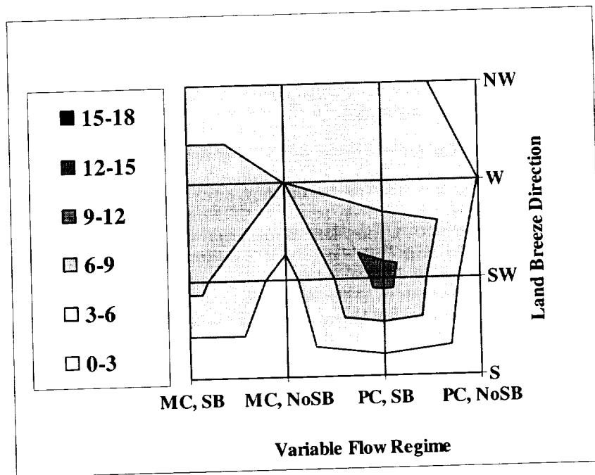
Figure 5.6. The frequency distribution of land-breeze directions from February 1995 to January 2002 for light and variable synoptic flow directions. The land breezes were grouped together for events that occurred during the MC months (October to May) preceded / not preceded by a sea breeze (MC, SB / MC, NoSB), and for events that occurred during the PC months (June to September) preceded / not preceded by a sea breeze (PC, SB / PC, NoSB).
