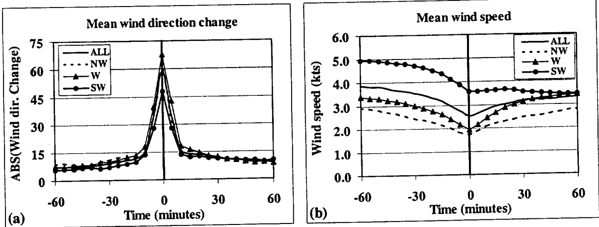
Figure 4.8. Five-minute mean wind variations at \pm 60 minutes relative to land-breeze passages during the MC months (October to May) for all land breezes (ALL), and for events with post-land breeze winds from the northwest (NW), west (W), and southwest (SW). (a) the absolute value of 54-ft wind direction changes (degrees), and (b) the 54-ft wind speed (kt). The bold vertical line at 0 minutes in each panel represents the time of the land-breeze passage.
