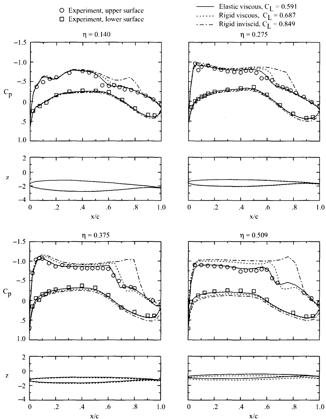
Figure 14. Wing pressure distributions and deformations for wind-tunnel case 4: M_\infty = 0.821 ; \alpha = 1.85^\circ ; R_c = 22 \times 10^6 ; q_\infty = 1788 psf; C_L = 0.537 .
