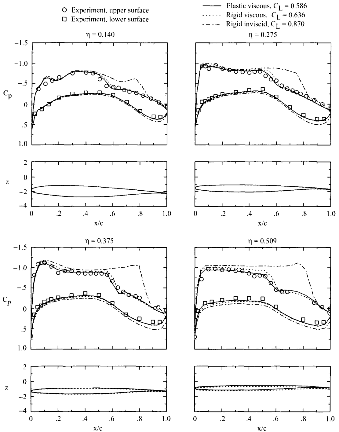
Figure 11. Wing pressure distributions and deformations for wind-tunnel case 1: M_\infty = 0.820 ; \alpha = 1.98^\circ ; R_c = 3 \times 10^6 ; q_\infty = 1052 psf; C_L = 0.527 .
