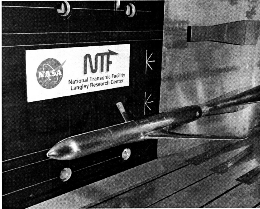
Figure 1. Wing-fuselage configuration of NTF Pathfinder-I lateral controls wing. Spoiler control surface is deflected in photograph.
