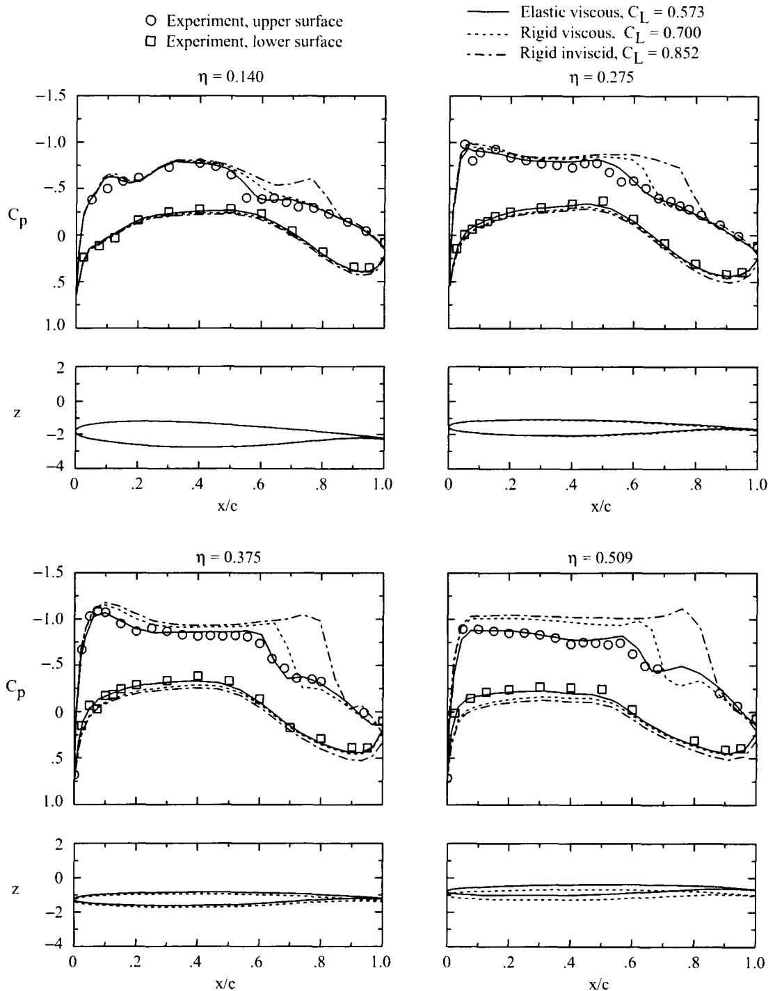
Figure 16. Wing pressure distributions and deformations for wind-tunnel case 6: M_\infty = 0.820 ; \alpha = 1.88^\circ ; R_{\bar{c}} = 30 \times 10^6 ; q_\infty = 2429 psf; C_L = 0.514 .
