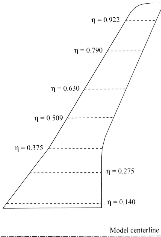
Figure 2. Wing planform sketch with pressure orifice rows.
