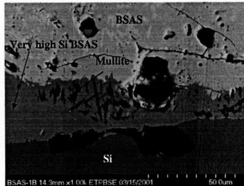
Fig. 2 SEM cross-section micrograph of the BSAS coating after 100 hour laser thermal gradient cycling test. The interface reactions resulted in a dark reaction BSAS layer with high Si concentrations. The mullite phase (very dark needle-shaped phase) precipitation was also found within the high Si reaction BSAS region.
