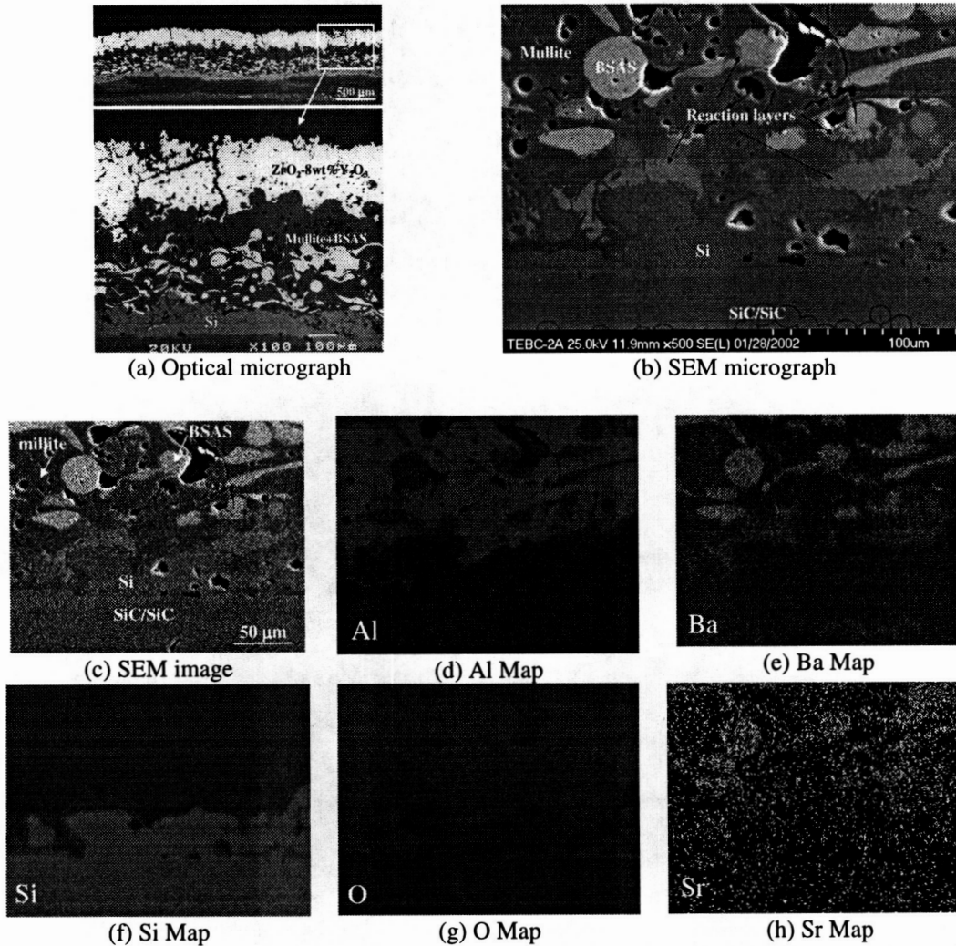
Fig. 3 SEM images and EDS element composition maps of the ZrO_2 -8wt% Y_2O_3 /BSAS+mullite mixture/Si on SiC/SiC ceramic matrix composite substrates after laser testing, showing significant interface reactions between BSAS and bond coat Si layer, and the BSAS and mullite. (a) and (b) Optical and SEM micrographs of the coating after 100 hours testing, showing the surface cracking and interface reactions; and (c) to (h) SEM cross-section
