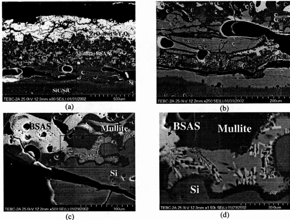
Fig. 5 SEM cross-section micrographs of the ZrO_2-8wt\%Y_2O_3/BSAS+mullite/Si on a SiC/SiC ceramic matrix composite substrate, after total 400 hours testing in the combined laser gradient thermal furnace water vapor through cyclic conditions. (a) Significant interfacial pore formation due to the water vapor attack through the vertical cracks under the thermal gradient cycling conditions. (b) Low melting eutectic phase was also observed near the BSAS-mullite-Si interfaces after the testing.
