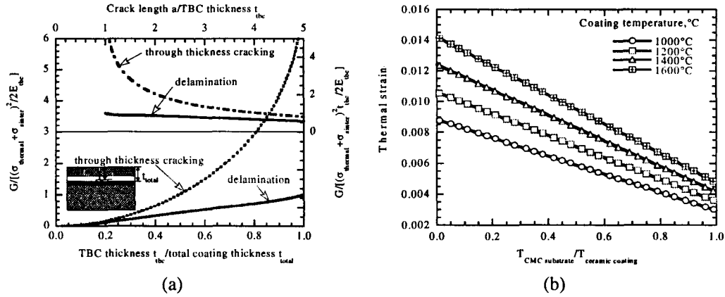
Fig. 4 (a) ZrO_2 - Y_2O_3 TBC layer on mullite-BSAS EBC and CMC substrates, the coating surface cracking and delamination energy release rates can increase significantly with a relatively thick, and larger thermal expansion ZrO_2 - Y_2O_3 TBC layer on mullite-BSAS EBC on CMC substrates. (b) The significantly larger thermal stresses/strains will be generated with increasing the thermal gradients (the temperature difference between the ceramic coating and the substrates).
